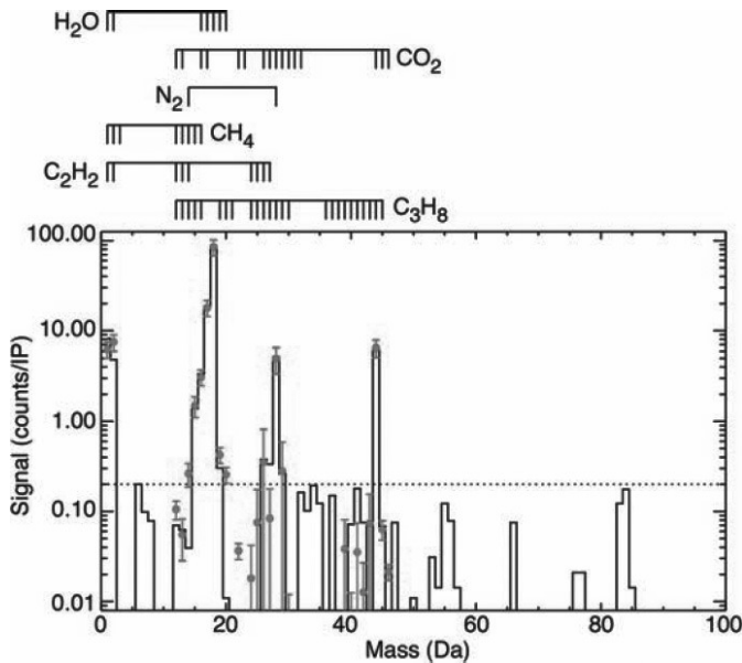
Fig. 6.13. The Cassini Ion and Neutral Mass Spectrometer sampled Enceladus's icy plume during a close flyby on July 14, 2005. It registered molecules whose atomic mass correspond to H 2 O, CO 2 , N 2 , CH 4 (methane), C 2 H 2 (acetylene), and C 3 H 8 (propane). Vertical axis values are counts per integration period. Dotted horizontal line shows the 1- \sigma noise level. From [44]. Reprinted with permission from AAAS.
