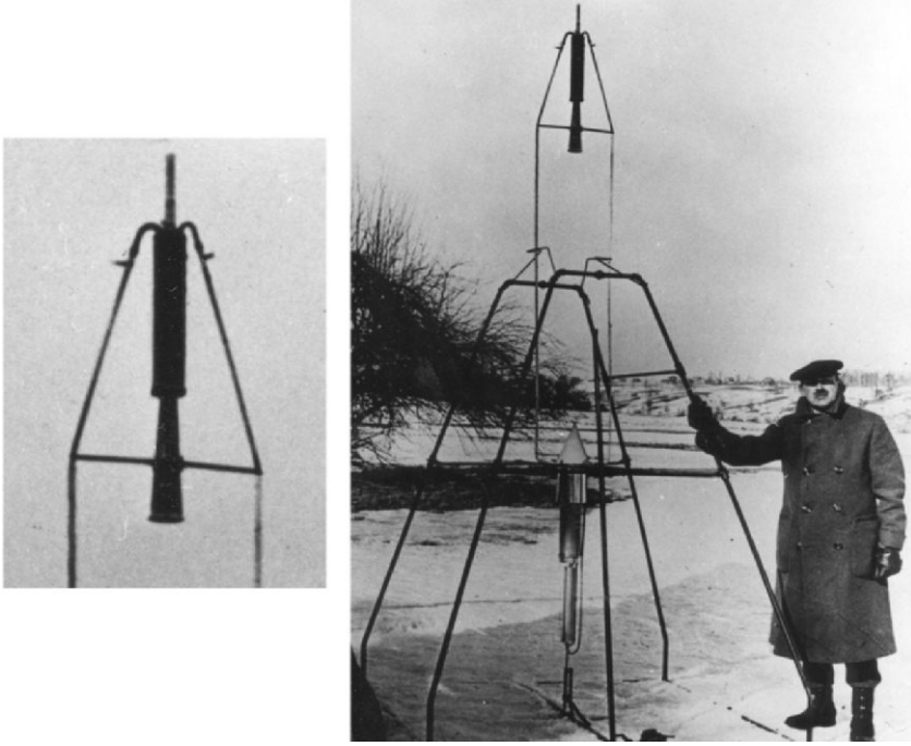
Fig. 4.6. Robert H. Goddard with his liquid-bipropellant rocket in its launch support frame. Detail (left) shows the combustion chamber and exhaust nozzle. For stability, the propellant tanks were mounted below the nozzle and capped with a cone for protection from the overhead exhaust plume. Adapted from image courtesy NASA.
