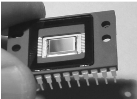
Fig. 6.2. The Kodak KAF-0402ME CCD image detector has 393,216 accessible pixels each 9\text{ }\mu\text{m} in size, arranged 768 horizontally by 512 vertically, visible here in the innermost rectangle. This rectangle would be situated at the focus of the imaging instrument, with the top of the silicon surface precisely in the instrument's focal plane. The twenty-four connector pins are for powering its internal electronics, providing clock and reset signals, and reading out the value of electric charge on each pixel. This particular model has been popular in amateur astronomy imaging work.
