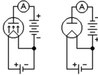
Fig. 1.7. Thermionic emission, known as “the Edison effect” and “cathode rays” prior to discovery of the electron in 1897 by British physicist J. J. Thomson (1856–1940), is seen as a current (arrows on left) flowing through a vacuum from a heated cathode to an anode, or “plate,” but only when the plate is given a more positive potential than the cathode. Note the absence of current when polarity of the large battery is reversed in the diagram on the right.
