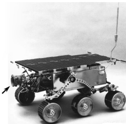
Fig. B.9. The APXS on the back end of Sojourner . Image ID JPL-25888BC courtesy NASA/JPL-Caltech.
