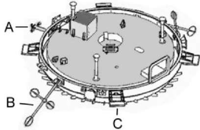
Fig. B.8. Huygens Probe with HASI sensors deployed. Inner cover (in place during flight operation) removed for clarity. “A” points out the pressure sensor inlet stub with two temperature sensors (microphone situated at its base), “B” shows one of 2 booms with electrical permittivity and wave sensors, “C” indicates one of four radar altimeter antennas, and the accelerometers are in the small housing near the spacecraft center. Data processing unit is upper left of center. Image courtesy ESA.
