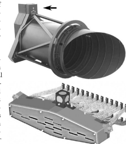
Fig. B.2. MRO HiRISE. Cassegrain telescope, with additional beam-folding optics in back, shown above enlargement of focal-plane assembly with fourteen linear CCDs (housed in back, see arrow). Courtesy NASA/JPL-Caltech.
