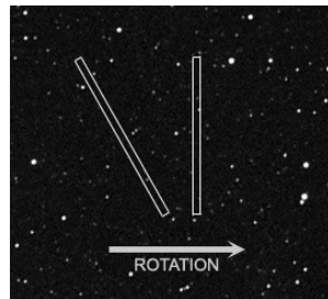
Fig. 3.10. Artist's conception of a V-slit star scanner's view against a field of stars. Spacecraft rotation first passes a star through the vertical "clock" slit as the slits move to the right. The star's subsequent passage through the slanted "cone" slit, based on a-priori knowledge of star-field geometry, provides enough information to determine spacecraft attitude in three axes.
