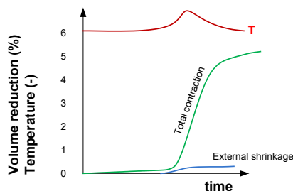
Figure 8-10: Typical contraction and external shrinkage.
