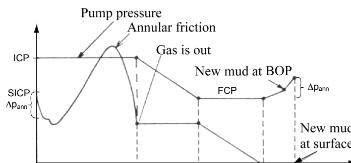
Figure 5-4: Fracturing during killing due to large choke line friction is avoided by means of the modified killing method; hide \Delta p_{\text{ann}} in SICP. The hidden \Delta p_{\text{ann}} must be gained back at the end of the circulation.
