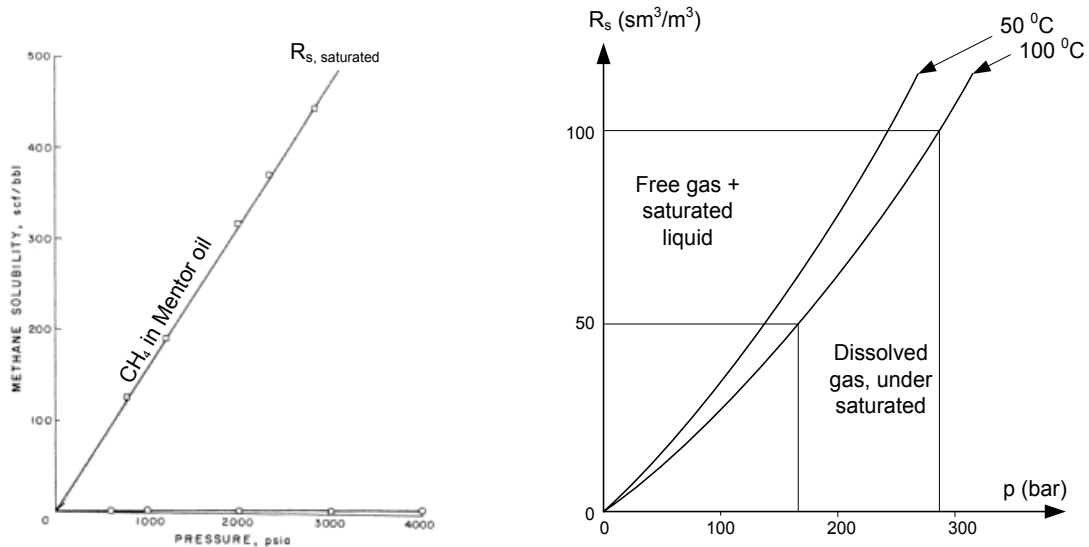
Figure 6-14: R_s for \text{CH}_4 in Mentor oil vs. well pressure. In figure to the right data points above the saturation curve indicate free gas in fully saturated base oil.
