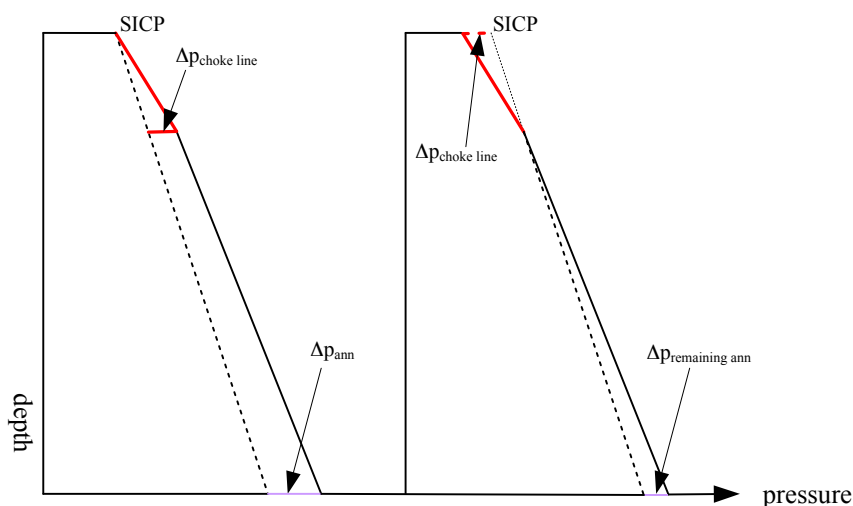
Figure 5-5: Modified offshore kill procedure, where choke line friction increases bottom pressures but where most of it is hidden in \Delta p_{\text{ann}} .
