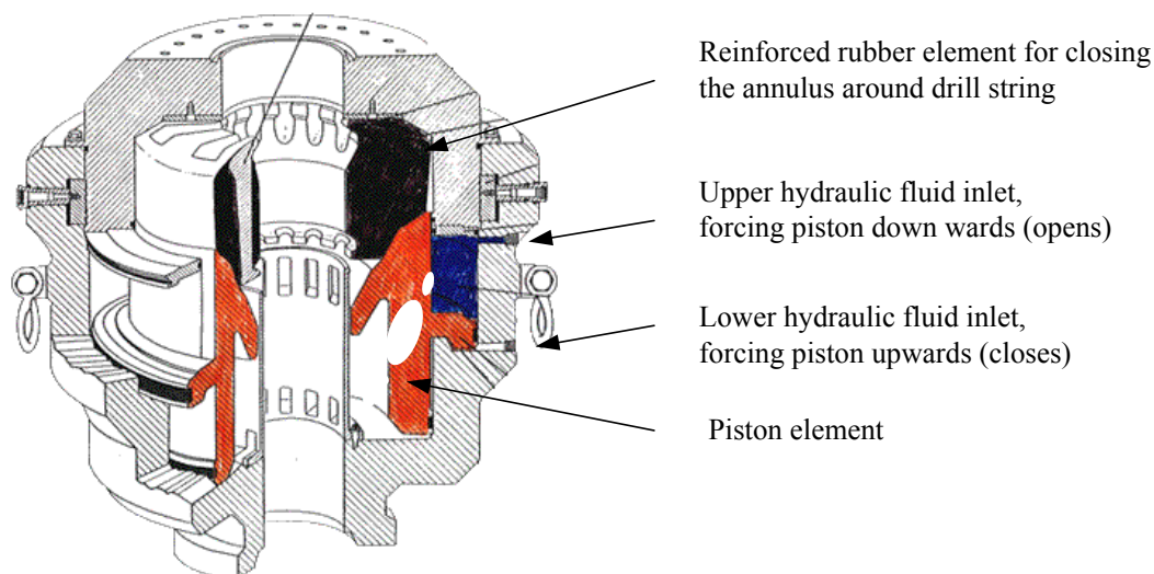
Figure 3-4: Spherical preventer.
