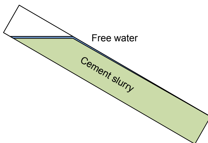
Figure 8-12: Schematic diagram showing fully developed water channeling.
