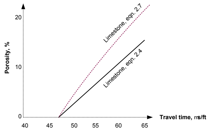
Figure 2-3: Porosity vs transit travel time in porous limestone (free after service companies).
