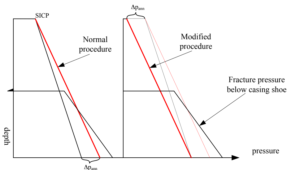
Figure 5-3: Modified slim hole killing procedure; hide \Delta p_{\text{ann}} in SICP.
