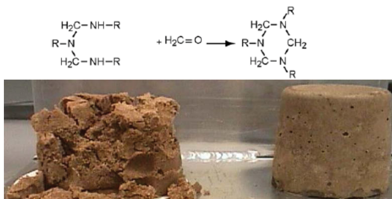
Figure 5-9: The soft sand is strengthened to become a hard sand stone. Complexion of melamine with formaldehyde. A strong 3-dimentional polymer network is formed. The resin can bond directly with the core itself thorough formation hydroxyl (-OH) groups (van Oort et al., 2011).
