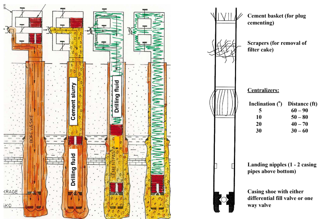
8-4: Primary cementing technique, including surface cement head and typical casing equipment when running in hole.
