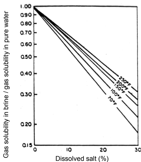
Figure 6-10: Correction of gas solubility for salt content (Petrucchi (1989)).
