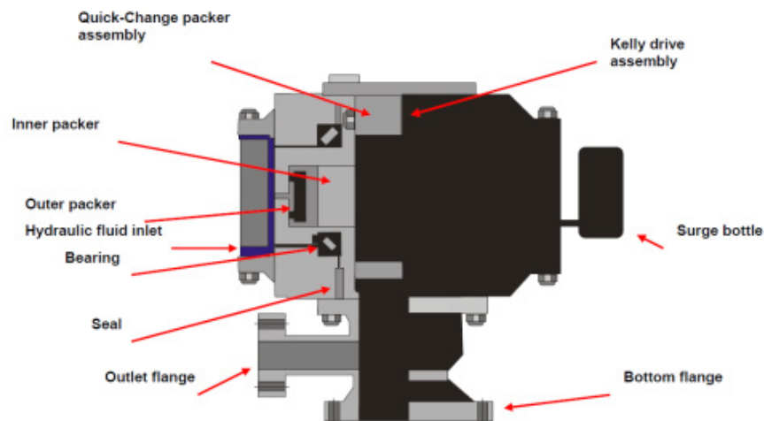
Figure 4-17: RBOP (Rehm et al., 2007).
