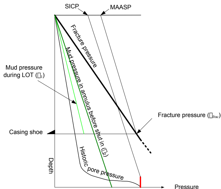
Figure 4-5: MAASP.
