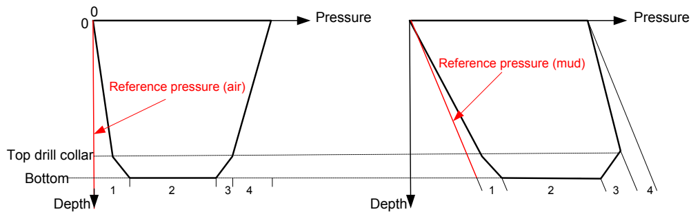
Figure 4-9: Well pressure during circulation through the well in a U-tube view, without gyrostatic pressure (left) and with (right). Numbered friction losses are: 1 – annulus, 2 – bit nozzles, 3 – inside drill collars, 4 – inside drill pipes.
