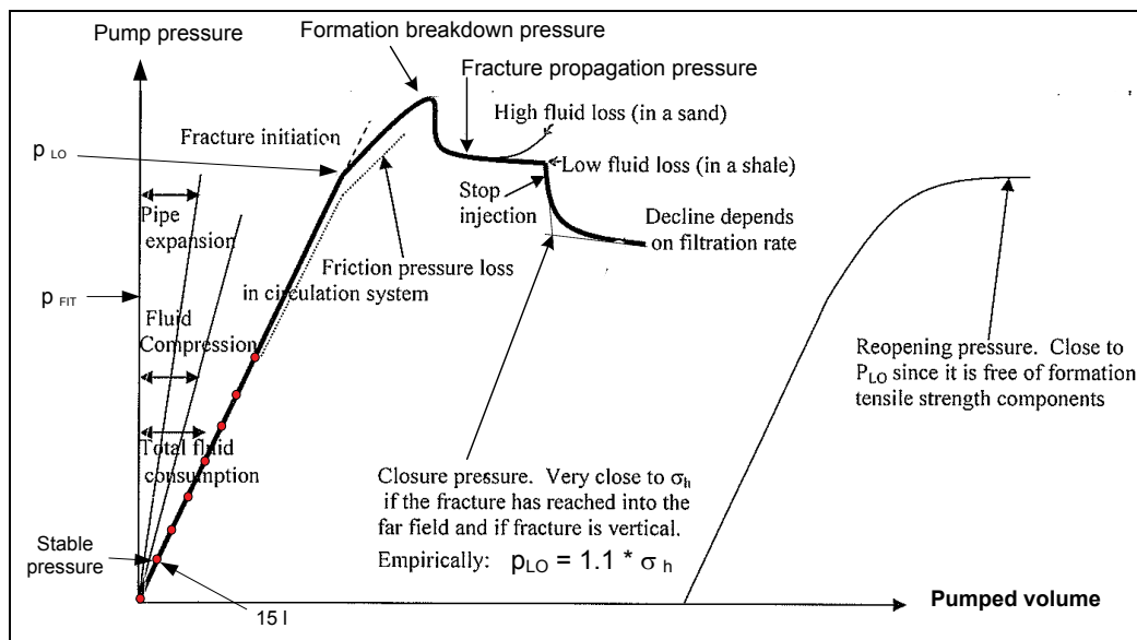
Figure 2-22: A full leak-off test. The linear pressure increase reflects the elastic properties of the fluid and the casing. The first sudden pressure drop reflects the breaking down of the formation. Data point sampling interval varies normally from 1 to maximum 5 seconds.
