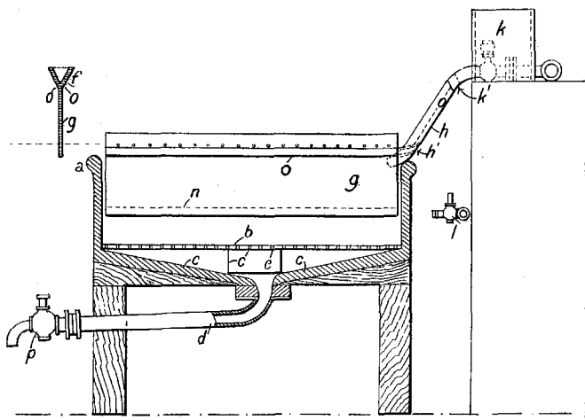
FIG. 20.—SECTIONAL ELEVATION OF THOMSON'S APPARATUS. a , Tank; b , False Bottom; c , Bottom; c' , Ribs; d , Draining Outlet; e , Grid; f , Troughs, with Aprons g ; h , Pipe, with Branches h' , leading to Troughs f ; k , Outlet Pipe of the Sulphuric Acid Tank k ; l , Water Supply Pipe; m , Pipe to supply of Nitrating Acids; o , Perforations of Trough f ; p , Cock to remove Acid.
