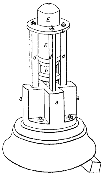
FIG. 55.—PRESSURE GAUGE.
