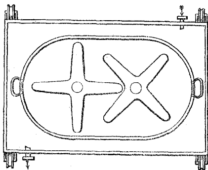
FIG. 32.—PLAN OF THE BOX CONTAINING THE EXPLOSIVE, IN M r ROBERTS' MACHINE.
