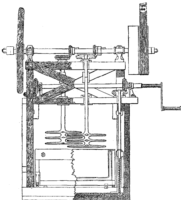
FIG. 31.—MR M'ROBERTS' MIXER FOR GELATINE EXPLOSIVES.
