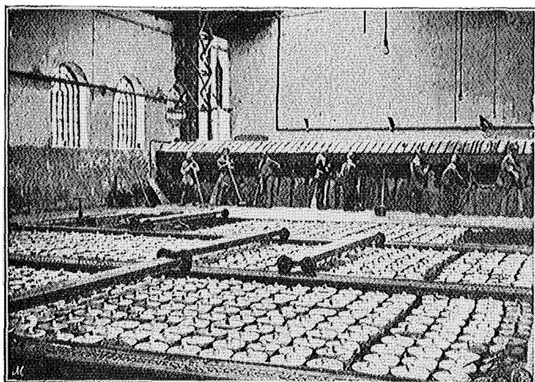
FIG. 12.—THE COOLING PITS.
