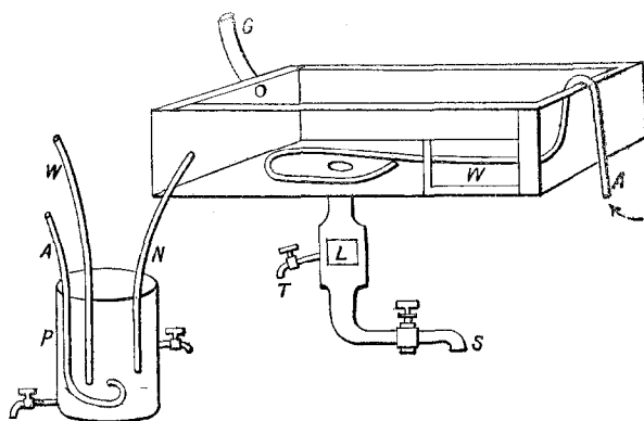
FIG. 8.—SEPARATOR. A , Compressed Air Pipes; G , Nitro-glycerine enters from Nitrator; N , Nitro-glycerine to P ; L , Lantern Window; W , Window in Side; S , Waste Acids to Secondary Separator; T , Tap to remove last traces of Nitro-glycerine; P , Lead Washing Tank; A , Compressed Air; W , Water Pipe; N , Nitro-glycerine from Separator.
