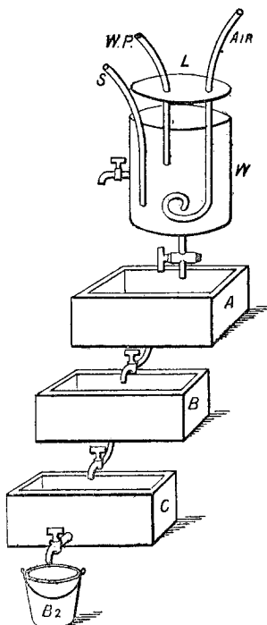
FIG. 9.—FILTERING AND WASHING PLANT. W , Lead Washing Tank; W.P. , Water Pipe; L , Lid; S , Nitro-glycerine from Separator; A, B, C , Filtering Tanks; B2 , Indiarubber Bucket.
