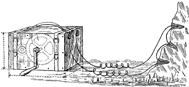
FIG. 36.—ELECTRIC EXPLODER.
