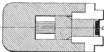
FIG. 60.—CRUSHER GAUGE. E , GAS CHECK.
