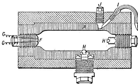
FIG. 59.—NOBLE'S PRESSURE GAUGE.
