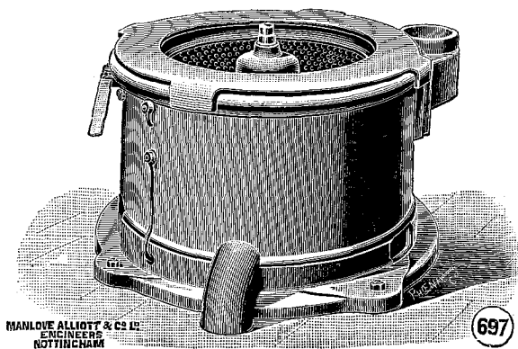
FIG. 14.—HYDRO-EXTRACTOR.
