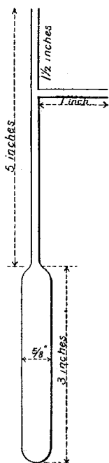
FIG. 49.—PAGE'S REGULATOR.
