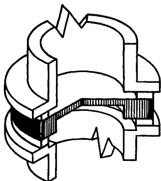
Figure 6-25. Monoblock-Type Rupture Disc Made of Brittle Graphite, Armored by a Steel Ring Bonded to the Disc Circumference. (Courtesy of Continental Disc Corporation.)
