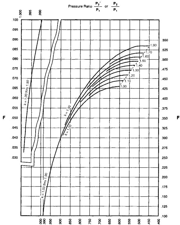
Figure 7-2. Flow Correction Factor F. (Courtesy of Anderson, Greenwood & Co., Source Catalog 90/9000-US.96.)
