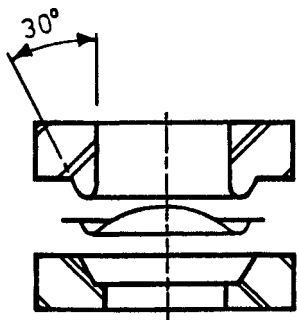
Figure 6-29. Exploded View of Rupture Disc Holder for Solid-Metal Forward-Domed Rupture Discs. (Courtesy of Continental Disc Corporation.)
