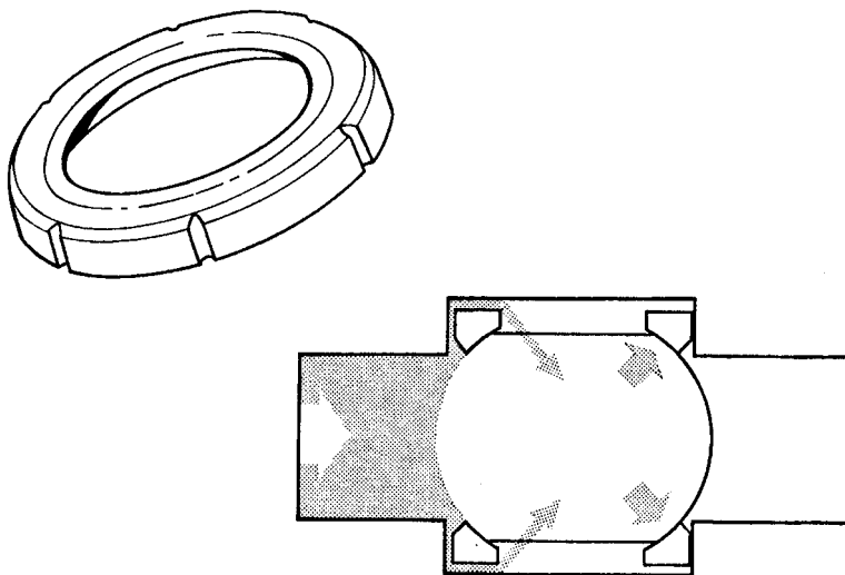
Figure 3-60. Schematic View of Ball Valve with Floating Ball and Torsion Seats, Showing Function of Pressure-Equalizing Slots in Periphery of Seats. (Courtesy of Worchester Valve Co., Ltd.)
