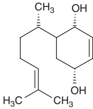
2,5-Dihydroxybisabola-3, 10-diene
