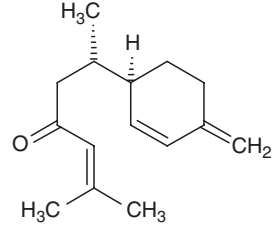
\alpha -Turmerone
