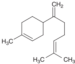
2,5-Dihydroxybisabola-3, 10-diene
