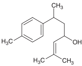
\alpha -Turmerol
