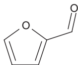
Furfural
