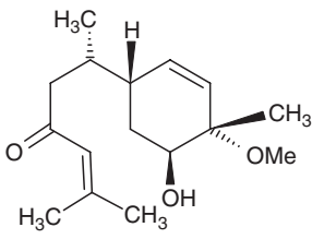
4-Methoxy-5-hydroxybisabola-2, 10-diene-9-one
