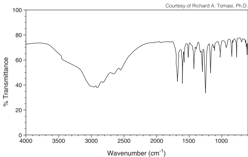
Spectrum B
