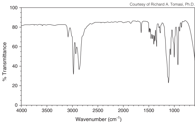
Spectrum B
