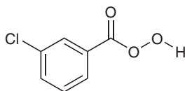
MCPBA
