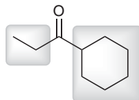
unsymmetrical
