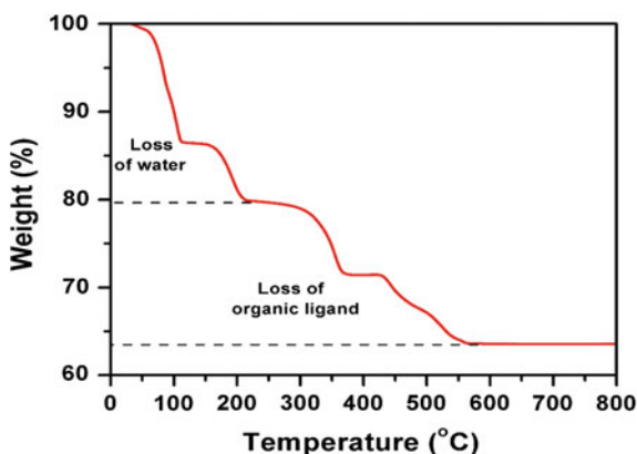
Fig. 5.2 TGA [ \text{Li}_2(\text{VO})_2(\text{HPO}_4)_2(\text{C}_2\text{O}_4) ] \cdot 6 \text{H}_2\text{O} in \text{N}_2 atmosphere at a heating rate of 5 °C min -1
