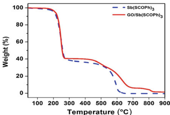
Fig. 7.1 TGA of Sb(SCOPh) 3 and rGO/Sb(SCOPh) 3 in nitrogen atmosphere at a heating rate of 10 °C min -1
