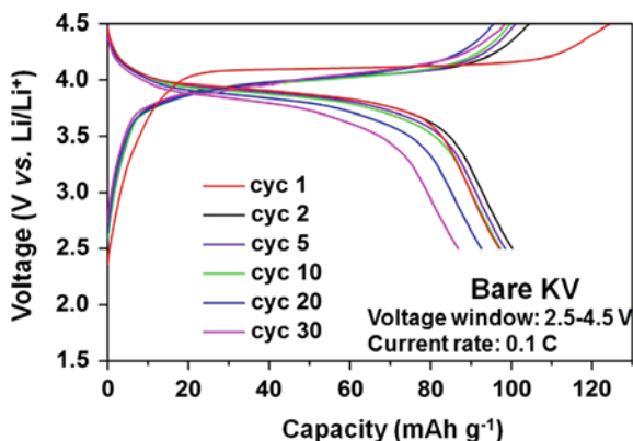
Fig. 4.10 Galvanostatic cycling studies of [K_2(VO)_2(HPO_4)_2(C_2O_4)] in the voltage range, 2.5–4.5 V at a current density of 11 \text{ mA g}^{-1} (0.1 C), showing voltage versus capacity profiles for few selected cycles
