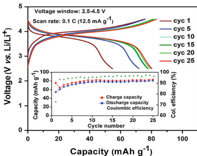
Fig. 3.8 Galvanostatic cycling studies (charge-discharge profiles) of [\text{Li}_2(\text{VO})_2(\text{HPO}_4)_2(\text{C}_2\text{O}_4)] at a current density of 12.5 \text{ mA g}^{-1} (0.1 C), showing voltage versus capacity plots for few selected cycles. The inset figure shows the variation of specific capacity and coulombic efficiency with cycle number
