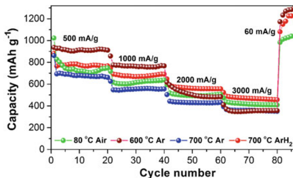
Fig. 8.9 Rate capability of rGO/Fe 3 O 4 synthesized at different conditions
