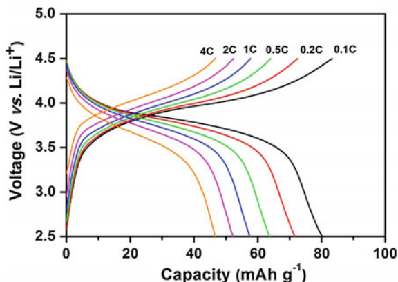
Fig. 3.9 Galvanostatic charge-discharge profiles of [\text{Li}_2(\text{VO})_2(\text{HPO}_4)_2(\text{C}_2\text{O}_4)] at different current rates (1 C represents a current density of 125 \text{ mA g}^{-1} )
