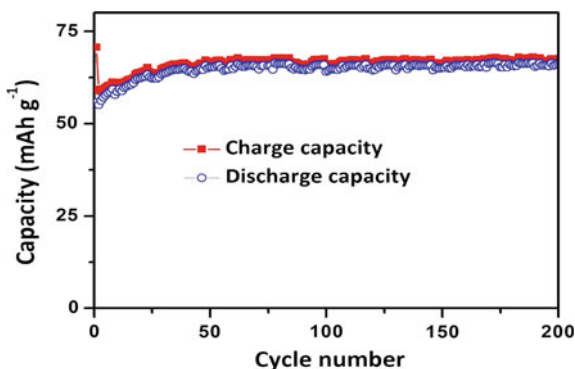
Fig. 6.13 Long term cycling of \alpha_1\text{-LiVOPO}_4 at a current rate of 0.5 C in the potential window of 2.5–4.5 V
