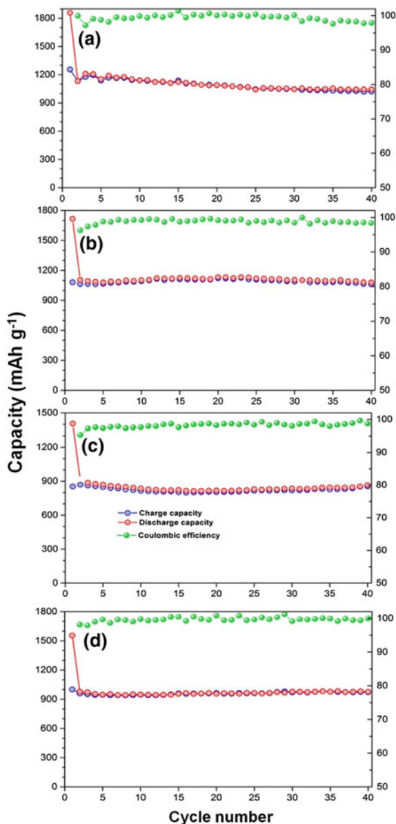
Fig. 8.8 Capacity versus cycle number plots of rGO/Fe 3 O 4 synthesized at: a 80 °C in air; b 600 °C in Ar; c 700 °C in Ar and d 700 °C in Ar-H 2
