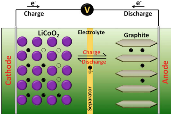
Fig. 1.2 Principle of operation of Lithium ion batteries. Full black circles and hollow circles represent the \text{Li}^+ ions and vacant Li sites respectively
