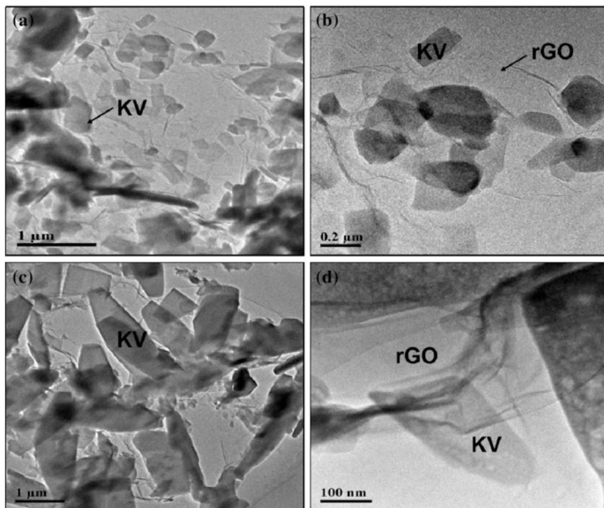
Fig. 4.8 TEM images of \text{rGO}/[\text{K}_2(\text{VO})_2(\text{HPO}_4)_2(\text{C}_2\text{O}_4)] \cdot 4.5\text{H}_2\text{O} containing 4 % rGO prepared in 12 h (a and b), prepared in 48 h (c and d)
