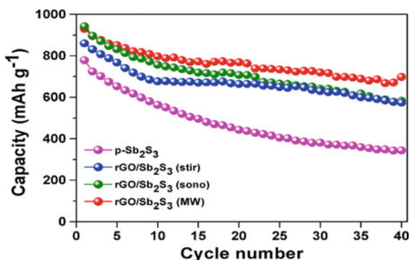
Fig. 7.7 Capacity (charge) versus cycle number plots of p-Sb 2 S 3 and rGO/Sb 2 S 3
