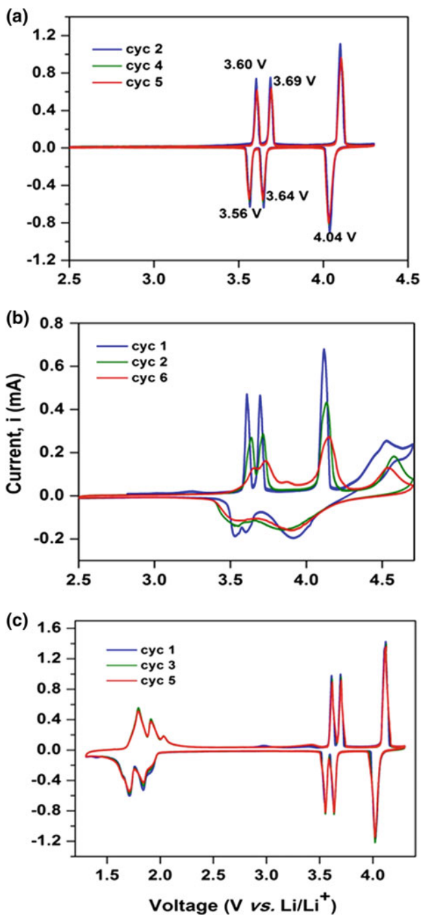
Fig. 5.11 Cyclic voltammograms (CV) of c-LVPV in the voltage window of a 2.5–4.3 V, b 2.5–4.7 V and c 1.3–4.3 V at a scan rate of 0.058 \text{ mV s}^{-1}
