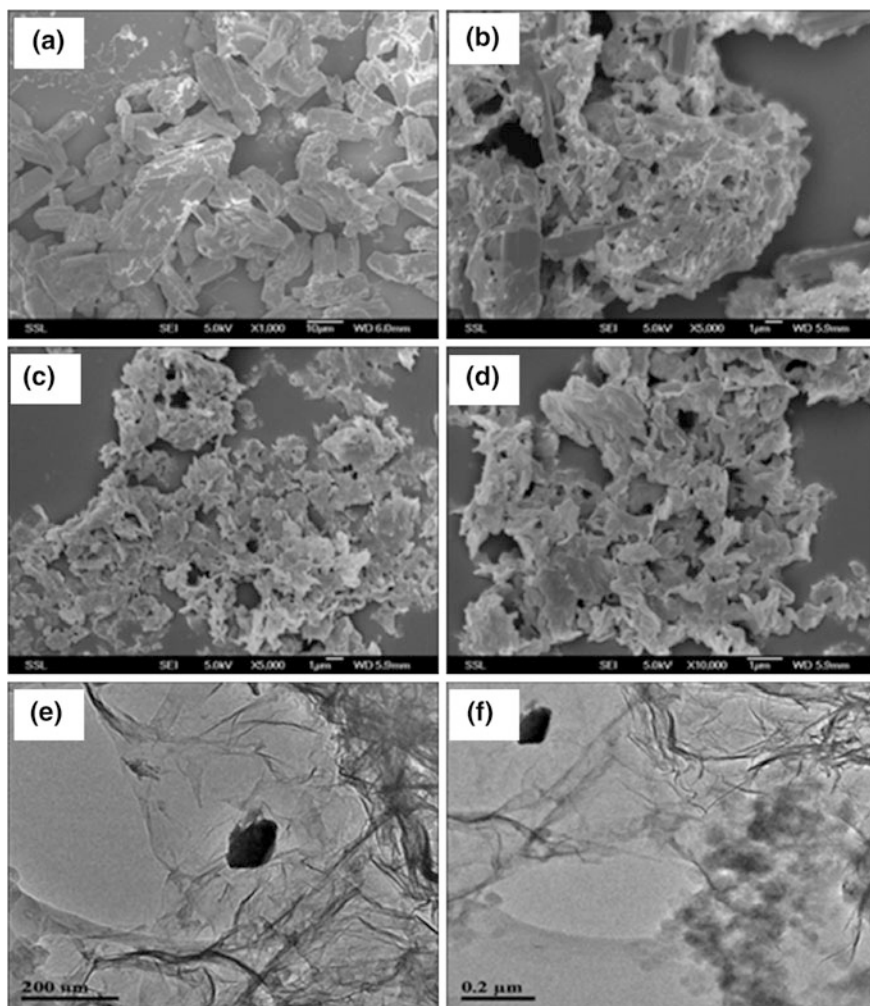
Fig. 7.4 SEM micrographs of a p-Sb 2 S 3 ; b rGO/Sb 2 S 3 (stir); c rGO/Sb 2 S 3 (sono); d rGO/Sb 2 S 3 (MW) and e and f TEM images of rGO/Sb 2 S 3 (MW)
