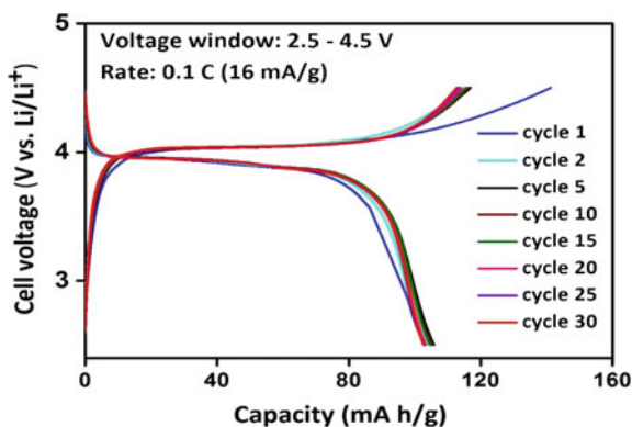
Fig. 6.10 Galvanostatic charge-discharge cycling of \alpha_1 -LiVOPO 4 at a current rate of 0.1 C in the potential window of 2.5–4.5 V
