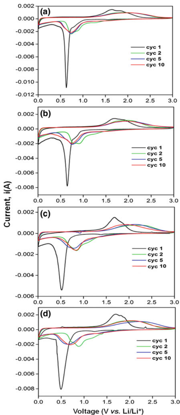
Fig. 8.11 Cyclic voltammograms (CV) of \text{rGO}/\text{Fe}_3\text{O}_4 synthesized at: a 80 °C in air; b 600 °C in Ar; c 700 °C in Ar and d 700 °C in \text{Ar-H}_2
