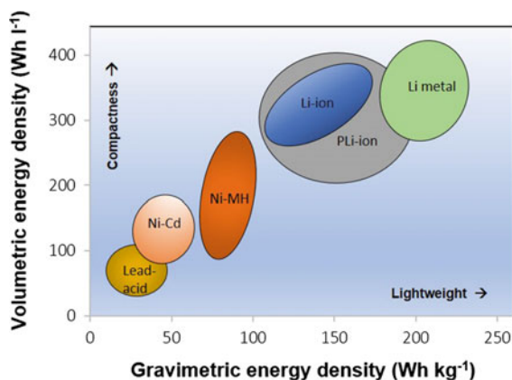
Fig. 1.1 Comparison of gravimetric and volumetric energy densities of various secondary batteries
