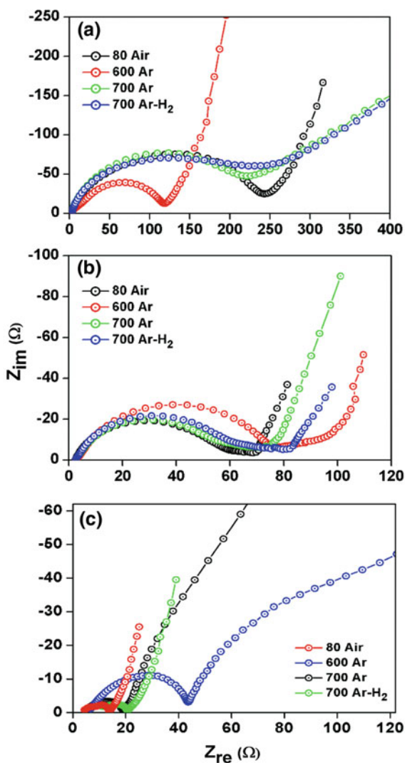
Fig. 8.12 Nyquist plots of the different rGO/Fe 3 O 4 composites at: a OCV; b fully discharged state (1st cycle) and c fully discharged state (40th cycle)
