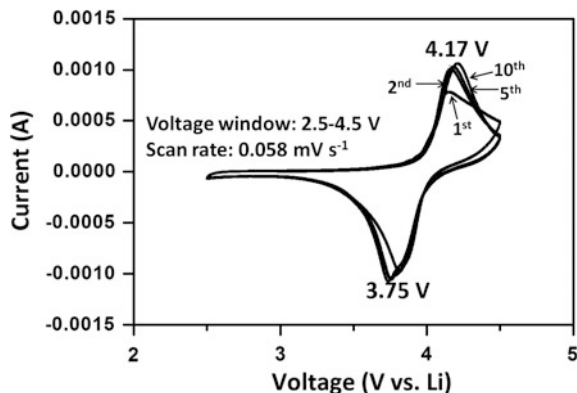
Fig. 6.14 Cyclic voltammograms of \alpha_1 -LiVOPO 4 at a scan rate of 0.058 mV s -1 in the potential window of 2.5–4.5 V
