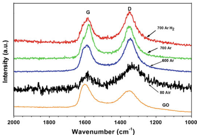
Fig. 8.3 Raman spectra rGO/Fe 3 O 4 synthesized at different conditions
