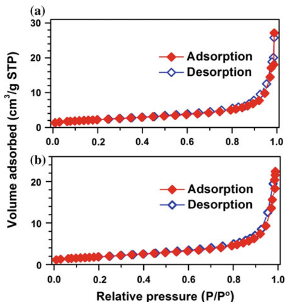
Fig. 4.9 N_2 adsorption-desorption isotherms of rGO composites of [K_2(VO)_2(HPO_4)_2(C_2O_4)] containing a 8 % rGO and b 4 % rGO
