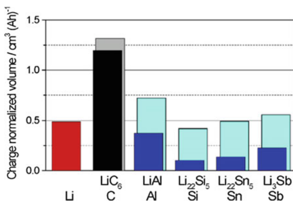
Fig. 1.10 Volume changes encountered in anode materials during lithiation. Reproduced from Ref. [140] with permission of Elsevier
