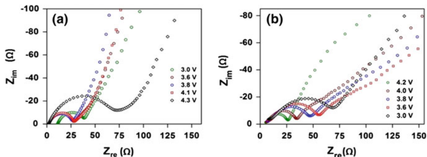
Fig. 5.12 Nyquist plots of c-LVPV at various voltages during a 1st charge and b 1st discharge cycle
