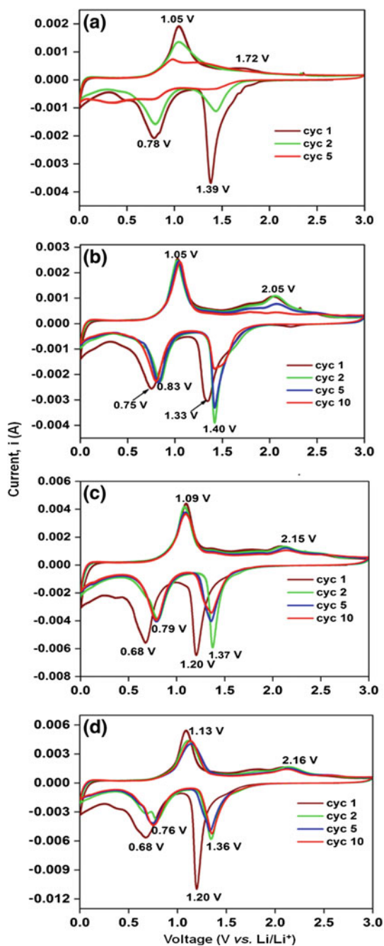
Fig. 7.8 Cyclic voltammograms (CV) of a pristine \text{Sb}_2\text{S}_3 ; b \text{rGO}/\text{Sb}_2\text{S}_3 (stir); c \text{rGO}/\text{Sb}_2\text{S}_3 (sono); and d \text{rGO}/\text{Sb}_2\text{S}_3 (MW)
