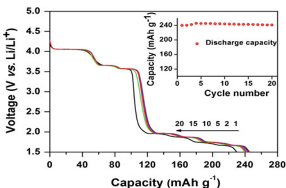
Fig. 5.10 Galvanostatic cycling of c-LVPV in the voltage window of 1.5 – 4.3 V at a current density of 50 \text{ mA g}^{-1} (For clarity, only the discharge cycles are shown). The inset graph shows the plot of discharge capacity versus cycle number
