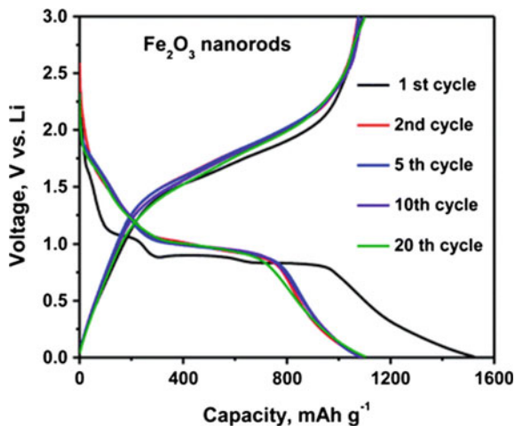
Fig. 1.11 Galvanostatic charge-discharge profiles of electrospun \text{Fe}_2\text{O}_3 nanorods. Reproduced from Ref. [156] with permission of the Royal Society of Chemistry
