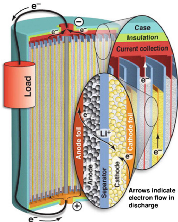
Fig. 1.3 Schematic of a cylindrical LIB assembly containing large number of electrochemical cells. Reproduced from Ref. [4] with permission of Elsevier
