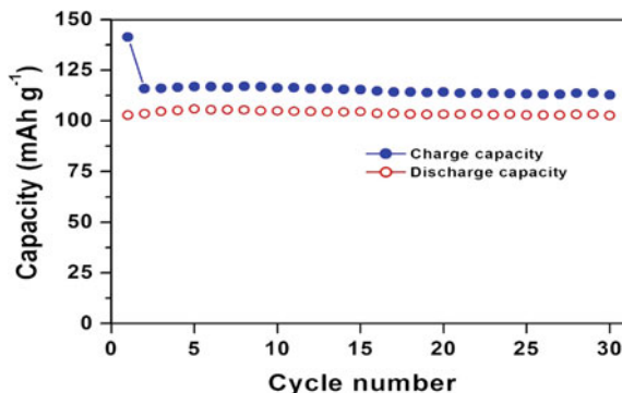
Fig. 6.11 Plot of capacity versus cycle number of \alpha - \text{LiVOPO}_4 at a current rate of 0.1 C in the potential window of 2.5–4.5 V
