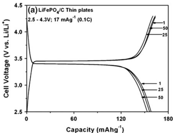
Fig. 1.8 Discharge-charge curves of \text{LiFePO}_4 nanoplates in the voltage range; 2.5–4.3 V. Reproduced from Ref. [57] with permission of the Royal Society of Chemistry
