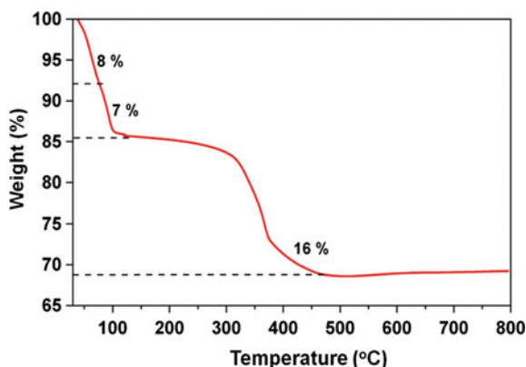
Fig. 4.5 TGA of [\text{K}_2(\text{VO})_2(\text{HPO}_4)_2(\text{C}_2\text{O}_4)] \cdot 4.5\text{H}_2\text{O} in \text{N}_2 flow at a heating rate of 5 °C \text{min}^{-1}
