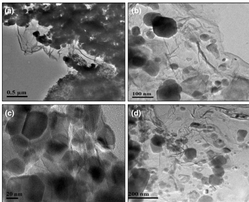
Fig. 8.5 Transmission electron micrographs of rGO/ \text{Fe}_3\text{O}_4 nanocomposites annealed at different conditions: a 80 °C in air; b and c 600 °C in Ar; d 700 °C in Ar- \text{H}_2
