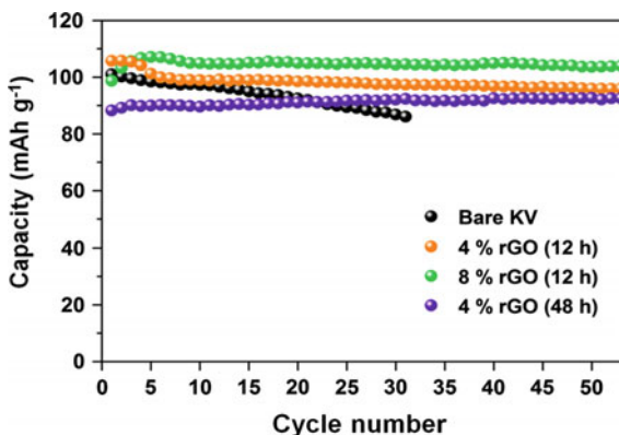
Fig. 4.12 Capacity (discharge) versus cycle number plots of bare [\text{K}_2(\text{VO})_2(\text{HPO}_4)_2(\text{C}_2\text{O}_4)] and different rGO/ [\text{K}_2(\text{VO})_2(\text{HPO}_4)_2(\text{C}_2\text{O}_4)] composites
