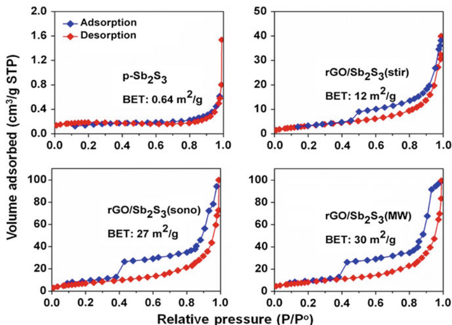
Fig. 7.5 Nitrogen adsorption-desorption isotherms of p-Sb 2 S 3 and rGO/Sb 2 S 3 composites
