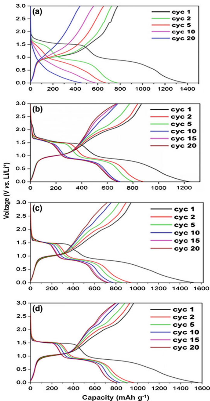
Fig. 7.6 Galvanostatic cycling of a p-Sb 2 S 3 ; b rGO/Sb 2 S 3 (stir); c rGO/Sb 2 S 3 (sono); and d rGO/Sb 2 S 3 (MW)
