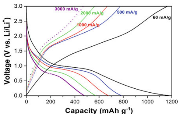
Fig. 8.10 Charge-discharge profiles at different current rates for rGO/Fe 3 O 4 obtained at 700 °C in Ar–H 2
