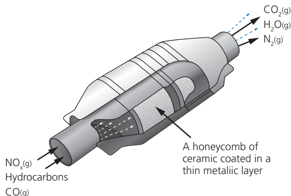
Figure 12.16 Catalytic converter.
