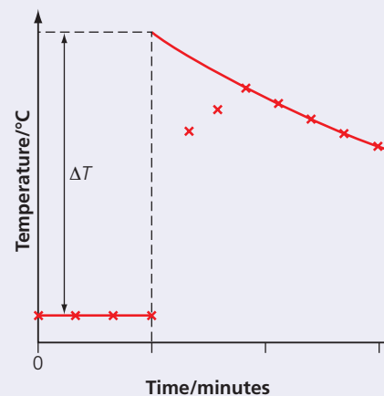
Figure 4.12 Estimating the maximum temperature of a neutralisation reaction.
