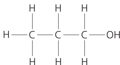
propan-1-ol
