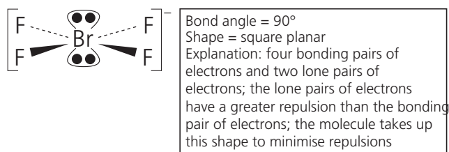
Figure 3.76 \text{BrF}_4^- ion.
