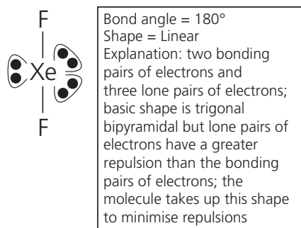
Figure 3.77 \text{XeF}_2 .
