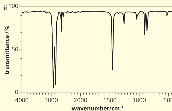
Spectrum 2
