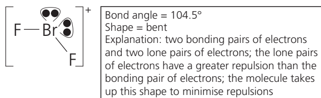
Figure 3.75 \text{BrF}_2^+ ion.
