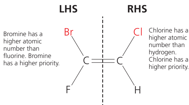
Z-1-bromo-2-chloro-1-fluoroethene
