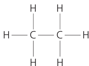
ethane
