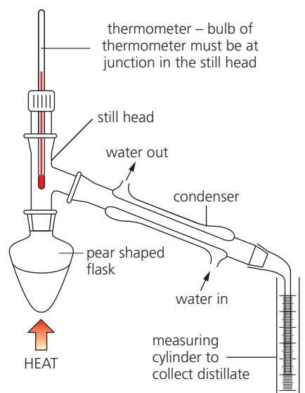
Figure 13.16 Distillation apparatus.
