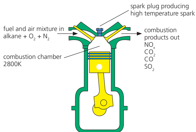
Figure 12.13 The internal combustion engine.
