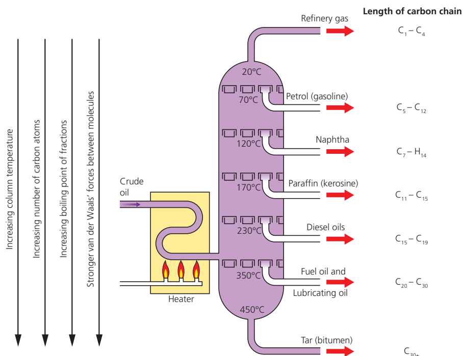
Figure 12.9 Fractional distillation of crude oil.
