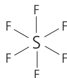
Bonding diagram
