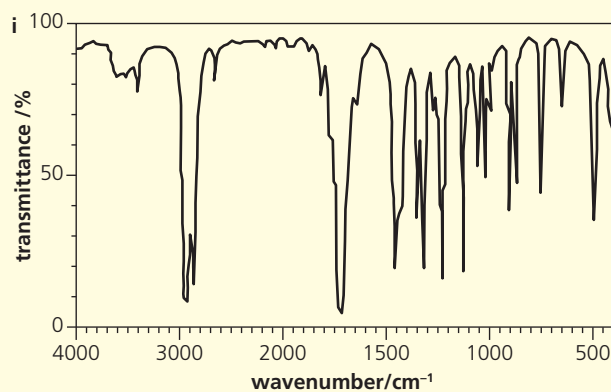
Spectrum 1
