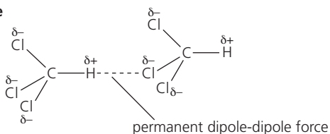
Trichloromethane
