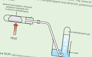
Figure 13.19 Laboratory preparation of methylpropene.
