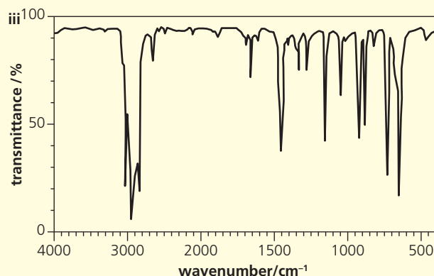
Spectrum 3
