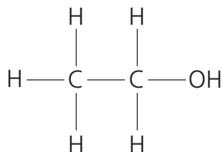
ethanol
