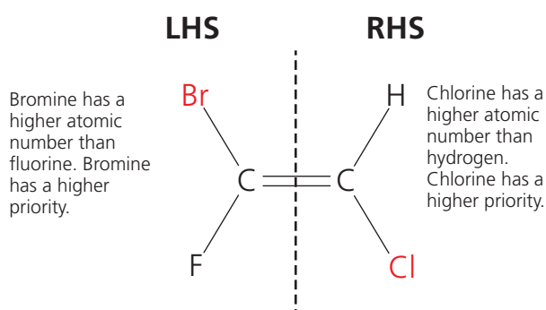
E-1-bromo-2-chloro-1-fluoroethene
