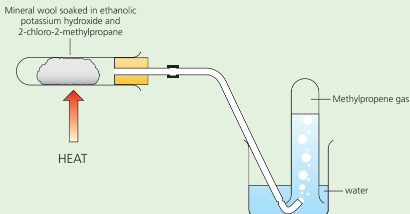
Figure 13.19 Laboratory preparation of methylpropene.
