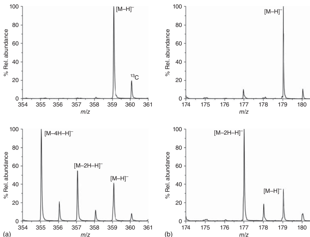
Figure 3.10 Effect of online DPPH• reaction experiments for selected components: (a) rosmarinic acid found in Rosmarinus officinalis extract and (b) caffeic acid found in Melissa officinalis . Reproduced from Maringer et al. [78] with permission of Wiley.
