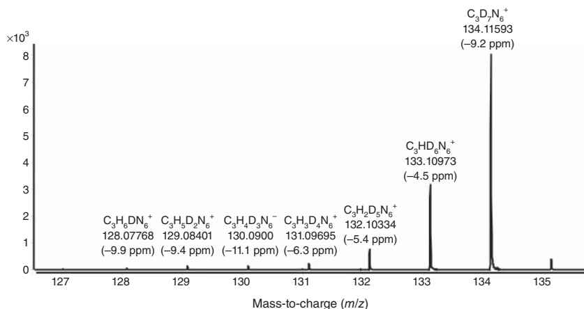
Figure 3.9 Mass spectrum for melamine from a CZE-ESI-Q-TOFMS run using a deuterium oxide/mono-deuterated MeOH (80:20), 0.1% formic acid sheath liquid.
