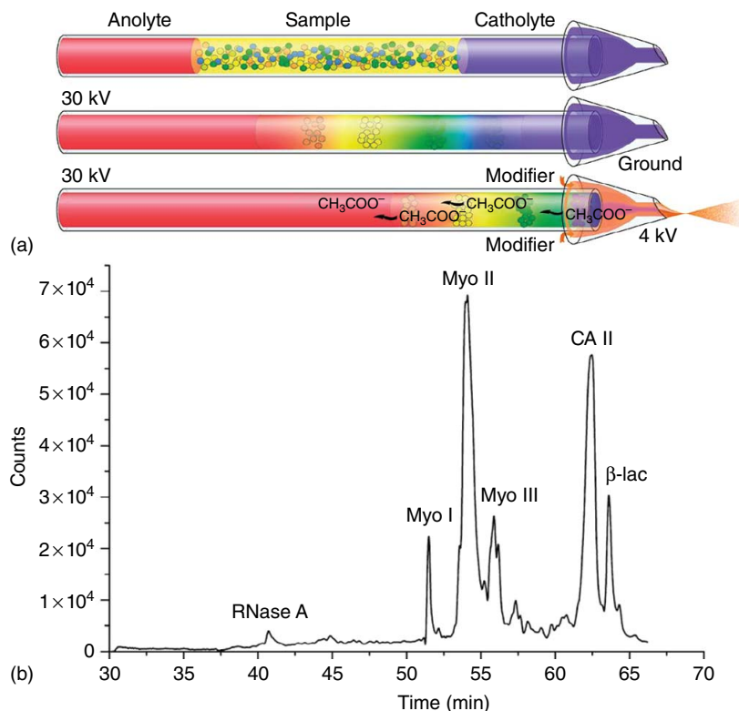
Figure 2.8 (a) Schematic diagram of automated cIEF-MS. The flow-through microvial provides the electrical contact and chemical environment for cIEF. The CE-MS interface improves the ionization efficiency of the mobilized effluent without significant
