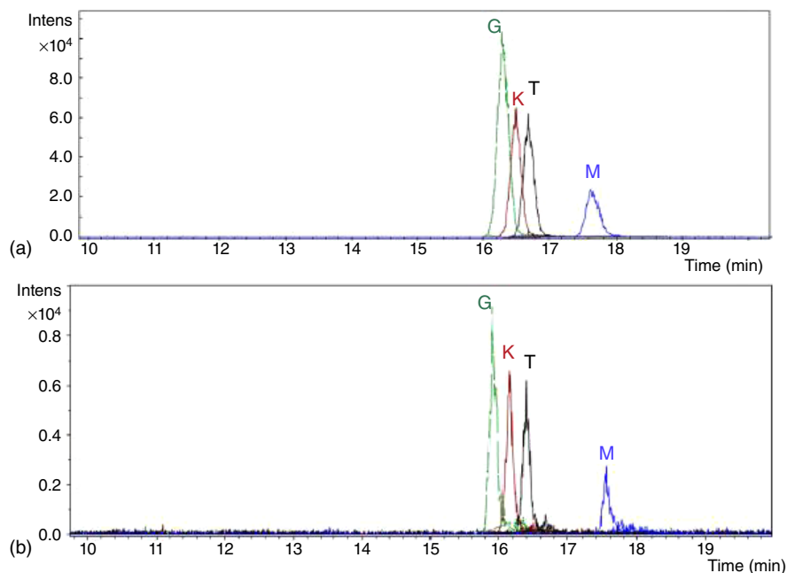
Figure 5.5 Overlaid extracted ion electropherograms of 50 mg kg -1 butyl 1-(pyridinyl-4-yl) piperidine 4-carboxylate derivative test mixture of potentially genotoxic alkyl halides (G, K, T, and M) using FESI at 10 kV for 150 s (a) of 500 mg kg -1 BPPC derivative test mix using typical hydrodynamic injection (b). Reproduced from van Wijk et al. [34] with permission of Elsevier.
