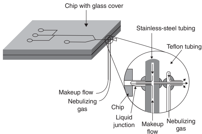
Figure 4.6 Glass chip-based CE/MS apparatus and the expanded view of the coupled microsprayer. Reproduced from Wachs and Henion [65] with permission of American Chemical Society.
