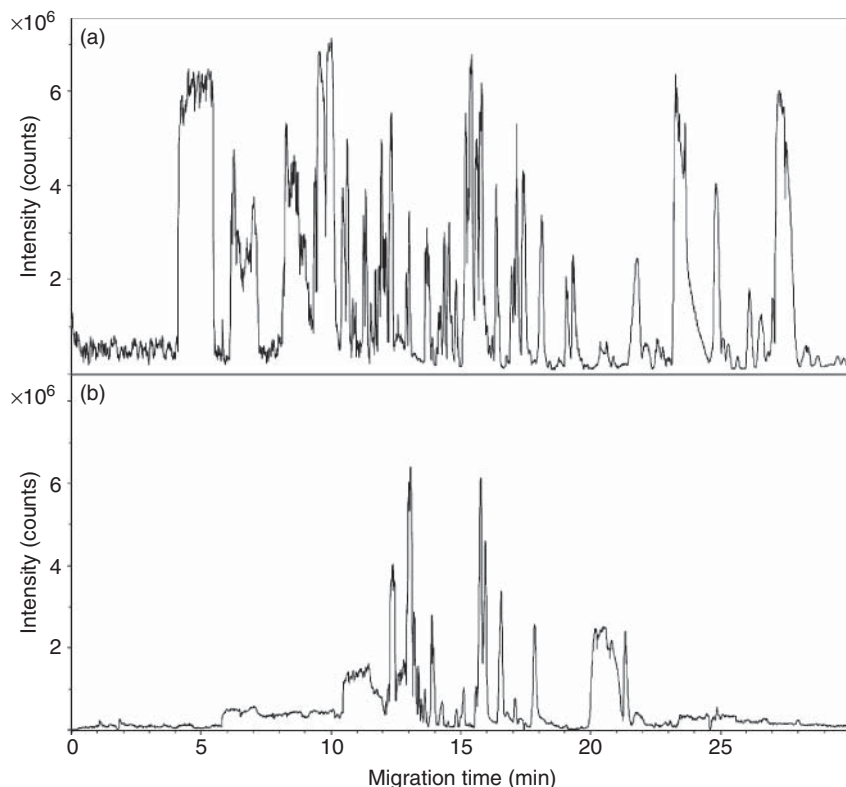
Figure 11.6 (a) Base peak electropherogram ( m/z 50–450) of human urine obtained with sheathless CE-MS using a porous tip sprayer. Conditions: BGE, 10% acetic acid (pH 2.2); sample injection, 2.0 psi for 30 s (1% of capillary volume). (b) Base peak electropherogram ( m/z 50–450) of human urine obtained with CE-MS using a sheath-liquid interface. Conditions: BGE, 10% acetic acid (pH 2.2); sample injection, 0.5 psi for 30 s (1% of capillary volume). (Reproduced from [76] with permission from American Chemical Society.)
