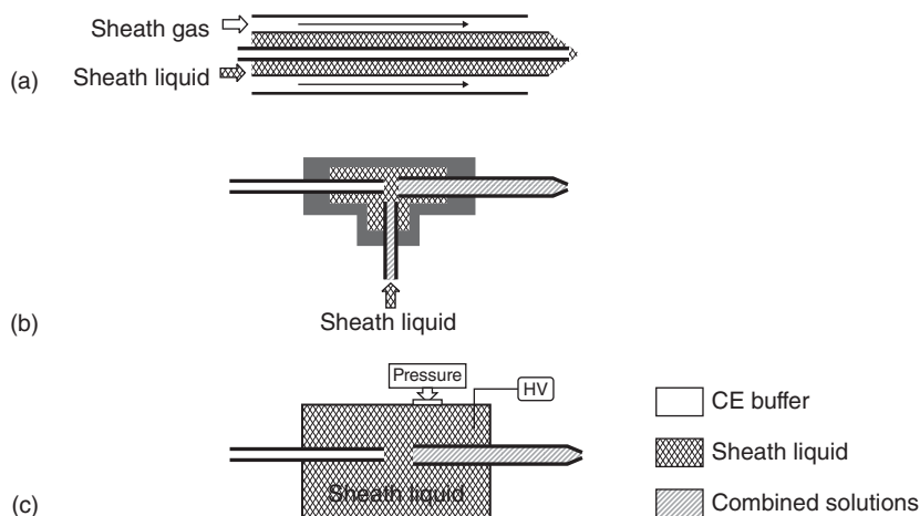
Figure 2.2 Common sheath-flow interface arrangements. (a) coaxial sheath-flow interface with sheath gas, (b) liquid junction interface, and (c) pressurized liquid junction interface. Reproduced from Maxwell and Chen [6] with permission of Elsevier.
