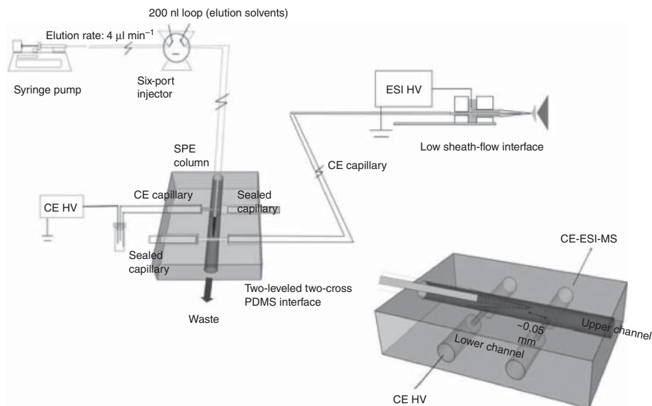
Figure 5.9 Schematic of on-line SPE CE-MS. Reproduced from Lee et al. [59] with permission of Wiley.
