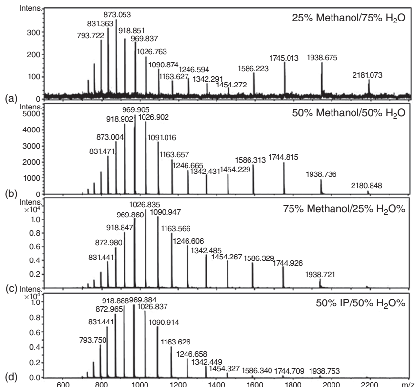
Figure 3.5 Effect of methanol and iso-propanol content in SL on charge state distribution of Bet v 1a. BGE: 10 mmol l^{-1} NH_4HCO_3 , pH 7.50; SL composition: 0.1% v/v
