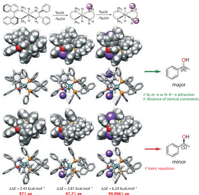
Figure 1.23 Transition states leading to R - and S -products: optimized 253 under DFT 218,219 /ωB97X-D 332 /SDD(Ru)/6-31G*(C, H,N, O,P, K)/SMD(propan-2-ol) 333 level of theory on the full model of trans -[RuH 2 ]{(S)-BINAP}[(S, S)-DPEN]} and its K-amidato complexes with acetophenone. The enantioselectivity for each complex is calculated based on difference in electronic energy using absolute rate theory. 184,185 Some H-atoms are omitted for the ball and stick model. (Reprinted with permission from Dub, P. A. et al., Dalton Trans. , 45, 6756–6781. Copyright 2016 Royal Society of Chemistry.)
