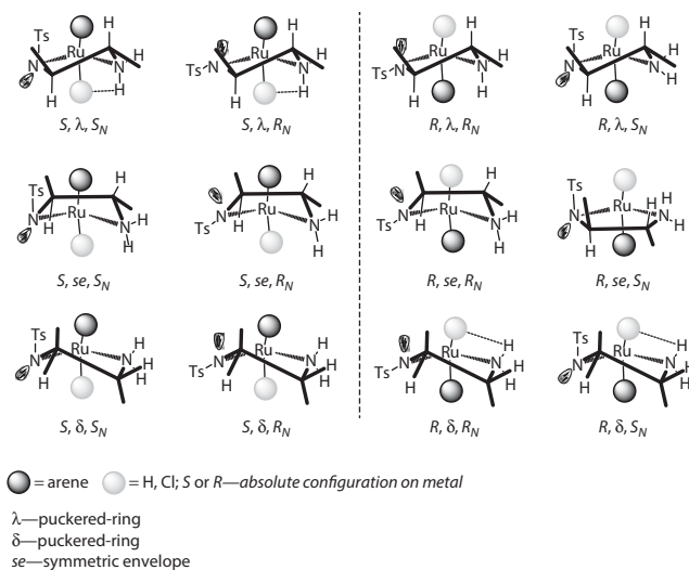
Chart 1.4 Isomers possible for the Noyori–Ikariya catalyst. (Adapted from Dub, P. A. et al., Dalton Trans. , 45, 6756–6781. Copyright 2016 Royal Society of Chemistry.)
