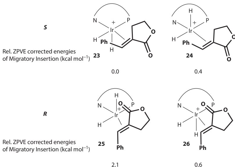
Scheme 1.52 Substrate coordination in four competing pathways in the asymmetric hydrogenation of exocyclic \alpha,\beta -unsaturated carbonyl compounds with an Ir/BiphPhox catalyst.
