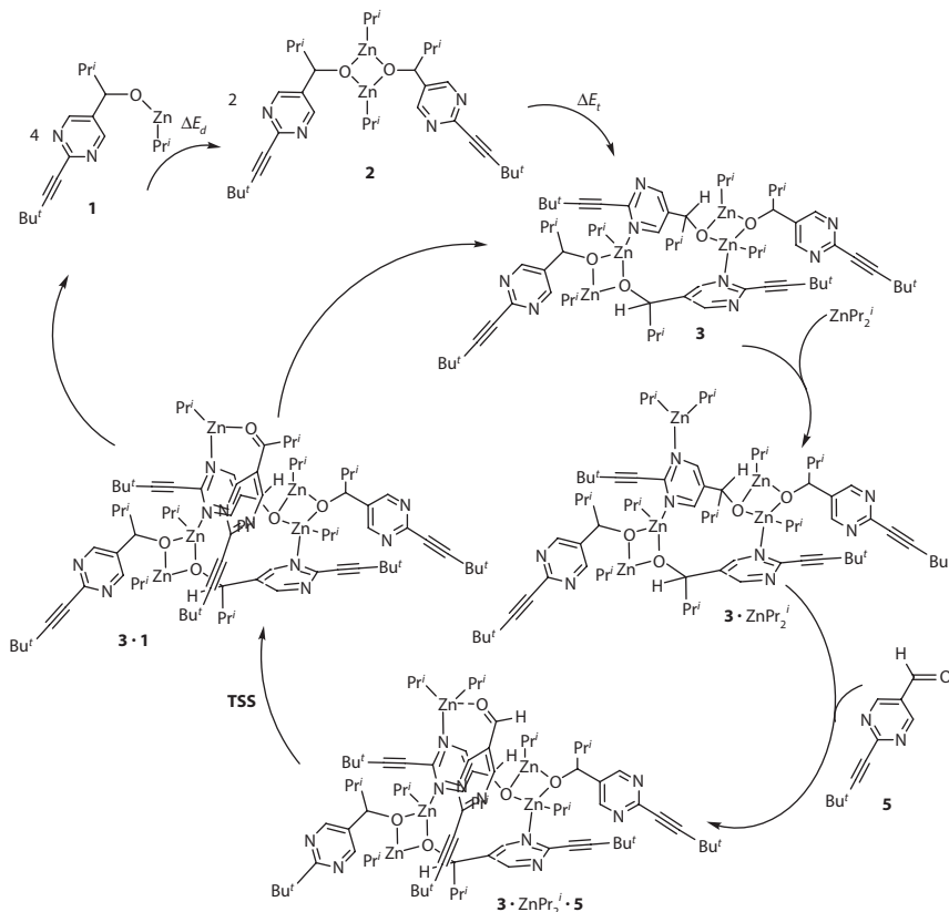
Scheme 2.20 Catalytic cycle of Soai Reaction involving tetrameric catalyst. (Reproduced with permission from Gridnev, I. D. et al., ACS Catal. , 2, 2137–2149, 2015.)
