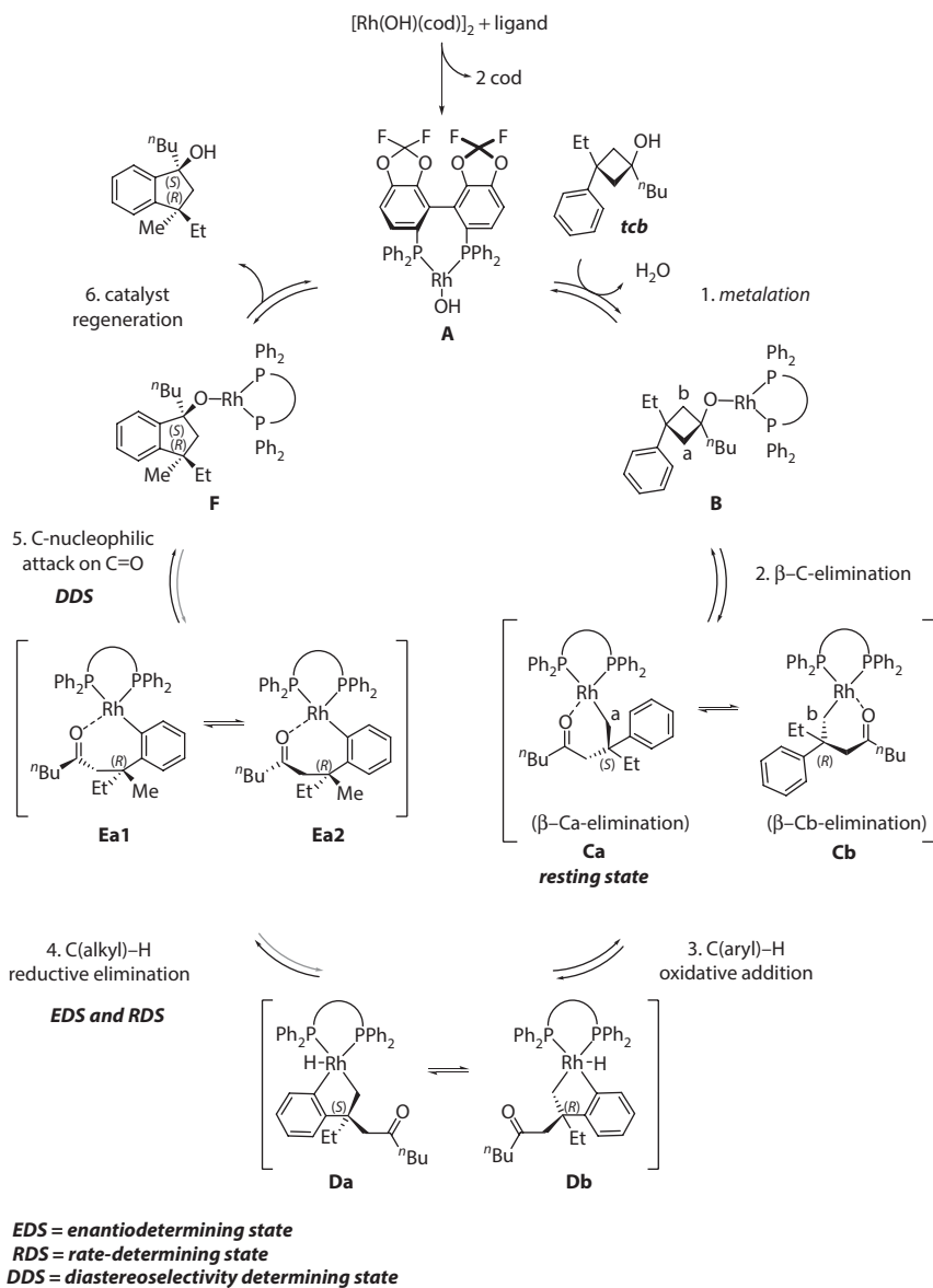
Figure 2.6 Computed catalytic cycle for Rh-Catalyzed Stereoselective Isomerization of tert -Cyclobutanol tcb under DFT/B3LYP/LANL2DZ(Rh)/6-31G*(all other) level of theory in the gas-phase. (Data from Yu, H. et al., Chem. Eur. J. , 20, 3839–3848, 2014.)
