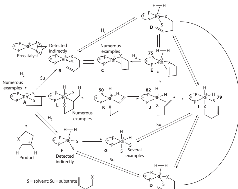
Scheme 1.29 Intermediates involved in the catalytic cycle of asymmetric hydrogenation. (Gridnev, I. D. and Imamoto, T., Chem. Commun. , 7447–7464, 2009. Reproduced by permission of The Royal Society of Chemistry.)
