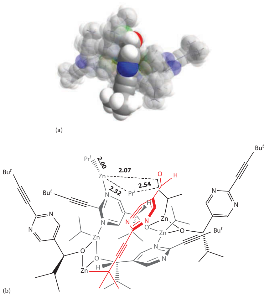
Figure 2.16 (a,b) Transition state for the direct transfer of the isopropyl group from the N-bound \text{ZnPr}_2 computed for the alkylation of aldehyde with the catalyst 4 (B3LYP/6-31G [CPCM, toluene]). The importance of the specifically shaped substrate accurately fitting to the cavity is illustrated on the space-filling model. (Reproduced with permission from Gridnev, I. D. et al., ACS Catal. , 2, 2137–2149, 2015.)
