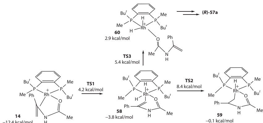
Scheme 1.17 Competition between migratory insertion and double bond dissociation in the dihydride intermediate 58 . (Reprinted with permission from Gridnev, I. D. and Imamoto, T. ACS Catal. , 5, 2911–2915. Copyright 2015 American Chemical Society.)
