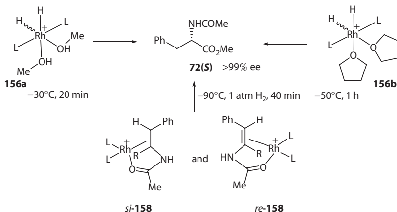
Scheme 1.38 Three different experiments carried out at decreased temperatures. (Gridnev, I. D. et al., Chem. Commun. , 48, 2186–2188, 2012. Reproduced by permission of The Royal Society of Chemistry.)
