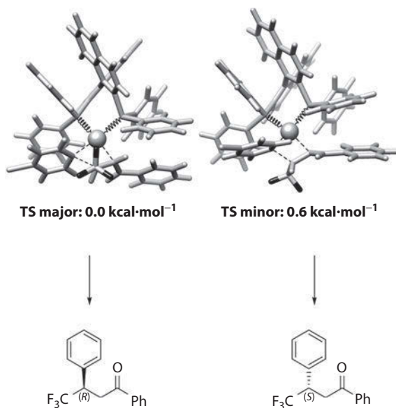
Figure 2.13 The most favorable transition states leading to major ( R )- and minor ( S )-product. Optimized at B3LYP/LANL2DZ(Rh)/6-31G*(all others) level of theory.
