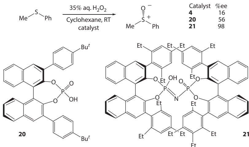
Scheme 3.8 Dependence of the optical yield in asymmetric sulfoxidation on the size of the catalyst. (Data from Jindal, G. and Sunoj, R. B., Angew. Chem. Int. Ed. , 53, 4432–4436, 2014.)
