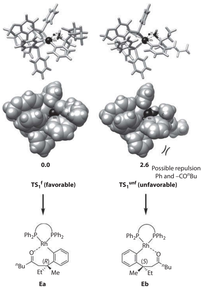
Figure 2.7 Enantioselectivity-determining transition states. Standard free energy (gas free energy calculations corrected by single-point solvation free energy), kcal/mol.
