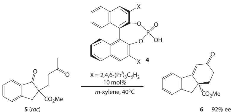
Scheme 3.3 Kinetic resolution catalyzed by chiral BINOL-based phosphoric acids.
