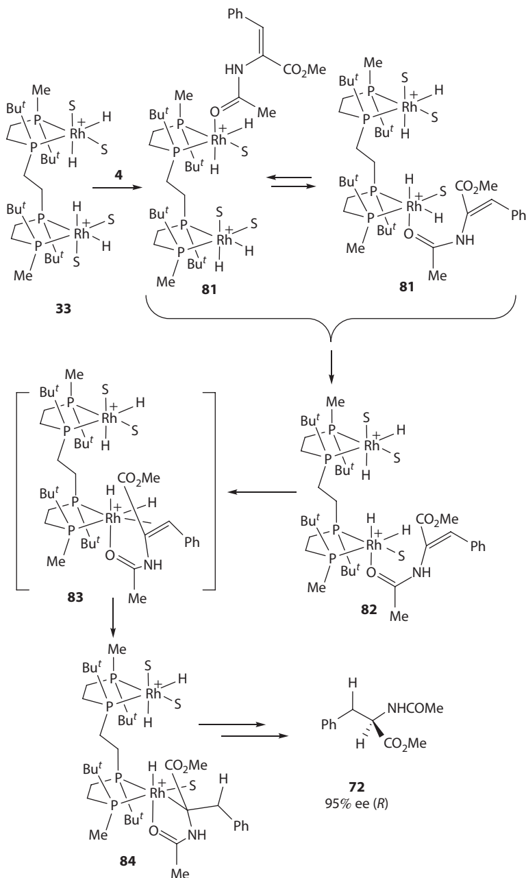
Scheme 1.24 Low-temperature reaction of dirhodium tetrahydride complex 33 with MAC 4 . (Gridnev, I. D. and Imamoto, T., Chem. Commun. , 7447–7464, 2009. Reproduced by permission of The Royal Society of Chemistry.)
