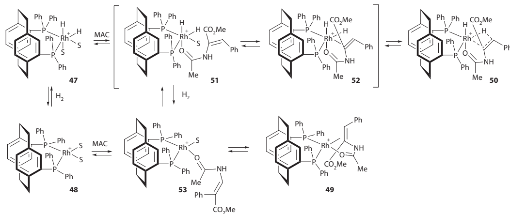
Scheme 1.14 Reversible formation of the agostic intermediate 50 . (Adapted from Heinrich, H. et al. Chem. Commun. , 1296–1297, 2001. With permission.)
