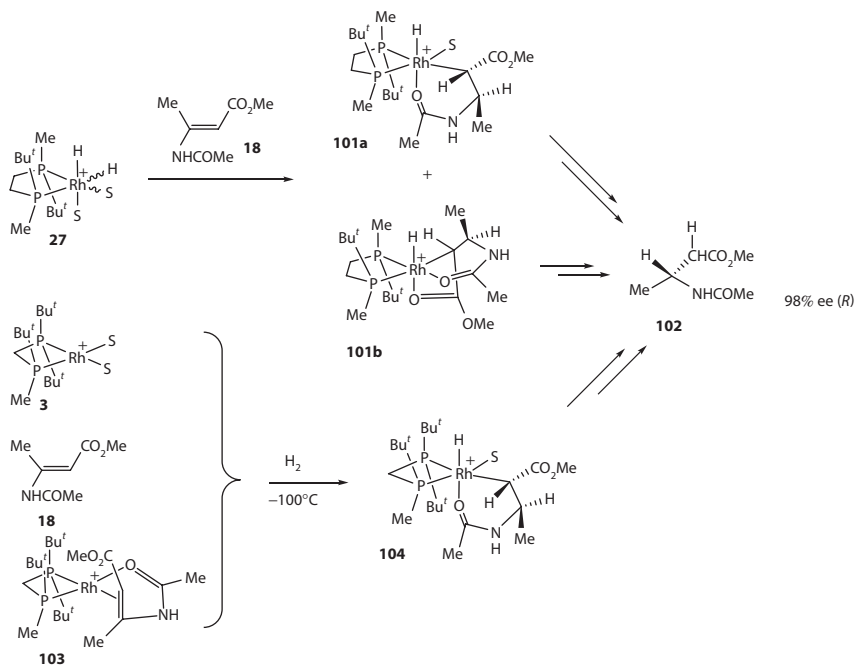
Scheme 1.28 Detection of \beta -monohydride intermediates in low-temperature reaction of solvate dihydride 27 and ester of \beta -dehydroamino acid 18 , and in low-temperature hydrogenation of the equilibrium mixture of 3 , 18 , and 103 .
