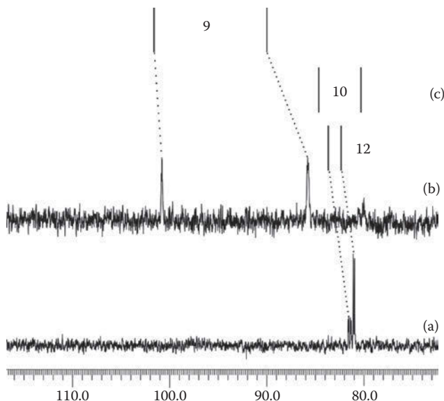
Figure 1.1 Section plots of ^{13}\text{C} NMR spectra (100 MHz, \text{CD}_3\text{OD} ) showing signals from carbon atoms of the coordinated double bond. (a) Solution obtained by the addition of two equivalents of MAC to a deuteriomethanol solution of 7 at 25^\circ\text{C} . Spectrum measured at 25^\circ\text{C} . (b) The same reagents were mixed at -100^\circ\text{C} and the sample was put into the pre-cooled probe of the NMR spectrometer. Spectrum measured at -90^\circ\text{C} . (c) Computed chemical shifts (BLYP/SDD(Rh)6-31 + G(2d,2p)/CPCM(methanol)). (Reprinted with permission from Imamoto, T. et al., J. Am. Chem. Soc. , 134, 1754–1769. Copyright 2012 American Chemical Society.)
