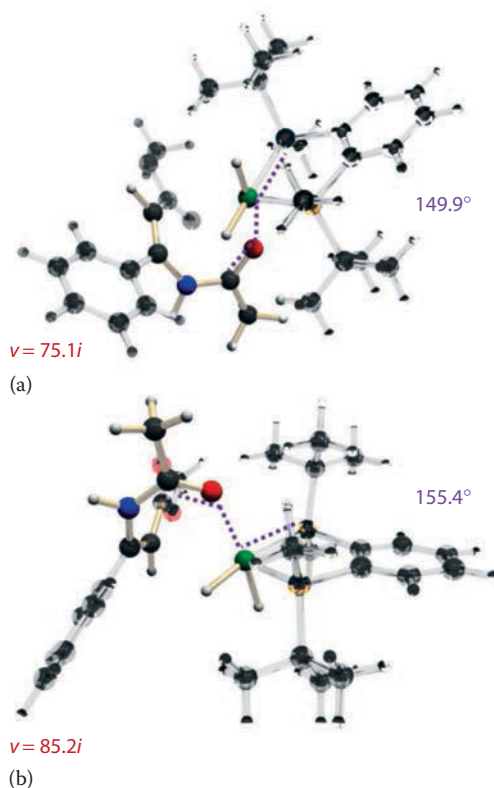
Figure 1.13 Optimized structures of TS19 (a, leads to the formation of R -product) and TS20 (b, leads to formation of S -product). The larger dihedral angle is observed in TS20 , because the forming chelating cycle avoids close approach to the Bu t group. (Reprinted with permission from Gridnev, I. D. et al., ACS Catal. , 4, 203–219. Copyright 2014 American Chemical Society.)
