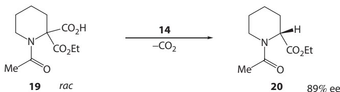
Scheme 3.25 Hybrid thiourea–cinchona-catalyzed asymmetric decarboxylative protonation. (Data from Blanchet, J. et al., Eur. J. Org. Chem. , 5493, 2008.)
