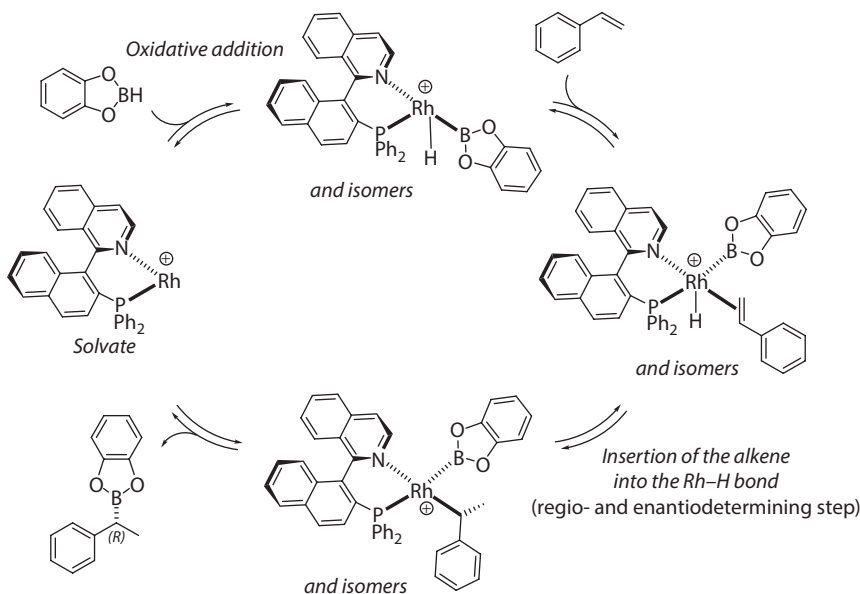
Scheme 2.14 Presently accepted catalytic cycle for the cationic Rh-catalyzed asymmetric hydroboration of vinylbenzene leading to Markovnikov product.
