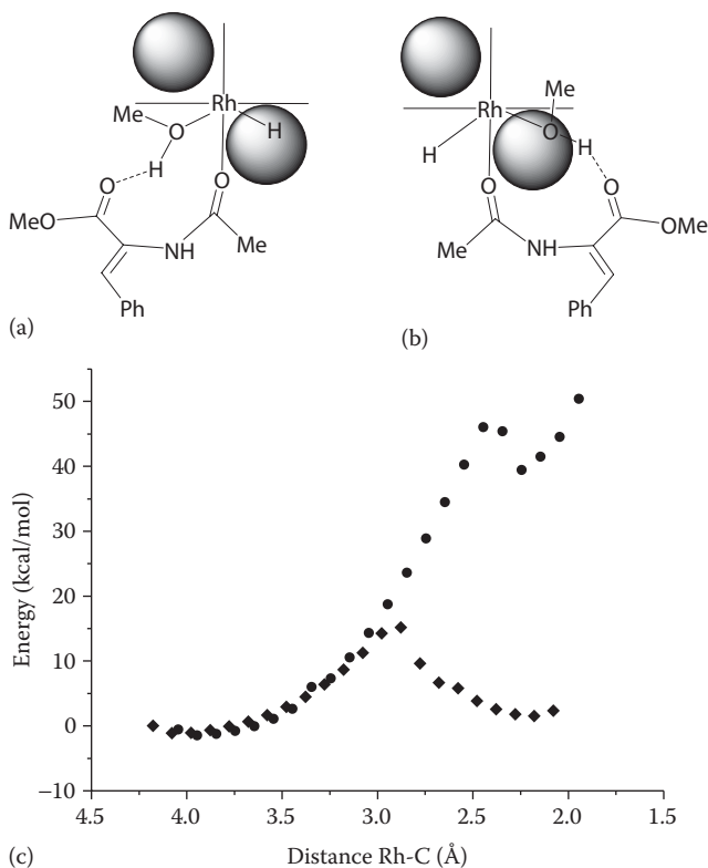
Figure 1.10 Scan of relative energies of the double bond replacing the MeOH molecule at the Rh coordination site: chelate cycle formed in a less hindered quadrant (squares); chelate cycle formed in a hindered quadrant (circles). Computed at the B3LYP/SDD(Rh)/6-31G(d, p)(all others)/CPCM(MeOH) level of theory with additional diffuse function for phosphorus. (Gridnev, I. D. et al., Dalton Trans. , 43, 1785–1790, 2014. Reproduced by permission of The Royal Society of Chemistry.)
