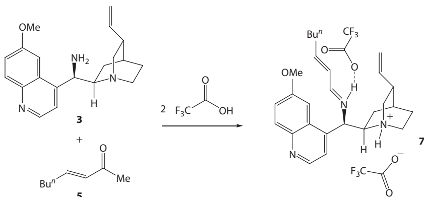
Scheme 3.13 Initial formation of iminium cation 7 .
