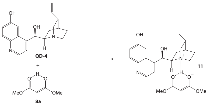
Scheme 3.15 Initial formation of complex 11 from cinchona alkaloid QD-4 and enole form of dimethyl malonate 8a suggested in the computational study. (Data from Jiang, H. et al., Int. J. Quant. Chem. , 114, 642–651, 2014.)
