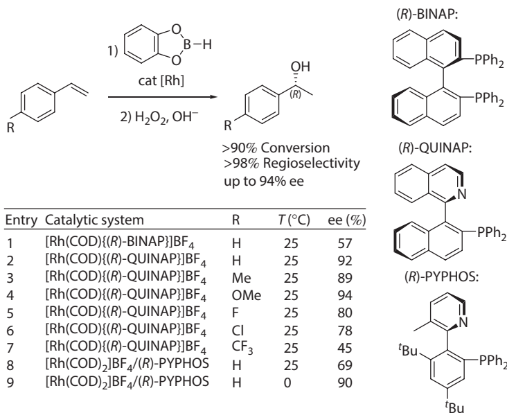
Scheme 2.13 Reactions.
