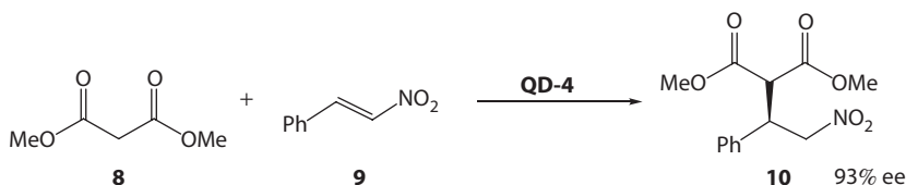
Scheme 3.14 Conjugate addition of dimethyl malonate to \beta -nitrostyrene catalyzed by cinchona alkaloid QD-4 .
