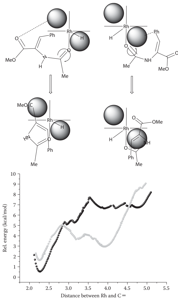
Figure 1.11 Scans of the relative energy of the double bond coordination to a free coordination site of the nonchelating Rh(III) octahedral complexes. Computations were done on the B3LYP-D3/6-31G*/SMD(methanol) level of theory. Gray spheres: coordination drawn in the upper left Scheme; black spheres: coordination drawn in the upper right Scheme.
