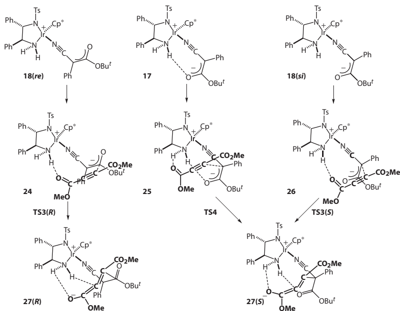
Scheme 2.6 Competing pathways in the C—C bond forming reaction catalyzed by the Ir complex 14. (Adapted with permission from Hasegawa, Y. et al., Bull. Chem. Soc. Jpn. , 85, 316–334, 2012. Copyright the Chemical Society of Japan.)
