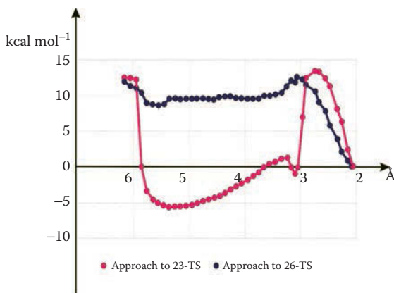
Figure 1.33 Energy scans simulating the approach of the substrate to the corresponding Ir hydrides. The final minima correspond to the completely optimized structures of adducts. (Liu, Y. et al.: Mechanism of the asymmetric hydrogenation of exocyclic \alpha,\beta -unsaturated carbonyl compounds with an iridium/BiphPhox catalyst: NMR and DFT studies. Angew. Chem. Int. Ed. 2014, 53, 1901–1905. Copyright Wiley-VCH Verlag GmbH & Co. KGaA. Reproduced with permission.)
