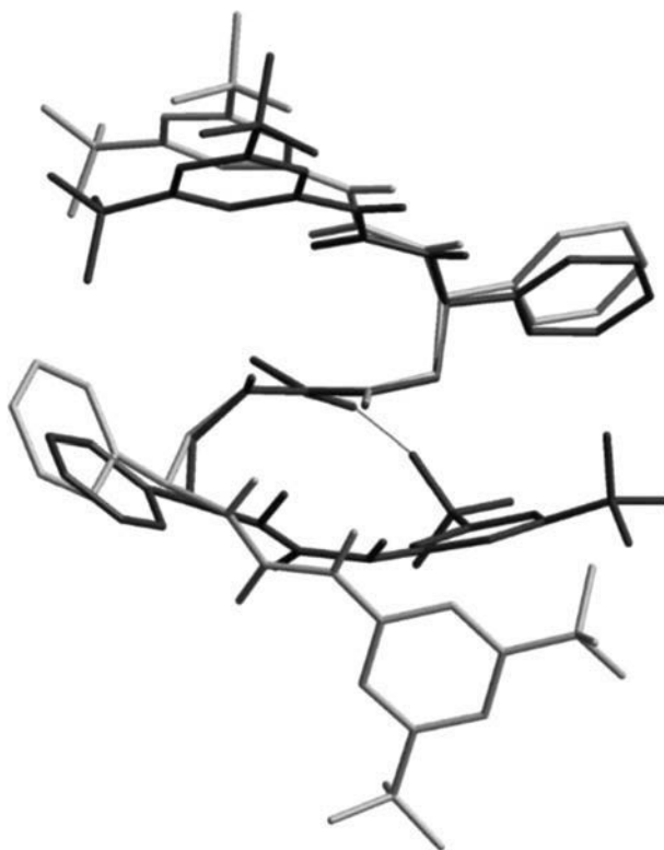
Figure 3.13 The 3D superposition of the catalyst structures in TS11 (light tube: B3LYP/6-31G*, dark tube: M05-2X/6-31G*). (Adapted with permission from Odagi, M. et al., J. Am. Chem. Soc. , 137, 1909–1915. Copyright 2015 American Chemical Society.)
