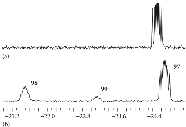
Figure 1.6 Hydride region of the ^1\text{H} NMR spectrum (400 MHz, \text{CD}_3\text{OD} ) of the reaction mixture obtained by the low-temperature hydrogenation of the equilibrium mixture of 27 , 94 , 95a and 95b : (b) at -90^\circ\text{C} ; (a) at -50^\circ\text{C} . Assignment of 97 as \alpha -monohydride, and of 98 , 99 as \beta -monohydrides was confirmed by the experiments using ^{13}\text{C} labeled enamide 51 similar to that described in Figure 1.5. (Reprinted with permission from Gridnev, I. D. et al., J. Am. Chem. Soc. , 123, 5268–5276. Copyright 2001 American Chemical Society.)
