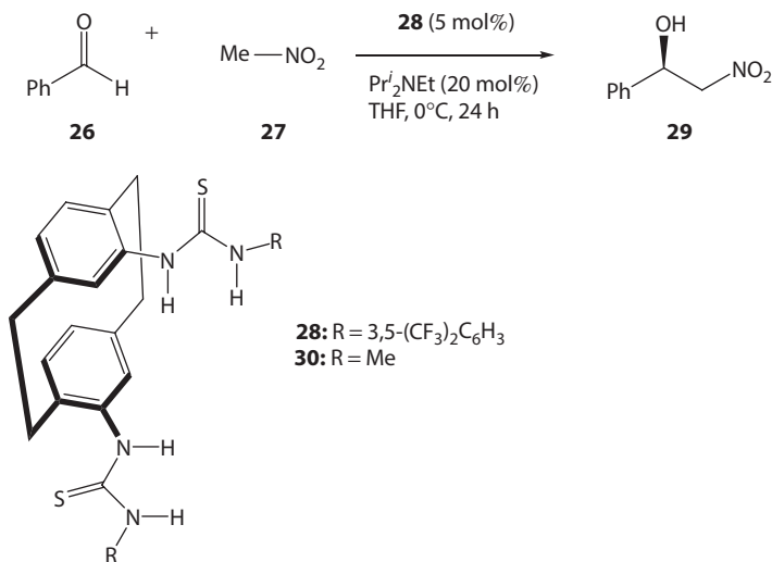
Scheme 3.27 Cyclophane-based bistiourea-catalyzed asymmetric Henry reaction. (Data from Kitagaki, S. et al., Chem. Commun. , 49, 4030–4032, 2013; Breugst, M. and Houk, K. N., J. Org. Chem. , 79, 6302–6309, 2014.)
