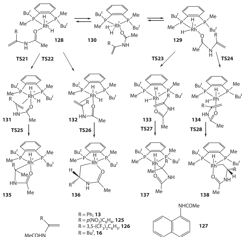
Scheme 1.34 Enantioselective stages in the asymmetric hydrogenation of enamides. (From Gridnev, I. D. and Imamoto, T. Izv. Akad. Nauk, Ser. Khim. , 1514–1534, 2016. With permission.)
