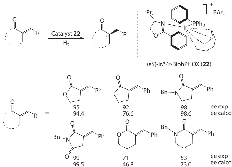
Scheme 1.51 Asymmetric hydrogenation of exocyclic \alpha,\beta -unsaturated carbonyl compounds with an Ir/BiphPhox catalyst.
