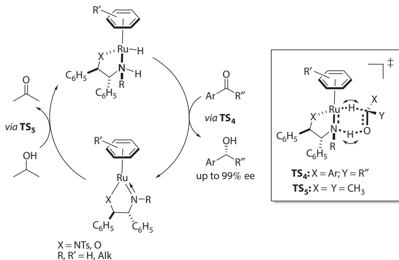
Scheme 1.42 Catalytic cycle for the transfer hydrogenation of aromatic ketones by an active form of the Noyori-Ikariya (pre)catalyst 2 from early studies. Formation of the major enantiomeric product is shown. (Reprinted with permission from Dub, P. A. et al., Dalton Trans. , 45, 6756–6781. Copyright 2016 Royal Society of Chemistry.)
