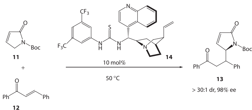
Scheme 3.22 Michael addition reaction catalyzed by hybrid thiourea–cinchona alkaloid catalyst 14 . (Data from Zhu, J.-L. et al., J. Org. Chem. , 77, 9813–9825, 2012.)
