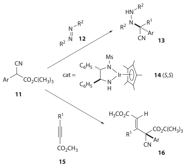
Scheme 2.3 Opposite stereochemical outcome of the C—N and C—C bond forming reactions using the same catalyst 14 and phenyl- \alpha -cyanoacetate 11 .
