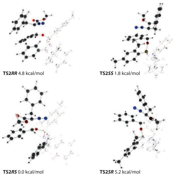
Figure 3.15 Optimized structures of the diastereomeric transition states for the C–C bond formation accompanied by release of N 2 . (Adapted with permission from Wang, Y. et al., J. Phys. Chem. A , 119, 8422–8431. Copyright 2015 American Chemical Society.)
