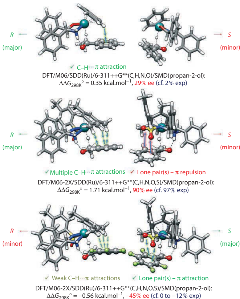
Figure 1.25 (S)-RuH[( R , R )-N(Ts)CH(Ph)CH(Ph)NH 2 ]( \eta^6 -mes)-C 6 H 5 C(O)CH 3 or C 6 F 5 C(O)CH 3 : optimized transition states leading to R - and S -products. The enantioselectivity is calculated 254 based on difference in free energies using absolute rate theory. 184,185
