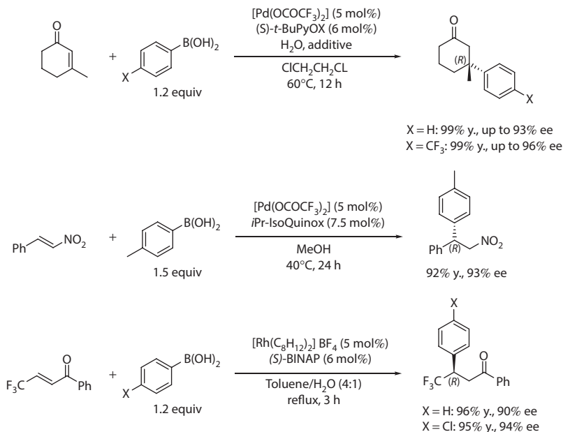
Scheme 2.10 Catalytic reactions.
