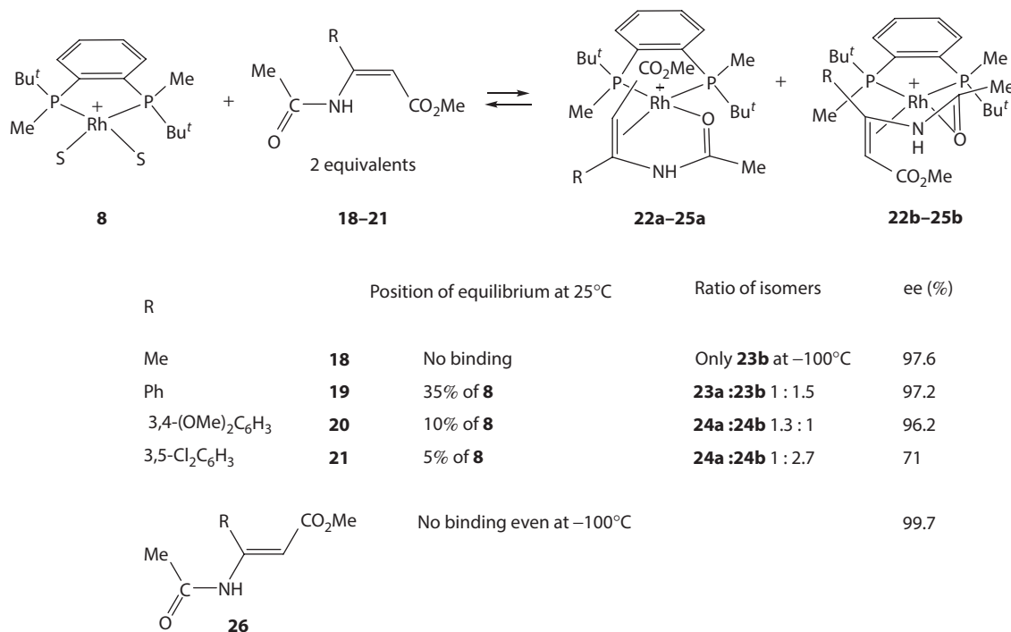
Scheme 1.6 Formation of catalyst-substrate complexes of catalyst 8 and esters of \beta -dehydroamino acids. (From Gridnev, I. D. et al., ACS Catal. , 4, 203–219, 2014. With permission.)
