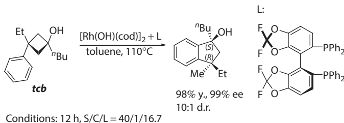
Scheme 2.8 Rh-catalyzed stereoselective isomerization of tert-cyclobutanol tcb into corresponding chiral indanole.
