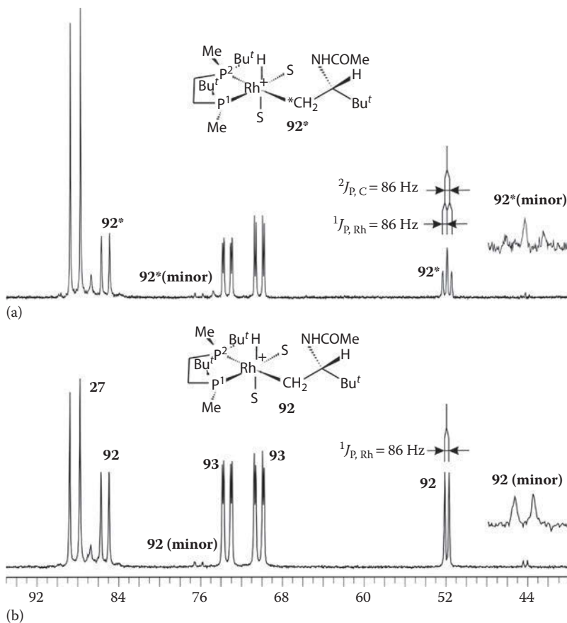
Figure 1.5 ^{31}\text{P} NMR spectra (162 MHz, -90^\circ\text{C} , \text{CD}_3\text{OD} ) of the reaction mixtures containing monohydride intermediate 92 : (b) unlabeled: (a) labeled with ^{13}\text{C} at the methylene carbon atom. Additional large coupling observed in the case of the labeled compound proves that 92 has a structure of \beta -monohydride. The minor isomer is evidently also \beta -monohydride; the ee obtained after quenching of the sample is higher than that calculated based on the relative amounts of major and minor diastereomers. Hence, the major and minor isomers differ in the configuration of the Rh atom. Catalyst–substrate complex 93 was also formed in this experiment. Low-temperature hydrogenation of 93 yields identical spectra. (Reprinted with permission from Gridnev, I. D. et al., J. Am. Chem. Soc. , 123, 5268–5276. Copyright 2001 American Chemical Society.)
