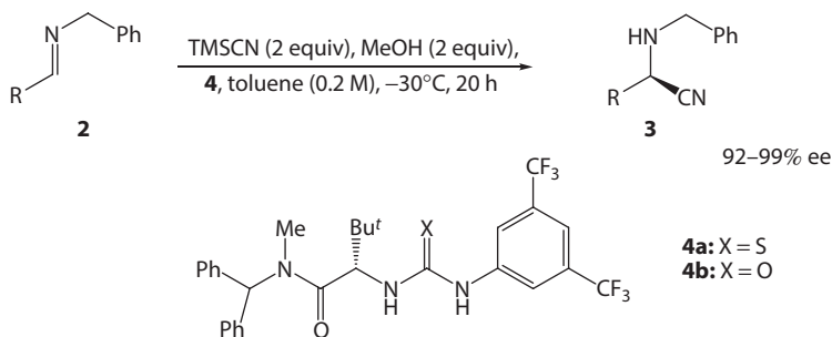
Scheme 3.19 Model reaction used for combined experimental and computational study. (Adapted with permission from Zuend, S. J. and Jacobsen, E. N., J. Am. Chem. Soc. , 129, 15872–15883. Copyright 2007 American Chemical Society.)
