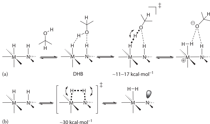
Scheme 1.44 Two ways of H-H bond formation. (Reprinted with permission from Dub, P. A. et al., Dalton Trans. , 45, 6756–6781. Copyright 2016 Royal Society of Chemistry.)
