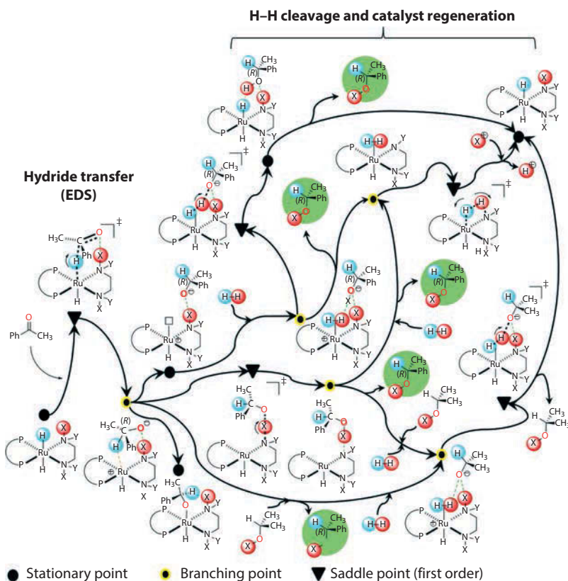
Scheme 1.48 “Reaction path” 198,340 (conceivable catalytic pathways and their crossover) of the catalytic hydrogenation of acetophenone with the active form of 1 using the assumption that tunneling is involved in so-called H-H bond cleavage via metal-ligand cooperation and that computational accuracy is >10 kcal/mol ( X = Y = \text{H} and/or \text{K} ). There are five possibilities to neutralize the anion of the product obtained after EDS hydride transfer and regenerate the catalyst via three associated TS's corresponding to H-H bond cleavage. Some selected stationary and saddle points are omitted for clarity. (Reprinted with permission from Dub, P. A. et al., Dalton Trans. , 45, 6756–6781. Copyright 2016 Royal Society of Chemistry.)
