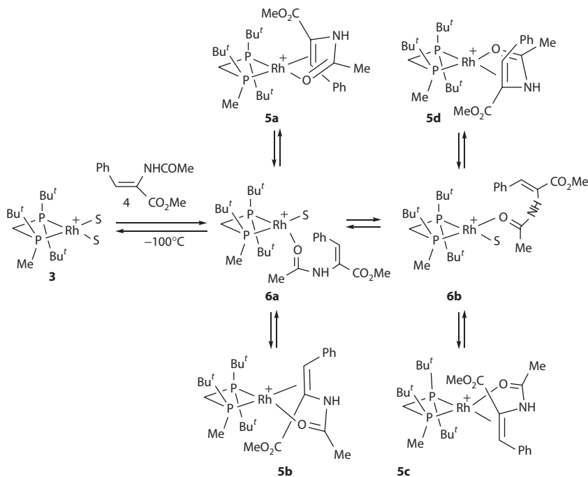
Scheme 1.2 Low-temperature reaction of catalyst 3 and substrate 4 . (Gridnev, I. D. and Imamoto, T., Chem. Commun. , 7447–7464, 2009. Reproduced by permission of The Royal Society of Chemistry.)
