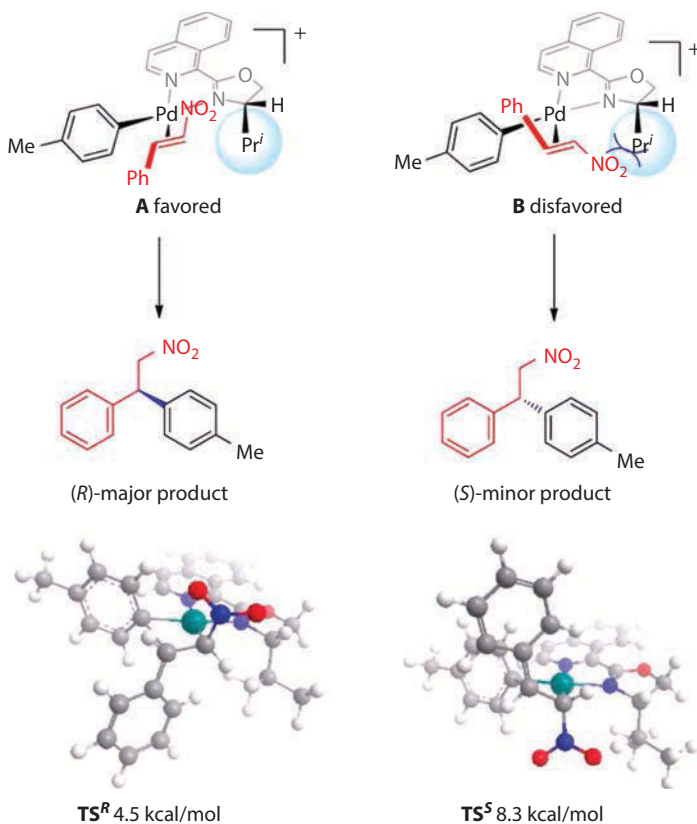
Figure 2.12 Stereochemical model for Pd-catalyzed enantioselective Michael addition of arylboronic acid to nitroalkene. (Adapted with permission from He, Q. et al., Org. Lett. , 17, 2250–2253. Copyright 2015 American Chemical Society.)
