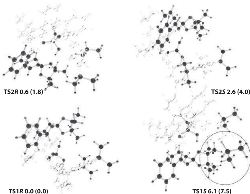
Figure 3.2 Optimized structures of the transition states TS1R , TS2R , TS1S , and TS2S . In full brightness are shown the reactants, \text{HPO}_4 unit of the catalyst and the isopropyl substituents interfering with the allylboronate in the TS1S . Relative energies in kcal/mol are shown for the B3LYP/6-31G* optimizations in gas phase, the values in brackets are results of energy calculations with B3LYP-D3. (Adapted with permission from Wang, H. et al., J. Org. Chem. , 78, 1208–1215. Copyright 2013 American Chemical Society.)
