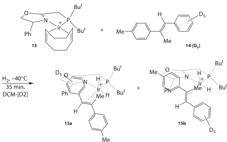
Scheme 1.50 Interception of dihydride intermediates 15a and 15b . (From Gruber, S. and Pfaltz, A., Angew. Chem. Int. Ed. , 53, 1896–1900, 2014. With permission.)
