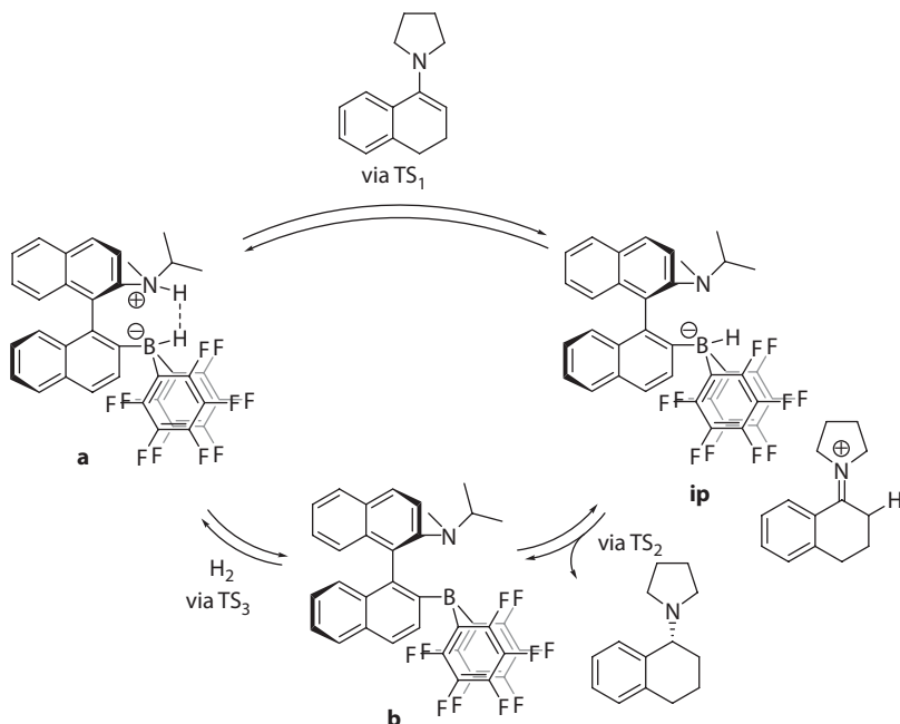
Figure 3.16 Proposed catalytic cycle for the FLP-catalyzed asymmetric hydrogenation of 1,2-dihydro-4-pyrrolidinonaphthalene.
