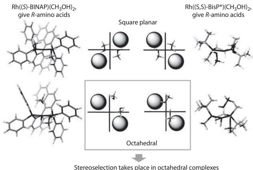
Figure 1.18 Optimized structures (B3LYP/SDD) of the square planar solvate Rh(I) complexes [\text{Rh}((S)\text{-BINAP})(\text{CH}_3\text{OH})_2]^+ and [\text{Rh}((S,S)\text{-}t\text{-Bu-BisP}^*)(\text{CH}_3\text{OH})_2]^+ (top), and octahedral solvate dihydride Rh(III) complexes [\text{RhH}_2((S)\text{-BINAP})(\text{CH}_3\text{OH})_2]^+ and [\text{RhH}_2((S,S)\text{-}t\text{-Bu-BisP}^*)(\text{CH}_3\text{OH})_2]^+ (below). The orientation of the methanol molecules helps to determine the less hindered quadrant in each case (in octahedral complexes the equatorially coordinated methanol molecule is brought away from the substituents on the phosphorus atoms, hence only the position of the axially coordinated methanol molecule is informative). In case of the P-chiral t -Bu-BisP* complexes (right), the quadrant diagram is the same for Rh(I) and Rh(III) because the relative size of the substituents always remains the same. Hence, it can be concluded that when a large substituent is in the upper left corner, R -amino acids are produced. In the case of tetraphenyl-substituted BINAP complexes, the quadrant diagram is opposite for square planar and octahedral complexes. The Rh-( S )-BINAP complex gives R -amino acids in asymmetric hydrogenation, hence the arrangement of the larger and smaller substituents in the stereodiscriminating step must be the same as in the t -Bu-BisP* case. Thus, one can conclude from these data that stereoselection takes place in octahedral complexes. (Gridnev, I. D. and Imamoto, T., Chem. Commun. , 7447–7464, 2009. Reproduced by permission of The Royal Society of Chemistry.)
