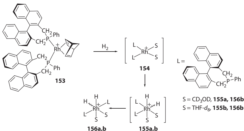
Scheme 1.37 Hydrogenation of the catalytic precursor 153 . (Gridnev, I. D. et al., Chem. Commun. , 48, 2186–2188, 2012. Reproduced by permission of The Royal Society of Chemistry.)
