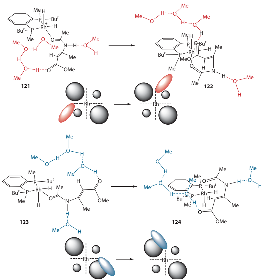
Scheme 1.33 Modeling the coordination of the double bond with four methanol molecules. (Reprinted with permission from Gridnev, I. D. et al., ACS Catal. , 4, 203–219. Copyright 2014 American Chemical Society.)
