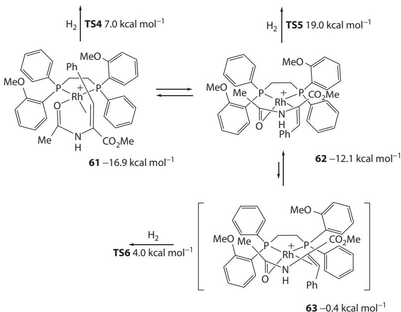
Scheme 1.18 Oxidative addition of H_2 to the catalyst–substrate complexes 61 – 63 . (From Gridnev, I. D. and Imamoto, T. Izv. Akad. Nauk, Ser. Khim. , 1514–1534, 2016. With permission.)
