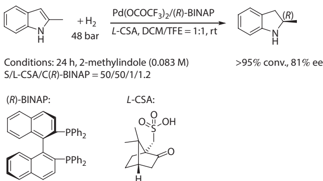
Scheme 1.53 Catalytic hydrogenation of 2-Methylindole
