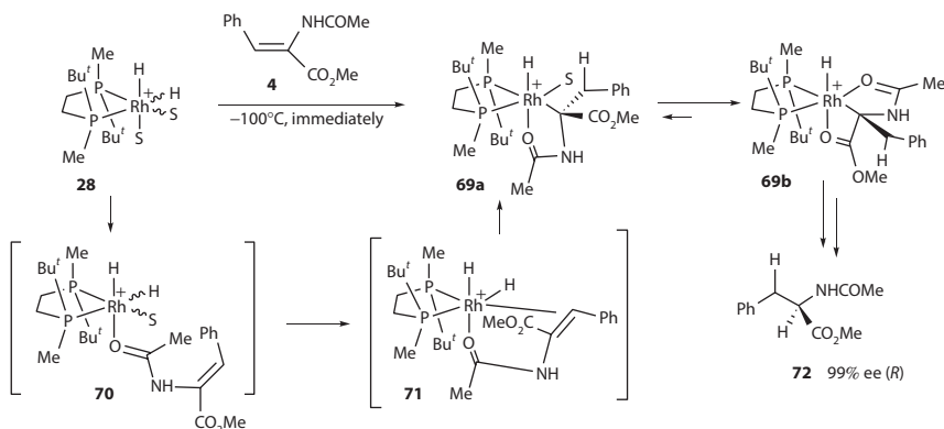
Scheme 1.20 Enantioselective low-temperature reaction of solvate dihydride 28 with MAC ( 4 ). (Reprinted with permission from Gridnev, I. D. et al., J. Am. Chem. Soc. , 122, 7183–7194. Copyright 2000 American Chemical Society.)
