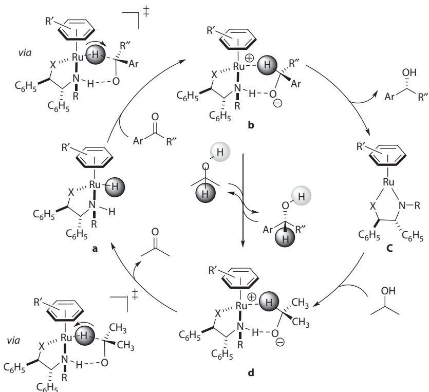
Scheme 1.46 A revised catalytic cycle for the asymmetric transfer hydrogenation of aromatic ketones in propan-2-ol by the Noyori-Ikariya (pre)catalyst 2 demonstrates crossover of the reaction pathways: the product is obtained via a H - /H + outer-sphere hydrogenation mechanism and/or step-wise metal-ligand bifunctional mechanism (see text). Formation of the major enantiomeric product is shown. (Adapted from Dub, P. A. et al., J. Am. Chem. Soc. , 135, 2604–2619. Copyright 2013 American Chemical Society.)
