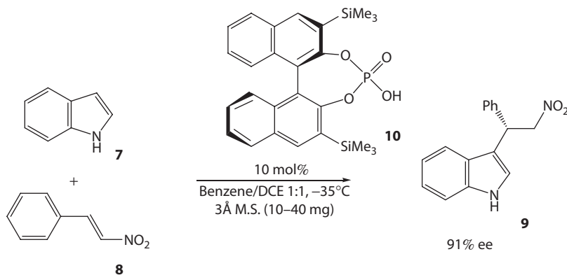
Scheme 3.4 Friedel–Crafts alkylation of indole with nitrostyrene.
