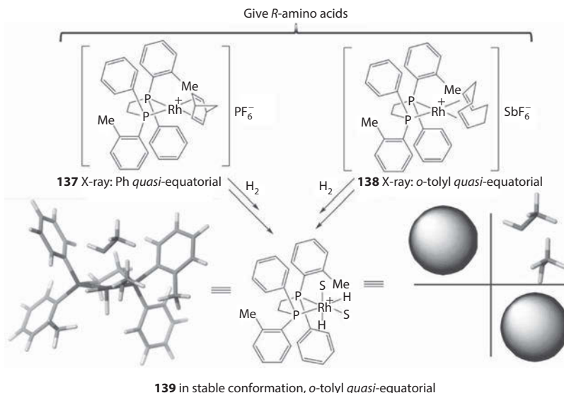
Figure 1.19 In the case of P-chiral ligands with flat aryl substituents, the relative size of the substituents is determined conformationally. (Gridnev, I. D. and Imamoto, T., Chem. Commun. , 7447–7464, 2009. Reproduced by permission of The Royal Society of Chemistry.)
