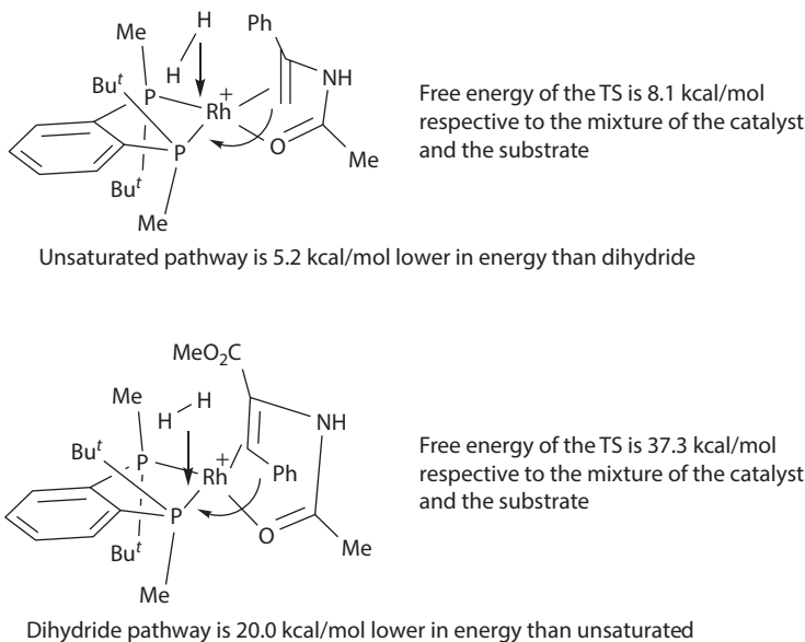
Scheme 1.8 Influence of the substrate structure on the mechanism of H_2 activation.
