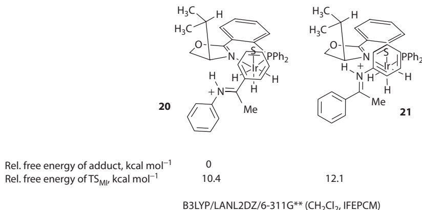
Figure 1.31 Iminium cations 20 , 21 preceding two competing transition states and their relative free energies. 391 The 3D structures of these transition states are available on the CD.
