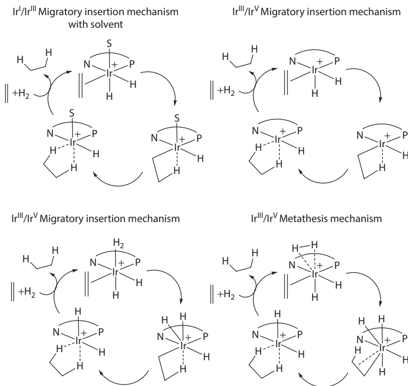
Figure 1.27 Four possible mechanisms of the Ir-catalyzed hydrogenation of simple olefins.
