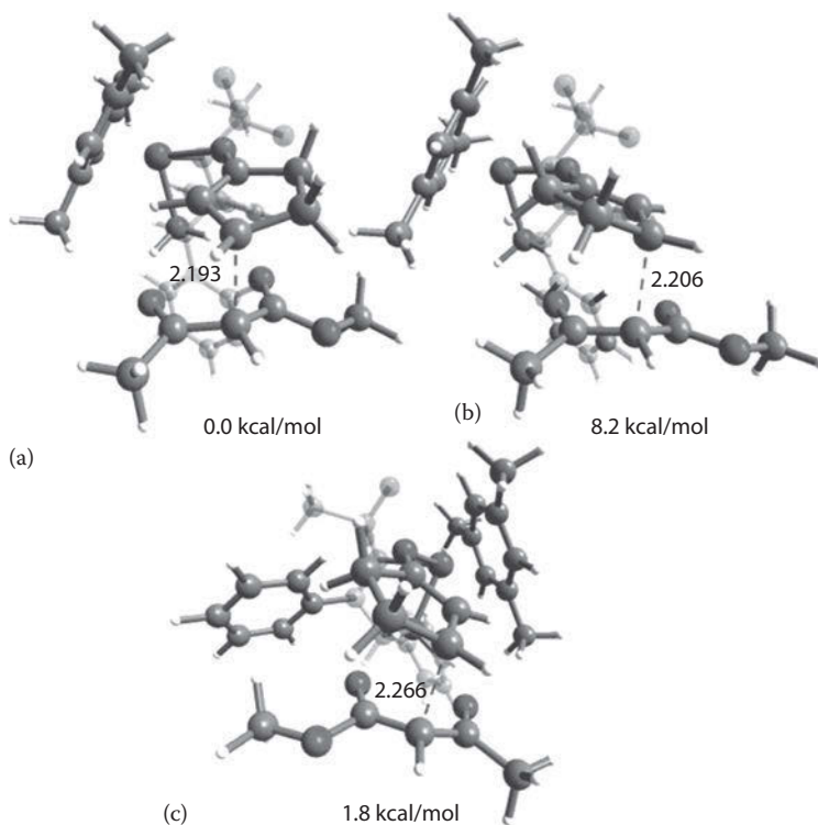
Figure 2.1 Transition states for the Michael addition reaction of malonic ester 61 and cyclopentenone 8 leading to 10(R) (a) and to 10(S) (b and c) and their computed relative energies. (Adapted with permission from Gridnev, I. D. et al., J. Am. Chem. Soc. , 132, 16637–16650. Copyright 2010 American Chemical Society.)
