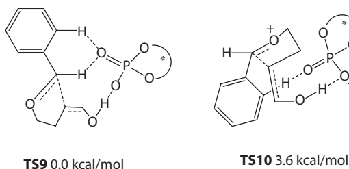
Figure 3.4 Schematic representation of the hydrogen bonding in TS11 and TS12 . (Reproduced from Kanomata, K. et al., Chem. Sci. , 5, 3515–3523, 2014. With permission from The Royal Society of Chemistry.)
