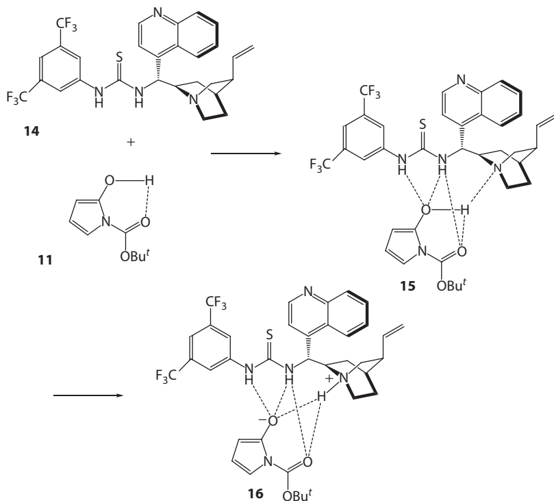
Scheme 3.23 Formation of the catalyst–substrate complex 16 . (Data from Zhu, J.-L. et al., J. Org. Chem. , 77, 9813–9825, 2012.)
