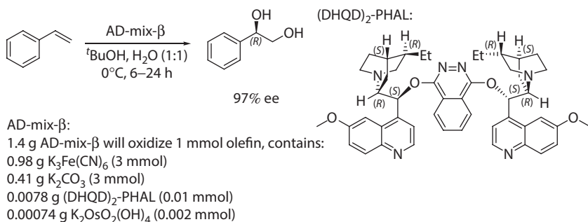
Scheme 2.9 Classical Sharpless asymmetric dihydroxylation reaction.
