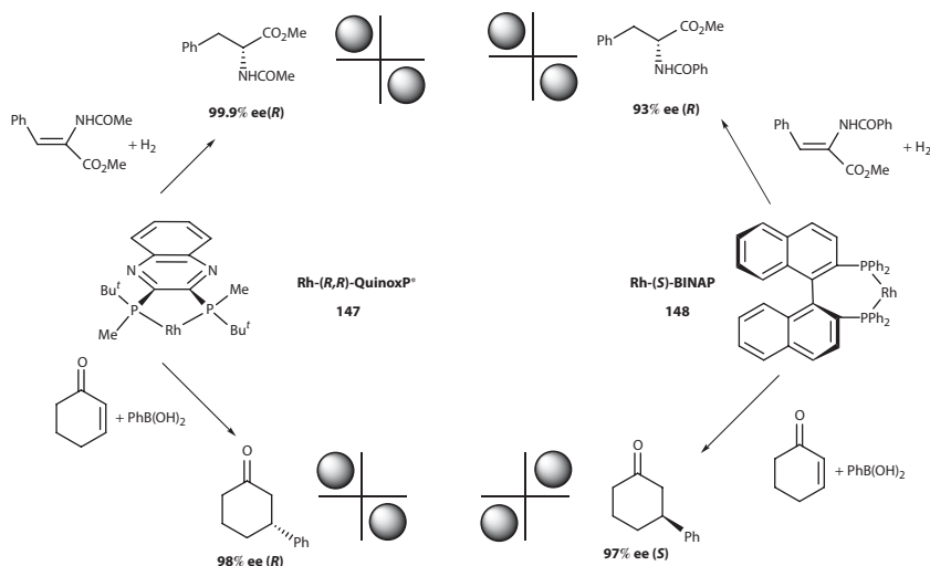
Scheme 1.35 Switch of the sense of enantioselection in the case of Rh-(S)-BINAP complex. (Gridnev, I. D. and Imamoto, T., Chem. Commun. , 7447–7464, 2009. Reproduced by permission of The Royal Society of Chemistry.)
