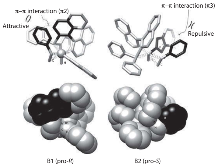
Figure 2.14 The most stable isomers of penta-coordinated H-Rh-(ligand)-catecholborane-styrene complex leading to R - and S -configured products under the assumption that the process proceed via insertion of the double bond into the Rh-H bond.
