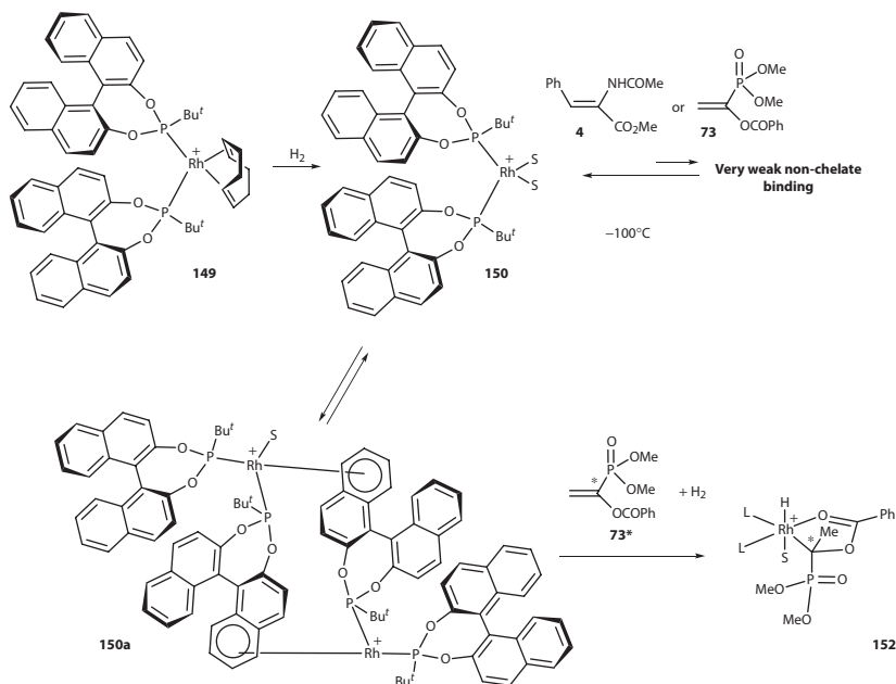
Scheme 1.36 Intermediates detected with the bis-monophosphorus-Rh complex 71 as a catalyst. (Gridnev, I. D. and Imamoto, T., Chem. Commun. , 7447–7464, 2009. Reproduced by permission of The Royal Society of Chemistry.)
