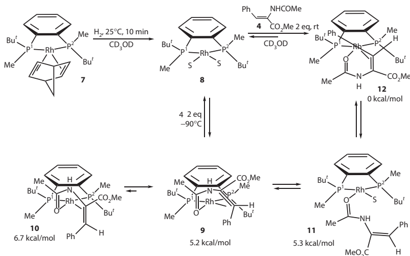
Scheme 1.3 Formation of catalyst–substrate complexes with catalyst 8 and substrate 4 . (Reprinted with permission from Imamoto, T. et al., J. Am. Chem. Soc. , 134, 1754–1769. Copyright 2012 American Chemical Society.)
