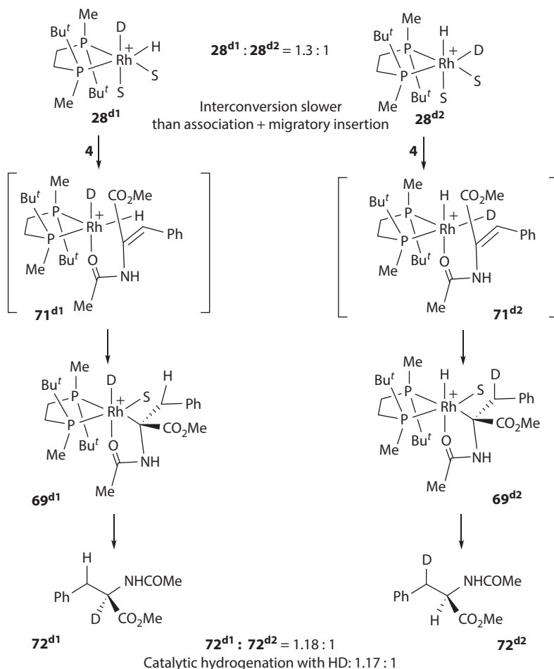
Scheme 1.21 Distribution of deuterium in the hydrogenation product in low-temperature experiments and in catalytic hydrogenation using HD. (Reprinted with permission from Gridnev, I. D. et al., J. Am. Chem. Soc. , 122, 7183–7194. Copyright 2000 American Chemical Society.)
