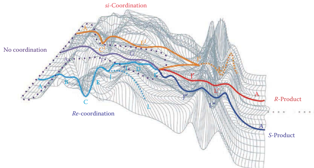
Figure 1.7 Schematic phophile of potential energy for the catalytic cycle of the Rh-catalyzed asymmetric hydrogenation. For explanation see text and Scheme 1.29.
