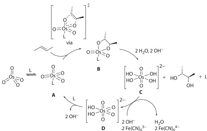
Figure 2.9 Catalytic cycle for the asymmetric dihydroxylation reaction in two phases 'BuOH-H 2 O with \text{K}_3\text{Fe}(\text{CN})_6 as the stoichiometric reoxidant. The ligand is bound via tertiary nitrogen atom.
