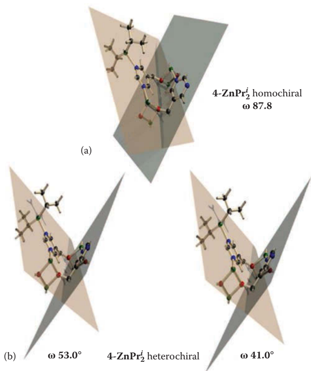
Figure 2.15 Optimized structures of homo- (a) and hetero (b) chiral adducts 4 \bullet \text{ZnPr}_2^i and the angles between pyrimidinyl rings in these molecules that characterize the spaciousness of their 3D cavities.
