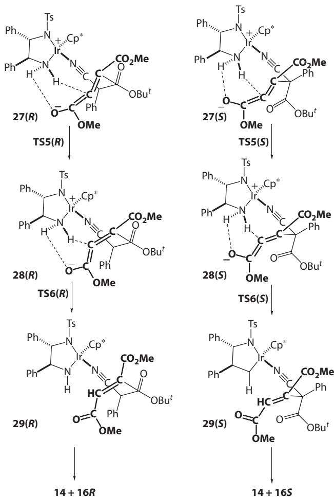
Scheme 2.7 Stereoselective proton transfer in bent allenic intermediates 27(R) and 27(S) . (Adapted with permission from Hasegawa, Y. et al., Bull. Chem. Soc. Jpn. , 85, 316–334, 2012. Copyright the Chemical Society of Japan.)
