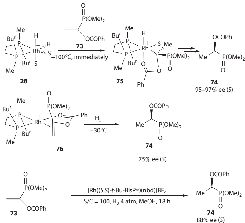
Scheme 1.22 Comparison of the results of low-temperature reaction of 28 and 73 , hydrogenation of the strongly bound catalyst–substrate complex 76 , and catalytic hydrogenation of 73 . 40,41 (Gridnev, I. D. and Imamoto, T., Chem. Commun. , 7447–7464, 2009. Reproduced by permission of The Royal Society of Chemistry.)
