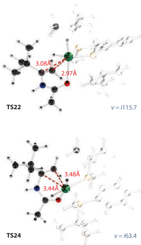
Figure 1.17 Optimized structures of the TS22 and TS24 in the case of substrate 16 . (From Gridnev, I. D. and Imamoto, T. Izv. Akad. Nauk, Ser. Khim. , 1514–1534, 2016. With permission.)
