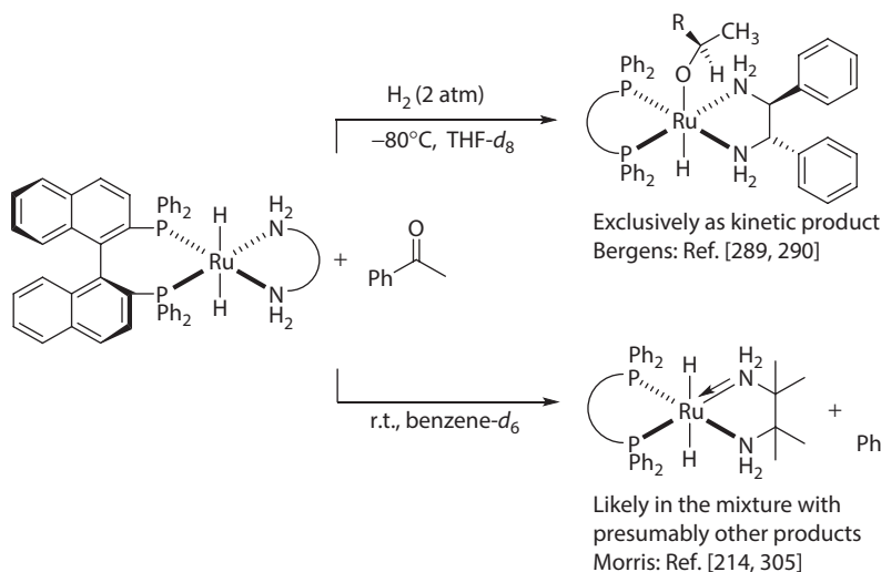
Scheme 1.43 Reported reaction between a trans -dihydride–Ru complex and acetophenone depending on the nature of the NN ligand and other parameters as determined by ^1\text{H} NMR experiment. The outcome of both reactions can be explained based on the existence of a high-energy and/or short lifetime intermediate, not detected (observed) by ^1\text{H} NMR spectroscopy. (Reprinted with permission from Dub, P. A. et al., Dalton Trans. , 45, 6756–6781. Copyright 2016 Royal Society of Chemistry.)
