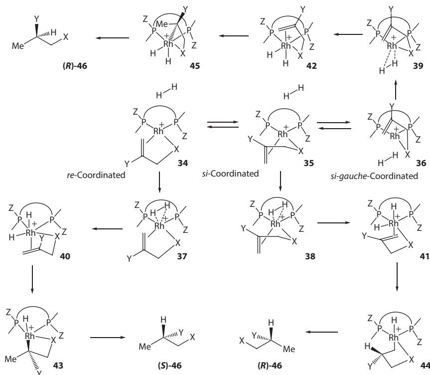
Scheme 1.13 Stereoselection via unsaturated pathway.
