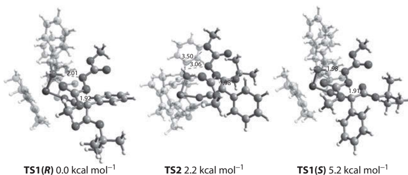
Figure 2.3 Optimized structures and relative energies of the transition states TS1(R) , TS2 , and TS1(S) . (Adapted with permission from Hasegawa, Y. et al., Bull. Chem. Soc. Jpn. , 85, 316–334, 2012. Copyright the Chemical Society of Japan.)
