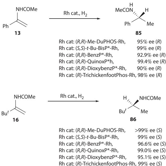
Scheme 1.25 Opposite sense of enantioselection observed in the asymmetric hydrogenation of enamides 13 and 16 .
