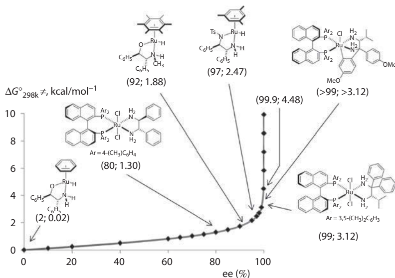
Figure 1.22 Energy differences between averaged catalytic reaction activation barriers leading to major and minor enantiomeric products as a function of the experimentally observed enantioselectivity for AH or ATH of acetophenone catalyzed by 1 and 2 or their derivatives, respectively. RT = 0.59 kcal/mol. (Reprinted with permission from Dub, P. A. et al., Dalton Trans. , 45, 6756–6781. Copyright 2016 Royal Society of Chemistry.)
