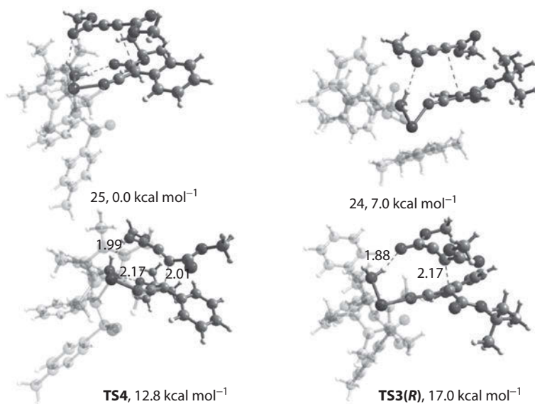
Figure 2.4 Optimized structures and relative energies of adducts and transition states in the C–C bond formation reaction catalyzed by Ir complex 14 . (Adapted with permission from Hasegawa, Y. et al., Bull. Chem. Soc. Jpn. , 85, 316–334, 2012. Copyright the Chemical Society of Japan.)
