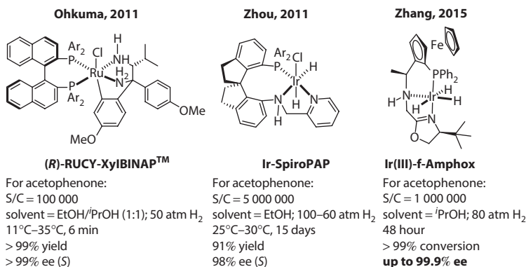
Chart 1.2 Practical hydrogenation catalysts for enantioselective ketones reduction.
