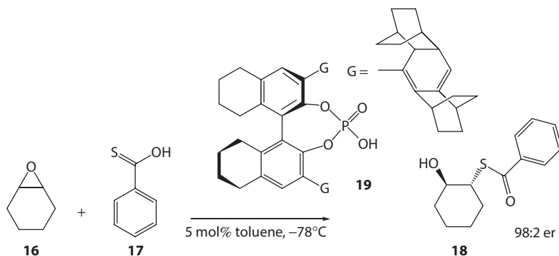
Scheme 3.7 Hydrogenated BINOL-catalyzed thiocarboxylsis of mesoepoxide to generate \beta -hydroxy thioesters. (Data from Ajitha, M. and Huang, K.-W., Org. Biomol. Chem. , 13, 10981–1985, 2015.)
