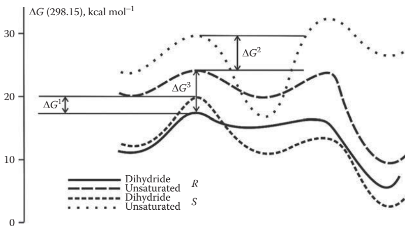
Figure 1.12 Sections of profiles of free energy for the enantioselective stages of the four different catalytic pathways in hydrogenation of 26 catalyzed by 8 . (Reprinted with permission from Gridnev, I. D. et al., ACS Catal. , 4, 203–219. Copyright 2014 American Chemical Society.)
