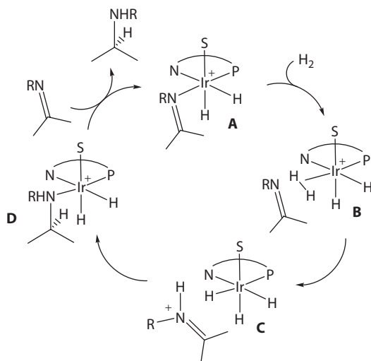
Figure 1.30 Catalytic cycle for the Ir-catalyzed asymmetric hydrogenation of imines. Dihydrogen replaces coordinated imine in A yielding molecular hydrogen complex B with a molecule of imine in the outer sphere. Then imine is protonated by one of the hydrogen atoms from the \text{H}_2 molecule to give neutral \text{Ir}^{\text{III}} complex C . The following hydride transfer of the hydride trans - to phosphorus gives the catalyst–product complex D . Replacement of the product with a new substrate molecule finishes the catalytic cycle recovering A .
