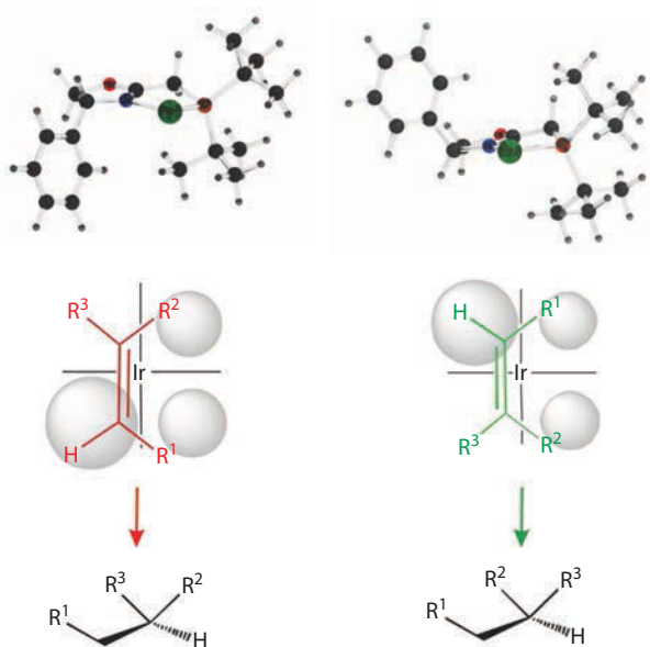
Figure 1.29 Empirical rule for elucidating handedness of the hydrogenation product in the Ir-catalyzed asymmetric hydrogenation of trisubstituted olefins. The most facile migratory insertion takes place if the olefin is coordinated trans -to phosphorus.
