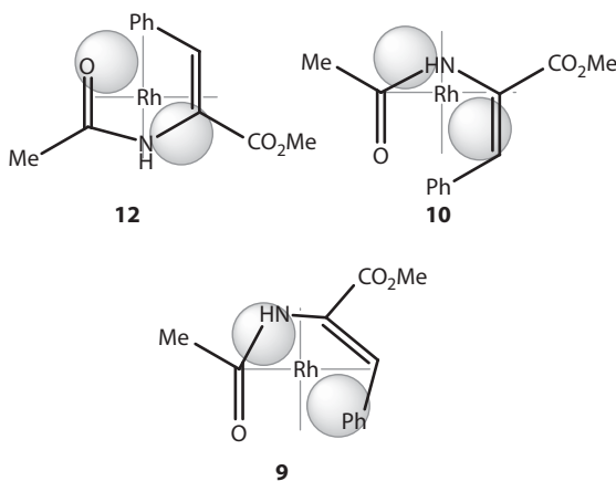
Figure 1.2 Schematic representation of the modes of coordination of the double bond in the catalyst-substrate complexes 9 , 10 , 12 . (From Gridnev, I. D., J. Synth. Org. Chem. Jpn. , 74, 1250–1264, 2014. With permission.)
