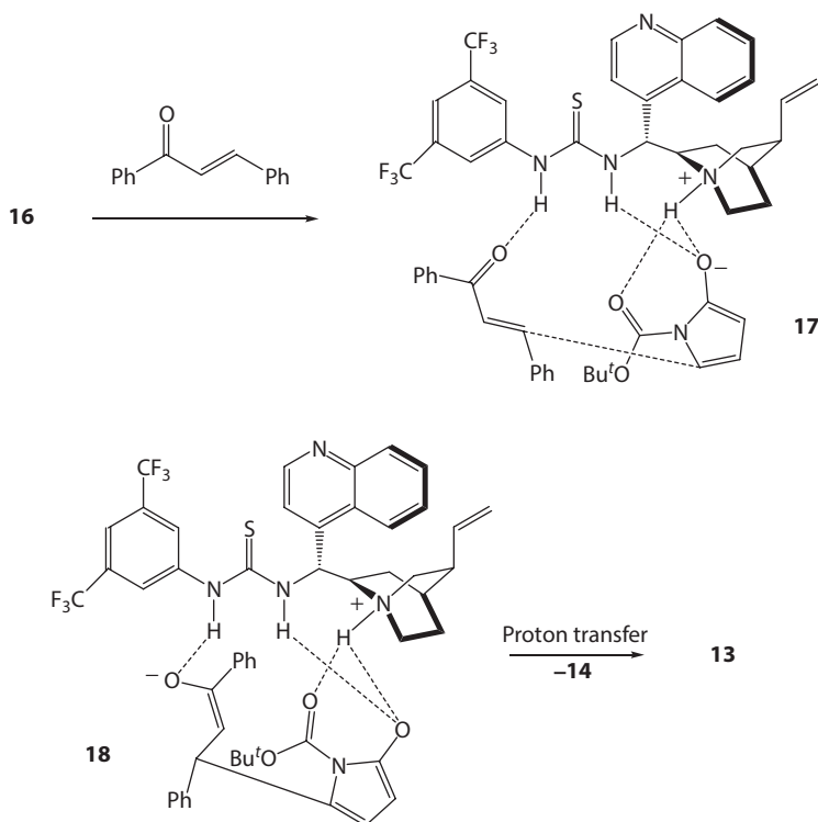
Scheme 3.24 Stereoselective C–C bond formation step.
