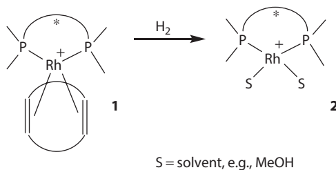
Scheme 1.1 Formation of a catalyst 2 from a catalytic precursor 1 .
