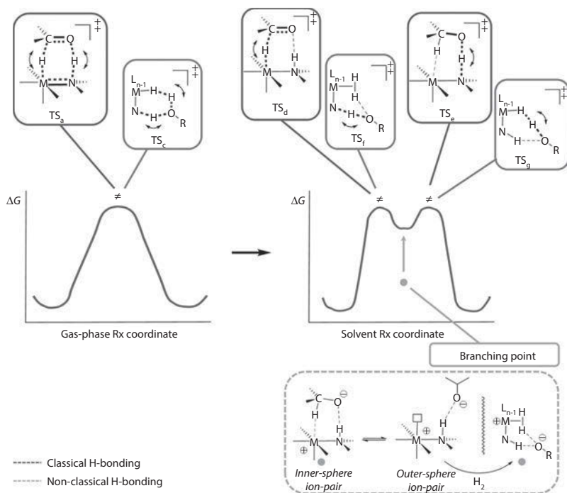
Figure 1.21 Schematic two-dimensional (2D) energy/reaction coordinate type diagram in gas phase and solution for the processes of complete C=O group hydrogenation/dehydrogenation and H–H bond cleavage/formation, respectively. The free energy ( y -axis) is not scaled.
