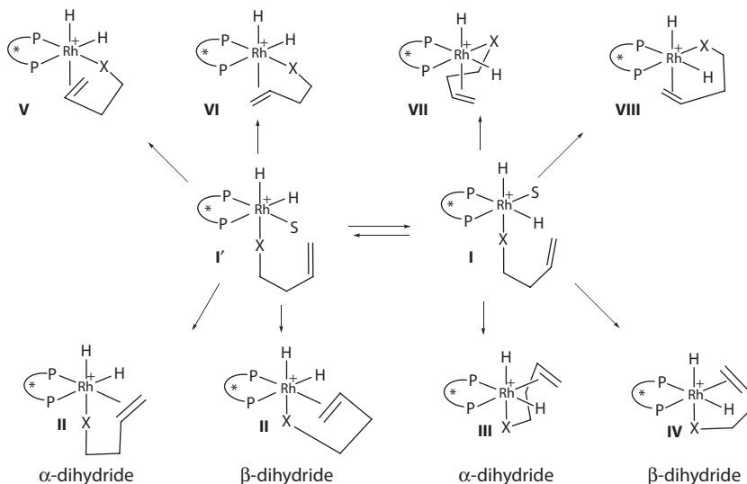
Scheme 1.30 Possible ways for the double bond coordination in I and I'.
