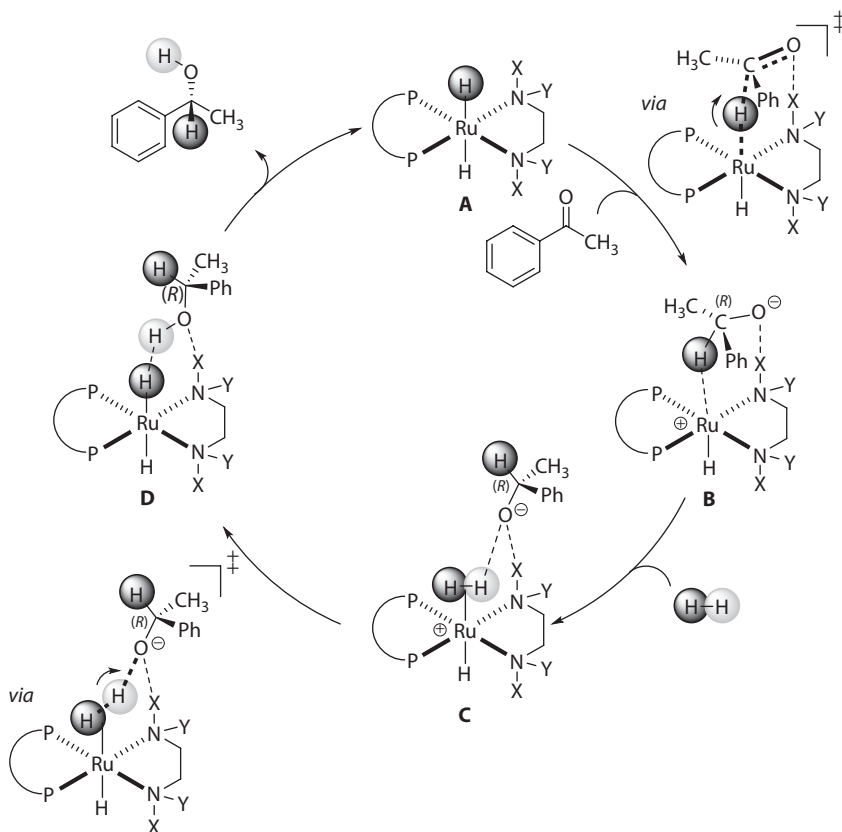
Scheme 1.45 A revised catalytic cycle for the asymmetric hydrogenation of aromatic ketones in propan-2-ol by Noyori's (pre)catalyst 1 based on a computed MEP 253 follows a H - /H + outer sphere hydrogenation mechanism (see text). KO- t -C 4 H 9 -free conditions: X = Y = H. Under high KO- t -C 4 H 9 concentration: X = Y = K and/or H. Formation of the major enantiomeric product is shown. (Adapted from Dub, P. A. et al., J. Am. Chem. Soc. , 136, 3505–3521. Copyright 2014 American Chemical Society.)
