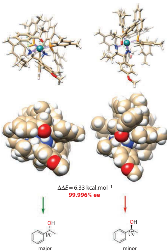
Figure 1.24 [RuH{(S)-xylbinap}]{(S)-daipena}–acetophenone: two diastereomeric transition states leading to (R)-1-phenylethanol and (S)-1-phenylethanol. Optimized under DFT 218,219 /ωB97X-D 332 /SDD(Ru)/6-31G*(C, H,N, O,P)/SMD(propan-2-ol) 333 level of theory. The enantioselectivity is calculated based on difference in electronic energies by using absolute rate theory. 184,185
