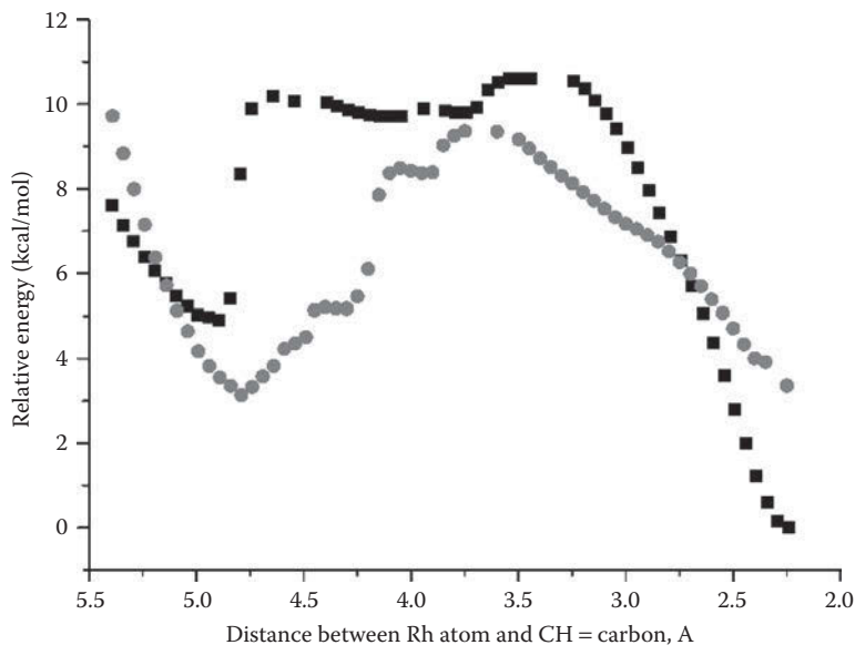
Figure 1.14 Scans of the relative energies changes during the approach of the CH = carbon atom to Rh. Gray: from 121 to 122 . Black: from 123 to 124 . (Reprinted with permission from Gridnev, I. D. et al., ACS Catal. , 4, 203–219. Copyright 2014 American Chemical Society.)
