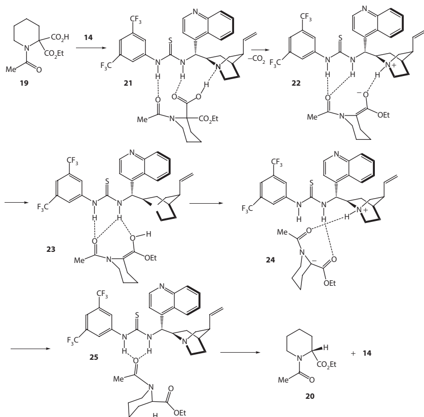
Scheme 3.26 Computed relatively facile mechanism of the enantioselective decarboxylative protonation. (Adapted with permission from Sengupta, A. and Sunoj, R. B., J. Org. Chem. , 77, 10525–10536. Copyright 2012 American Chemical Society.)
