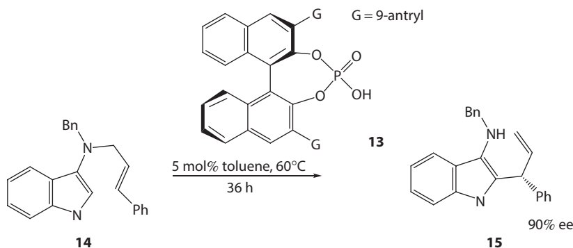
Scheme 3.6 Enantioselective indole aza-Claisen rearrangement.
