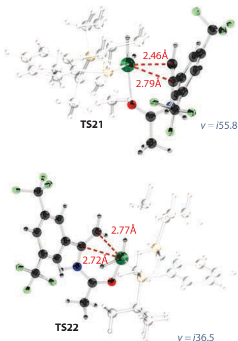
Figure 1.16 Optimized structures of the TS21 and TS22 in the case of substrate 13 . (From Gridnev, I. D. and Imamoto, T. Izv. Akad. Nauk, Ser. Khim. , 1514–1534, 2016. With permission.)
