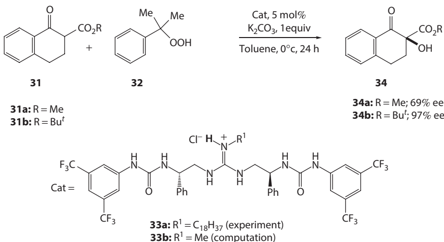
Scheme 3.28 \alpha -Hydroxylation of \beta -ketoesters. (Data from Odagi, M. et al., Chem. Eur. J. , 19, 16740–16745, 2013.)
