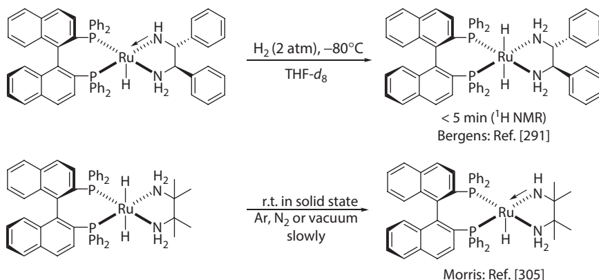
Scheme 1.47 Interpretation of chemical reactivity based on NMR experiment and/or visual observation. (Reprinted with permission from Dub, P. A. et al., Dalton Trans. , 45, 6756–6781. Copyright 2016 Royal Society of Chemistry.)
