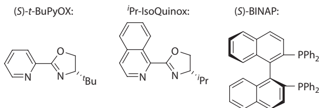
Chart 2.1 Chiral ligands used in the Hayashi–Miyaura reaction.
