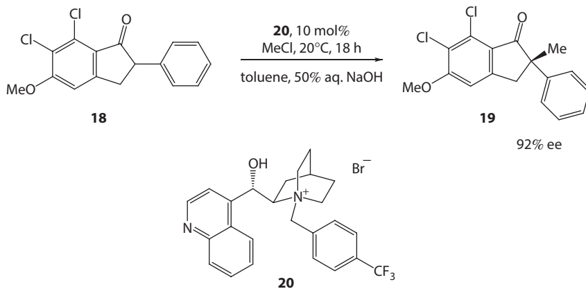
Scheme 3.17 Enantioselective phase-transfer alkylation catalyzed by 20 .
