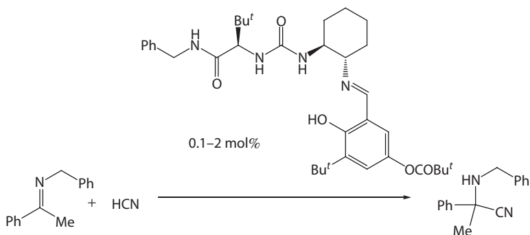
Scheme 3.18 Strecker reaction catalyzed by urea-based catalyst 1 .
