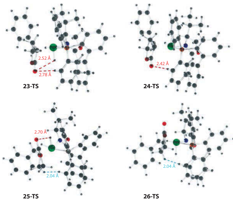
Figure 1.32 Optimized structures of the migratory insertion transition states in the asymmetric hydrogenation of exocyclic \alpha,\beta -unsaturated carbonyl compounds with an Ir/BiphPhox catalyst. The 3D structures of these transition states are available on CD.
