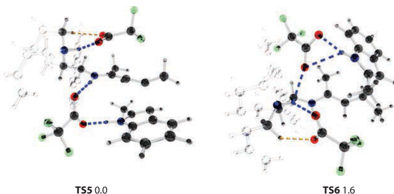
Figure 3.9 Optimized transition-state structures for the addition of indole 4 to the iminium ion assembly 7 . Relative free energies ( \Delta\Delta G^{318} ) given in kcal/mol; M06-2X/6-311++G(d,p)/SMD//M06-2X/6-31G(d). (Adapted with permission from Moran, A. et al., J. Am. Chem. Soc. , 135, 9091–9098. Copyright 2013 American Chemical Society.)
