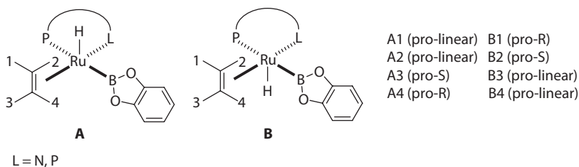
Chart 2.2 Isomers to produce different reaction products.
