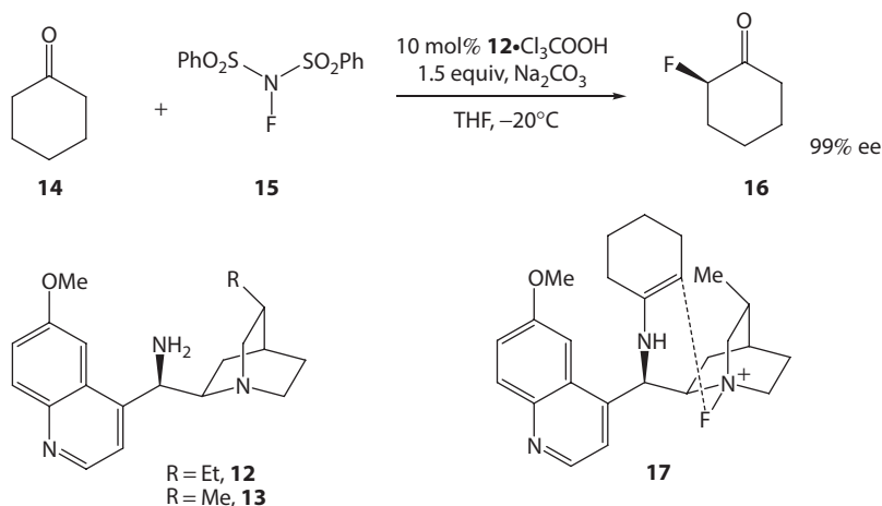
Scheme 3.16 Enantioselective monofluorination of cyclic ketones. (Data from Kwiatkowski, P. et al., J. Am. Chem. Soc. , 133, 1738–1741, 2011; Lam, Y.-h. and Houk, K. N., J. Am. Chem. Soc. , 136, 9556–9559, 2014.)
