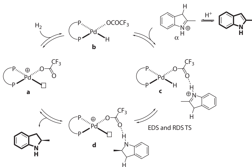
Figure 1.34 Proposed mechanism for the asymmetric hydrogenation of 2-methylindole.
