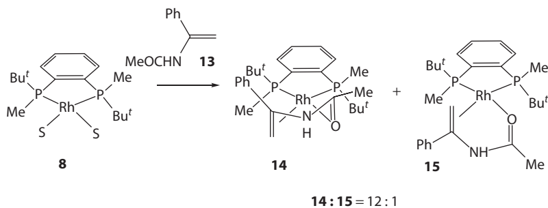
Scheme 1.4 Formation of the catalyst–substrate complexes 14 and 15 .
