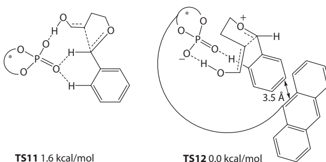
Figure 3.5 Schematic representation of the hydrogen bonding in TS11 and TS12 . (Kanomata, K. et al., Chem. Sci. , 5, 3515–3523, 2014. Adapted with permission from The Royal Society of Chemistry.)
