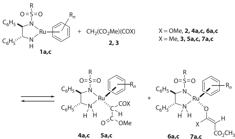
Scheme 2.1 Formation of amino complexes 4–7.
