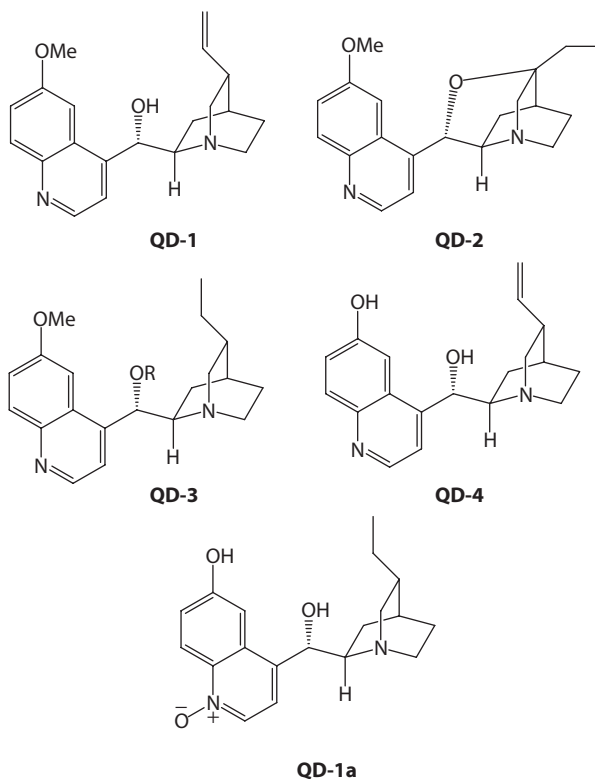
Scheme 3.9 Cinchona alkaloids used as organocatalysts.
