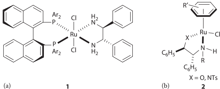
Chart 1.1 Noyori (1995) and Noyori–Ikariya (1995) catalysts.
