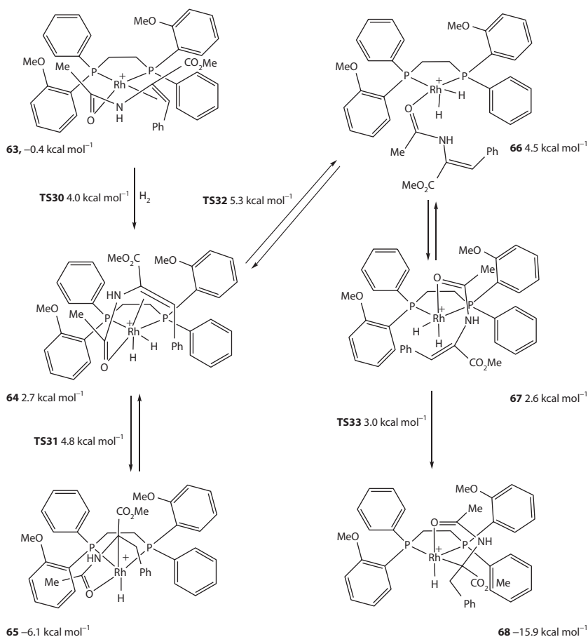
Scheme 1.19 Competition between migratory insertion-reductive elimination and double bond dissociation in the dihydride intermediate 64 . (From Gridnev, I. D. and Imamoto, T. Izv. Akad. Nauk, Ser. Khim. , 1514–1534, 2016. With permission.)
