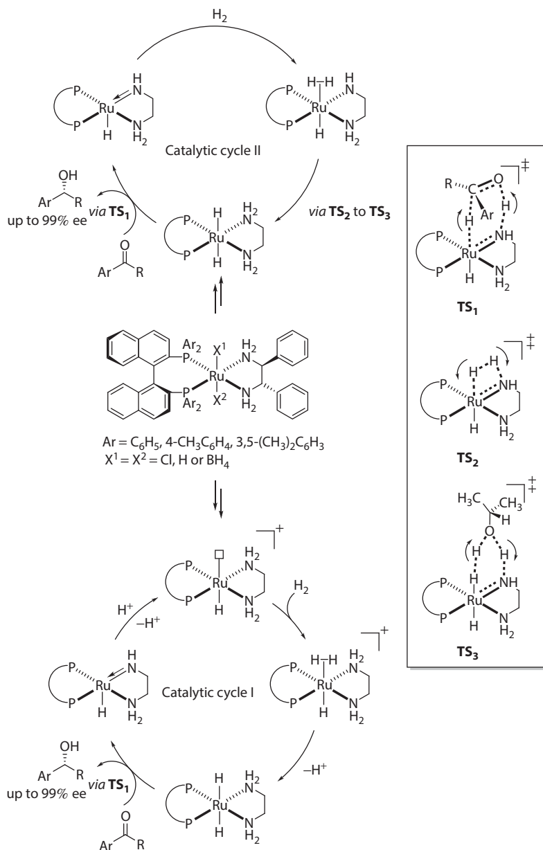
Scheme 1.41 Catalytic cycle for the hydrogenation of aromatic ketones by an active form of the Noyori (pre)catalyst 1 from early studies: catalytic cycle I (base-free conditions), catalytic cycle II (under high KO- t -C 4 H 9 concentration). Formation of the major enantiomeric product is shown. (Reprinted with permission from Dub, P. A. et al., Dalton Trans. , 45, 6756–6781. Copyright 2016 Royal Society of Chemistry.)
