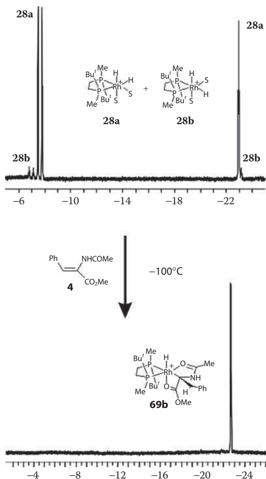
Figure 1.4 Hydride region of ^1\text{H} NMR spectra (600 MHz, \text{CD}_3\text{OD} , -95^\circ\text{C} ) of the sample initially containing solvate dihydrides 28a , b in equilibrium with the solvate complex 27 at -100^\circ\text{C} obtained by placing the sample to the probe precooled to -100^\circ\text{C} . Immediate stereoselective reaction takes place yielding the corresponding monohydride intermediate. The fact that the equatorial hydride trans to phosphorus ( \delta = -7.7 , ^2J_{\text{H-P}} = 186 Hz) was transferred in this reaction is well illustrated. (Gridnev, I. D. and Imamoto, T., Chem. Commun. , 7447–7464, 2009. Reproduced by permission of The Royal Society of Chemistry.)
