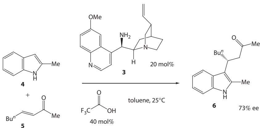
Scheme 3.12 Alkylation of indole 4 catalyzed by cinchona-based amine 3 .
