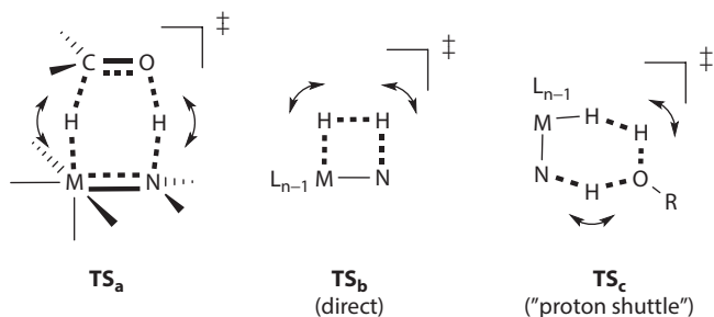
Chart 1.3 Transition states proposed by Noyori and co-workers.
