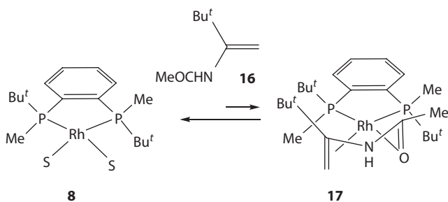
Scheme 1.5 Formation of the catalyst-substrate complex 17 .
