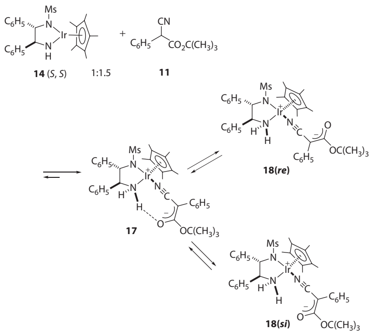
Scheme 2.4 Reaction of catalyst 14 with phenyl- \alpha -cyanoacetate 11 .
