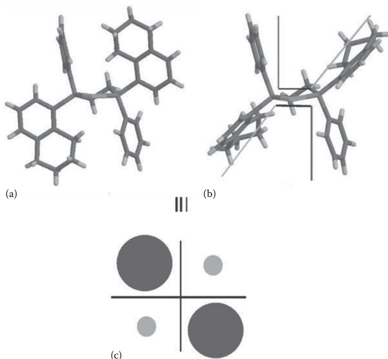
Figure 1.20 Models built with using the X-ray structure of the cyclooctadienylrhodium complex of the diphosphine 17 : (a) X-ray structure without the cod ligand; (b) structure obtained by rotation around P–C bonds of the tetrahydronaphthalenyl substituent; and (c) quadrant diagram corresponding to the upper structure—hindered quadrants are made by axial phenyls. (Reprinted with permission from Gridnev, I. D. and Imamoto, T., Acc. Chem. Res. , 37, 633–644. Copyright 2004 American Chemical Society.)
