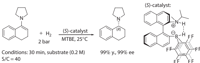
Scheme 3.31 FLP-catalyzed asymmetric hydrogenation of 1,2-dihydro-4-pyrrolidinonaphthalene.
