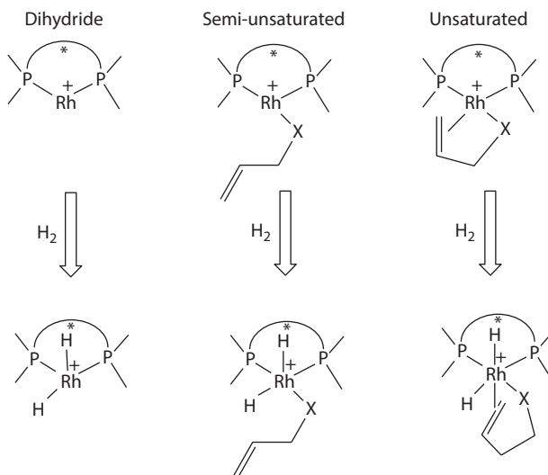
Scheme 1.7 Three possible modes of hydrogen activation in Rh-catalyzed asymmetric hydrogenation of activated olefins. For the clarity reasons here and further the coordinated molecules of solvent completing square planar for Rh(I) or octahedral for Rh(III) configuration are not shown.
