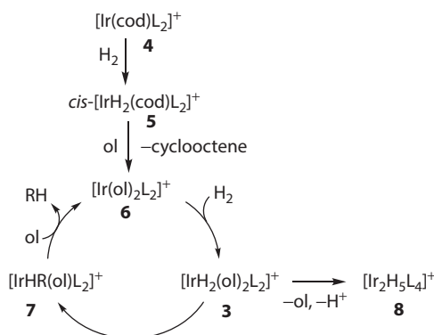
Figure 1.26 Catalytic cycle for Ir-catalyzed hydrogenation of olefins. (Data from Crabtree, R. H. et al., J. Am. Chem. Soc. , 104, 6994–7001, 1982.)
