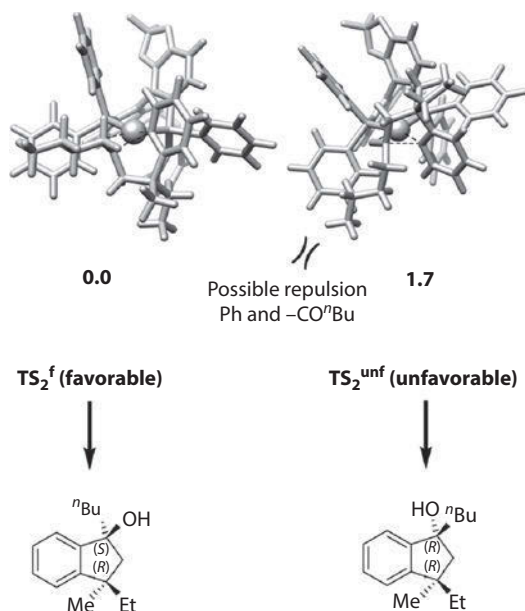
Figure 2.8 Diastereoselectivity-determining transition states. Standard free energy (gas free energy calculations corrected by single-point solvation free energy), kcal/mol.
