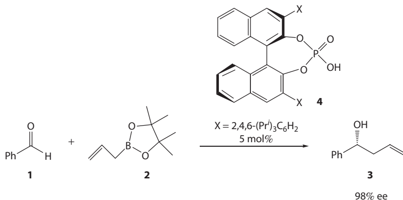
Scheme 3.1 Asymmetric catalytic allylboration. (Data from Jain, P. and Antilla, J. C., J. Am. Chem. Soc. , 132, 11884–11886, 2010.)
