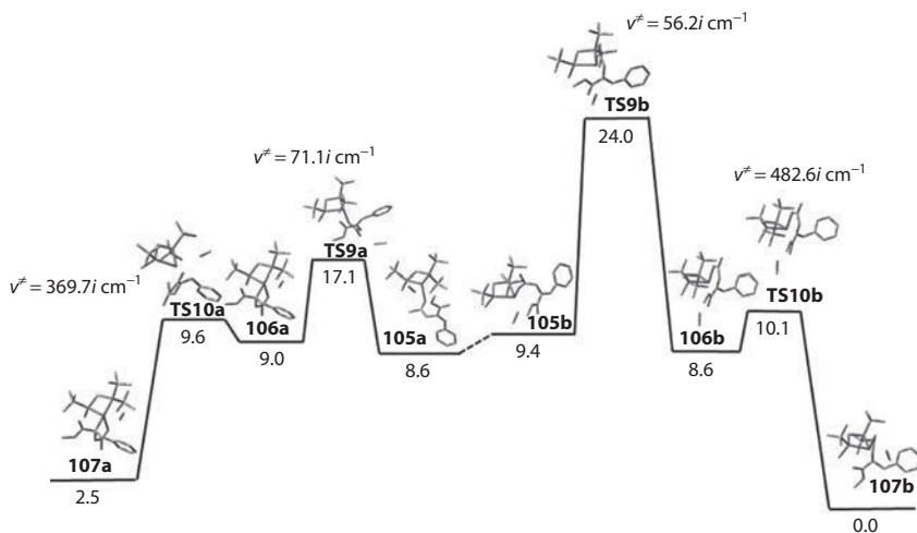
Figure 1.8 Pathways for the double bond coordination and migratory insertion steps in the nonchelating complexes 105a and 105b computed on the B3LYP/SDD level of theory. (Reprinted with permission from Gridnev, I. et al., J. Am. Chem. Soc. , 130, 2560–2572. Copyright 2008 American Chemical Society.)
