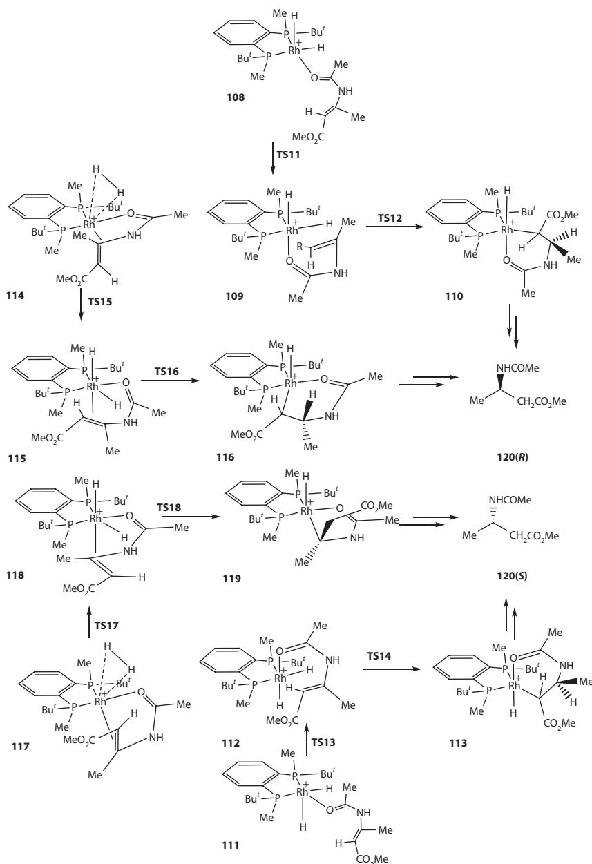
Scheme 1.32 Four computed pathways for the formation of the products 120(R) and 120(S) in hydrogenation of 26 catalyzed by Rh-BenzP* complex 8 . (Reprinted with permission from Gridnev, I. D. et al., ACS Catal. , 4, 203–219. Copyright 2014 American Chemical Society.)
