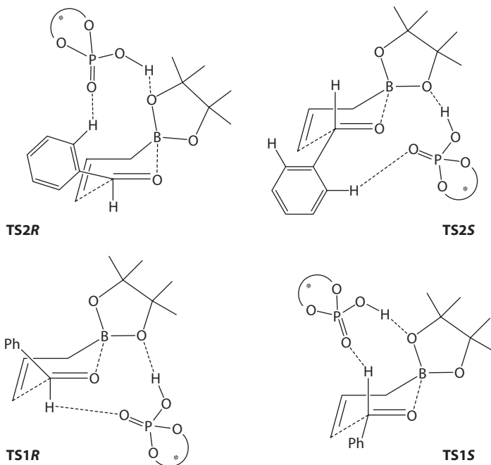
Scheme 3.2 Schematic drawings of the transition states in asymmetric catalytic allylboration.
