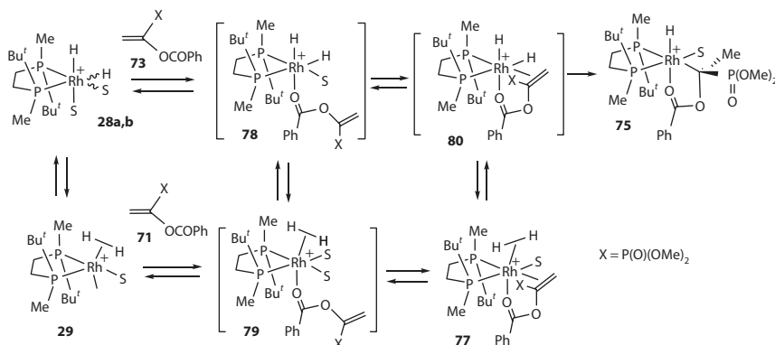
Scheme 1.23 Possible pathways leading to 75 . (From Gridnev, I. D. et al., Proc. Natl. Acad. Sci. U.S.A. , 101, 5385–5390, 2004. With permission.)
