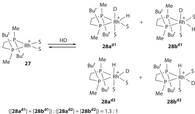
Scheme 1.11 Hydrogenation of 27 with HD. (Reprinted with permission from Gridnev, I. D. et al., J. Am. Chem. Soc. , 122, 7183–7194. Copyright 2000 American Chemical Society.)
