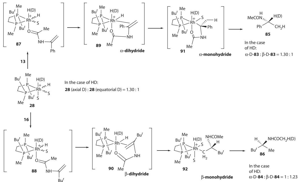
Scheme 1.26 Different reaction pathways in asymmetric hydrogenation of enamides 13 and 16 . (Reprinted with permission from Gridnev, I. D. et al., J. Am. Chem. Soc. , 123, 5268–5276. Copyright 2001 American Chemical Society.)
