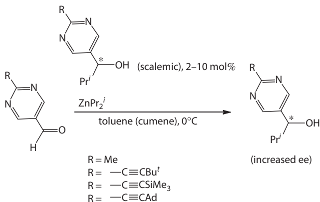
Scheme 2.15 Soai autoamplification reaction.
