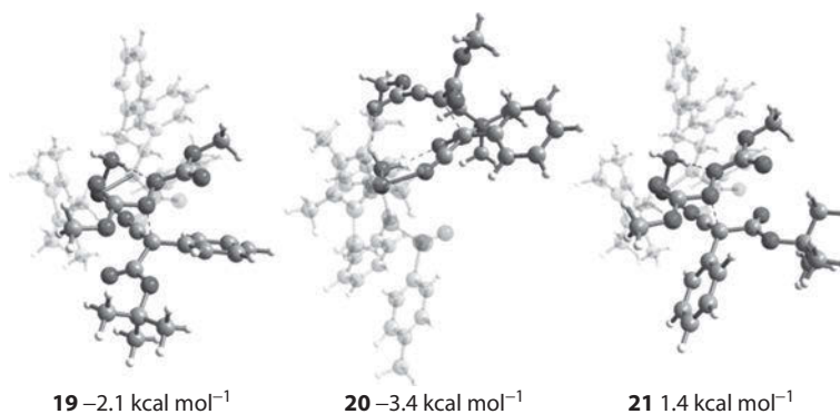
Figure 2.2 Optimized structures and relative energies of the adducts 19–21 . (Adapted with permission from Hasegawa, Y. et al., Bull. Chem. Soc. Jpn. , 85, 316–334, 2012. Copyright the Chemical Society of Japan.)
