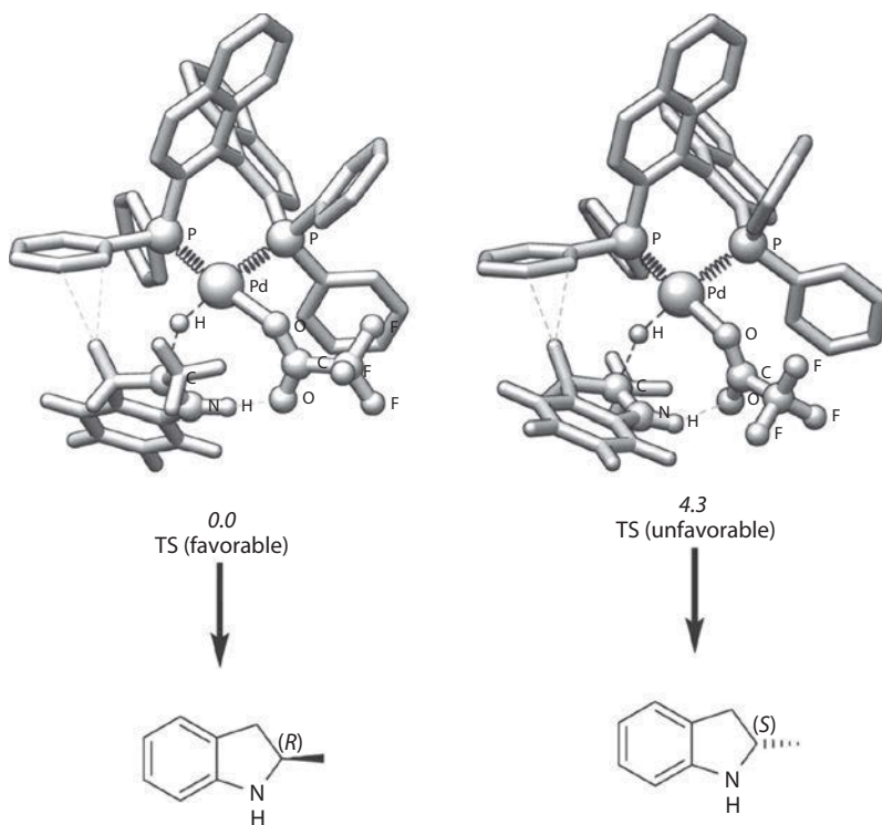
Figure 1.35 [\text{PdH}(\text{OCOCF}_3)]\text{-(R)-BINAP} ]-2-methylindole: two diastereomeric transition states leading to major ( R )-2-methylindoline and minor ( S )-2-methylindoline. \Delta G(\text{solv})_{298\text{ K}^\circ} = E(\text{SCF}) + \text{ZPE} - \text{TS}(\text{gas}) + G^{\text{solv}} , kcal/mol. Selected hydrogen atoms are omitted for clarity.
