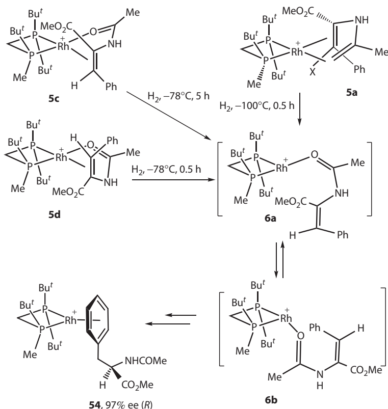
Scheme 1.15 Three low-temperature hydrogenation experiments yielding the same result. (Gridnev, I. D. and Imamoto, T., Chem. Commun. , 7447–7464, 2009. Reproduced by permission of The Royal Society of Chemistry.)
