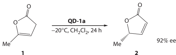
Scheme 3.10 Catalytic biomimetic isomerization of olefins. (Data from Wu, Y. et al., J. Am. Chem. Soc. , 133, 12458–12461, 2011.)
