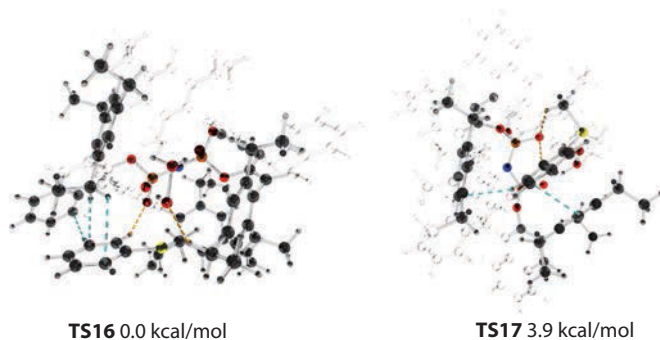
Figure 3.7 Stabilizing CH... \pi (blue) and CH...O (red) interactions found in the transition states for the sulfoxidation of thioanisole catalyzed by imidodiphosphonic acid 21 . (From Jindal, G. and Sunoj, R. B.: Axially Chiral Imidodiphosphoric Acid Catalyst for Asymmetric Sulfoxidation Reaction: Insights on Asymmetric Induction. Angew. Chem. Int. Ed. 2014. 53, 4432–4436. Copyright Wiley-VCH Verlag GmbH & Co. KGaA. Adapted with permission.)
