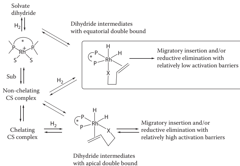
Scheme 1.40 The flux of catalysis can proceed only via the dihydride intermediates with equatorially coordinated double bond.
