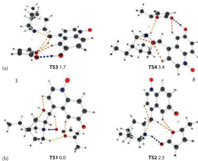
Figure 3.8 Optimized structures (M05-2x/6-31+G(d)/SMD) and relative energies (kcal/mol) of the protonation stage transition states in Scenarios I (a) and III (b). The weak noncovalent interactions important for the stereoselection are shown by orange dotted lines. (Adapted with permission from Xue, X. S. et al., J. Am. Chem. Soc. , 135, 7462–7473. Copyright 2013 American Chemical Society.)
