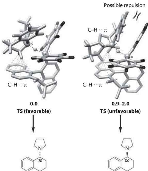
Figure 3.17 The most stable transition states leading to the (R) and (S) product enantiomers. Energy, kcal·mol -1 . Selected hydrogen atoms are omitted for clarity.
