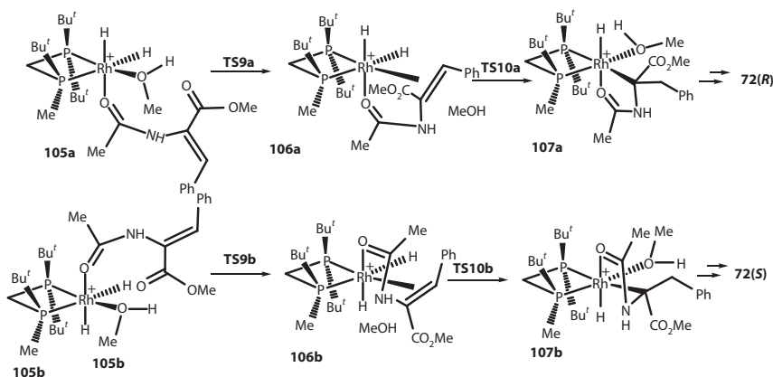
Scheme 1.31 Double bond coordination and migratory insertion steps in the nonchelating dihydride complexes 105a and 105b . (Reprinted with permission from Gridnev, I. et al., J. Am. Chem. Soc. , 130, 2560–2572. Copyright 2008 American Chemical Society.)
