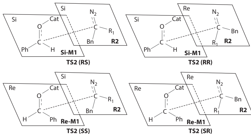
Figure 3.14 Illustration of the Stereochemistry in the C–C Bond Formation Step. (Reproduced with permission from Wang, Y. et al., J. Phys. Chem. A , 119, 8422–8431. Copyright 2015 American Chemical Society.)
