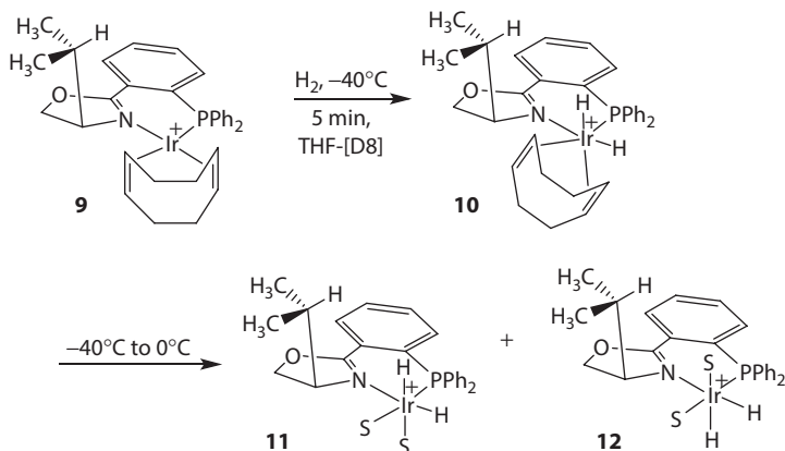
Scheme 1.49 Low-temperature hydrogenation of [\text{Ir}(\text{PhOX})(\text{cod})]^+\text{BARF}^- 9 . (From Mazet, C. et al., J. Am. Chem. Soc. , 126, 14176–14181, 2004. With permission.)
