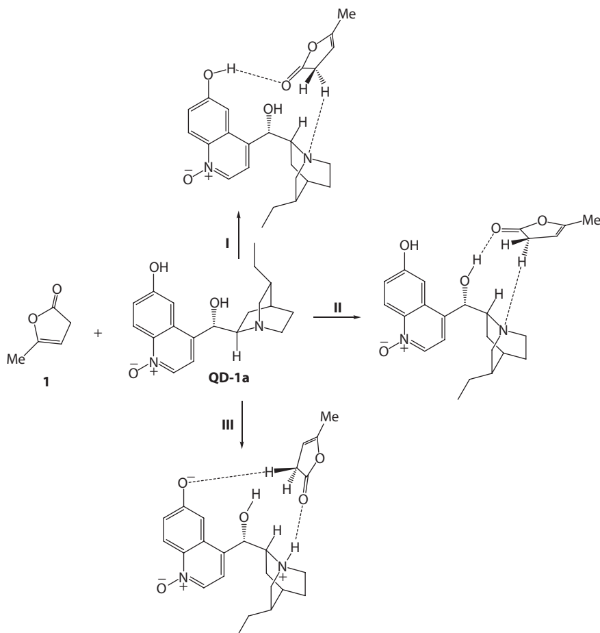
Scheme 3.11 Three routes computed for the isomerization of 1 catalyzed by cinchona alkaloid QD-1a . (Data from Xue, X. S. et al., J. Am. Chem. Soc. , 135, 7462–7473, 2013.)
