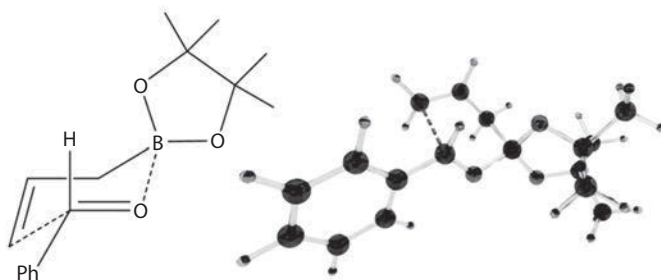
Figure 3.1 Transition state of noncatalytic allylboration. (Data from Wang, H. et al., J. Org. Chem. , 78, 1208–1215, 2013.)
