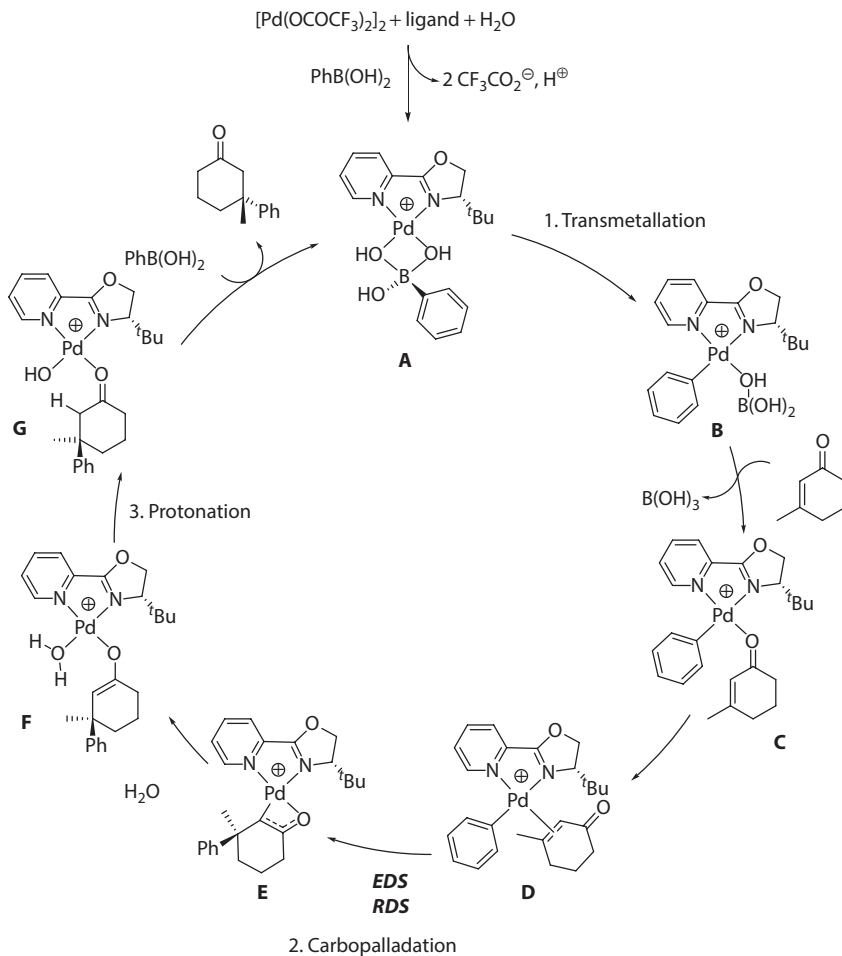
Scheme 2.11 Catalytic cycle for Pd-catalyzed conjugate addition of phenylboronic acid to 3-methyl-2-cyclohexenone.
