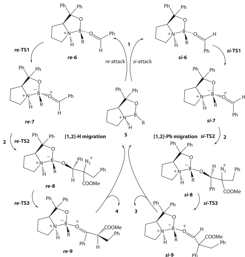
Scheme 3.30 Catalytic cycles for the [1,2]-Ph and [1,2]-H migrations. (Adapted with permission from Wang, Y. et al., J. Phys. Chem. A , 119, 8422–8431. Copyright 2015 American Chemical Society.)
