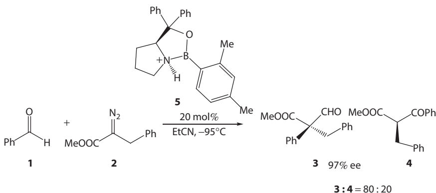
Scheme 3.29 N -Protonated chiral oxazaborolidine-catalyzed C – C ( C – H ) insertion reaction. (Data from Gao, L. et al., J. Am. Chem. Soc. , 135, 14556–14559, 2013.)
