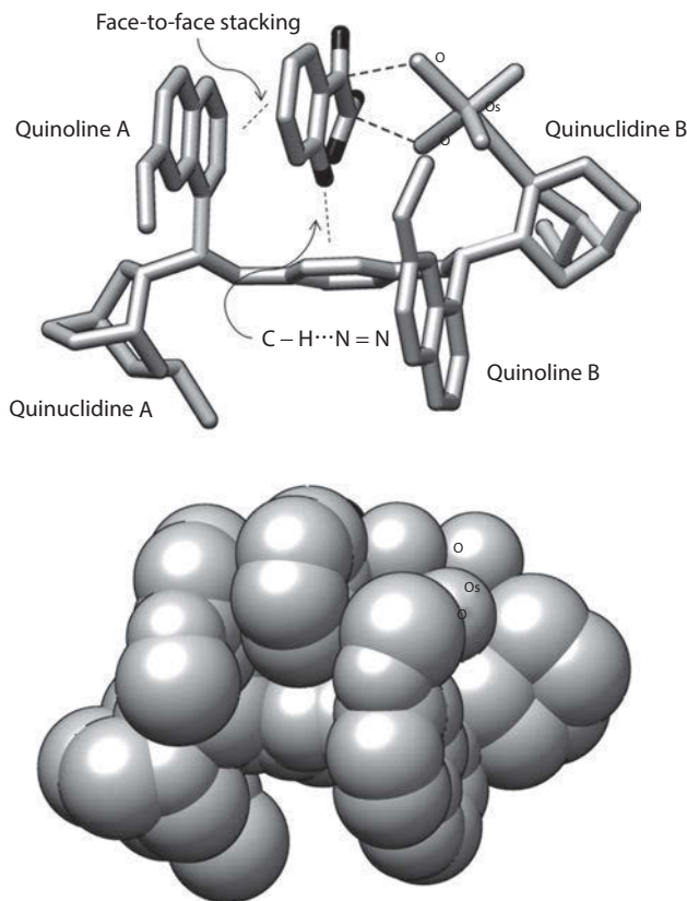
Figure 2.10 The most favorable transition state S1 leading to major ( R )-1-phenyl-1,2-ethandiol. Noncritical hydrogen atoms are omitted for clarity.
