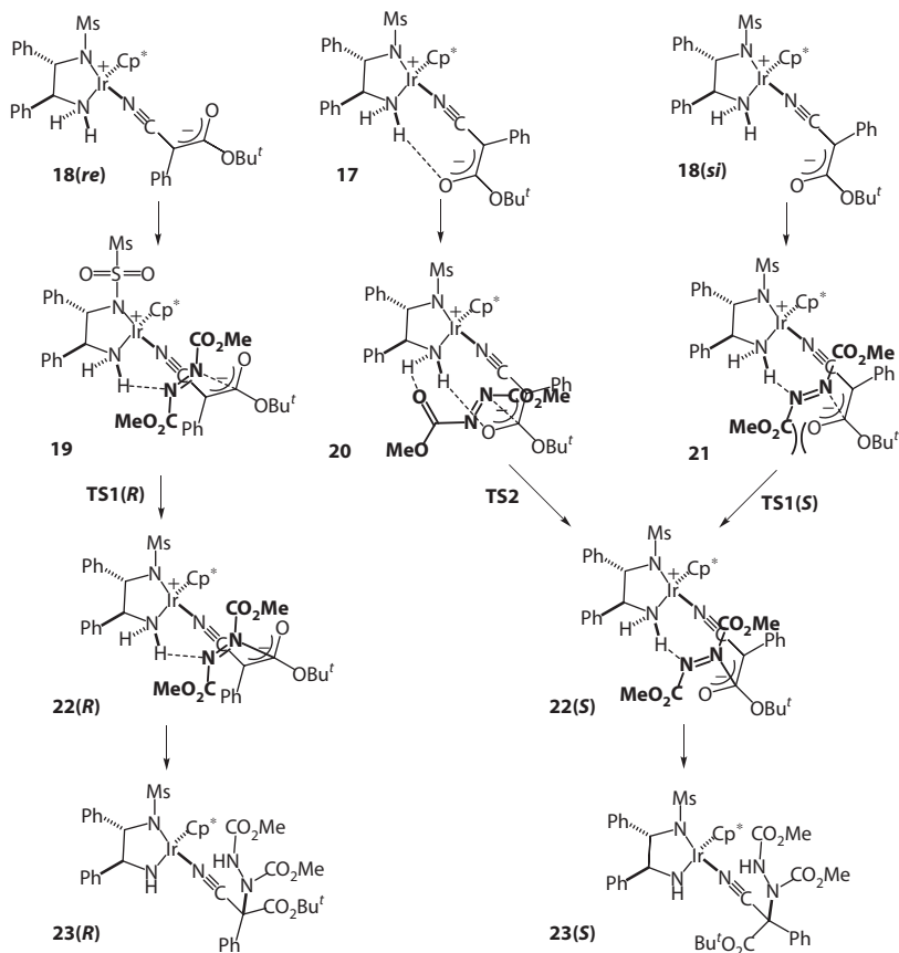
Scheme 2.5 Three competing pathways in the C—N bond forming reaction catalyzed by the Ir complex 14 . (Data from Hasegawa, Y. et al., Bull. Chem. Soc. Jpn. , 85, 316–334, 2012.)
