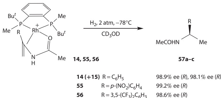
Scheme 1.16 Low-temperature hydrogenation experiments proving dissociation of the double bond after oxidative addition of H 2 .
