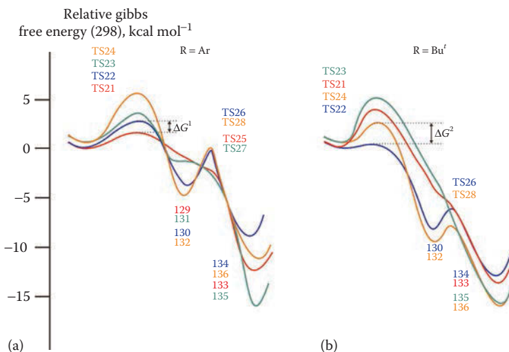
Figure 1.15 Sections of the potential energy profiles for the double bond coordination and migratory insertion steps for the aryl (a) and t -butyl (b) substituted enamides. (Reprinted with permission from Gridnev, I. D. and Imamoto, T. Izv. Akad. Nauk, Ser. Khim. , 1514–1534, 2016. With permission.)
