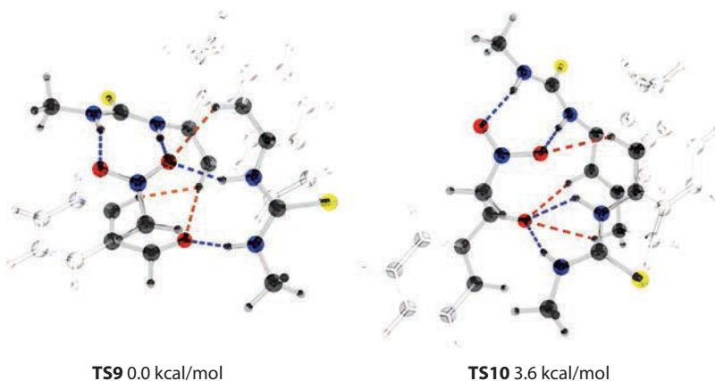
Figure 3.12 Structures of the transition states leading to the formation of R ( TS9 ) and S ( TS10 ) products of the Henry reaction. Strong conventional hydrogen bonds are shown in blue, and the weak disperse interactions in orange dotted lines. (Adapted with permission from Breugst, M. and Houk, K. N., J. Org. Chem. , 79, 6302–6309. Copyright 2014 American Chemical Society.)
