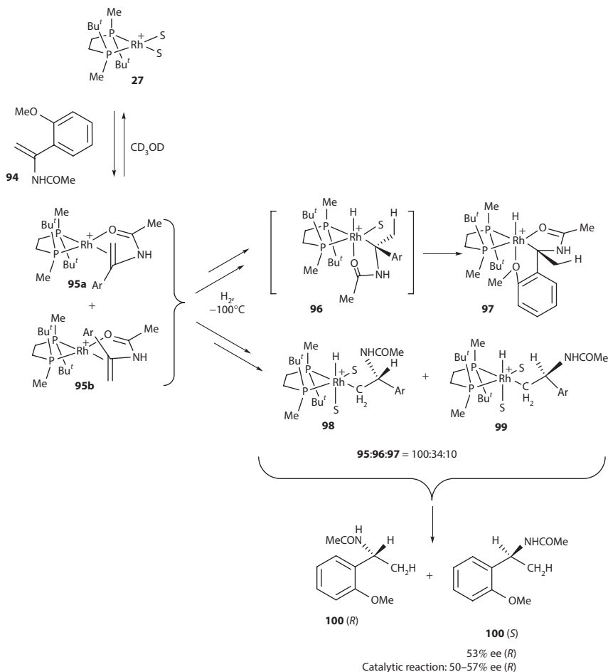
Scheme 1.27 Competition of the reaction pathways in the asymmetric hydrogenation of enamide 94 . (Reprinted with permission from Gridnev, I. D. et al., J. Am. Chem. Soc. , 123, 5268–5276. Copyright 2001 American Chemical Society.)
