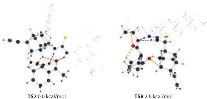
Figure 3.11 Diastereomeric transition states for the direct protonation of the enolate carbon. (Adapted with permission from Sengupta, A. and Sunoj, R. B., J. Org. Chem. , 77, 10525–10536. Copyright 2012 American Chemical Society.)
