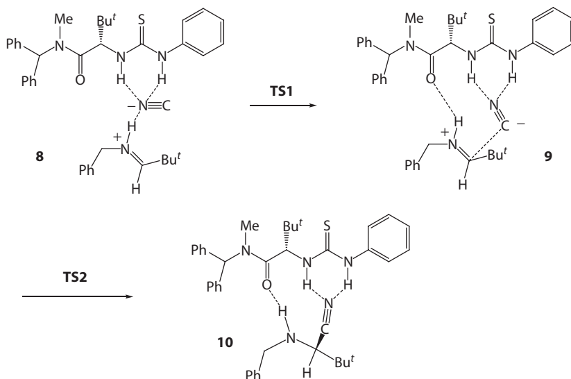
Scheme 3.21 Enantioselective steps in hydrocyanation reaction catalyzed by the model thiourea catalyst 7 . (Data from Zuend, S. J. and Jacobsen, E. N., J. Am. Chem. Soc. , 129, 15872–15883, 2007.)
