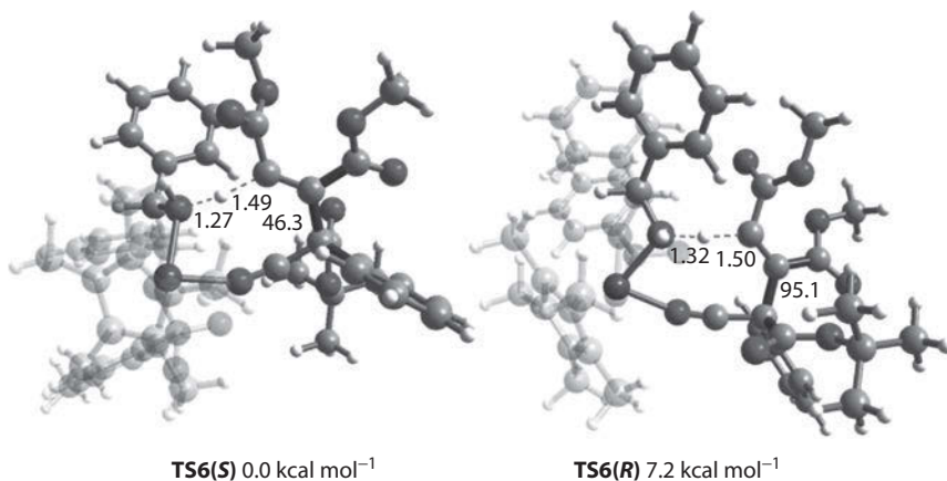
Figure 2.5 Transition states for the stereoselective proton transfer. (Adapted with permission from Hasegawa, Y. et al., Bull. Chem. Soc. Jpn. , 85, 316–334, 2012. Copyright the Chemical Society of Japan.)
