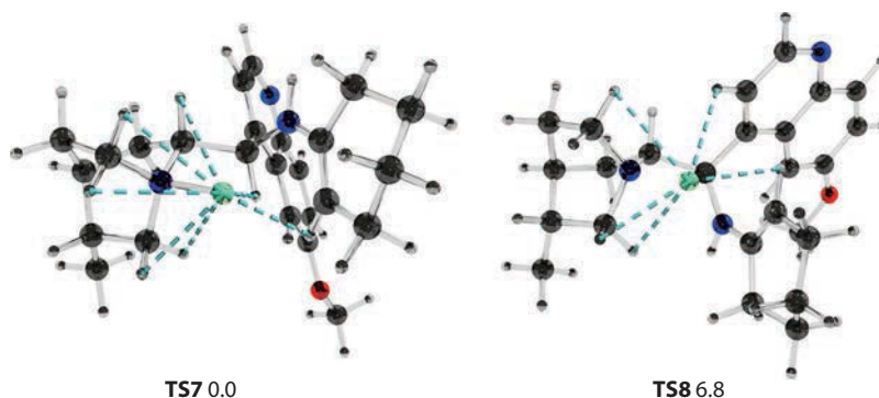
Figure 3.10 Optimized structures of TS7 and TS8 (B3LYP-D3(BJ)/def2-TZVPP-IEFPCM (THF)//B3LYP/6-31G(d)-IEF-PCM (THF)). (Data from Lam, Y.-H. and Houk, K. N., J. Am. Chem. Soc. , 136, 9556–9559, 2014.)
