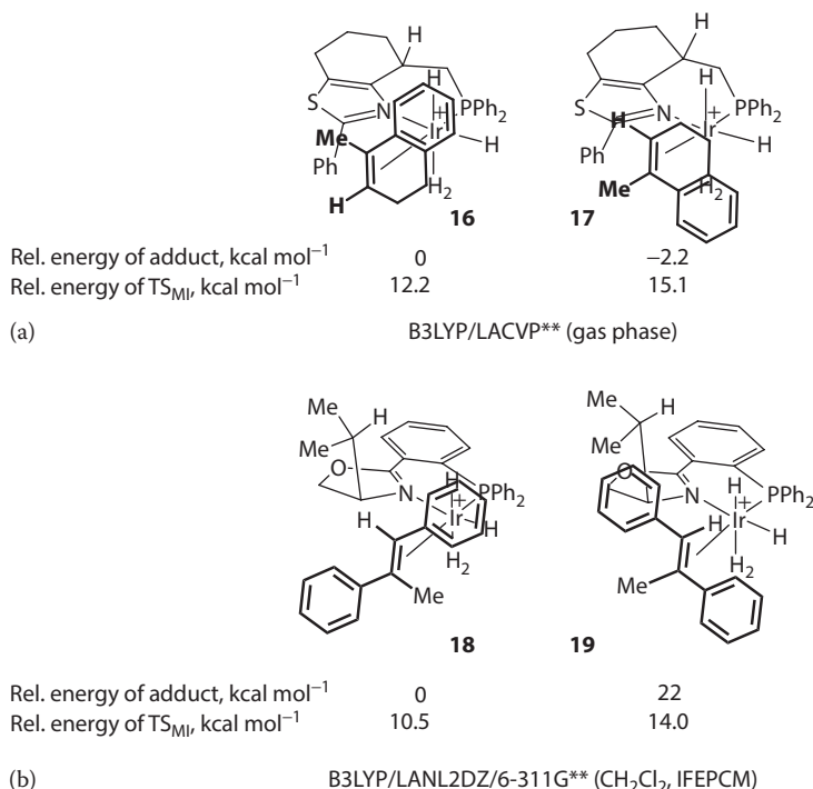
Figure 1.28 Structures of the [Ir(H) 2 (olefin)(H 2 )] + complexes and relative energies for them and corresponding transition states of migratory insertion computed in (a) 390 and (b). 391 The 3D structures of these transition states are available on the CD.
