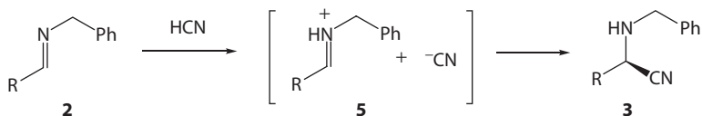
Scheme 3.20 Formation of iminium ion intermediate 5 . (Data from Zuend, S. J. and Jacobsen, E. N., J. Am. Chem. Soc. , 129, 15872–15883, 2007.)
