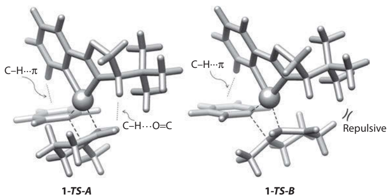
Figure 2.11 The most favorable transition states leading to major ( R )- and minor ( S )-product. Optimized at BP86/SDD(Pd)/6-31G*(all others) level of theory.
