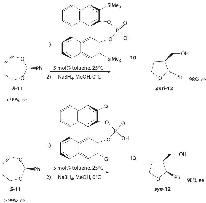
Scheme 3.5 Stereoselective Petasis–Ferrier-type rearrangement catalyzed by chiral phosphoric acids. (Data from Kanomata, K. et al., Chem. Sci. , 5, 3515–3523, 2014.)
