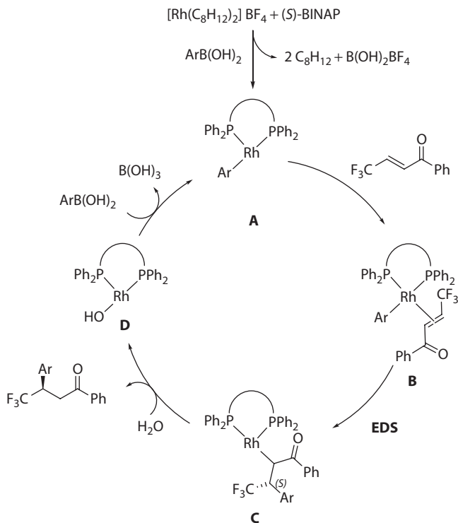
Scheme 2.12 Catalytic cycle for Rh-catalyzed conjugate addition of arylboronic acid to the acyclic enone.
