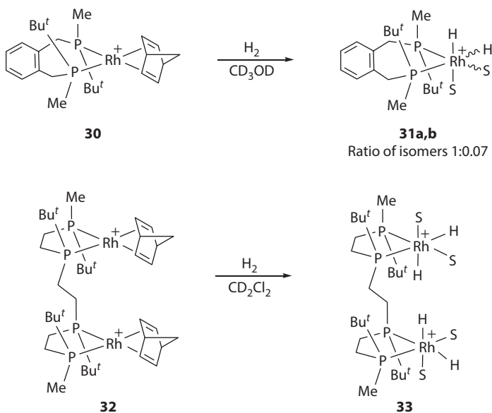
Scheme 1.12 Irreversible formation of solvate dihydrides. (Gridnev, I. D. and Imamoto, T., Chem. Commun. , 7447–7464, 2009. Reproduced by permission of The Royal Society of Chemistry.)
