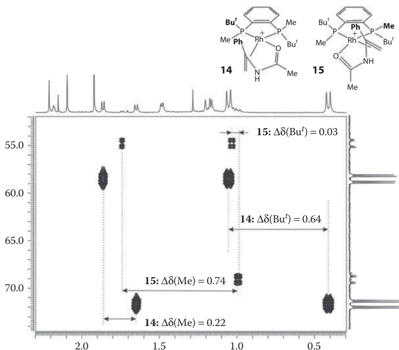
Figure 1.3 ^1\text{H} - ^{31}\text{P} HMBC NMR spectrum (600 MHz, \text{CD}_3\text{OD} , -60^\circ\text{C} ) of the equilibrium mixture of catalyst-substrate complexes 14 and 15 (section plot). Shielding of one of the t -butyl groups in 14 and one of the methyl groups in 15 defines the mode of the double bond coordination in both complexes, whereas the relative stabilities of these complexes suggest that a C-H... \pi interaction is the main stereoregulating factor. (Reprinted with permission from Gridnev, I. D. and Imamoto, T. ACS Catal. , 5, 2911–2915. Copyright 2015 American Chemical Society.)
