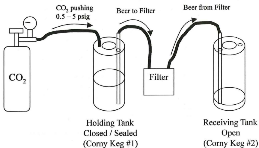
Figure 2: Typical Homebrew Filtration Setup
