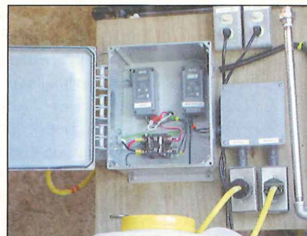
Steve added two electric temperature control elements for accurate and precise heating of his liquor tank and kettle.
