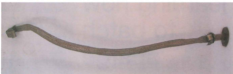
A stainless steel braid (picture at right) separates the wort from the grains. It is made from a water supply line. A valve on the outside of the cooler (above) regulates the outflow of wort.
