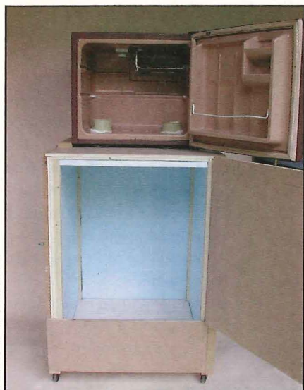
The DraftErator is an insulated box cooled by a dorm fridge. It will keep four Cornelius kegs at serving temperature.
