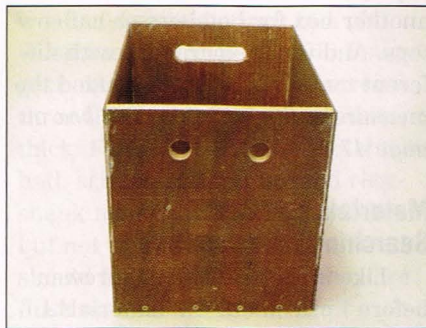
To add handles for easier transport: Just start with two drilled holes, then connect the dots with a saber saw.
