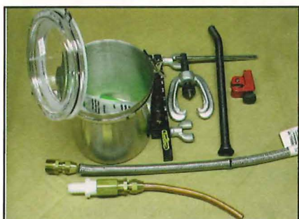
The parts: fittings, a tubing cutter, tubing bender, flare tools and hose.
