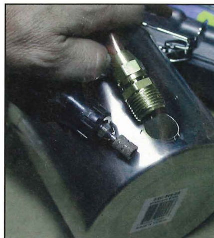
Drill a starter hole and then enlarge it progressively until it fits.
