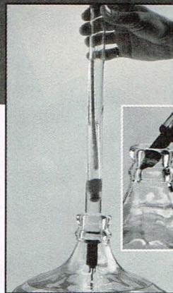
The Thief Easy hydrometer readings. Touch tip to return sample.
