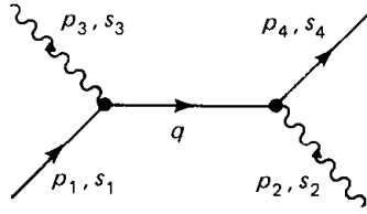
Figure 7.6 Compton scattering.
