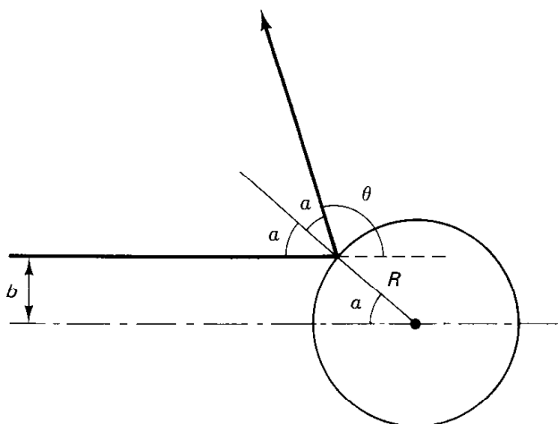
Figure 6.2 Hard-sphere scattering.
