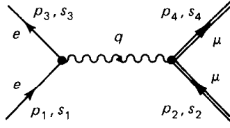
Figure 7.2 Electron-muon scattering.
