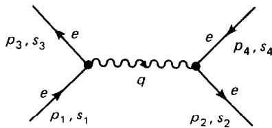
Figure 7.4 Electron-positron scattering.
