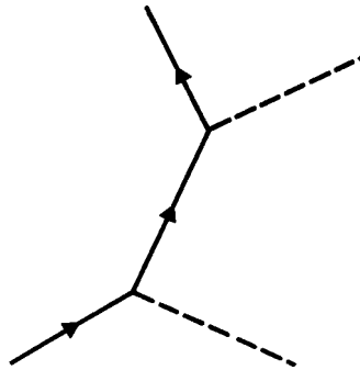
electron-photon scattering
