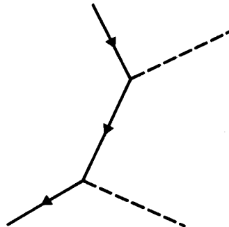
positron-photon scattering
