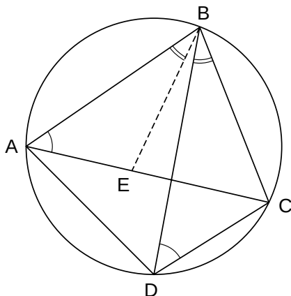
FIG. 35. Ptolemy's Theorem.
