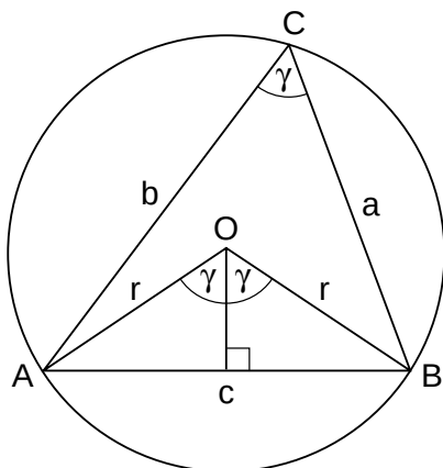
FIG. 31. The Law of Sines: the acute case.
