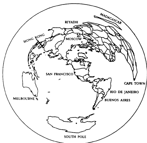
FIG. 67. Azimuthal equidistant world map centered at San Francisco.
