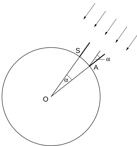
FIG. 23. Eratosthenes’s measurement of the earth’s circumference.
