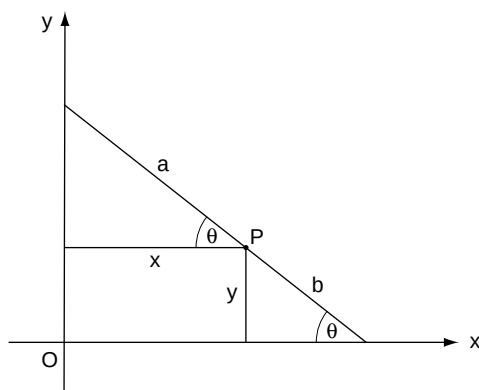
FIG. 49. As \theta varies, P describes an arc of an ellipse.
