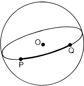
FIG. 66. Arc of a great circle.
