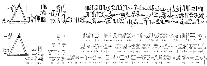
FIG. 1. Problem 56 of the Rhind Papyrus.
