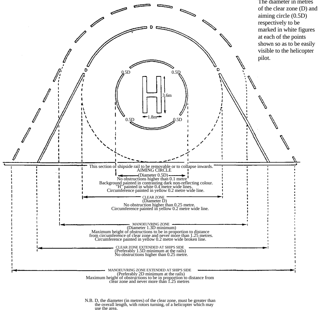
Figure 1: Landing area at the ship's side
