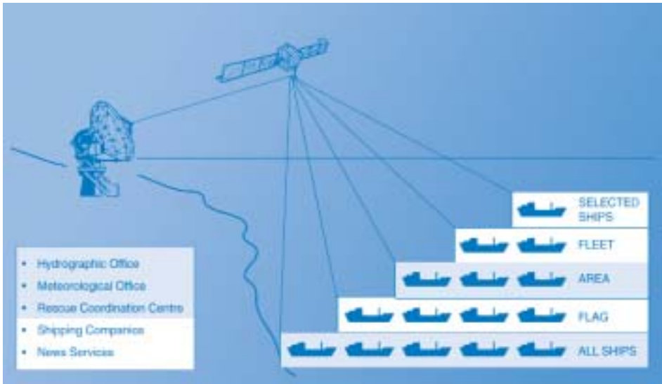
Basic concept of the Inmarsat Enhanced Group Calling System (the shaded area indicates functions of the SafetyNet™ Service)
