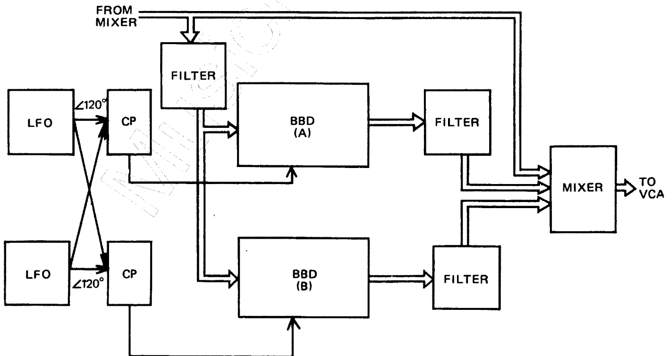
ENSEMBLE BLOCK DIAGRAM
