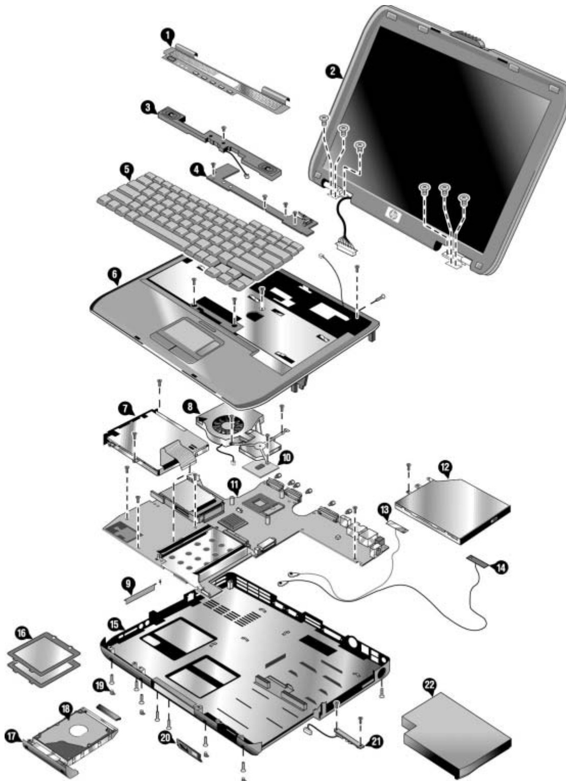
Figure 4-1 Exploded View
