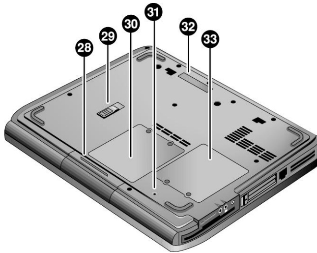
Figure 1-3. Bottom View
