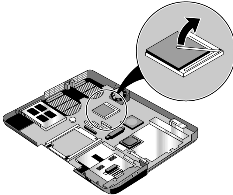
Figure 2-29. Removing the CPU Module
