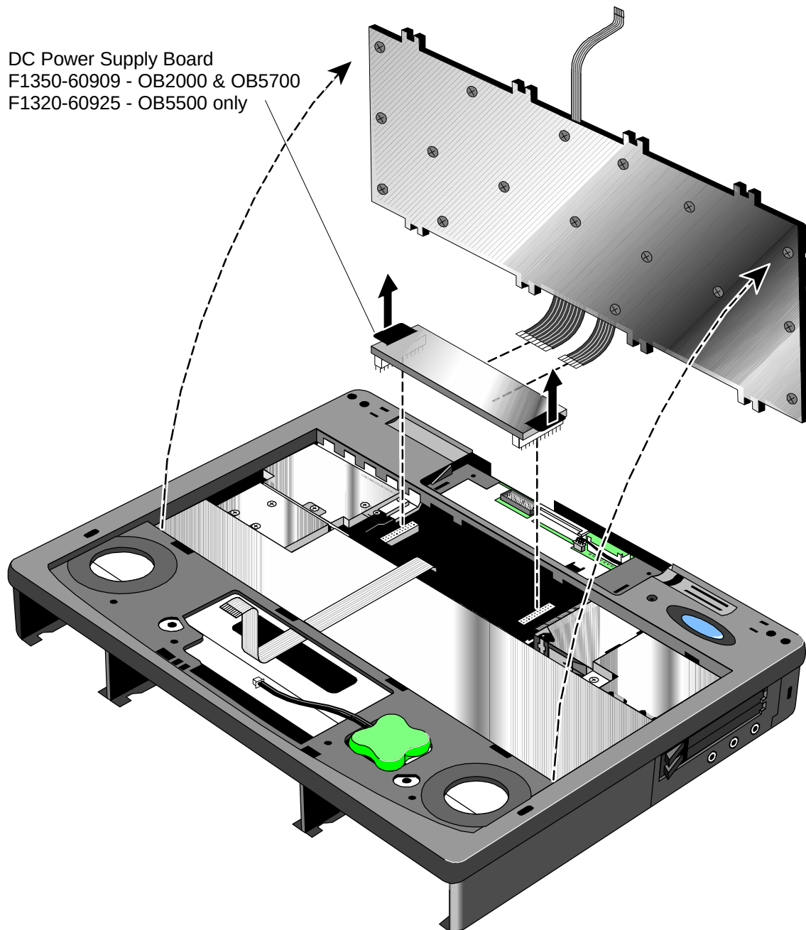
Figure 34 - Keyboard Removal
