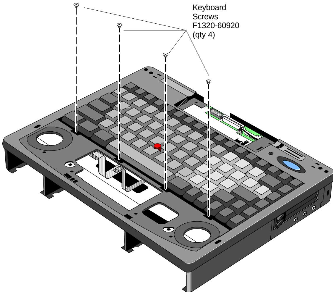
Figure 33 - Keyboard Screws
