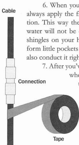
Drawing 1: The proper way to put the final wrap on vertically running coax joint.
