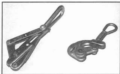
Photo 2: Klein Chicago cable grip on left and Klein Haven's grip on right.
