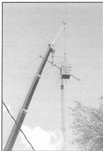
Photo 5: This is how the damaged antenna was removed. It's still a handful.
