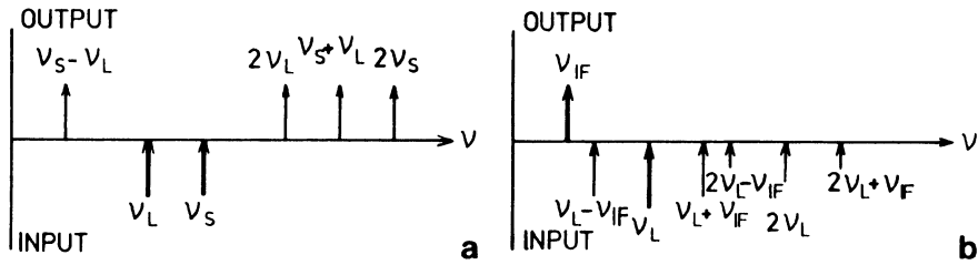
Fig. 5.4 Input and output frequencies of a mixer. The thick arrows are the given values. There are two methods to specify the system: (a) when two input frequencies, \nu_{LO} and \nu_s are given. In case (b) when \nu_{LO} and \nu_{IF} are specified. In this case, signals from both the upper sideband ( \nu_{LO} + \nu_{IF} ) and lower sideband ( \nu_{LO} - \nu_{IF} ) contribute to the IF signal
