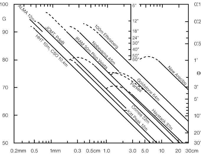
Fig. 7.8 The gain G in dB ( left axis ) of some high-precision filled aperture radio telescopes is plotted against wavelength \lambda . The Full Width to Half Power, \theta is plotted on the right axis . The ALMA 12 m antennas will have the same properties as the APEX antenna. The curve for these antennas extends to 0.3 mm, and to longer wavelengths, where it joins the curve for the Kitt Peak 12 m antenna which has a lower surface accuracy. The 15 m diameter JCMT (James Clerk Maxwell Telescope) on Mauna Kea and PdeB (IRAM Plateau de Bure interferometer) antennas are also shown. Smaller but highly accurate antennas are a part of the SOFIA and Herschel observatories
