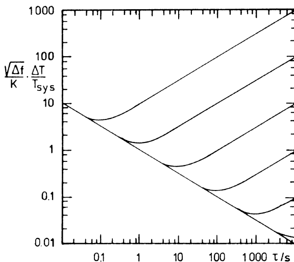
Fig. 4.9 The time dependence of the relative receiver uncertainty, \Delta T_{\text{RMS}}/T_{\text{sys}} normalized to unit bandwidth \Delta \nu . K is a factor accounting for data taking procedures (Table 4.3). For a total power system, ( K = 1 ). The different one-parameter curves are characterized by the value \tau_m in (4.49). The turn off in each curve gives the integration time leading to the smallest value for \Delta T_{\text{RMS}}/T_{\text{sys}}
