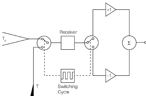
Fig. 4.8 A balanced receiver employing Dicke switching between a load at the temperature T_{\text{ref}} , and the sky at T_A . The box joined by dotted lines connecting the two switches indicates a square wave switching cycle. This is alternately multiplied by +1 or -1 , so that the response from the reference is subtracted from sky synchronously in the adding section on the far right
