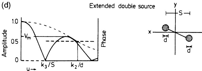
Fig. 9.4 The visibility function for various brightness distribution models. The solid lines are amplitudes, the dashed lines are phases. (a) A point source displaced from the phase center; a displacement of x_0 = 1'' shifts phase by one fringe for a k_1 = 206265 wavelength baseline. (b) A displaced Gaussian shaped extended source of FWHP 1'' ; the amplitude reaches a value of 0.5 at k_2 = 91000 wavelengths. (c) Two point sources with an intensity ratio R ; the period of amplitude and phase depends on the separation. If the centroid of the double is the phase center, the sign of phase gives the direction of the more intense components, with positive to the east. (d) Two extended double sources; this has been obtained from the response to a pair of point sources by multiplying the visibility amplitude by the envelope shown in (b). The numerical values are k_3 = 103000 if s = 1'' and k_2 = 91000 if d = 1'' [after Fomalont and Wright (1974)]
