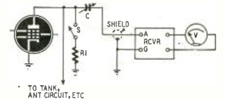
Fig. 3—Circuit showing tuning method.
