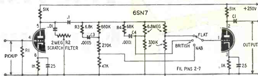
Fig. 3—Selective equalizer for amplitude-actuated pickups has rolloff switch.
