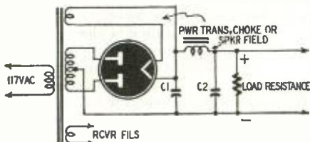
Fig. 1—A basic full-wave power supply.
