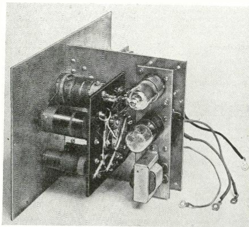
Instead of a standard chassis, author fastened metal strips to rear of panel.
