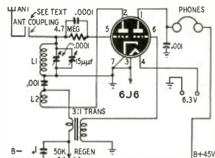
Fig. 2—Simple receiver you can build.
