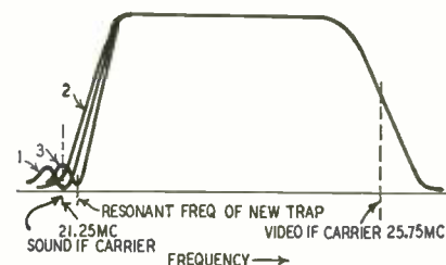
Fig. 3—Standard-receiver i.f. response (1) and two for intercarrier (2 and 3).
