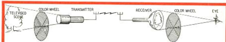
Fig. 1—CBS system uses a color wheel at the transmitter and one at the receiver.
