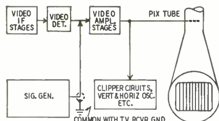
Fig. 4—Tie generator to a video grid.
