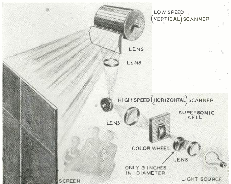
Fig. 11—Skiatron Corp. proposes adaptation of CBS color wheel to its projector.
