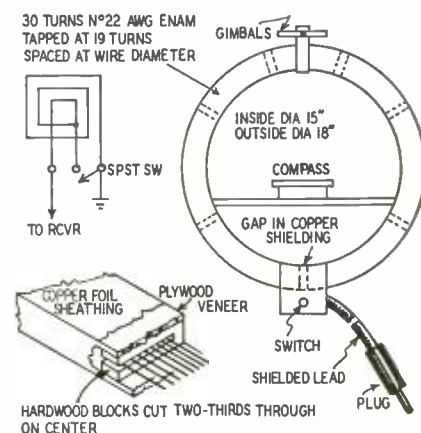
Fig. 3—The loop may be built as shown here or a surplus unit purchased.
