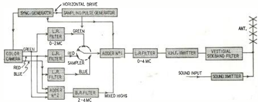
Fig. 2—Block diagram shows how the RCA system operates at the transmitter end.
