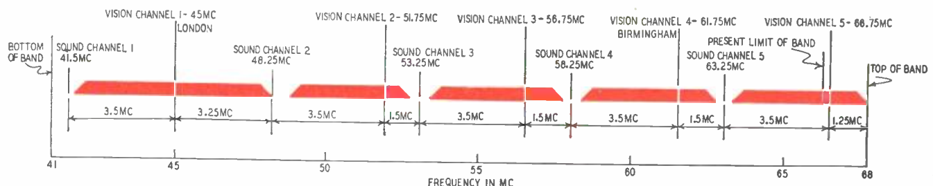
TV channel assignments in Britain. All except No. 1 have asymmetric sidebands. Channels 1 and 4 are those now employed. JANUARY, 1950
