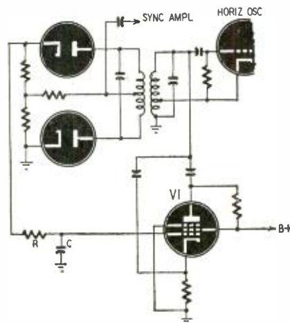
Fig. 7—A horizontal sweep with a.f.c.
