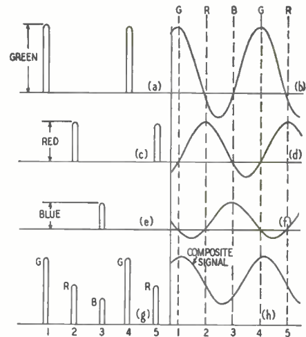
Fig. 3—The sampling system takes pulses of each color, integrating them.
