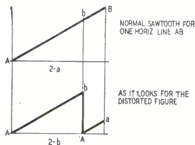
Fig. 2—Horizontal sweep is too fast.
