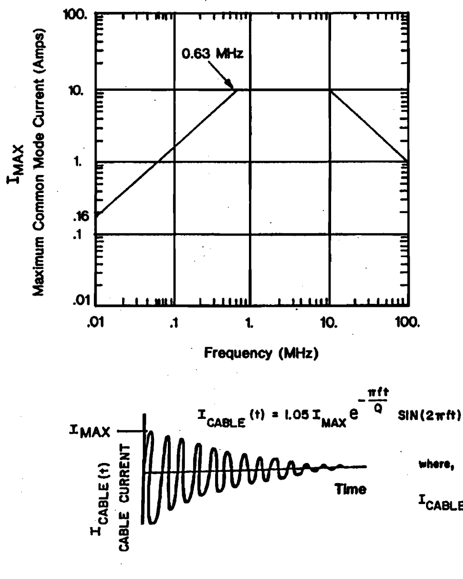
FIGURE 6-12. LIMIT FOR CS11
