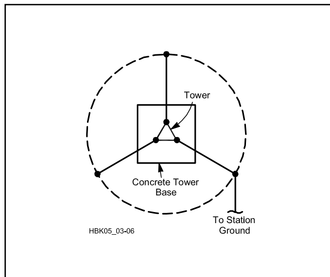
Figure 26.25 — Schematic of a properly grounded tower. A bonding conductor connects each tower leg to a ground rod and a buried (1 foot deep) bare, tinned copper ring (dashed line), which is also connected to the station ground and then to the ac safety ground. Locate ground rods on the ring, as close as possible to their respective tower legs. All connectors should be compatible with the tower and conductor materials to prevent corrosion. See text for conductor sizes and details of lightning and voltage transient protection.
