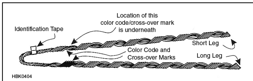
Figure 26.37 — Preformed guy wire “dead end” grip. The grip is wound around the guy wire and holds the load through friction.
