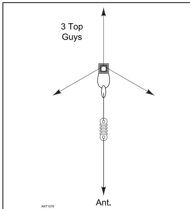
Figure 26.10 — For a mast supporting a wire antenna, the guys should be equally spaced at 120^\circ around the mast with one guy directly in line with the antenna.
