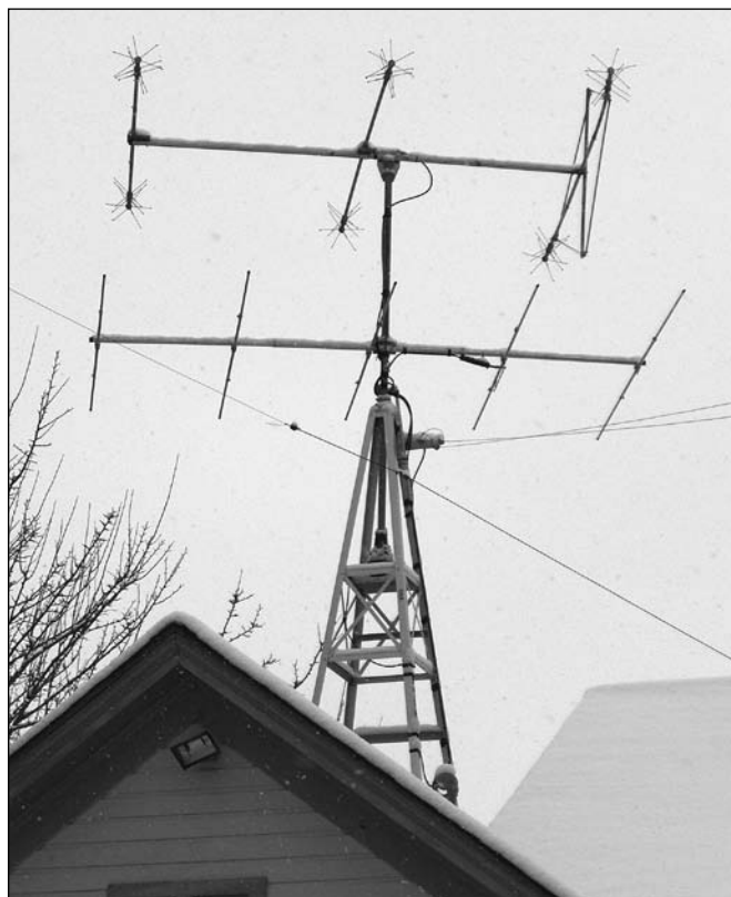
Figure 26.14 — A roof mounted tower will give your antenna a chance to get up in the air with a minimal impact and cost. (Photo by Redd Swindells, AI2N)
