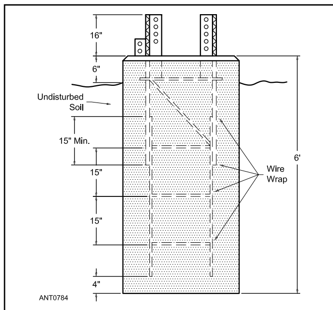
Figure 26.23 — Another example of a concrete base for a 70-foot lattice crank-up tower.
