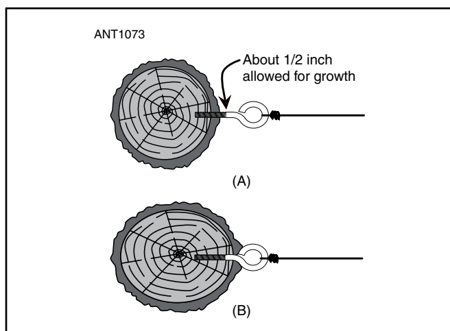
Figure 26.5 — The best way to secure a wire to a tree is with an eye-screw threaded into the wood (A). As the tree grows and expands, however, the eye-screw will become embedded (B) and must be removed and replaced.
