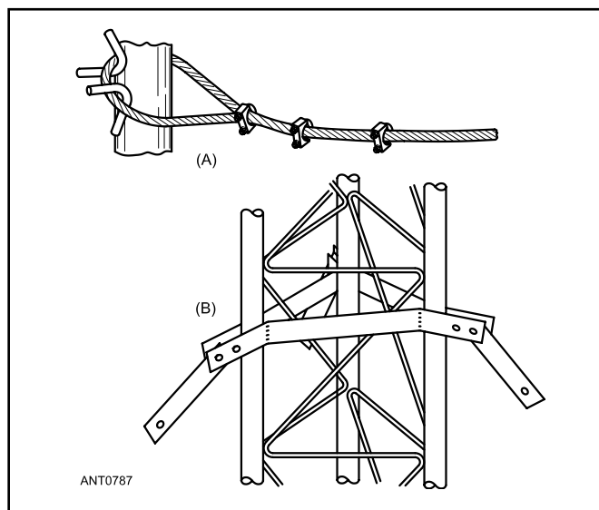
Figure 26.38 — Two methods of attaching guy wires to tower. See text for discussion.
