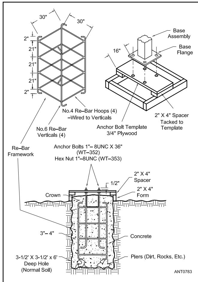
Figure 26.22 — Plans for installing concrete base for a 70-foot tubular crank-up tower. Although the instructions vary from tower to tower, this is representative of the type of concrete base specified by most manufacturers.
