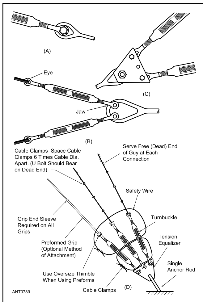
Figure 26.39 — Variety of means available for attaching guy wires and turnbuckles to anchors.
