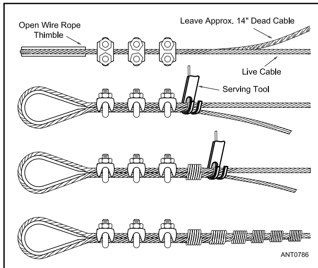
Figure 26.35 — Traditional method for securing the end of a guy wire. This technique is becoming increasingly uncommon as Preforms replace cable clamps.
