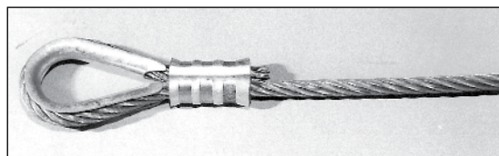
Figure 26.36 — Swaged guy wire end using Nicopress fitting.
