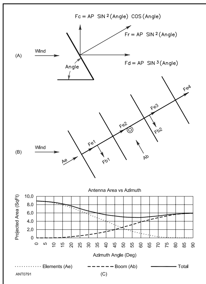
Figure 26.49 — Description of how loads are developed on a Yagi. At A, F_r is the resultant force from the wind load on a generalized member. F_d is the load acting downwind (drag) that creates the load on the tower. F_c is the lateral component of the wind load. The term A is the flat projected area (FPA), which is the broadside area normal to the wind. The term P is the wind pressure. At B, A_e is the total element area, while A_b is the total boom area. All the loads due to the wind act normal to the antenna sections—the force on element #1 ( F_{e1} ) acts along the axis of the boom, for example. At C, a plot of the effective FPA as a function of the azimuthal wind direction for a Yagi, ignoring drag coefficients. The Yagi in this example has 9.0 square feet of element FPA and 6.0 square feet of boom FPA. The worst-case FPAs occur with the beam pointed in the wind and with the boom broadside to the wind. To determine the actual tower loading, the actual drag coefficients and wind pressures must be used.
