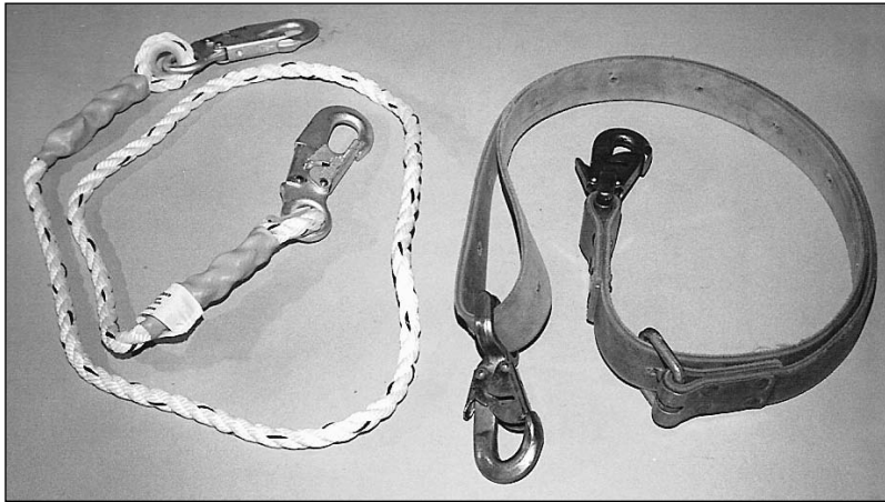
Figure 26.2 — A fixed-length rope positioning lanyard on the left and a versatile Klein adjustable lanyard on the right. They both use double-locking snap-hooks.
