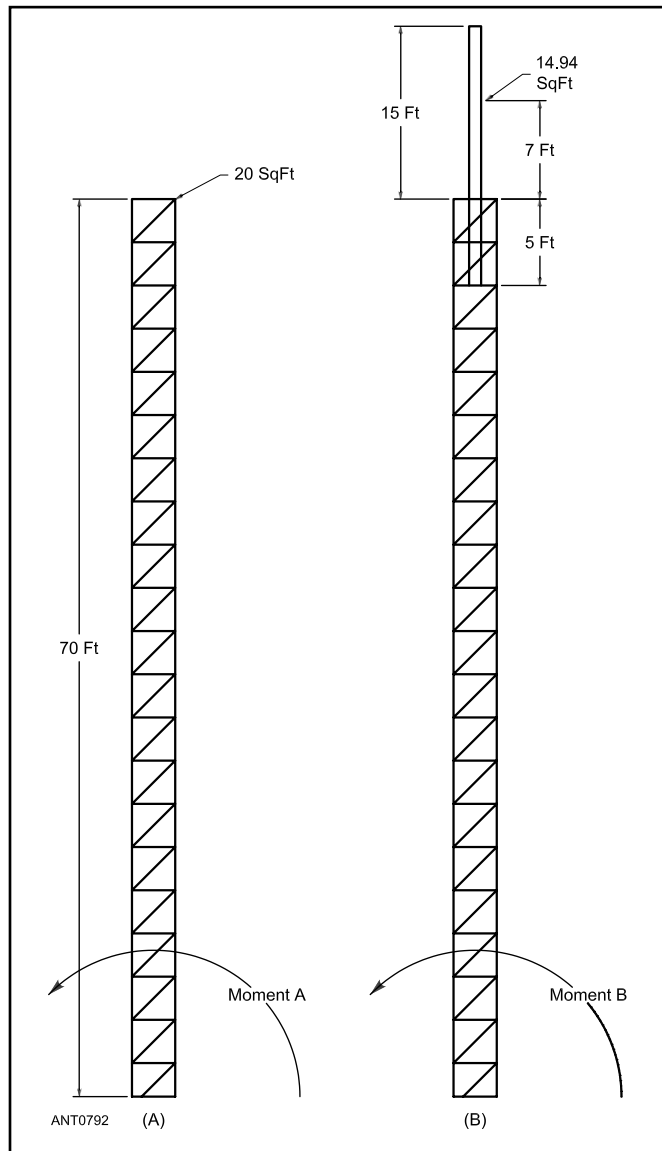
Figure 26.50 — At A, a 70-foot tower rated for 20 square feet of antenna load at the top. At B, the same tower with a 2-inch OD, 20-foot long mast, with an antenna mounted 7 feet above the top of the tower. Both configurations produce the same tower load.
