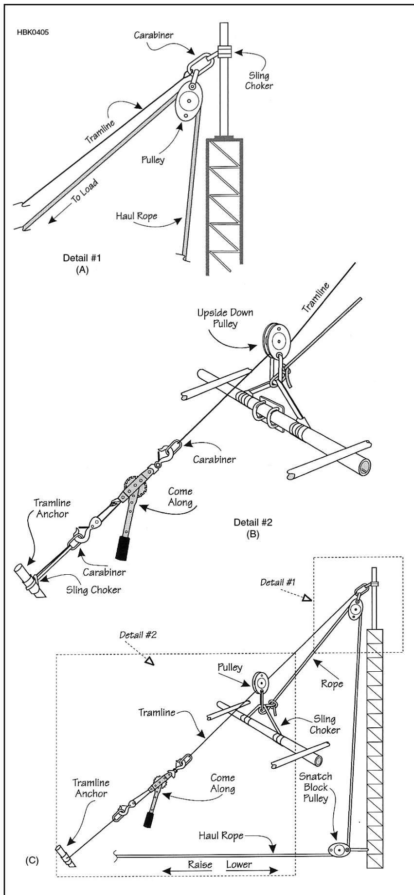
Figure 26.43 — A schematic drawing of the tram line system. At A, rigging the top of the tower for tramming antennas. Note the use of a sling and carabiner. (B) Rigging the anchor of the tramline. A come-along is used to tension the tramline. (C) The tram system for getting antennas up and down. Run the antenna part way up the tramline for testing before installation. It just takes a couple of minutes to run an antenna up or down once the tramline is rigged.
