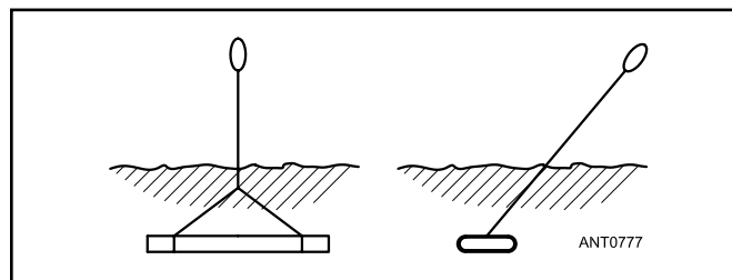
Figure 26.13 — Buried "dead-man" guy anchors (see text).
