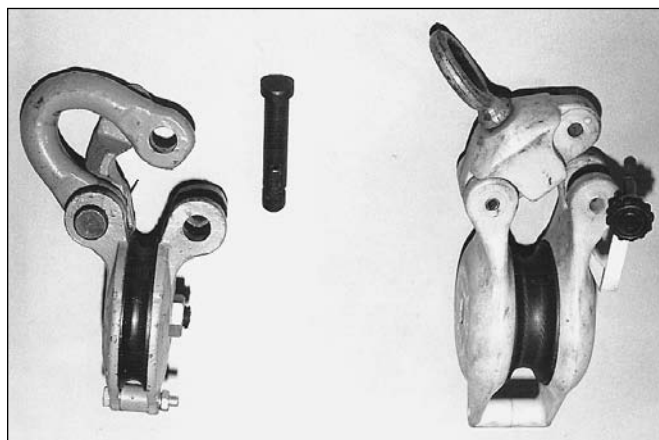
Figure 26.33 — (A) closed snatch-block pulleys. (B) open snatch-block pulleys.
