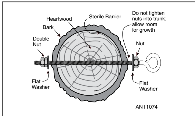
Figure 26.6 — For heavy antenna loads, an eyebolt passed through the trunk or limb will support more weight than an eye-screw. Allow about \frac{1}{2} inch of play between the bolt and trunk or limb. Don't tighten the bolt completely; this allows for tree growth.
