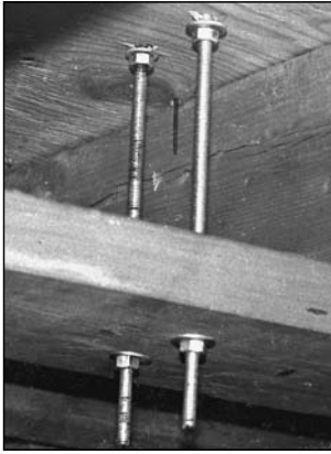
Figure 26.15 — The strengthened anchoring for the roof-mounted tower. Bolts run through the roof and through the anchor plate (2 × 6) between joists. (Photo by Jane Wolfert)
