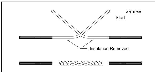
Figure 25.3 — Correct method of splicing antenna wire. Solder should be flowed into the wraps after the connection is completed. After cooling, the joint should be sprayed with acrylic to prevent oxidation and corrosion.
