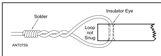
Figure 25.4 — When fastening antenna wire to an insulator, do not make the wire loop too snug. After the connection is complete, flow a non-acid core solder into the turns. When the joint has cooled completely, spray it with acrylic.
