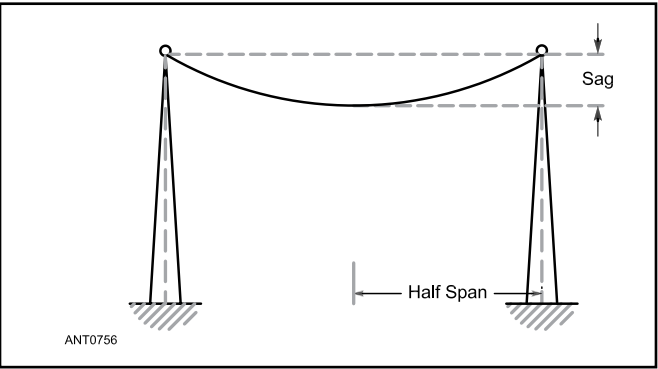
Figure 25.1 — The half span and sag of a long-wire antenna.
