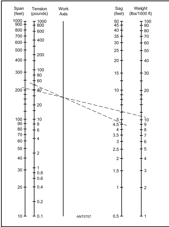
Figure 25.2 — Nomograph for determining wire sag. (courtesy John Elengo, W1DQ)
