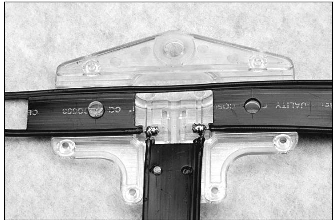
Figure 25.7 — The Ten-Tec “Acro-Bat” is made for attaching parallel-wire feed line to a wire antenna. It provides strain relief and reinforcement to the feed line to keep the conductors from breaking due to repeated flexing and bending in the wind.
