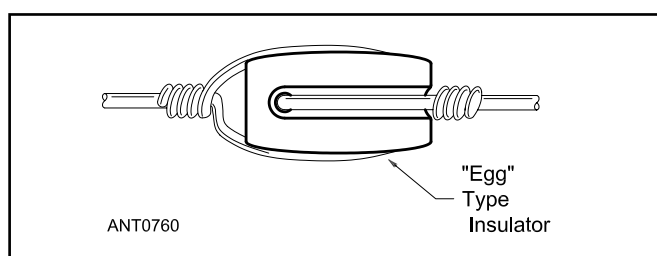
Figure 25.5 — Conventional manner of fastening wire to a strain insulator. This method decreases the leakage path and increases capacitance, as discussed in the text.
