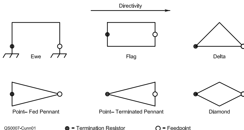
Figure 22.21 — Configurations of the flag and pennant antennas. The dimensions of the Flag, both Pennants, and the Diamond (a modification of the Flag) are 29 feet by 14 feet. The Delta (a type of half-Diamond) is 17 feet high and 28 feet long. The ground-independent antennas are 6 feet above ground.
