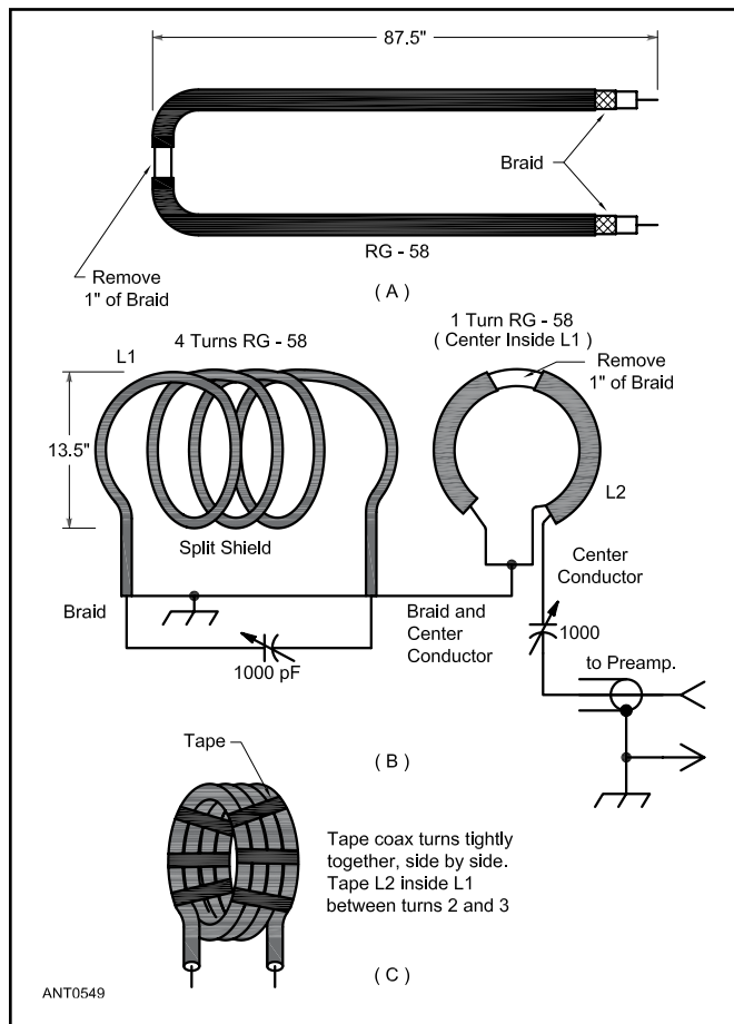
Figure 22.37 — Components and assembly details of the shielded loop shown in Figure 22.36. The dimensions and values given are for 1.8 MHz operation.
