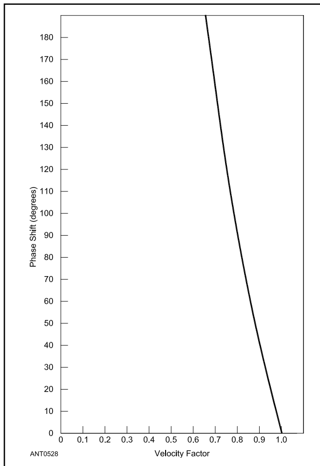
Figure 22.3 — This curve shows phase shift (per wavelength) as a function of velocity factor on a Beverage antenna. Once the phase shift for the antenna goes beyond 90°, the gain drops off from its peak value, and any increase in antenna length will decrease gain.
