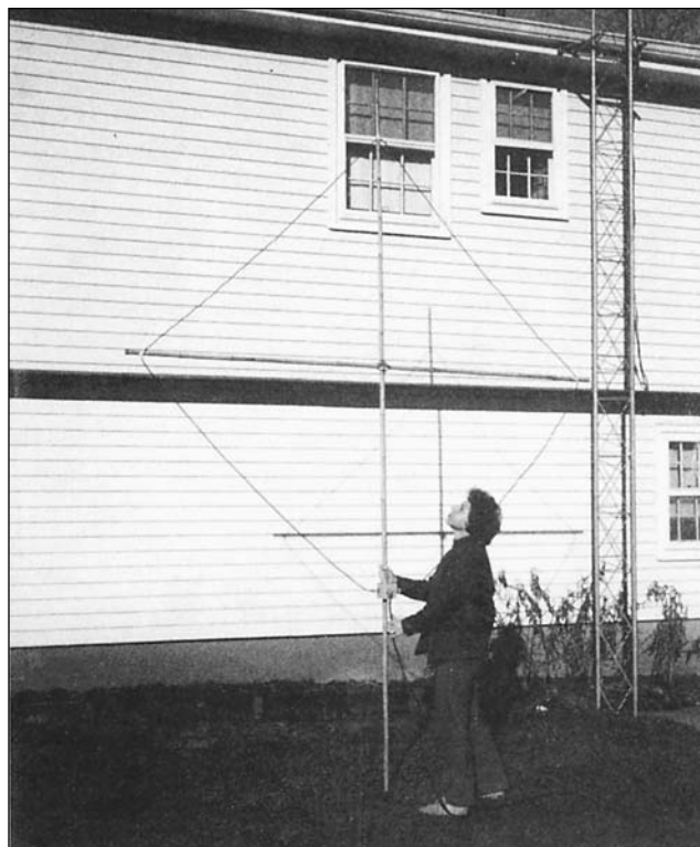
Figure 22.22 — The 160 meter shielded loop uses bamboo cross arms to support the antenna.
