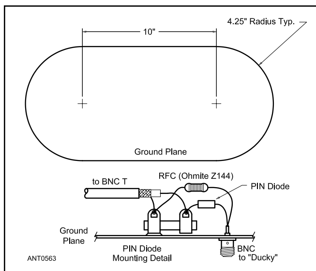
Figure 22.46 — Ground-plane layout and detail of parts at the antenna connectors.
