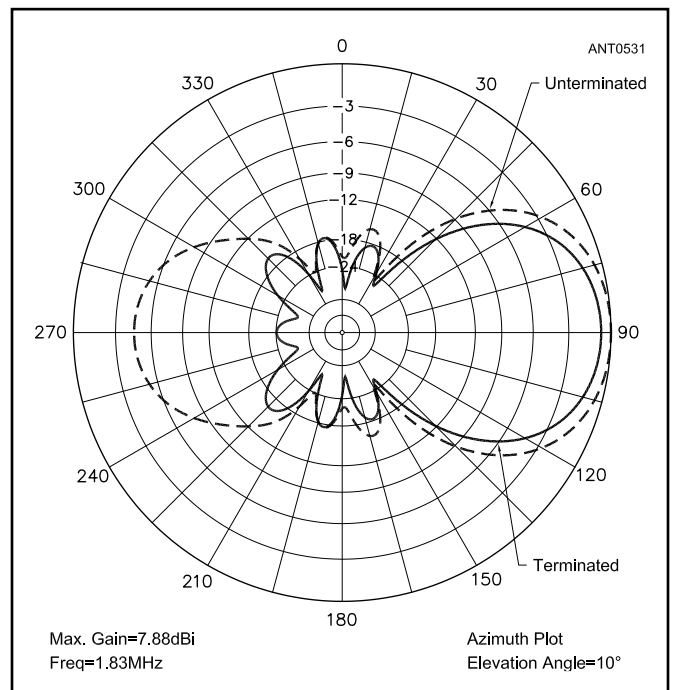
Figure 22.6 — Comparing the azimuthal patterns for a 2- \lambda Beverage, terminated (solid line) and unterminated (dashed line).
