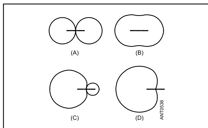
Figure 22.24 — Small-loop field patterns with varying amounts of antenna effect — the undesired response of the loop acting merely as a mass of metal connected to the receiver antenna terminals. The straight lines show the plane of the loop.
