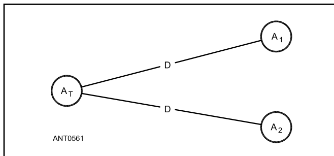
Figure 22.44 — If both receiving antennas are an equal distance ( D ) from the transmitting antenna, there will be no difference in the phase angles of the signals in the receiving antennas. Therefore, the detector will not detect any phase modulation, and the audio tone will disappear from the output of the detector.
