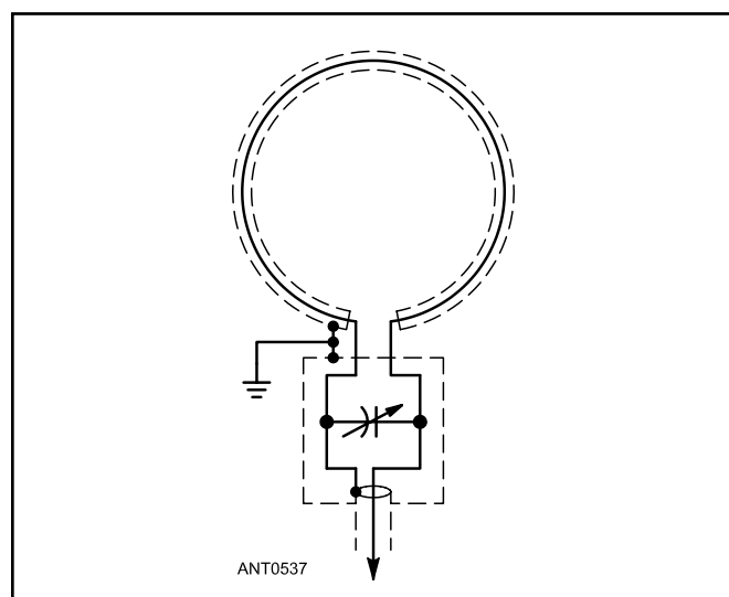
Figure 22.25 — Shielded loop for direction finding. The ends of the shielding turn are not connected, to prevent shielding the loop from magnetic fields. The shield is effective in balancing the loop's response to electric fields.
