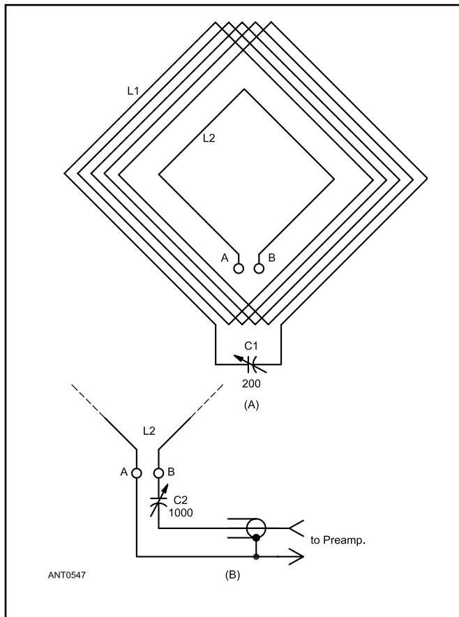
Figure 22.34 — A multitransform antenna is shown at A. L2 is the coupling loop. The drawing at B shows how L2 is connected to a preamplifier.
