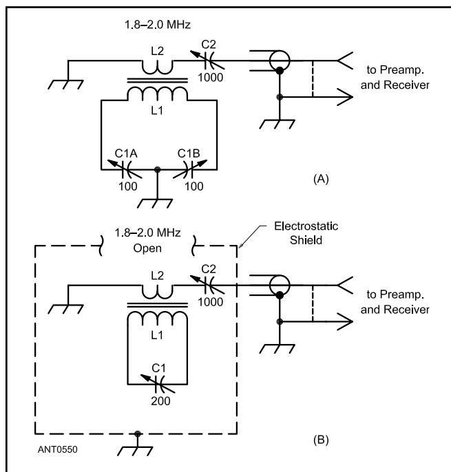
Figure 22.38 — At A, the diagram of a ferrite loop. C1 is a dual-section air-variable capacitor. The circuit at B shows a rod loop contained in an electrostatic shield channel (see text). A suitable low-noise preamplifier is shown in Figure 22.41.
