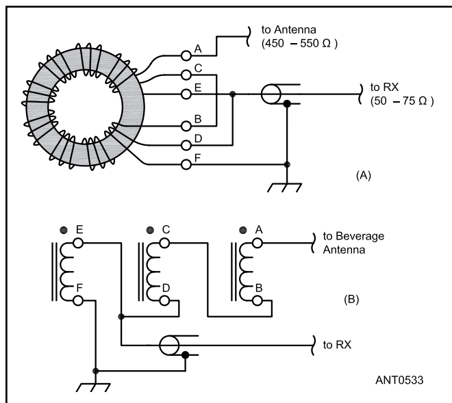
Figure 22.8 — Constructing the feed point transformer for a single-wire Beverage. See text for details.
