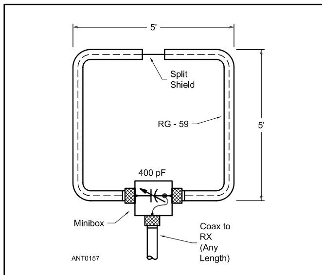
Figure 22.23 — Schematic diagram of the loop antenna. The dimensions are not critical provided overall length of the loop element does not exceed approximately 0.1 \lambda . Small loops which are one half or less the size of this one will prove useful where limited space is a consideration.
