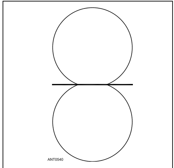
Figure 22.27 — Field pattern for a ferrite rod antenna. The dark bar represents the rod on which the loop turns are wound.
