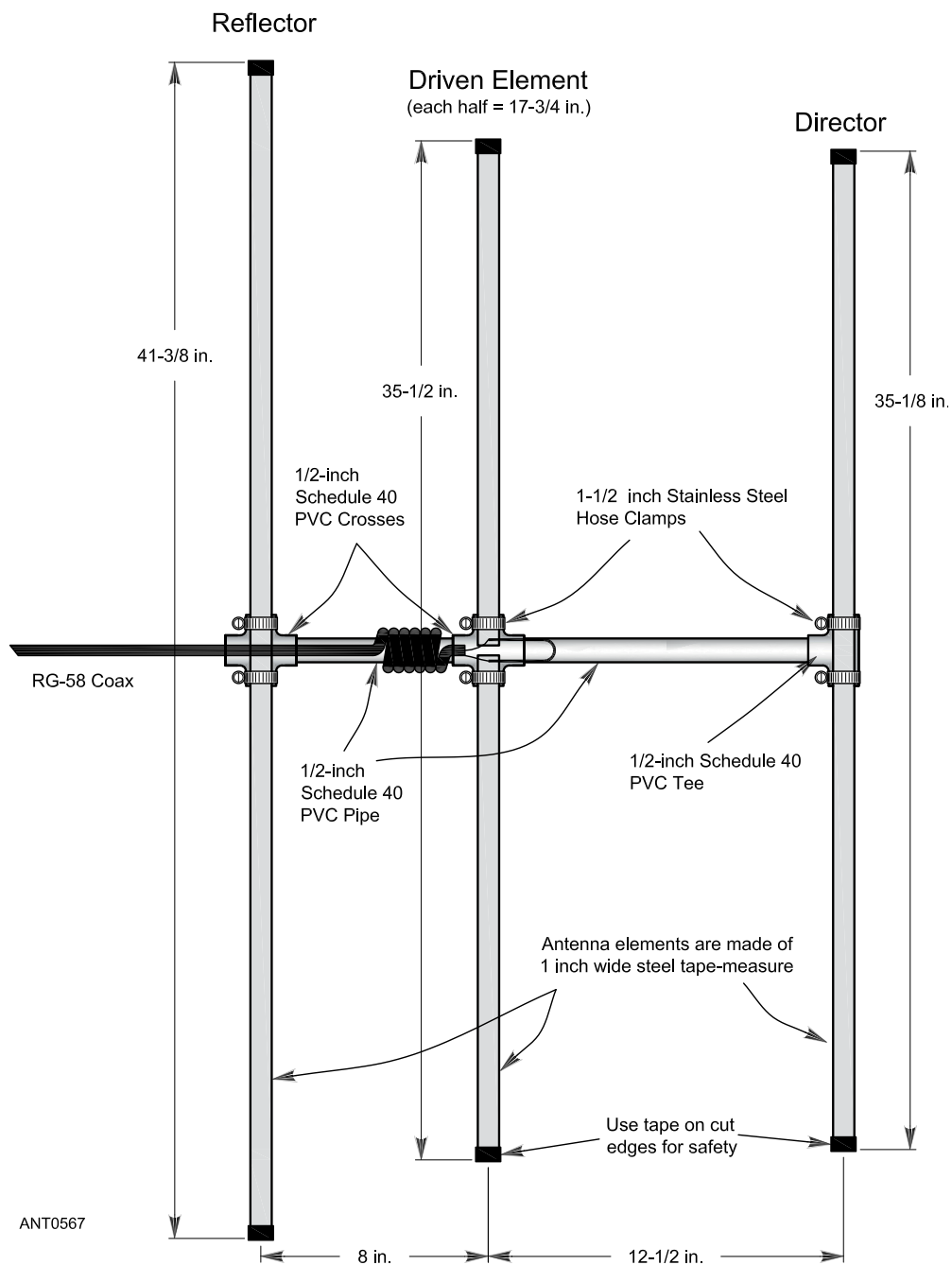
Figure 22.47 — Tape-measure beam dimensions.
