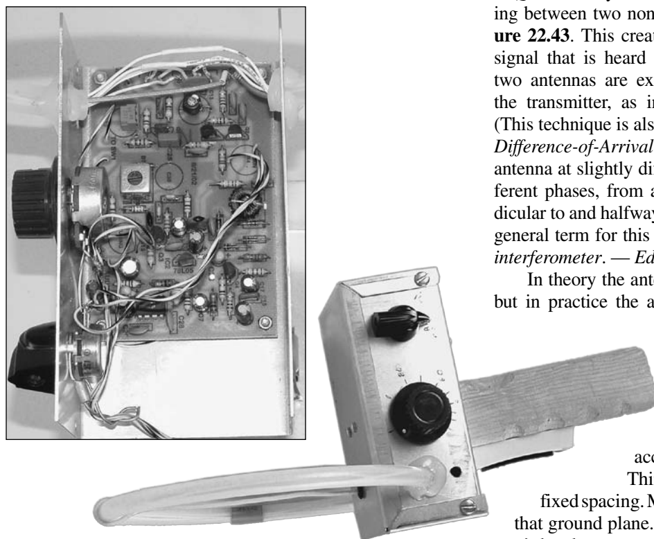
Figure 22.42 — The integrated antenna, handle, and receiver are built into a RadioShack aluminum box. The controls are made to be operated with one hand while using the antenna.
