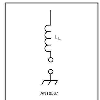
Fig 21.3 — The capacitive reactance at frequencies below the resonant frequency of the whip can be canceled by adding an equivalent inductive reactance in the form of a loading coil in series with the antenna.
