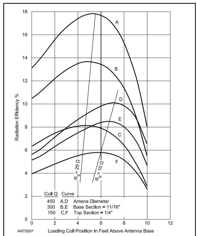
Fig 21.13 — Radiation efficiency of 11-foot antennas at 3.9 MHz.
