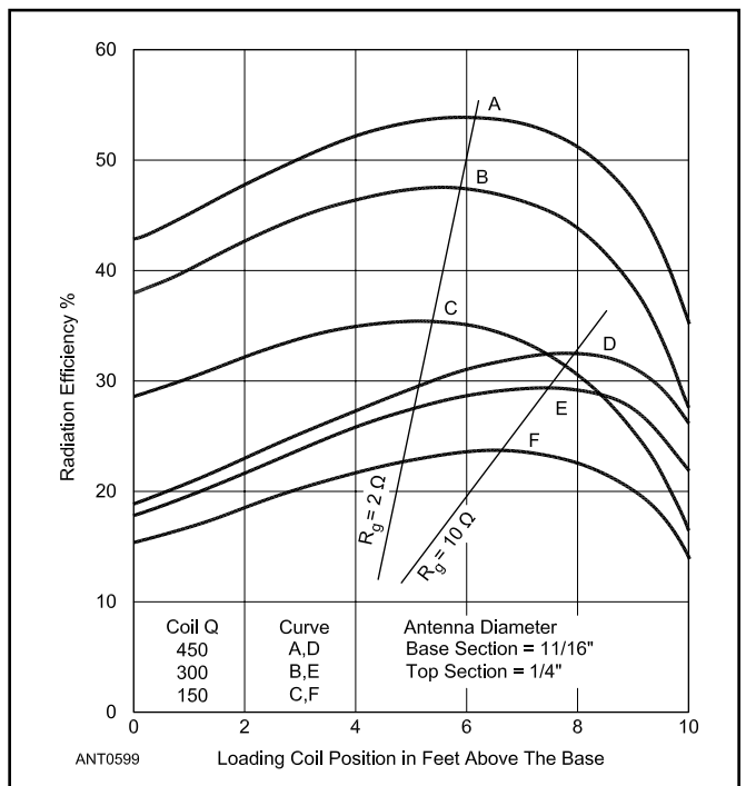
Fig 21.15 — Radiation efficiency of 11-foot antennas at 7.225 MHz.
