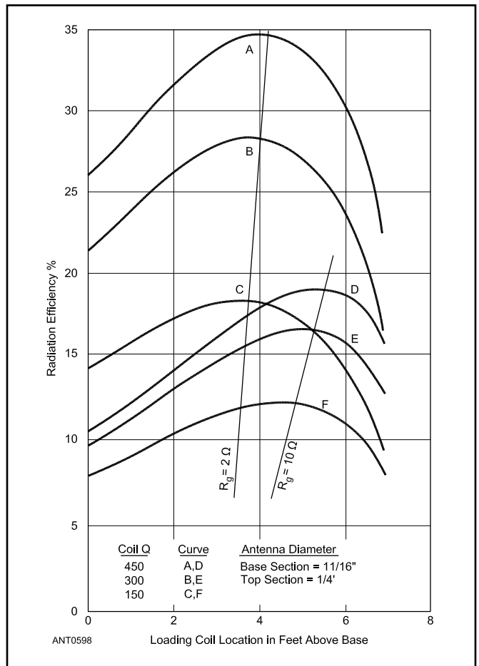
Fig 21.14 — Radiation efficiency of 8-foot antennas at 7.225 MHz.
