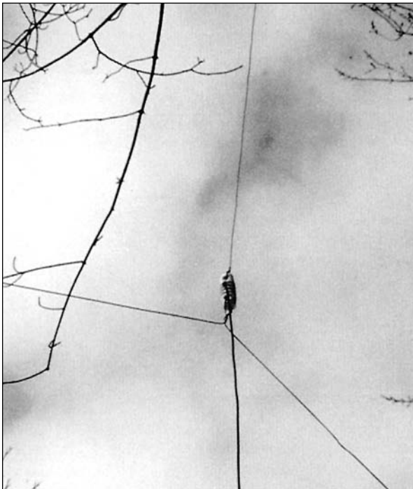
Figure 19.10 — The feed point of the tree-mounted ground-plane antenna. The outside ends of the two radial wires may be tied off to stakes or other convenient points.
