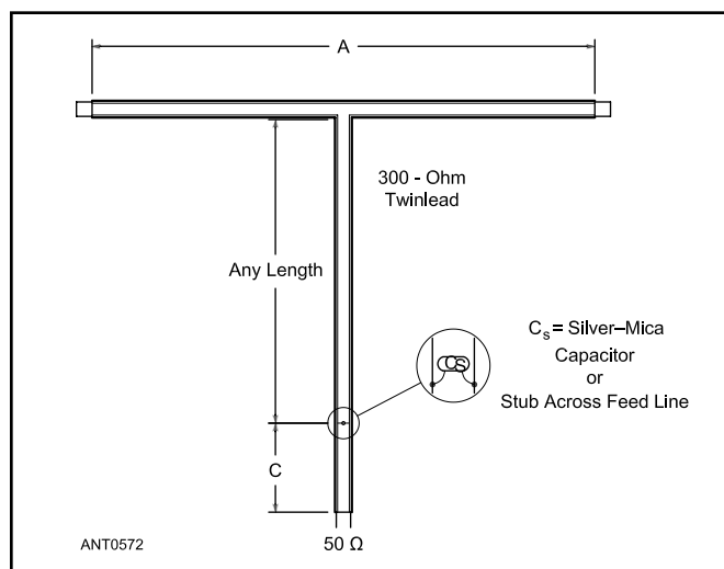
Figure 19.3 — A twinlead folded dipole makes an excellent portable antenna that is easily matched to 50- \Omega equipment. See text and Table 19-3 for details.
