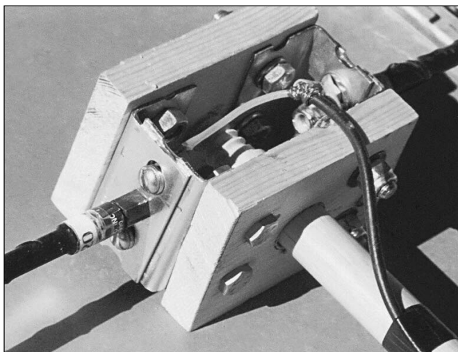
Figure 19.7 — The homemade dipole center support showing the wooden mast, the antenna mounts and the connected transmission line.
