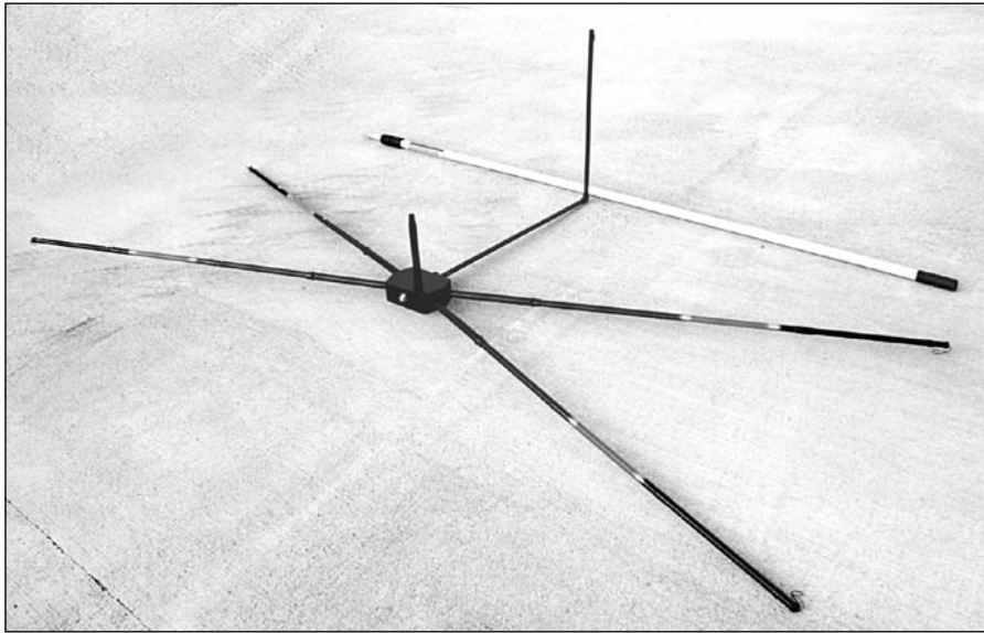
Figure 19.22 — Broken down into its major components — spreaders, hub, feed line support, and wire elements — the beam is ready for transport.
