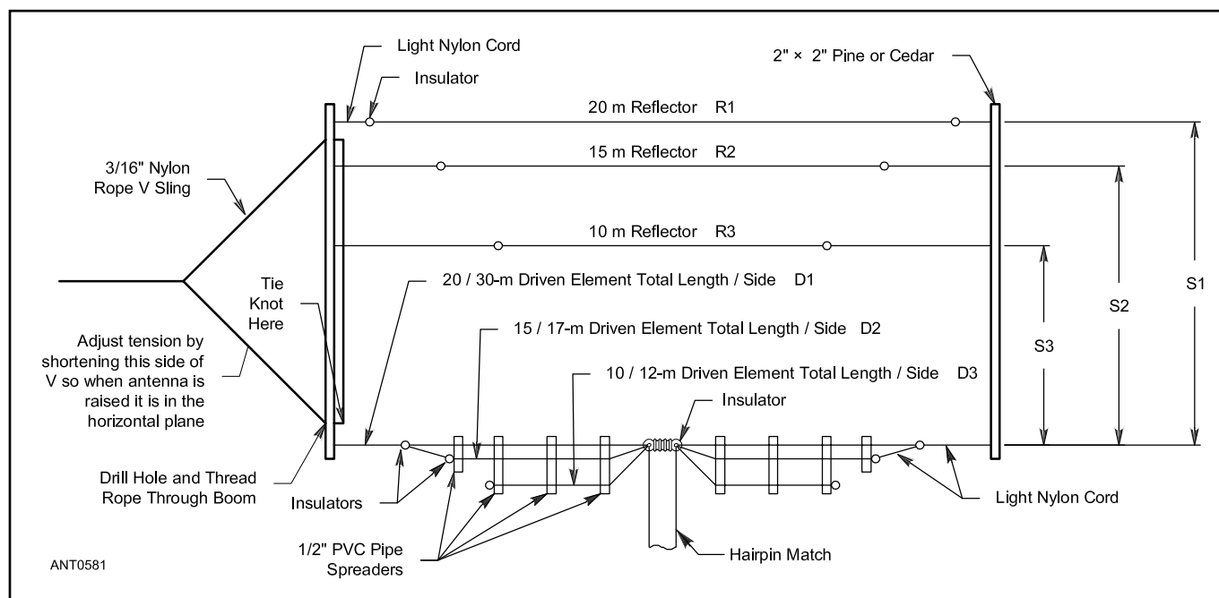
Figure 19.18 — Dimensions for VE7CA's 2-element 10/15/10 meter triband Yagi.
