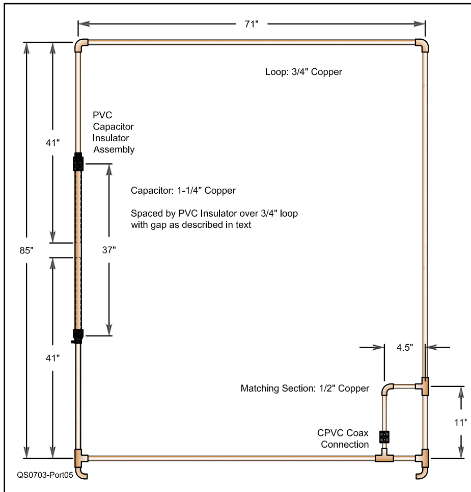
Figure 19.14 — Tuning capacitor and loop assembly details.
