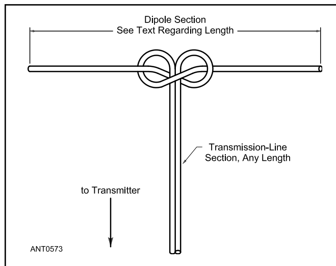
Figure 19.1 — The electrician's knot, often used inside lamp bases and appliances in lieu of a plastic grip, can also serve to prevent the feed line section of a zip-cord antenna from unzipping itself under the tension of dipole suspension. To tie the knot, first use the right-hand conductor to form a loop, passing the wire behind the un-separated zip cord and off to the left. Then pass the left-hand wire of the pair behind the wire extending off to the left, in front of the un-separated pair, and thread it through the loop already formed. Adjust the knot for symmetry while pulling on the two dipole wires.
