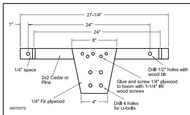
Figure 19.17 — Dimensions for the boom-to-mast bracket of the 2-element 6 meter quad.
