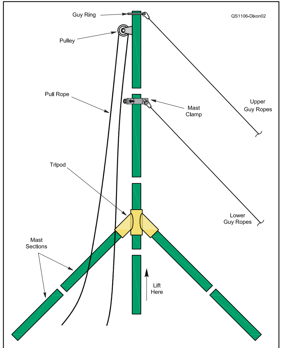
Figure 19.24 — Aluminum mast sections can be combined with a tripod center section to create a mast up to 40 feet high.
