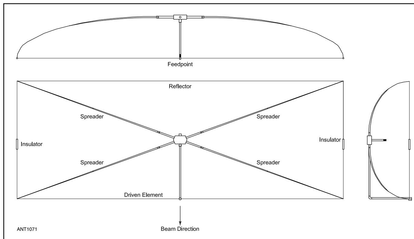
Figure 19.21 — An overview of the antenna and its components. Side drawings show the approximate final bend of the fishing poles with the wire elements attached.
