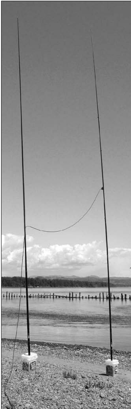
Figure 19.23 — A five-gallon plastic bucket filled with sand and rocks weighs from 40 to 60 pounds and makes a solid base for a fiberglass mast.
