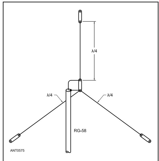
Figure 19.11 — Dimensions and construction of the tree-mounted ground-plane antenna.
