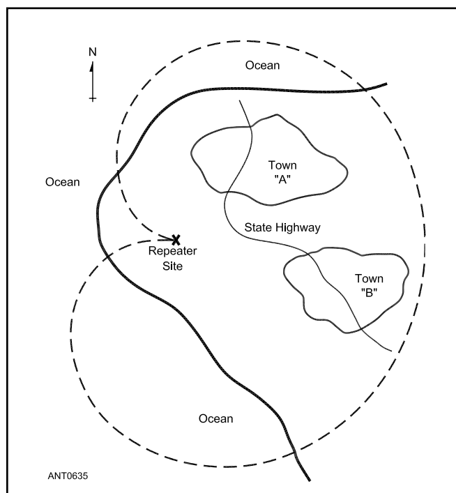
Figure 18.3 — There are many situations where equal repeater coverage is not desired in all directions from the “machine.” One such situation is shown here, where the repeater is needed to cover only towns A and B and the interconnecting highway. An omnidirectional antenna would provide coverage in undesired directions, such as over the ocean. The broken line shows the radiation pattern of an antenna that is better suited to this circumstance.
