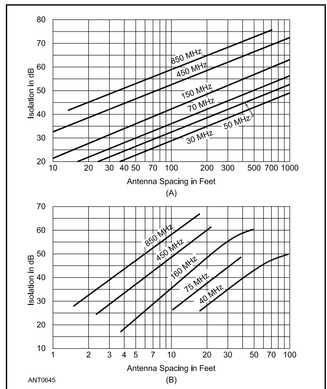
Figure 18.13 — At A, the amount of attenuation (isolation) provided by horizontal separation of vertical dipole antennas. At B, isolation afforded by vertical separation of vertical dipoles.
