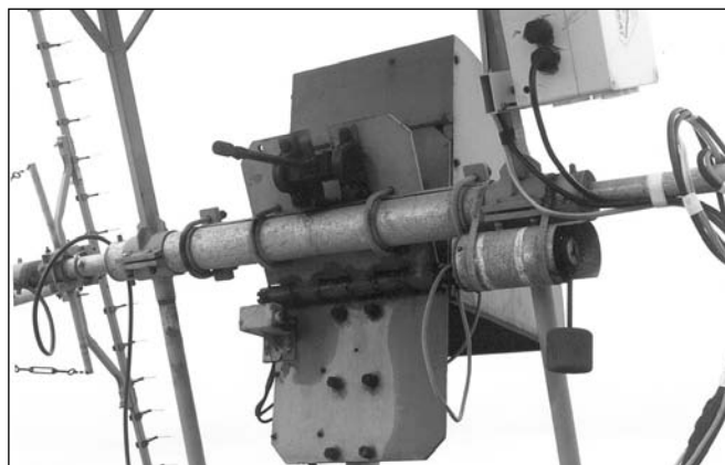
Figure 17.61 — I8CVS’s homebrew elevation mechanism using a very large, industrial hinge as the pivot and a jackscrew drive. (I8CVS photo)
