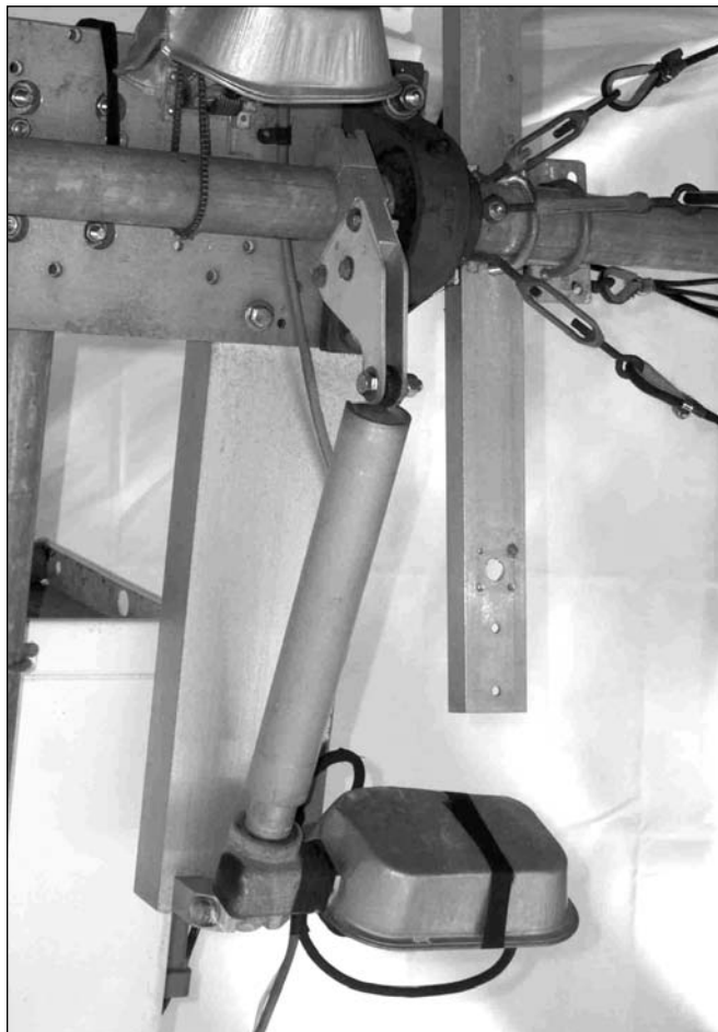
Figure 17.60 — KD1K’s homebrew elevation rotator drive using a surplus-store drive screw mechanism. Note also the large journal bearing supporting the elevation axis pipe shaft. (KD1K photo)
