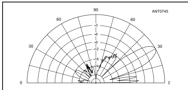
Figure 17.27 — EZNEC Pro elevation pattern for four 14-element 2 meter Yagis ( 3.6\lambda boom lengths) at an elevation angle of 30^\circ above the horizon. The computed system gain is 21.5 dBi, suitable for 2 meter EME. This assumes that the phasing system is made of open-wire transmission lines so that feed line losses can be kept below 0.25 dB.
