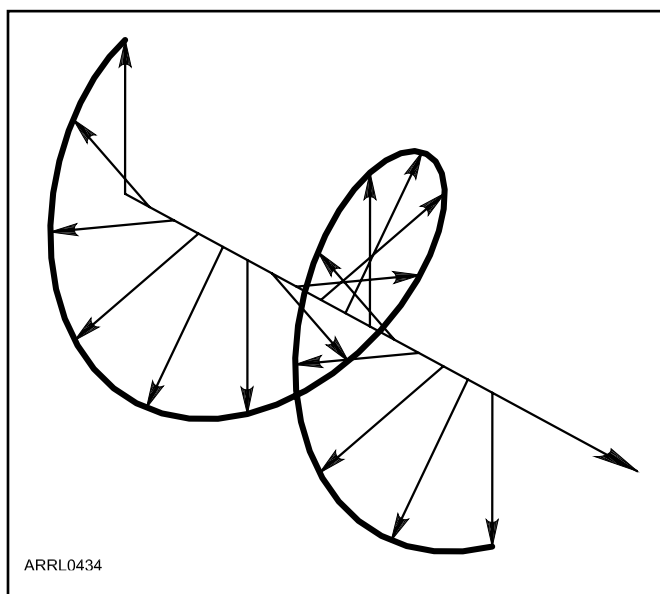
Figure 17.9 — The polarization of a circularly polarized wavefront rotates around its central axis, either clockwise (right-hand or RHCP) or counterclockwise (left-hand or LHCP).
