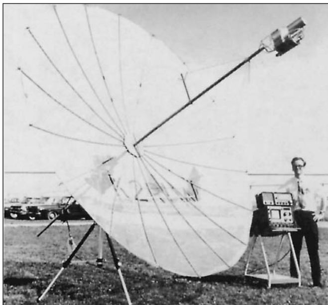
Figure 17.54 — A 12-foot stressed parabolic dish set up for satellite signal near 2280 MHz. A preamplifier is shown taped below the feed horn. The dish was designed by K2RIW, standing at the right. The complete QST construction article is available on this book's CD-ROM.
