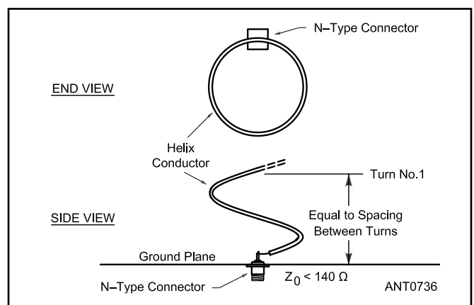
Figure 17.21 — End view and side view of peripherally fed helix.
