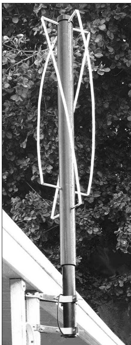
Figure 17.18 — W6NBC's Quadrifilar Helix base station antenna (W6NBC photo)
