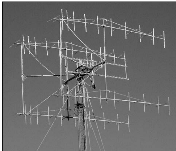
Figure 17.8 — Array of four 10-element, dual-polarization 144-MHz Yagis at KL7UW. Alaskan frost makes the horizontal and vertical elements stand out clearly. A pair of loop Yagis for 1296 MHz can be seen inside the 2 meter array.
