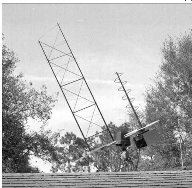
Figure 17.19 — At top, a 16-turn S-band helical antenna. This is about the maximum length of any practical helix. Note the SSB UEK2000 downconverter mounted behind the reflector of the antenna. At bottom, a pair of helical antennas for service on 2 meters and 70 cm. The 2 meter helical antenna is not small! (KD1K photos.)
