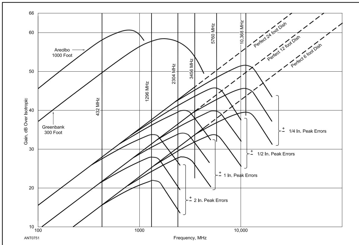
Figure 17.36 — Parabolic-antenna gain versus size, frequency and surface errors. All curves assume 60% aperture efficiency and 10-dB power taper. Graph by K2RIW for amateur bands, using display technique of J. Ruze, British IEE.
