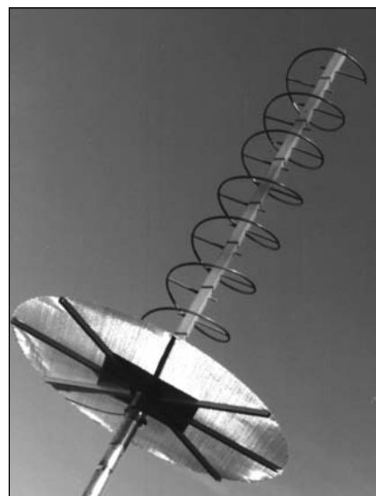
Figure 17.24 — The portable 435-MHz helix assembled and ready for operation. (WØCY photo)
