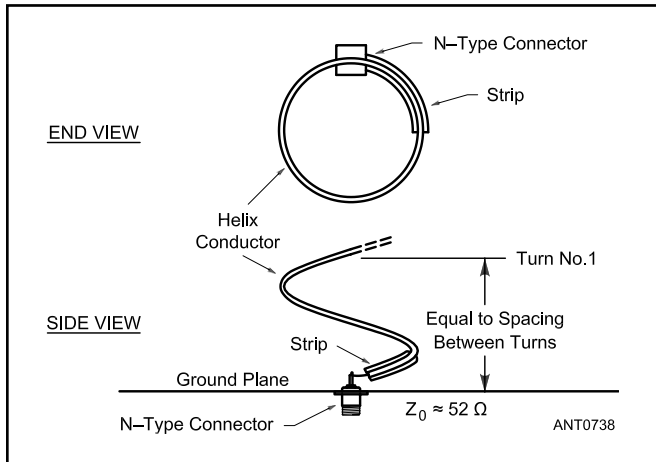
Figure 17.23 — End view and side view of peripherally fed helix with metal strip added to improve transformer action.
