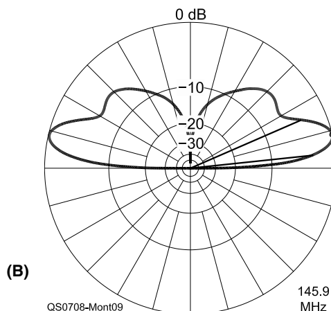
Figure 17.17 — The Lindenblad antenna in A has circular polarization and an omnidirectional azimuthal pattern as shown in B. (AA2TX photo)
