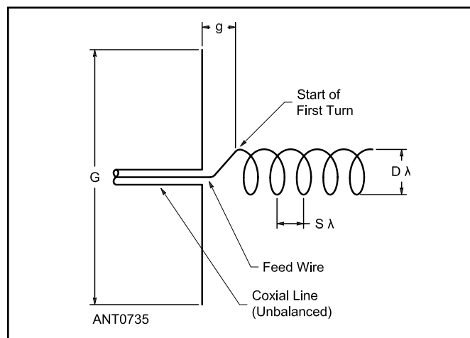
Figure 17.20 — The basic helical antenna and design parameters.
