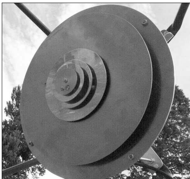
Figure 17.39 — A triband (U, L and S bands) patch-CP feed for large dish antennas for HEO service. (W0LMD photo)
