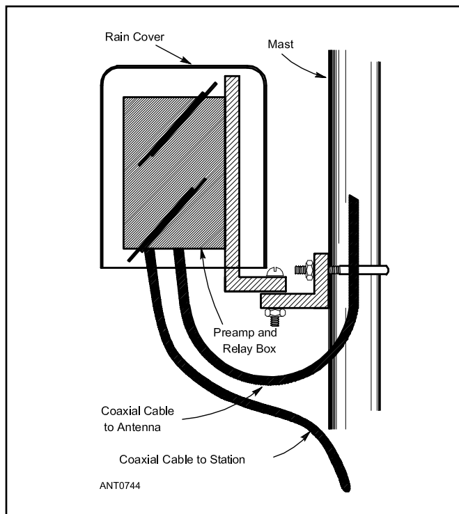
Figure 17.57 — Protection for tower-mounted equipment need not be elaborate. Be sure to dress the cables as shown so that water drips off the cable jacket before it reaches the enclosure. One hazard for such open-bottom enclosures is that of animals gnawing on the cable insulation. Flying insects also like to build their houses in these enclosures.
