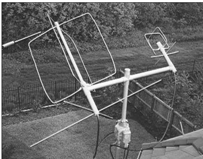
Figure 17.4 — Jerry Brown, K5OE, uses his Texas Potato Masher antennas to work LEO satellites.
