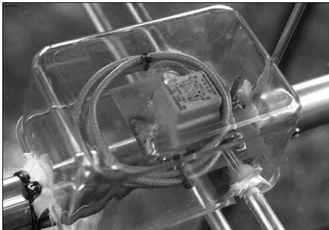
Figure 17.55 — KLM 2M-22C antenna CP switching relay with relocated balun. The protective cover is needed for rain protection, be sure to use a polystyrene kitchen box, see text. (KD1K photo)
