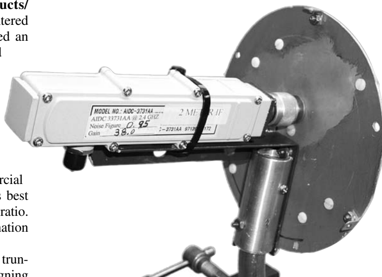
Figure 17.41 — The K5GNA S-band downconverter assembled to the rear of the patch feed assembly. The L-band connector is hidden in this view. (KD1K photo)
