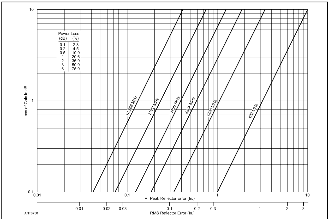
Figure 17.35 — Gain deterioration versus reflector error. By Richard Knadle, K2RIW.
