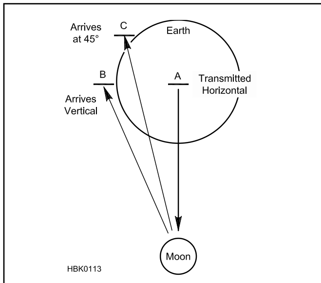
Figure 17.7 — The spherical Earth creates spatial polarization offsets for well-separated stations with horizon-oriented linear polarization. Here, a signal transmitted horizontally at A arrived with vertical polarization at B and midway between horizontal and vertical at C. When combined with Faraday rotation, offsets close to 45° can lead to apparent one-way propagation. See text for details.
