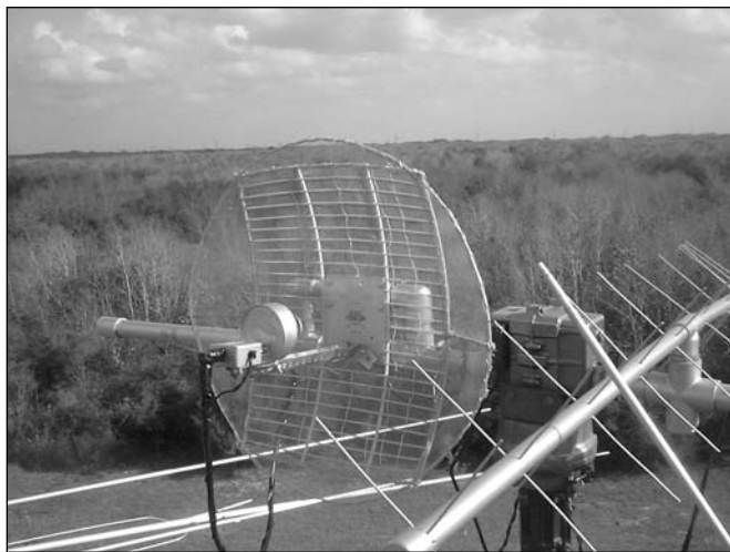
Figure 17.45 — K5GNA’s “circularized” mesh modification of an MMDS dish antenna with a helix-CP feed and preamp. The dish modification reduces the spillover loss by making the antenna fully circular. (K5OE photo)
