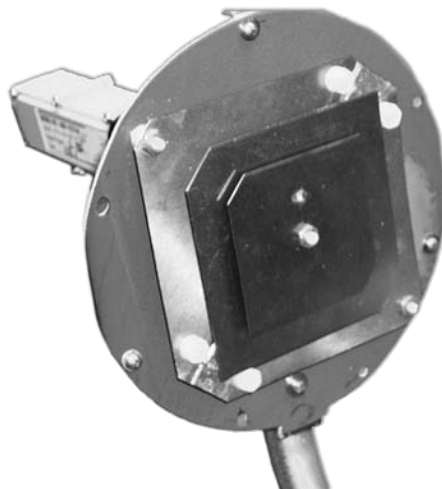
Figure 17.40 — Dual L-band and S-band patch feed assembly. (KD1K photo)
