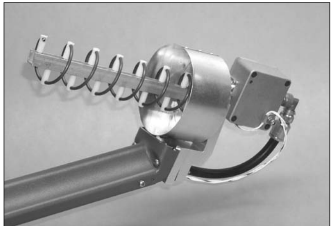
Figure 17.37 — A seven-turn LHCP S-band dish feed for a long f/D offset dish antenna. This helical antenna uses a cupped reflector and has a preamplifier mounted directly to the antenna feed point. (KD1K photo)
