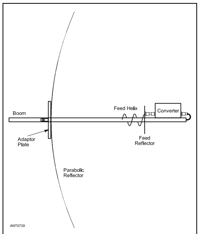
Figure 17.32 — Detail of 60-cm S-band dish antenna with feed.
