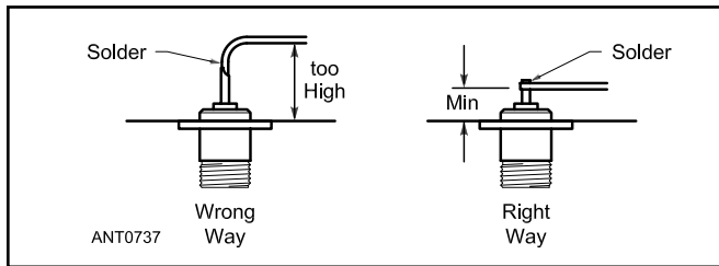
Figure 17.22 — Wrong and right ways to attach a helix to a type N connector for 50-Ω feed.
