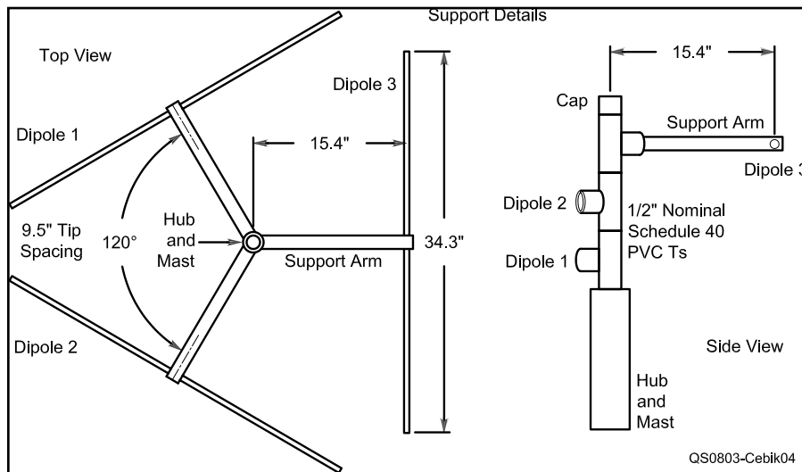
Figure 16.15 — Some details of the support structure used for the three-dipole 2 meter triangle.
