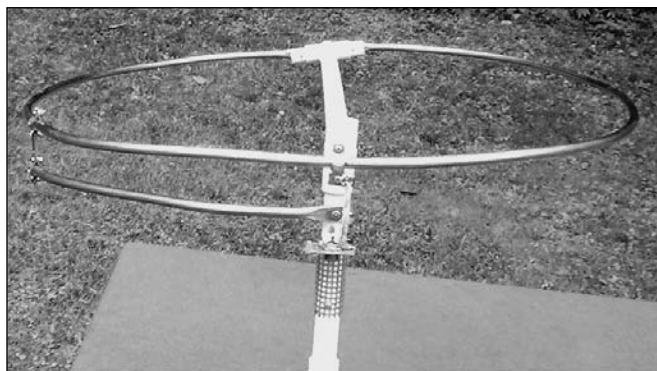
Figure 16.19 — The halo from the rear. A copper strap connects the matching section to the halo on the left.
