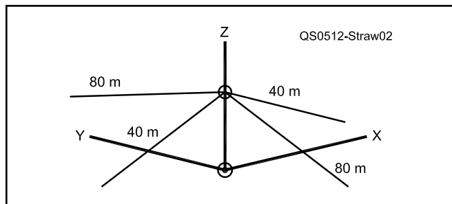
Figure 14.15 — Layout for two band inverted V dipoles for 40 and 80 meters. The two dipoles are fed together at the center and are laid out at right angles to each other to minimize interaction between them. Each end of both dipoles is kept 8 feet above ground for personal safety.
