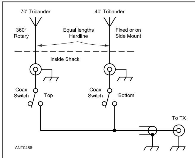
Figure 14.59 — Simple feed system for 70/40-foot stack of tribanders. Each tribander is fed with equal lengths of 0.5-inch 75- \Omega Hardline cables (with equal lengths of flexible coax at the antenna to allow rotation), and can be selected singly or in parallel at the operator's position in the shack. Again, no special provision is made in this system to equal SWR for any of the combinations.
