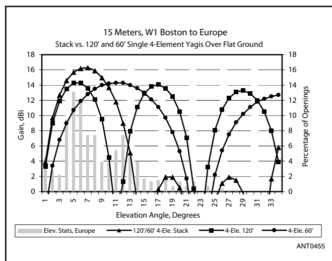
Figure 14.48 — Comparison of elevation patterns for K1EA's illustration about 15 meter Yagis mounted over flat ground, with elevation-angle statistics to Europe added. The stack at 120 and 60 feet yields a better footprint over the range of 3^\circ to 11^\circ at its half-power points, better than either antenna by itself.
