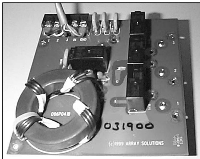
Figure 14.63 — Inside view of StackMatch. (Photo courtesy Array Solutions.)
