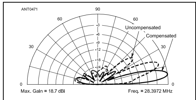
Figure 14.61 — Comparison of elevation responses for 7/5-element 10-meter stacks, with and without compensation for driven-element offset.
