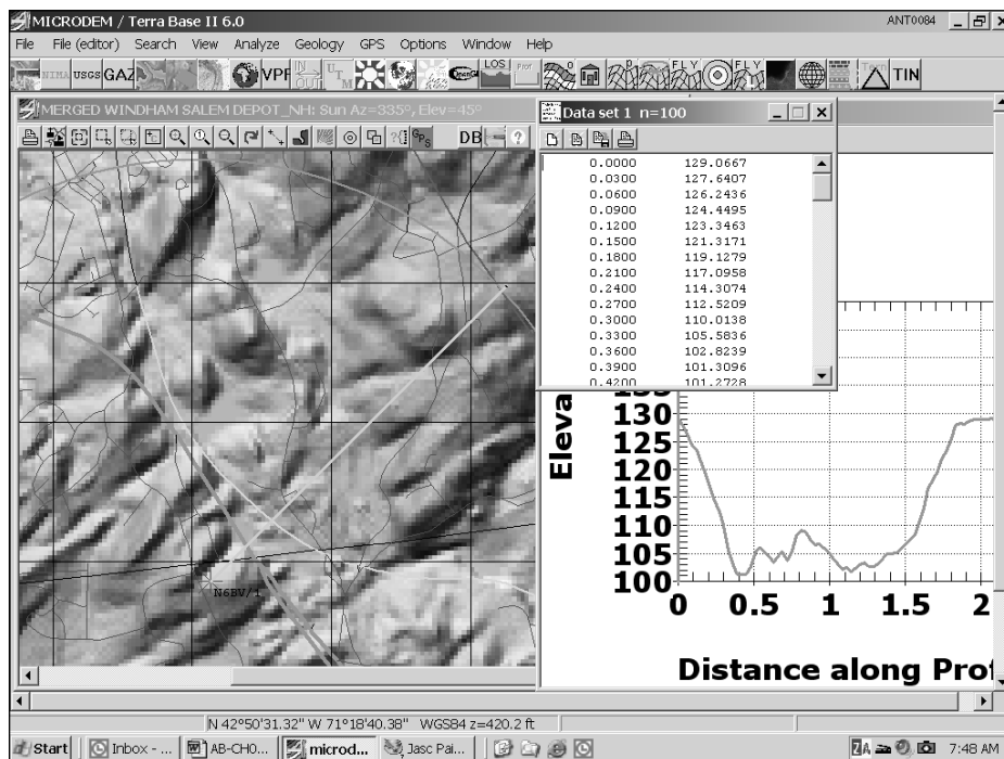
Figure 14.42 — A screen-capture of the MicroDEM program, showing the topographic map for the same terrain shown in Figure 14.41, together with the computed terrain profile along an azimuth of 45° on the path toward Europe from the N6BV/1 location in Windham, NH.
