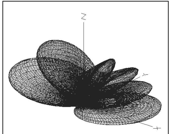
Figure 14.64 — 3D representation of the pattern for two 4-element 15-meter Yagis, with the top antenna at 95 and the bottom at 65 feet, but pointed in the opposite direction.
