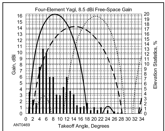
Figure 14.65 — HFTA screen shot of “BIP/BOP” operation of two 4-element 15-meter Yagis at 93 and 46 feet above flat ground. The elevation response in BOP (both out-of-phase) operation is shifted higher, peaking at about 21°, compared to the BIP (both in-phase) operation where the peak is at 8°. The dashed line is response of single Yagi at 46 feet.
