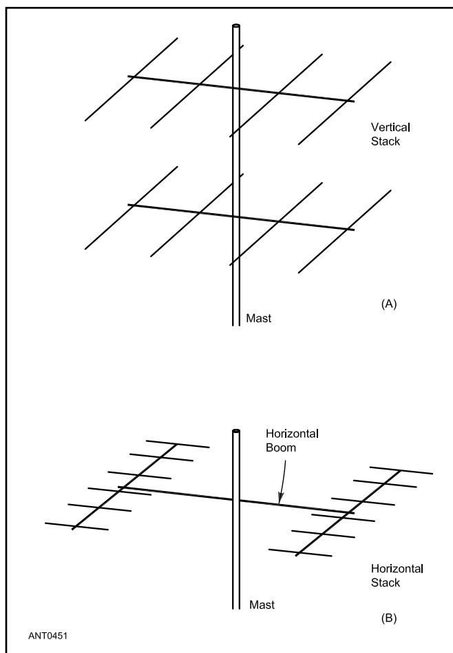
Figure 14.44 — Stacking arrangements. At A, two Yagis are stacked vertically (broadside) on the same mast. At B, two Yagis are stacked horizontally (collinear) side-by-side. At HF the vertical stack is more common because of mechanical difficulties involved with large HF antennas stacked side-by-side, whereas at VHF and UHF the horizontal stack is common.
