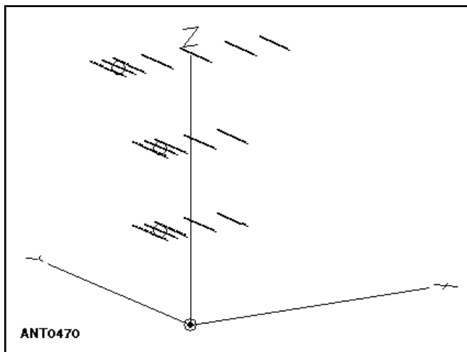
Figure 14.60 — Stacking dissimilar Yagis. In this case a 7-element 10-meter Yagi is stacked over two 5-element Yagis. Note the displacement of the 7-element Yagi's driven element compared to the position of the two 5-element Yagis. This leads to an undesired phase shift for the higher antenna.
