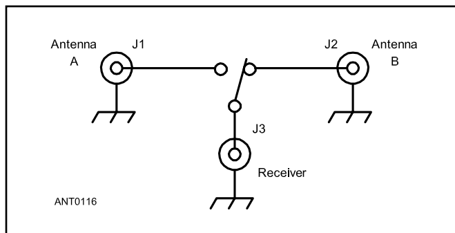
Figure 14.7 — When antennas are compared on fading signals, the time delay involved in disconnecting and reconnecting coaxial cables is too long for accurate measurements. A simple slide switch will do well for switching coaxial lines at HF. The four components can be mounted in a tin can or any small metal box. Leads should be short and direct. J1 through J3 are coaxial connectors.
