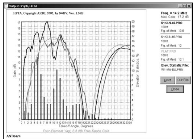
Figure 14.57 — HFTA screen shot showing the 20-meter elevation pattern for K1KI's North and South towers, with 100-foot high 4-element Yagis pointing into Europe at an azimuth of 45°. The responses are surprisingly different for two towers separated by only 600 feet.
