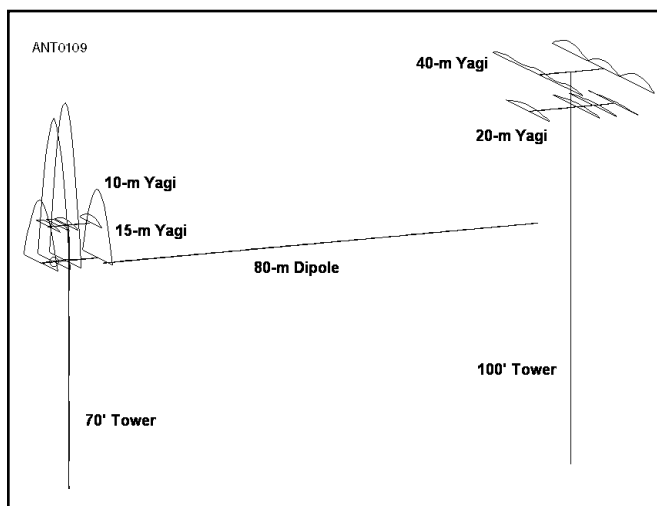
Figure 14.4 — The layout and 15 meter currents when the Yagis on the 100-foot tower are pointed toward the 70-foot tower. The 15 meter Yagi has been rotated to face the direction of the 100-foot tower (toward the Caribbean).
