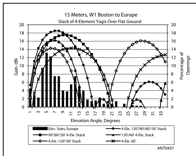
Figure 14.50 — Various stacks toward Europe from New England for 15 meters. The stack at 120 and 30 feet is clearly suboptimal, since the second lobe is higher than the first lobe. The 120/60-foot stack is better in this regard, but is still not as good a performer as the 90/60/30-foot stack. It's debatable whether going to four Yagis in the 120/90/60/30-foot stack is a good idea because it drops below the performance of the 90/60/30-foot stack at about 10^\circ in elevation. The exact distance between practical HF Yagis is not critical to obtain the benefits of stacking. For a stack of tribanders at 90, 60 and 30 feet, the distance in wavelengths between individual antennas is 0.87 \lambda at 28.5 MHz, 0.65 \lambda at 21.2 MHz, and 0.43 \lambda at 14.2 MHz.
