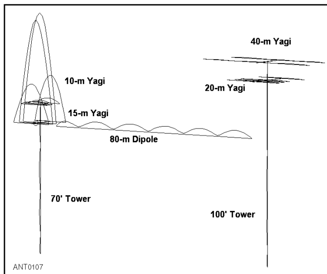
Figure 14.2 — Layout for two-tower antenna system, at 70 and 100 feet high and 150 feet apart. The 70-foot tower has a 4-element 10 meter Yagi at 80 feet on a 10-foot rotating mast and a 4-element 15 meter Yagi at 70 feet. An 80 meter dipole goes from the 70-foot tower to the 100-foot tower, which holds a 2-element 40 meter Yagi at 110 feet and a 4-element 20 meter Yagi at 100 feet. In this figure all the rotatable Yagis are facing the direction of Europe and the currents on the 15 meter Yagi are shown. Note the significant amount of current induced on the nearby 80 meter dipole that will cause a re-radiated signal!
