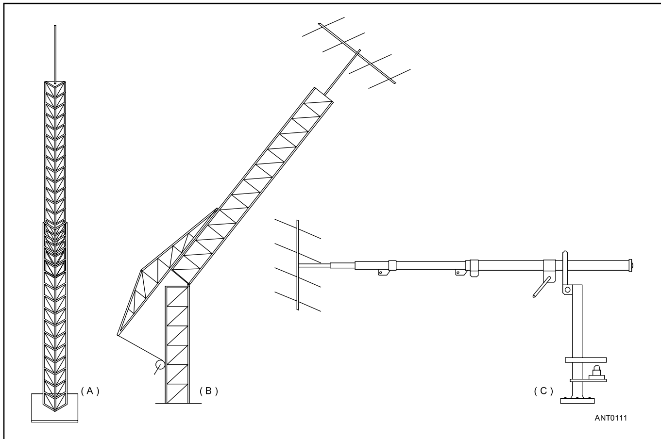
Figure 14.6 — Alternatives to a guyed tower are shown here. At A, the crank-up tower permits working on antennas at reduced height. It also allows antennas to be lowered during periods of no operation. Motor-driven versions are available. The fold-over tower at B and the combination at C permit working on antennas at ground level.
