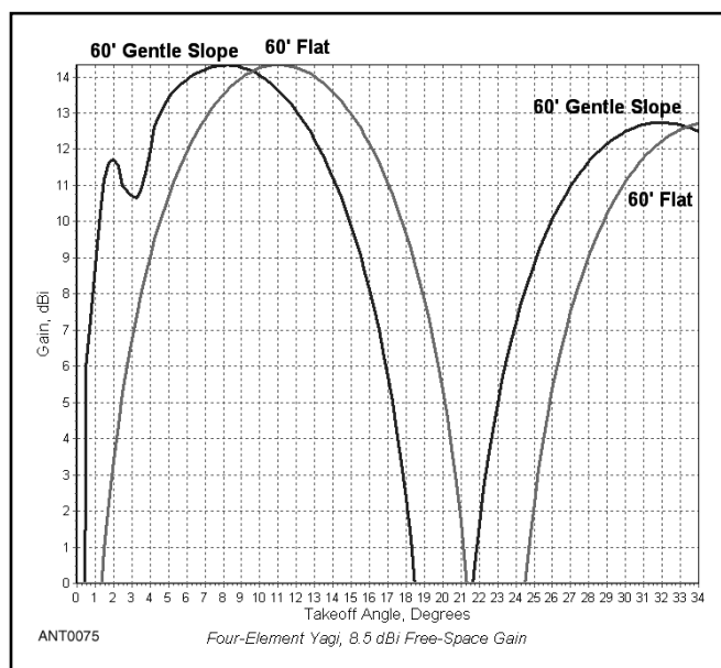
Figure 14.33 — Elevation response for terrain shown in Figure 14.32, using a 4-element 15 meter Yagi, 60 feet high. Note that the shape of the response is essentially shifted toward the left, toward lower elevation angles, by the angle of the sloping ground. For reference, the response for an identical Yagi placed over flat ground is also shown.
