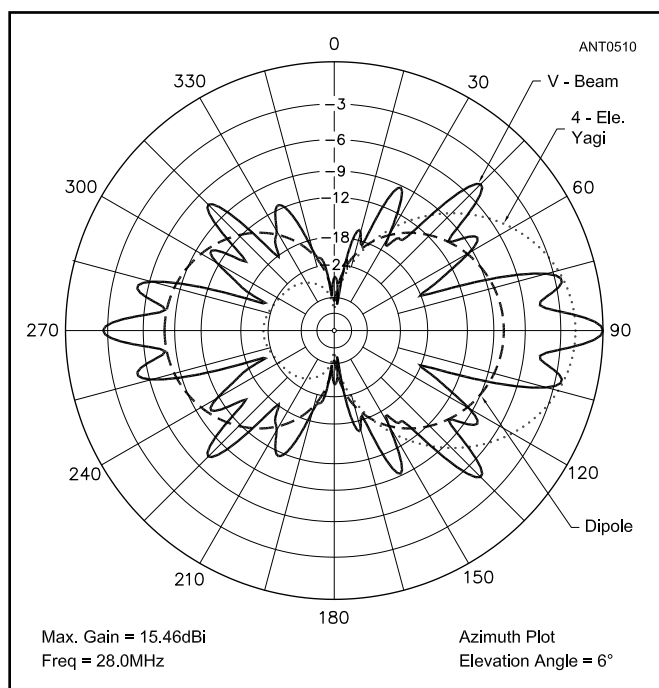
Figure 13.15 — The same 209-foot-per-leg V-beam as Figure 13.14, but at 28 MHz. Again, the two close-in sidelobes tend to spread out the azimuthal response some at 28 MHz.
