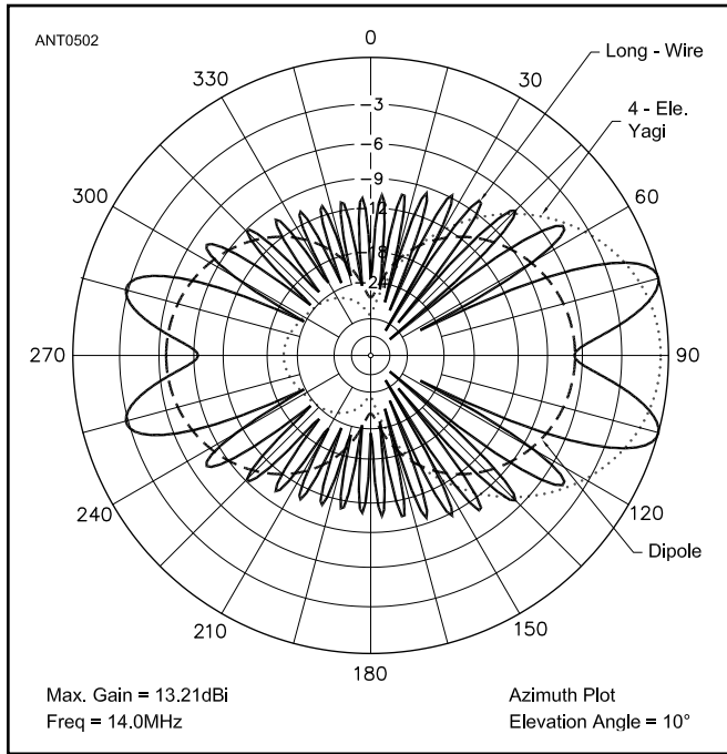
Figure 13.7 — The azimuthal-plane performance for an 8- \lambda (571 feet) long-wire antenna (solid line), compared with a 4-element Yagi (dotted line) and a \frac{1}{2} - \lambda dipole (dashed line).
