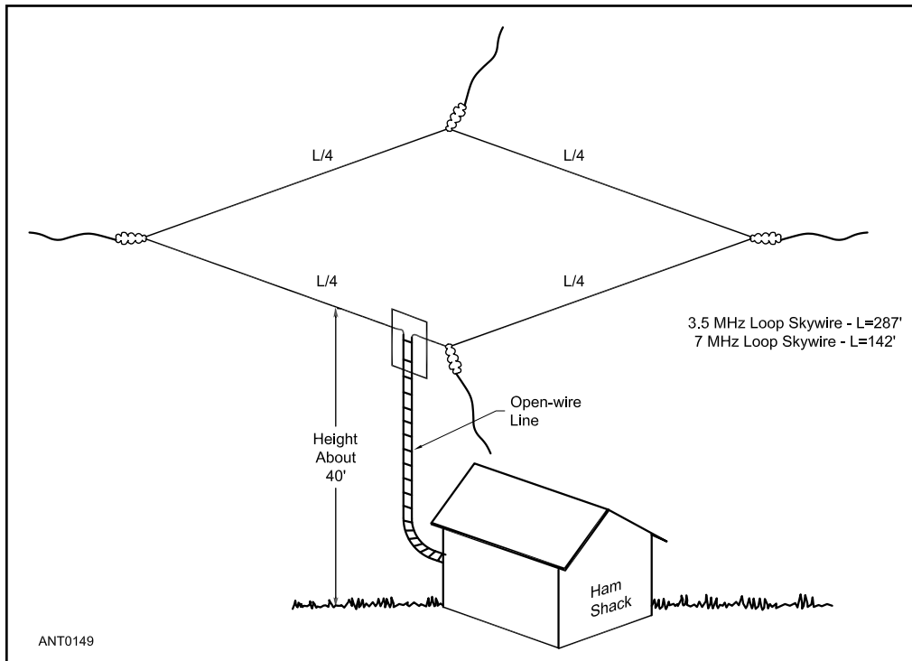
Figure 10.19 — A complete view of the Loop Skywire. The square loop is erected horizontally.
