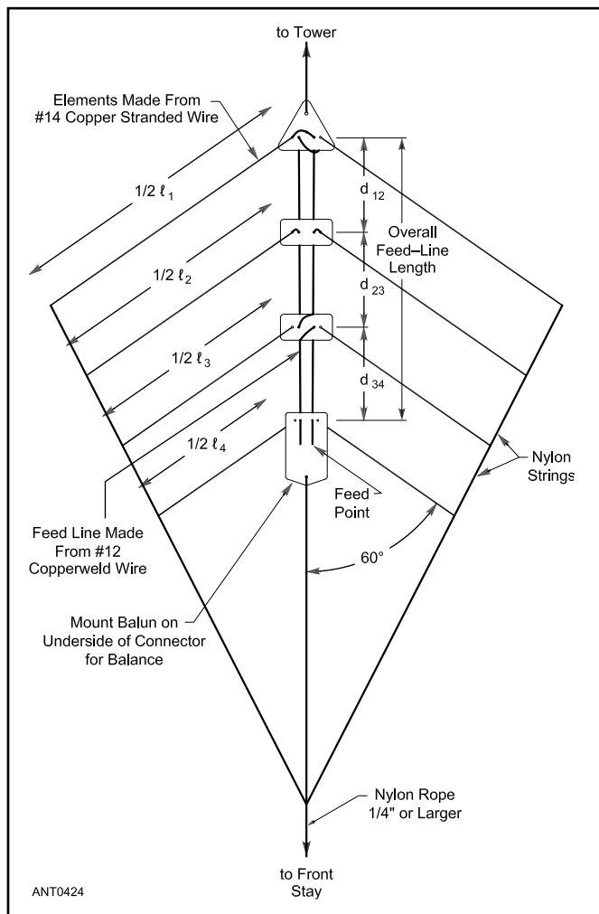
Figure 10.47 — The generic layout for the lower HF wire LPDA. Use a 4:1 balun on the forward connector. See Tables 10-4 and 10-5 for dimensions.
