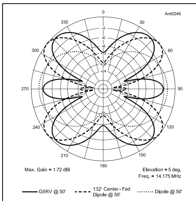
Figure 10.10 — Azimuth pattern at a 5° elevation angle for a 102-foot long, 50-foot high G5RV dipole (solid line). For comparison, the response for a 132-foot long, center-fed dipole at 50 feet height (dashed line) and a 33-foot long half-wave 20 meter dipole at 50 feet (dotted line) are also shown. The longest antenna exhibits about 0.5 dB more gain than the G5RV, although the response is more omnidirectional for the G5RV — an advantage for a wire antenna that is not usually rotatable.
