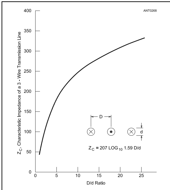
Figure 10.37 — Characteristic impedance of transmission-line mode in an open-sleeve antenna.
