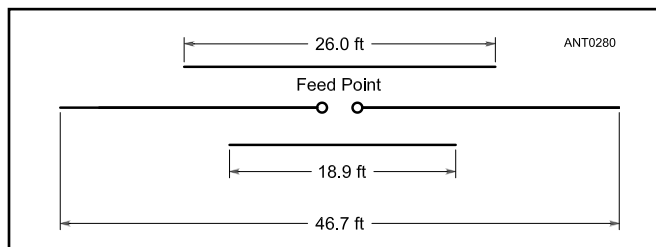
Figure 10.44 — Dimensions of a C-R dipole for the 30, 17 and 12 meter bands.
