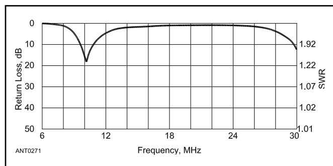
Figure 10.40 — Return loss and SWR of a 10 MHz vertical antenna. A return loss of 0 dB represents an SWR of infinity. The text contains an equation for converting return loss to an SWR value.
