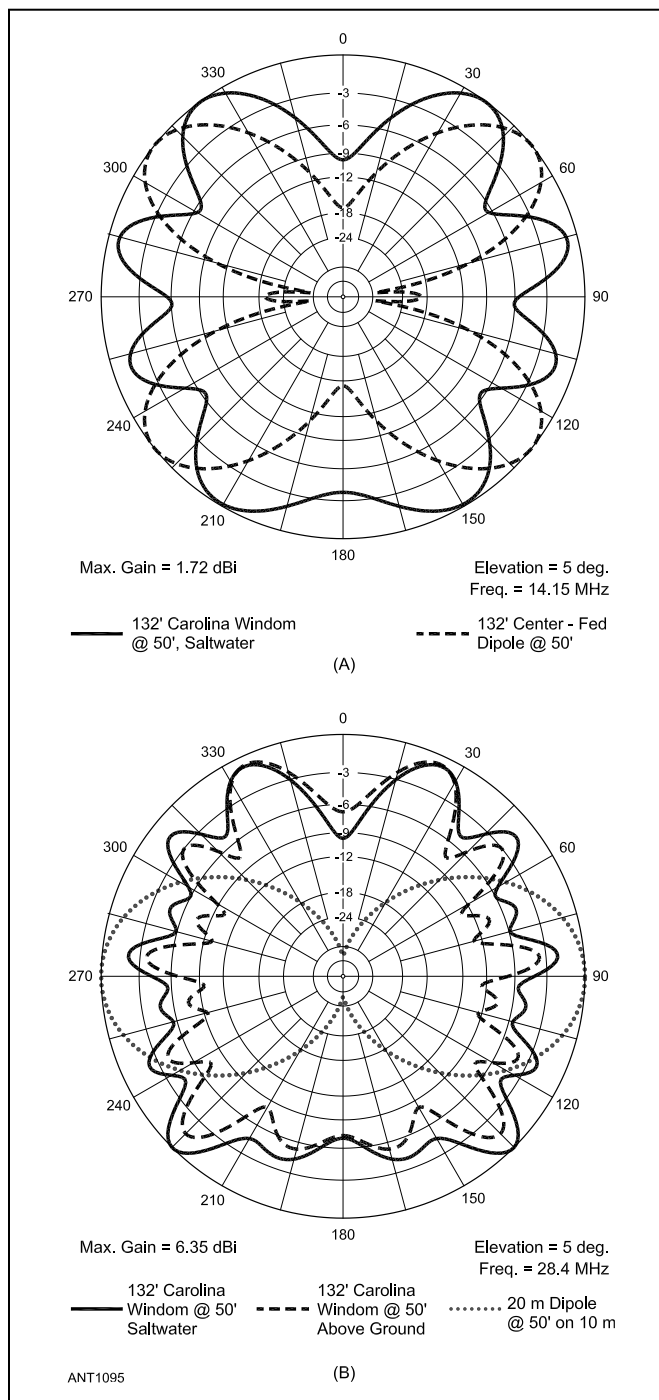
Figure 10.13 — At A, 20 meter azimuth patterns for a 132-foot long off-center fed Carolina Windom and a 132-foot long center-fed flattop dipole on 20 meters, both at a height of 50 feet above saltwater. The response for the Carolina Windom is more omnidirectional because the vertically polarized radiation from the 22-foot long vertical RG-8X coax fills in the deep nulls. At B, 10 meter azimuthal responses for a 132-foot long, 50-foot high Carolina Windom over saltwater (solid line) and over average ground (dashed line), compared to that for a 20 meter half-wave dipole at 50 feet (dotted line).
