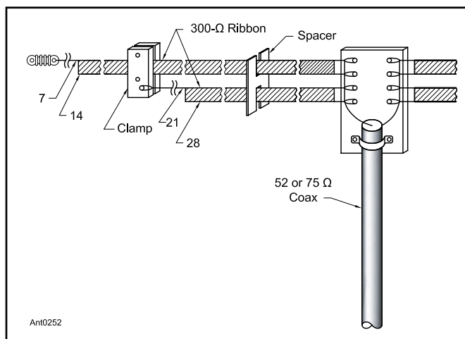
Figure 10.16 — Sketch showing how the twin-lead multiple-dipole antenna system is assembled. The excess wire and insulation are stripped away.
