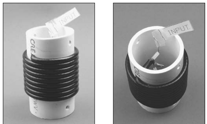
Figure 10.29 — Other views of a W8NX coax-cable trap.
