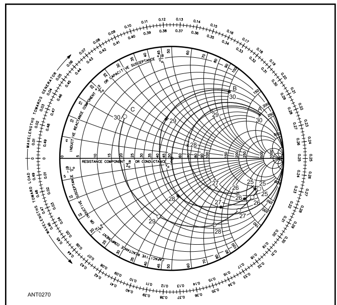
Figure 10.39 — Impedance of the open-sleeve monopole for the range 25-30 MHz. For curves A, B and C the spacings from the central monopole to the sleeve elements are 8, 6 and 4 inches, respectively.
