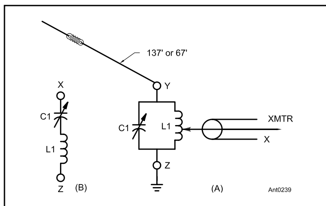
Figure 10.2 — If the antenna length is 137 feet, a parallel-tuned coupling circuit (A) can be used on each amateur band from 3.5 through 30 MHz, with the possible exception of the 10-, 18- and 24-MHz bands. C1 should be from 500-1000 pF with plate spacing capable of withstanding several hundred volts. L1 should be chosen to resonate with 20-80% of C1's maximum value. If the wire is 67 feet long, series tuning can be used on 3.5 MHz as shown at the left; parallel tuning will be required on 7 MHz and higher frequency bands. The L network shown in Figure 10.1B is also suitable for these antenna lengths.
