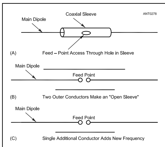
Figure 10.42 — Evolution of coupled-resonator antennas: At A, the coaxial-sleeve dipole; at B, the open-sleeve dipole; and at C, a coupled-resonator dipole, the most universal configuration.
