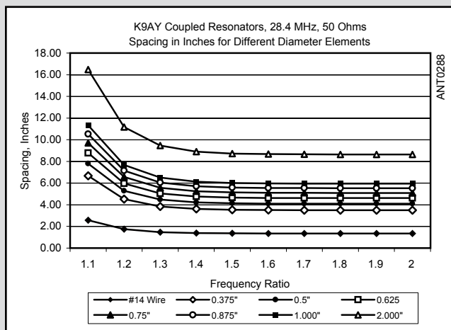
Figure 10.A — Graph of the spacing versus frequency ratio for two Coupled-Resonator elements at 28.4 MHz, for 50- \Omega feed point impedance.
