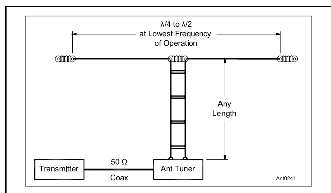
Figure 10.5 — A center-fed antenna system for multiband use.
