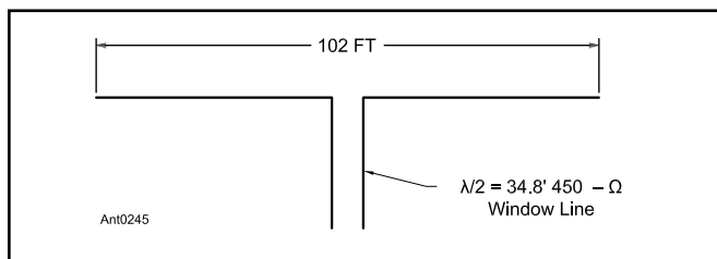
Figure 10.9 — The G5RV multiband antenna covers 3.5 through 30 MHz. Although many amateurs claim it may be fed directly with 50-Ω coax on several amateur bands, Louis Varney, its originator, recommends the use of a matching network on bands other than 14 MHz.
