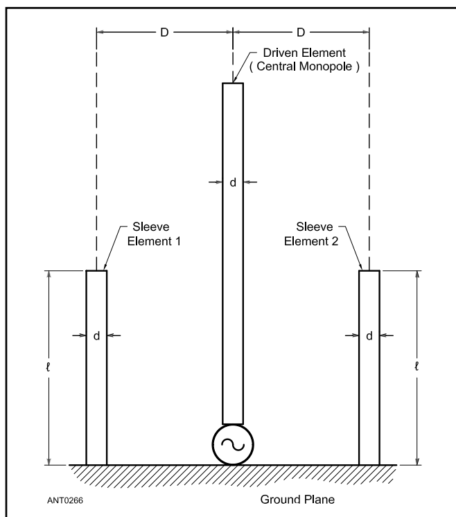
Figure 10.35 — Diagram of an open-sleeve monopole.
