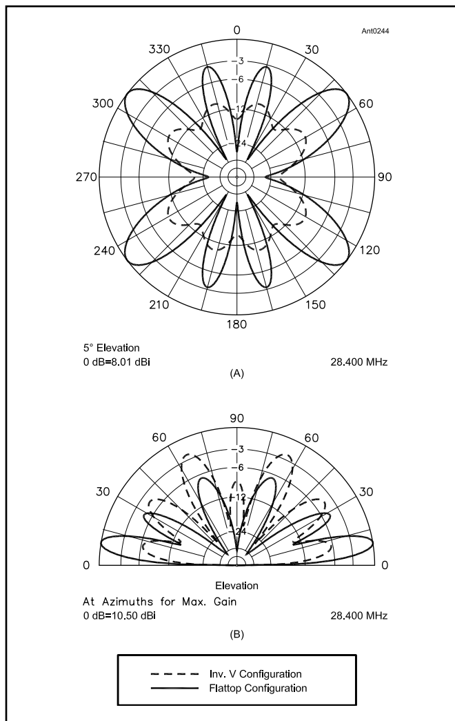
Figure 10.8 — Patterns on 10 meters for same antenna configurations as in Figs 10.6 and 10.7. Once again, the inverted V configuration yields a more omnidirectional pattern, but at the expense of almost 8 dB less gain than the flattop configuration at its strongest lobes.
