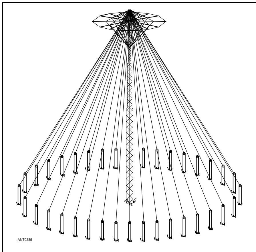
Figure 10.53 — The large W8NWF discone, designed for operation from 7 to 14 MHz, but useable with a tuning network in the shack for 3.8 MHz.
