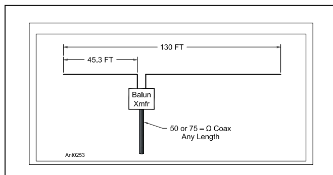
Figure 10.14 — The off-center-fed (OCF) dipole for 3.5, 7 and 14 MHz. A 1:4 or 1:6 balun is used at the feed point.
