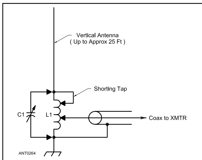
Figure 10.34 — Multiband vertical antenna system using base loading for resonating on 3.5 to 28 MHz. L1 should be wound with bare wire so it can be tapped at every turn, using #12 AWG wire. A convenient size is 2½ inches in diameter, 6 turns per inch (such as B&W 3029). Number of turns required depends on antenna and ground lead length, more turns being required as the antenna and ground lead are made shorter. For a 25-foot antenna and a ground lead of the order of 5 feet, L1 should have about 30 turns. The use of C1 is explained in the text. The smallest capacitance that will permit matching the coax cable should be used; a maximum capacitance of 100 to 150 pF will be sufficient in any case.
