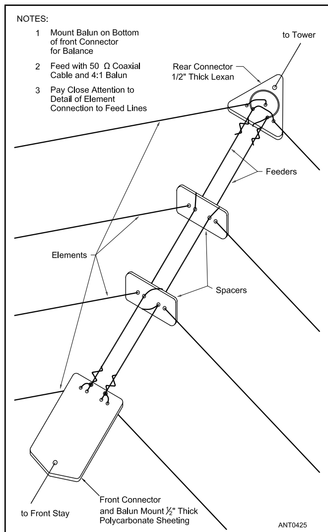
Figure 10.48 — Details of the electrical and mechanical connections of the elements to the phase-line. Knots in the nylon rope stay line are not shown.
