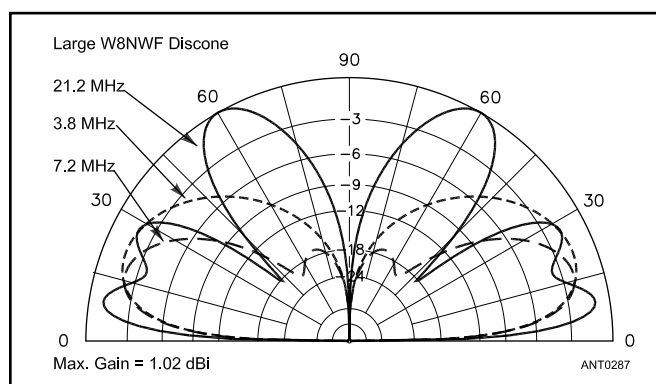
Figure 10.55 — Computed elevation-response patterns for the larger W8NWF discone for 3.8, 7.2 and 21.2 MHz operation. Again, as in Figure 10.54, the pattern degrades at 21.2 MHz, although it is still reasonably efficient, if not optimal.
