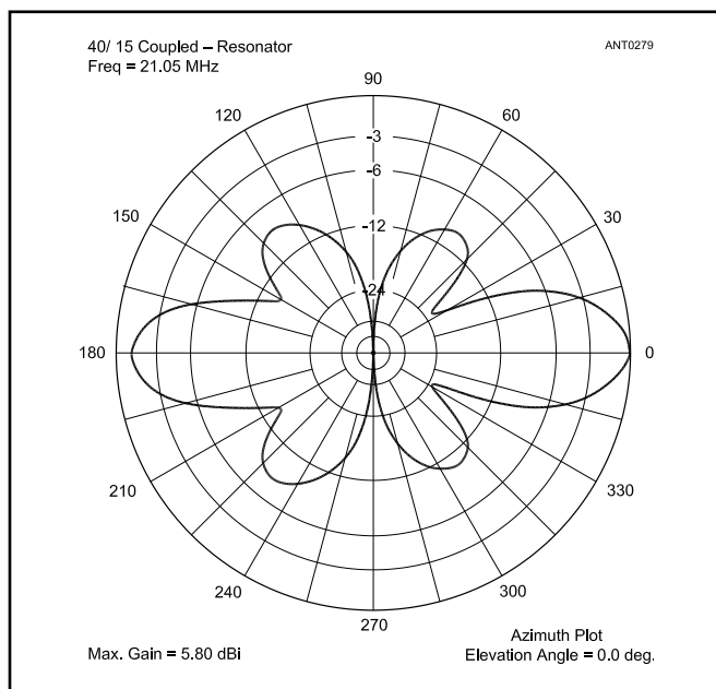
Figure 10.43 — Radiation pattern for the special case of a C-R antenna with the additional resonance at the third harmonic of the main dipole resonant frequency.
