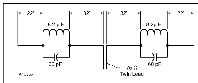
Figure 10.23 — Five-band (3.5, 7, 14, 21 and 28 MHz) trap dipole for operation with 75- \Omega feed line at low SWR (C. L. Buchanan, W3DZZ). The balanced (parallel-conductor) line indicated is desirable, but 75- \Omega coax can be substituted with a choke balun at the feed point to maintain symmetry. Dimensions given are for resonance (lowest SWR) at 3.75, 7.2, 14.15 and 29.5 MHz. Resonance is very broad on the 21-MHz band, with SWR less than 2:1 throughout the band.
