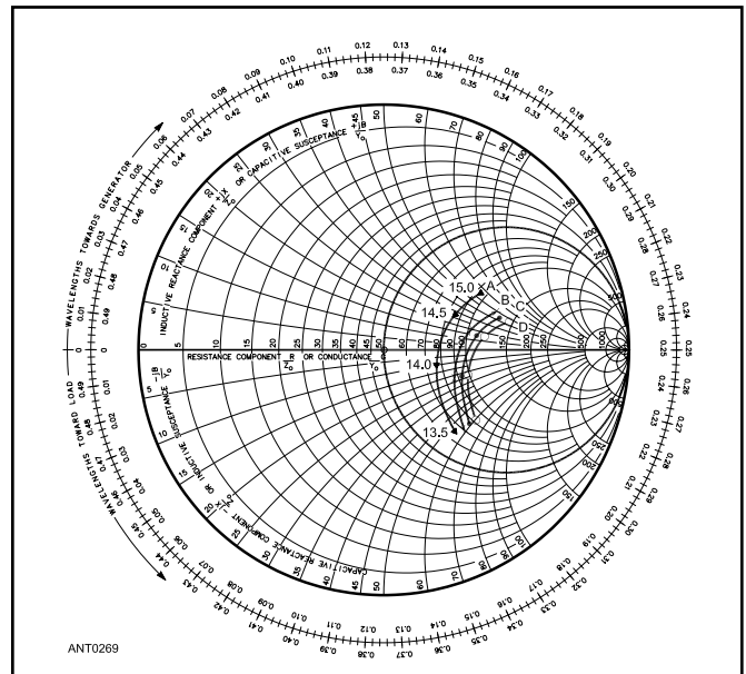
Figure 10.38 — Impedance of an open-sleeve monopole for the frequency range 13.5-15 MHz. Curve A is for a 14 MHz monopole alone. For curves B, C and D, the respective spacings from the central monopole to the sleeve elements are 8, 6 and 4 inches. See text for other dimensions.
