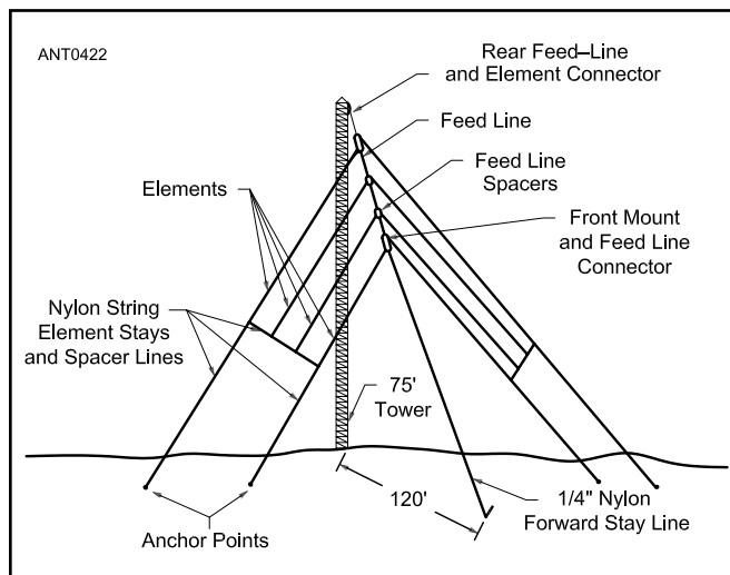
Figure 10.45 — Typical lower-HF wire 4-element log periodic dipole array erected on a tower.
