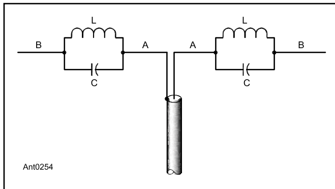
Figure 10.22 — A trap dipole antenna. This antenna may be fed with 50- \Omega coaxial line. Depending on the L/C ratio of the trap elements and the lengths chosen for dimensions A and B, the traps may be resonant either in an amateur band or at a frequency far removed from an amateur band for proper two-band antenna operation.
