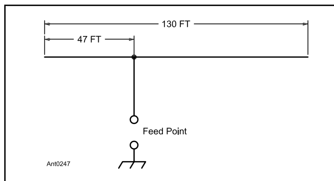
Figure 10.11 — The Windom antenna, cut for a fundamental frequency of 3.75 MHz. The single-wire feed line, connected 14% off center, is brought into the station and the system is fed against ground. The antenna is also effective on its harmonics.
