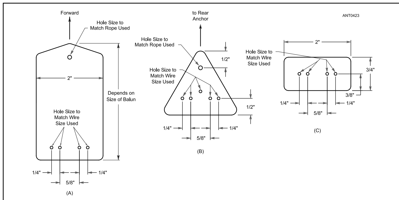
Figure 10.46 — Pieces for the LPDA that require fabrication. At A is the forward connector, made from \frac{1}{2} -inch polycarbonate. At B is the rear connector, also made from \frac{1}{2} -inch polycarbonate. At C is the pattern for the phase-line spacers, made from \frac{1}{4} -inch acrylic. Two spacers are required for the array.
