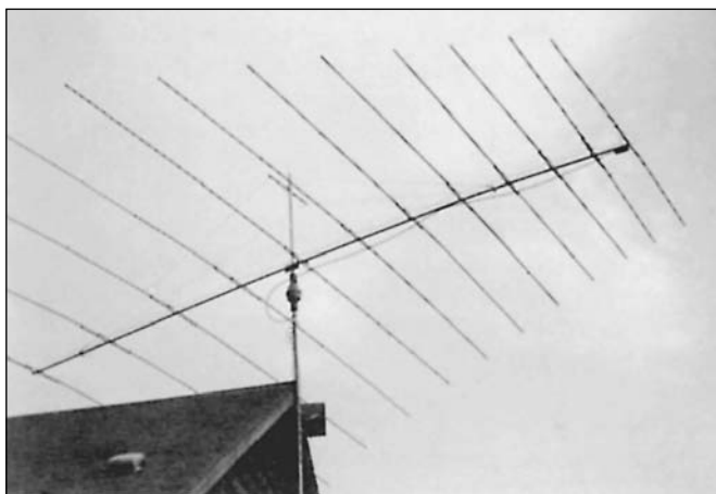
Figure 10.49 — The 13-30 MHz log periodic dipole array.
