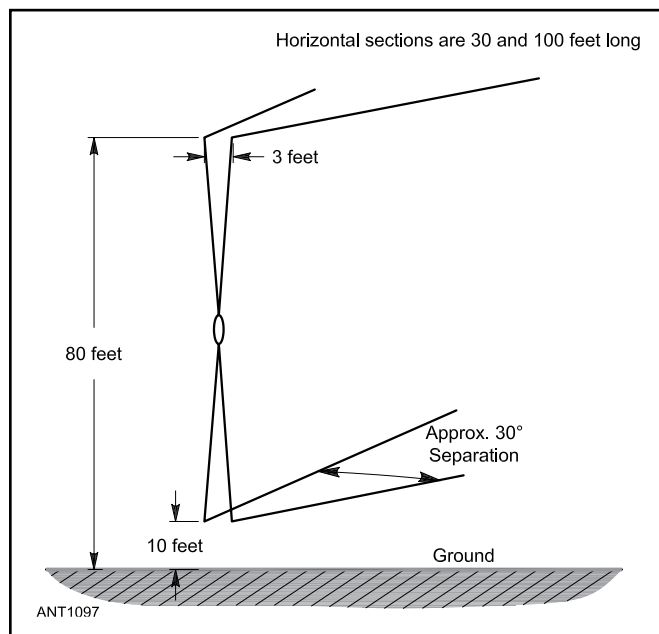
Figure 10.17 — The Double-L antenna by K2LQ is a pair of vertical dipoles with their ends bent to be parallel to the ground. The bottom horizontal wires should be at least 10 feet above ground. For single-band operation, install only a single dipole. The antenna works well as either a single-band or dual-band antenna.
