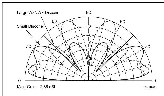
Figure 10.54 — Computed patterns showing elevation response of small discone at 28.5 MHz compared to that of the larger discone at 28.5 MHz. The cone wires are clearly too long for efficient operation on 10 meters, producing unwanted high-angle lobes that rob power from the desirable low-elevation angles.
