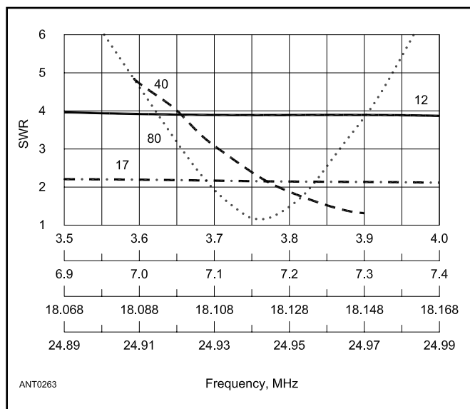
Figure 10.32 — Measured SWR curves for an 80, 40, 17 and 12 meter antenna, installed as an inverted V with 40-ft apex and 120^\circ included angle between legs.
