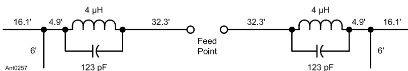
Figure 10.25 — A W8NX multiband dipole for 80, 40, 20, 15 and 10 meters. The values shown (123 pF and 4 μH) for the coaxial-cable traps are for parallel resonance at 7.15 MHz. The low-impedance output of each trap is used for this antenna.
