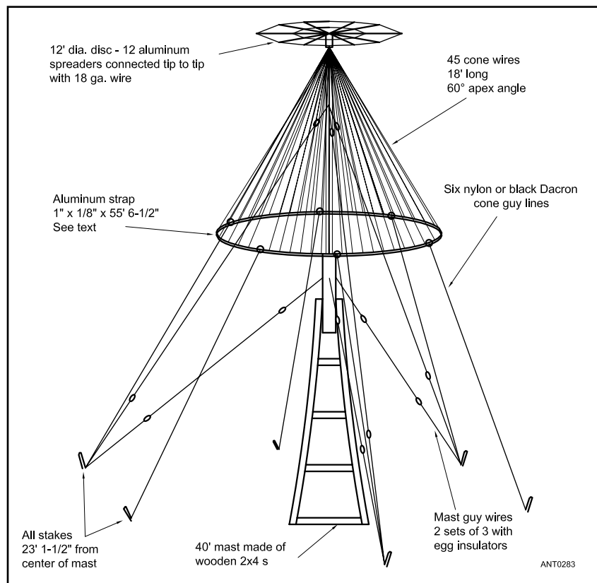
Figure 10.52 — Detailed drawing of the A-frame discone for 14 to 30 MHz. The disc assembly at the top of the A-frame is 12 feet in diameter. There are 45 cone wires, each 18 feet long, making a 60° included angle of the cone.
