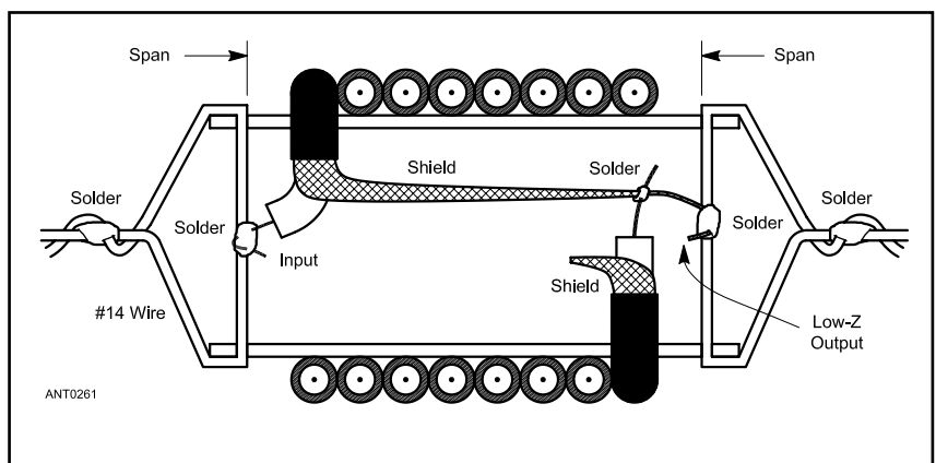
Figure 10.30 — Additional construction details for the W8NX coaxial-cable trap.
