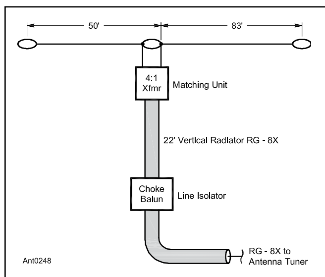
Figure 10.12 — Layout for flattop “Carolina Windom” antenna.
