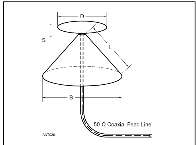
Figure 10.51 — Diagram of VHF/UHF discone, using a sheet-metal disc and cone. It is fed directly with 50-Ω coax line. The dimensions L and D, together with the spacing S between the disc and cone, determine the frequency characteristics of the antenna. L = 246 / f_{\text{MHz}} for the lowest frequency to be used. Diameter D should be from 0.67 to 0.70 of dimension L. The diameter at the bottom of the cone B is equal to L. The space S between disc and cone can be 2 to 12 inches, with the wider spacing appropriate for larger antennas.
