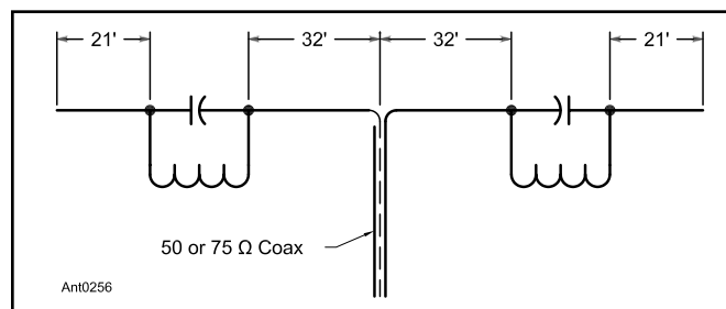
Figure 10.24 — Layout of multiband antenna using traps constructed as shown in Figure 10.25. The capacitors are 100 pF each, transmitting type, 5000-volt dc rating (Centralab 850SL-100N). Coils are 9 turns of #12 AWG wire, 2-1/2 inches diameter, 6 turns per inch (B&W 3029) with end turns spread as necessary to resonate the traps to 7.2 MHz. These traps, with the wire dimensions shown, resonate the antenna at approximately the following frequencies on each band: 3.9, 7.25, 14.1, 21.5 and 29.9 MHz (based on measurements by W9YJH).
