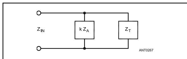
Figure 10.36 — Equivalent circuit of an open-sleeve antenna.
