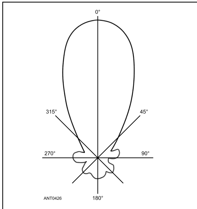
Figure 10.50 — Measured radiation pattern of the 13-30 MHz LPDA. The front-to-back ratio is about 14 dB at 14 MHz and increases to 21 dB at 28 MHz.
