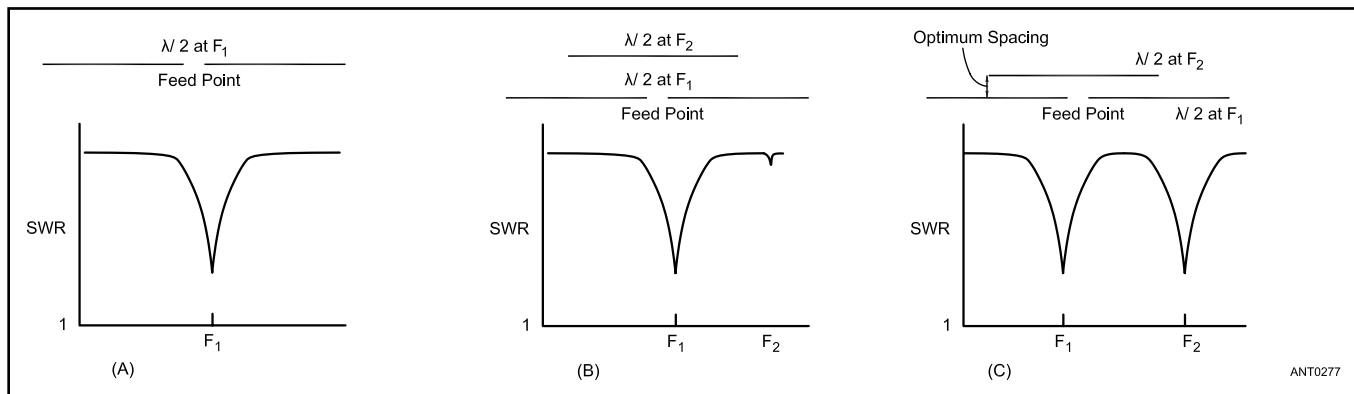
Figure 10.41 — At A, the SWR of a dipole over a wide frequency range. At B, a nearby conductor is just close enough to interact with the dipole. At C, when the second conductor is at the optimum spacing, the combination is matched at both frequencies.
