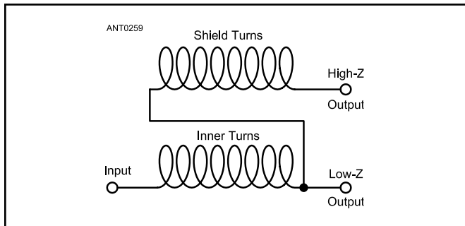
Figure 10.27 — Schematic for the W8NX coaxial-cable trap. RG-59 is wound on a 2 \frac{3}{8} -inch OD PVC pipe.
