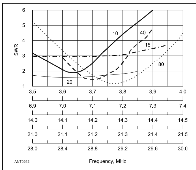
Figure 10.31 — Measured SWR curves for an 80, 40, 20, 15 and 10 meter antenna, installed as an inverted V with 40-ft apex and 120^\circ included angle between legs.
