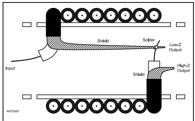
Figure 10.28 — Construction details of the W8NX coaxial-cable trap.
