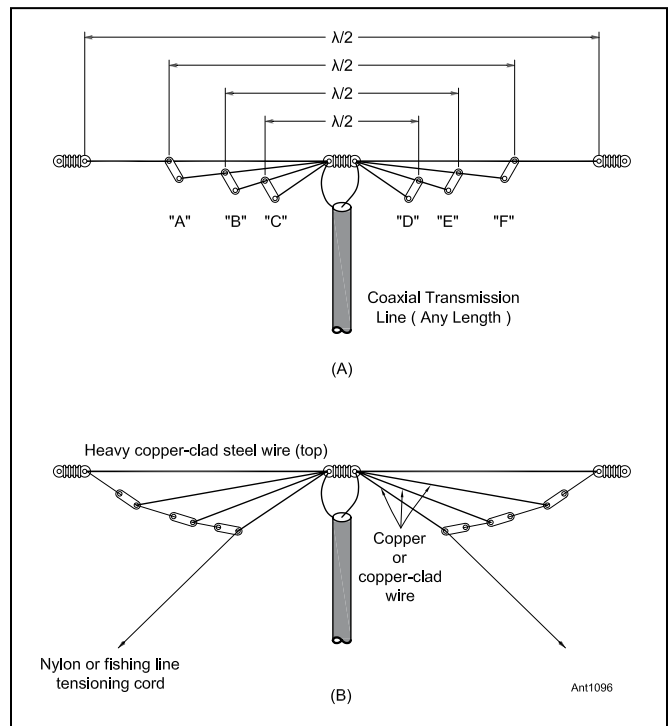
Figure 10.15 — At A, multiband antenna using paralleled dipoles all connected to a common low-impedance transmission line. The half-wave dimensions may be either for the centers of the various bands or selected to fit favorite frequencies in each band. Because of interaction among the various dipoles, the builder should expect to adjust lengths for resonance on each band. B shows a method of constructing the dipole that offers less interaction between the dipoles, making it easy to tune.
