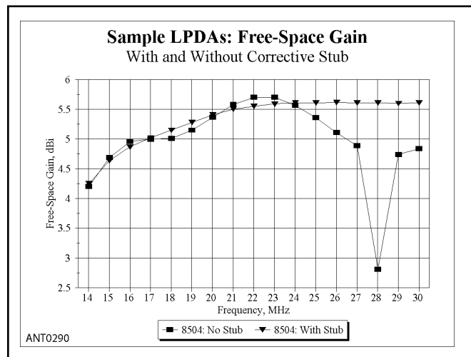
Figure 7.8 — A graph of the gain of model “8504” showing the frequency region in which a “weakness” occurs and its absence once a suitable stub is added to the array.
