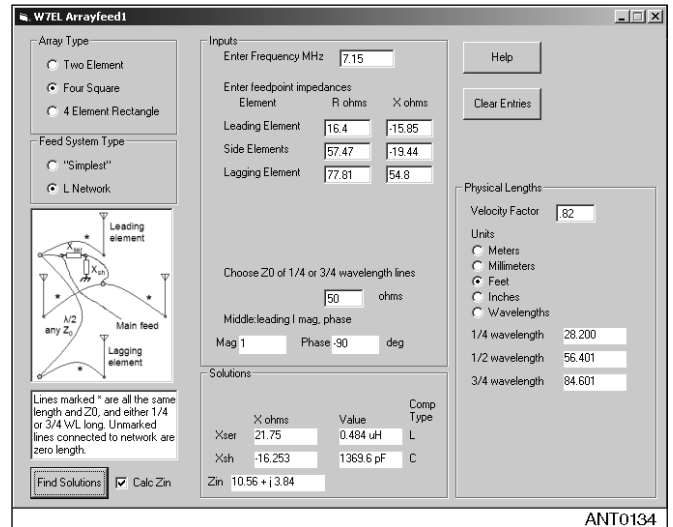
Figure 6.27 — L network setup for Four-Square array in Figure 6.25, fed with \lambda/4 (or 3\lambda/4 ) current-forcing feed system.
