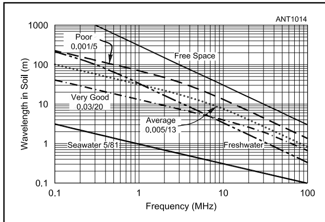
Figure 3.8 — Wavelength in typical soils as a function of frequency.
