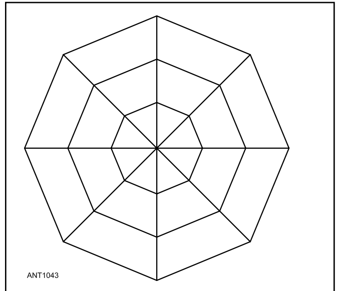
Figure 3.35 — Example of a wire counterpoise ground system.
