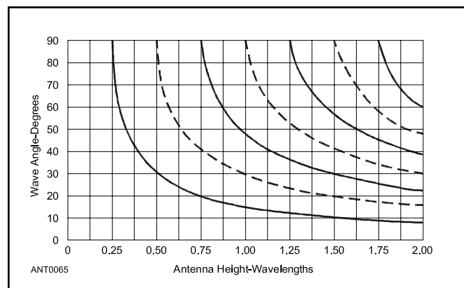
Figure 3.49 — Angles at which nulls and maxima (factor = 6 dB) in the ground-reflection factor appear for antenna heights up to two wavelengths over flat ground. The solid lines are maxima, dashed lines nulls, for all horizontal antennas. See text for examples. Values may also be determined from the trigonometric relationship \theta = \arcsin(A/4h) , where \theta is the wave angle and h is the antenna height in wavelengths. For the first maximum, A has a value of 1; for the first null A has a value of 2, for the second maximum 3, for the second null 4, and so on.
