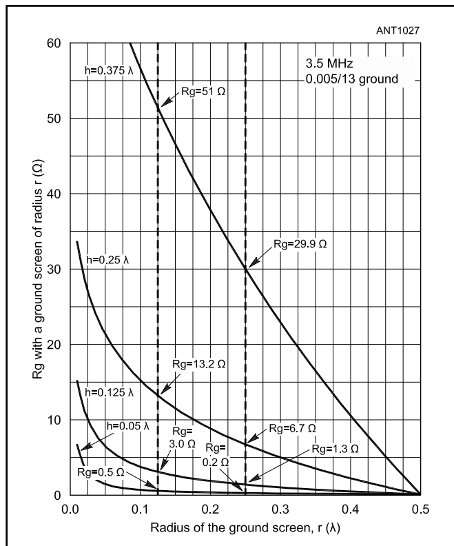
Figure 3.19 — Variation in R_g with ground screen radius. Normalized to include losses out to r = 0.5 \lambda .
