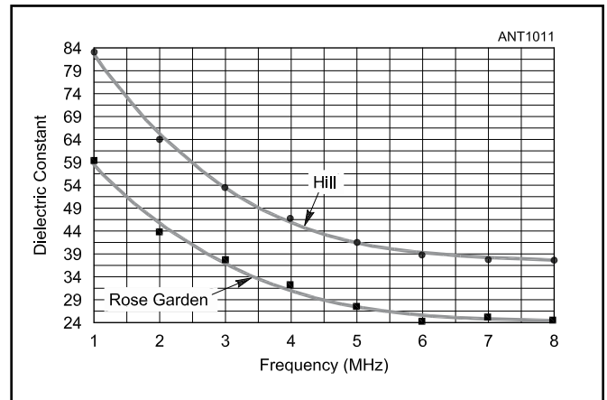
Figure 3.4 — Typical soil permittivity variation with frequency.
