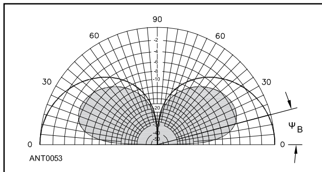
Figure 3.39 — Vertical-plane radiation pattern for a ground-mounted half-wave vertical. The solid line is the pattern for perfect earth. The shaded pattern shows how the response is modified over average earth ( k = 13 , G = 0.005 S/m) at 14 MHz. \psi is the pseudo-Brewster angle (PBA), in this case 14.8°.
