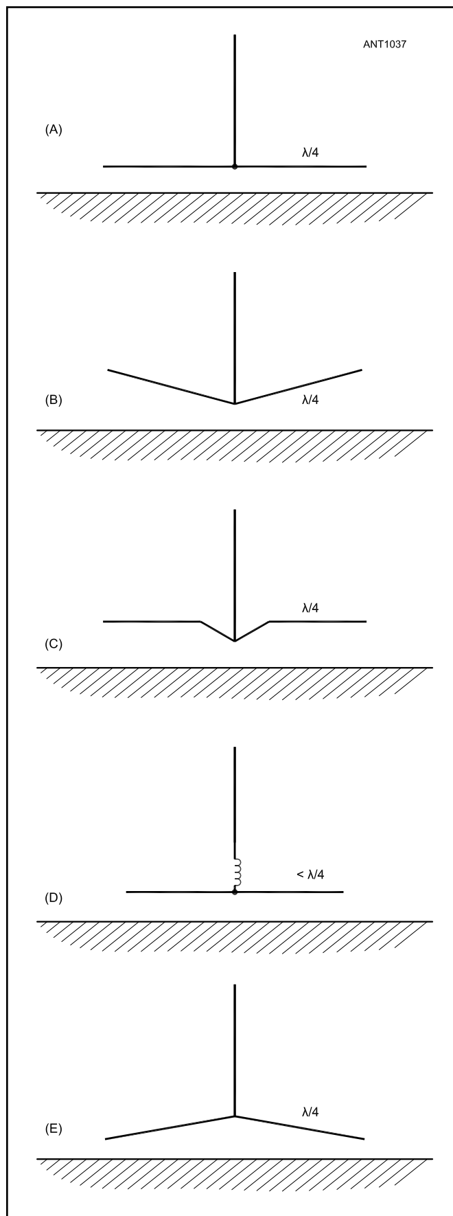
Figure 3.29 — Alternate elevated ground system configurations.
