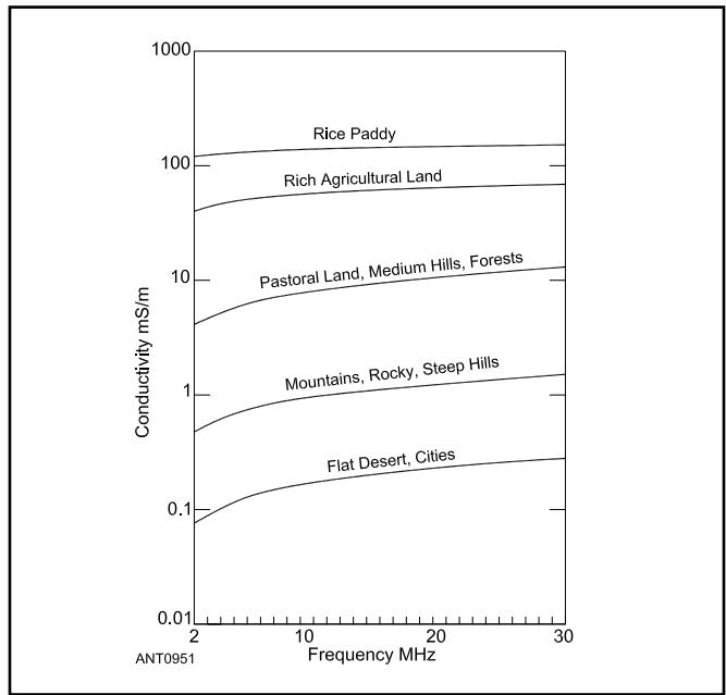
Figure 3.52 — Typical terrain conductivities versus frequency for 5 types of soils. This was measured by SRI. Units are mS/m. Conductivity of seawater is usually taken as 5000 mS/m. Conductivity of fresh water depends on the impurities present, and may be very low. To extrapolate conductivity values (for 500 to 1500 kHz) shown in Figure 3.2 for a particular geographic area to a different frequency, move from the conductivity at the left edge of this figure to the desired frequency. For example, in rocky New Hampshire, with a conductivity of 1 mS/m at BC frequencies, the effective conductivity at 14 MHz would be approximately 4 mS/m.
