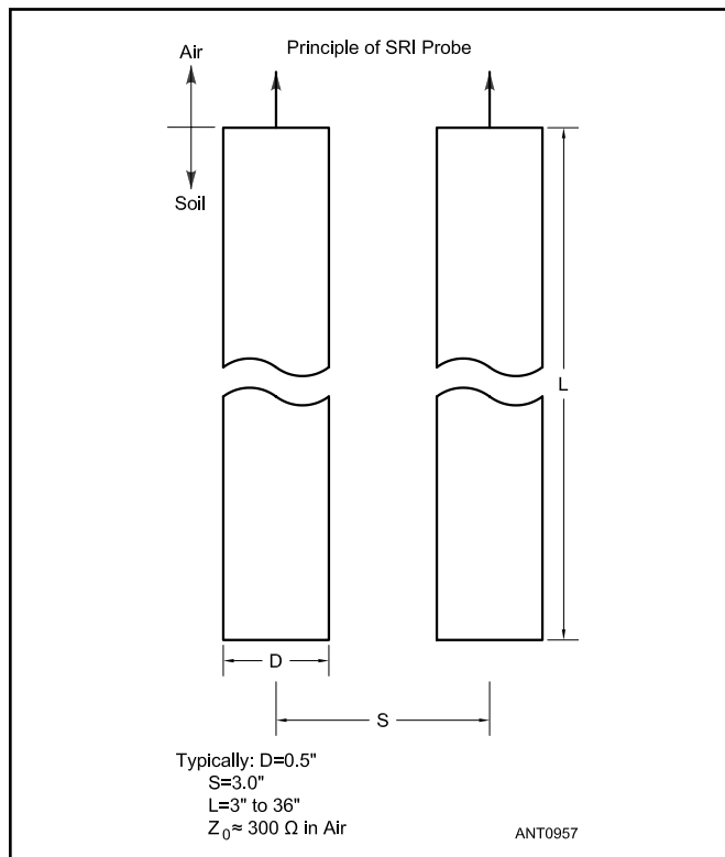
Figure 3.58 — High-frequency conductivity/dielectric constant measurement system. System for measuring ground conditions at frequencies up to about 100 MHz, devised by SRI and used to obtain the data in Figures 3.52 through 56. Basically, this is a section of transmission line with soil as the dielectric. Requires measurement of high impedances to good accuracy.
