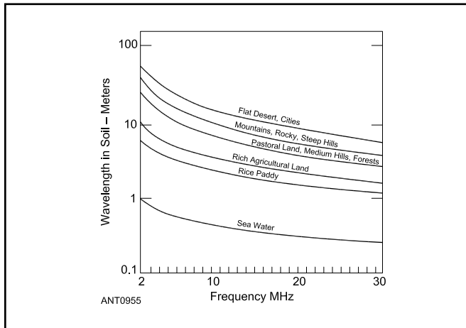
Figure 3.56 — Typical values of wavelength in soil. Because of its dielectric constant, the wavelength in soils and water will be shorter than that for a wave traveling in air. This can be important, since in a Method of Moment the accuracy is affected by the number of analysis segments per wavelength. Depending on the program being used, adjust the number of segments for antennas wholly or partly in the earth, for ground rods, and for antennas very close to earth.
