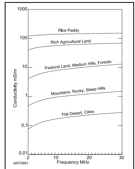
Figure 3.5 — Ground conductivity variation with frequency for different types of soils.
