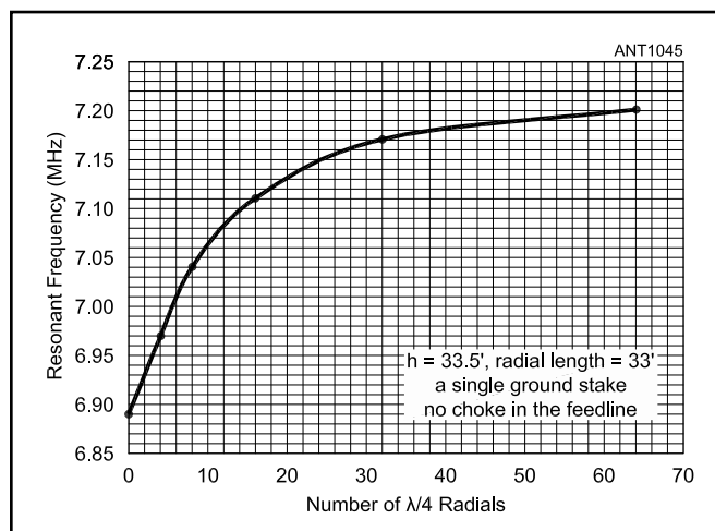
Figure 3.37 — A typical example of the effect on resonant frequency as the number of ground surface radials is varied.
