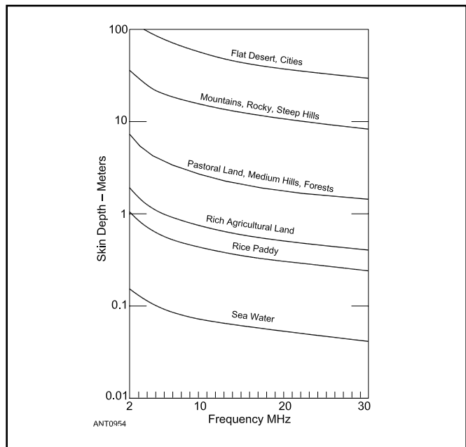
Figure 3.55 — Typical values of skin depth. The skin depth is the depth at which a signal will have decreased to 1/e of its value at the surface (to about 30%). The effective height above ground is essentially the same as the physical height for sea water, but may be much greater for the desert. For practical antennas, this may increase low-angle radiation, but at the same time will increase ground losses.
