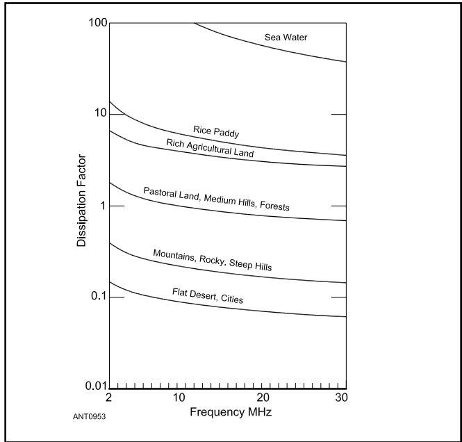
Figure 3.54 — Typical values of dissipation factor. The soil behaves as a leaky dielectric. These curves showing the dimensionless dissipation factor versus frequency for various types of soils and for sea water. The dissipation factor is inversely related to soil conductivity. Among other things, a high dissipation factor indicates that a signal penetrating the soil or water will decrease in strength rapidly with depth.
