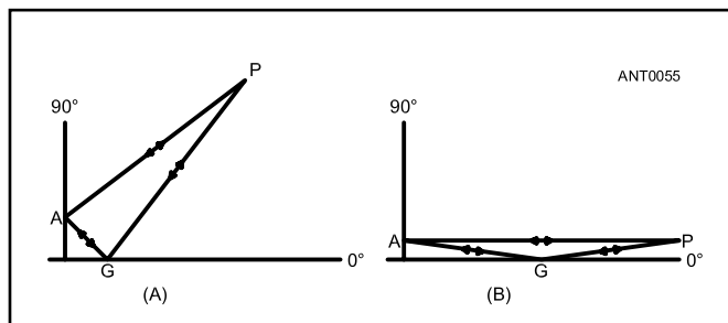
Figure 3.41 — The direct wave and the reflected wave combine at point P to form the pattern (P is very far from the antenna). At A the two paths AP and AGP differ appreciably in length, while at B these two path lengths are nearly equal.
