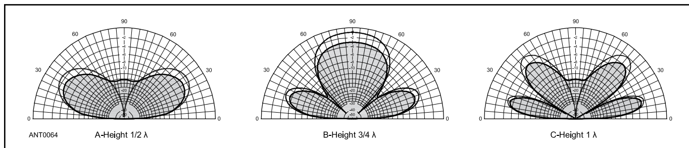
Figure 3.48 — Vertical-plane radiation patterns of half-wave horizontal dipole antennas at 45^\circ from the antenna wire over flat ground. The solid-line and shaded curves represent the same conditions as in Figures 3.46 and 3.47. These patterns are scaled so they may be compared directly with those of Figures 3.46 and 3.47.
