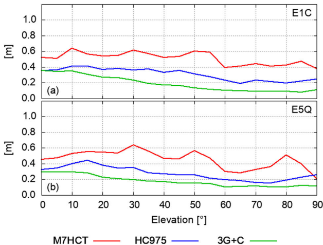
Figure 4: Elevation dependent RMS(MP) of signals E1C and E5Q.
