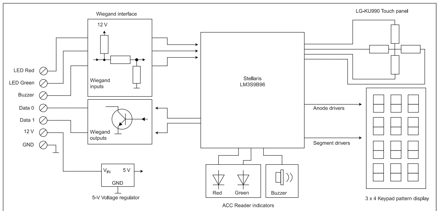
Figure 1 —The block diagram of the device reflects the typical structure of an AC PIN reader. The keypad pattern display and the touch panel are, in this case, substituted for a 3 \times 4 push button array of a standard PIN reader.
