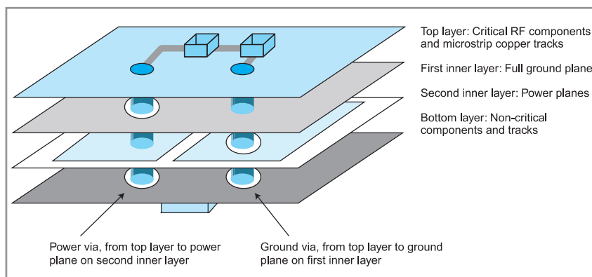
Figure 1 —Using a four-layer PCB is the easiest solution for a good grounding structure. Usually, the first inner layer is devoted to a full ground plane. The top layer, just above the ground plane, is used for all critical RF components and microstrip tracks. The second inner layer is used for power supplies. And lastly, the bottom layer can be used for less critical components and tracks.
