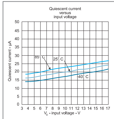
Figure 3 —Input voltage versus quiescent current of the TPS62110
