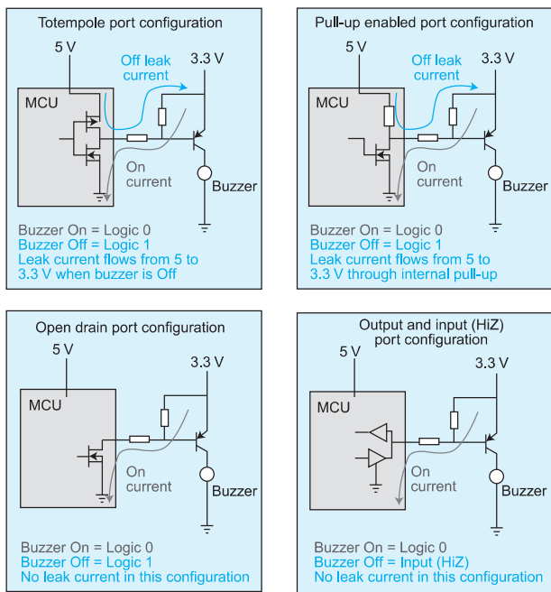
Figure 9—Mixed-signal interfacing current paths
