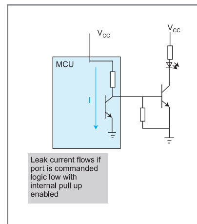
Figure 7—A simple LED driving circuit that could complicate things if the MCU is not properly configured
