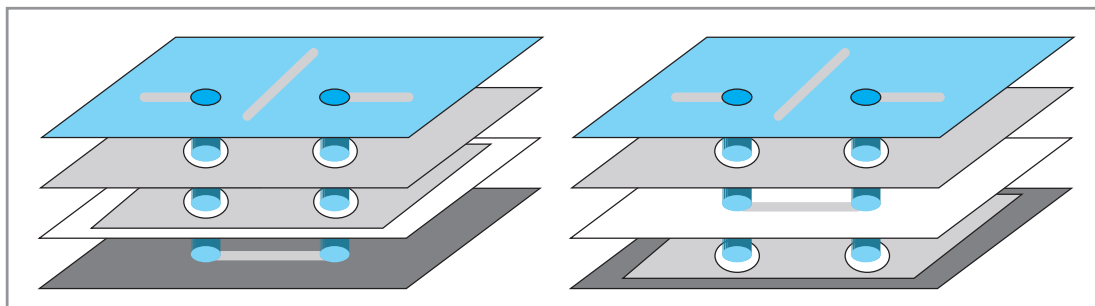
Figure 5 —These figures show you two alternatives when you absolutely must have two RF tracks crossing each other: either through the bottom layer (left) or through a stripline on the second inner layer (right). In both cases, plenty of vias should be used to avoid RF leakage.
