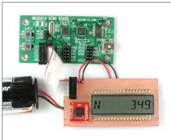
Photo 1 —A Maxim MAXQ610 microcontroller, a custom board containing the magnetic sensor, an LCD, and a display driver provide all of the necessary functions for a digital compass.
