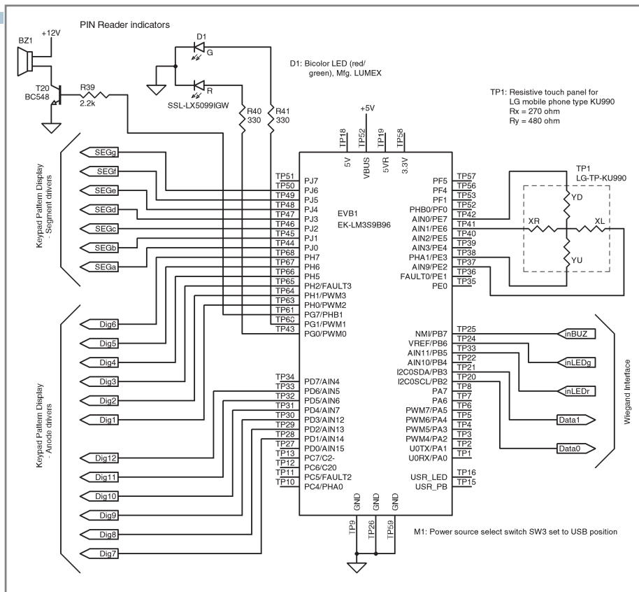
Figure 2 —The DK-LM359B96 evaluation board is powered via a VBU5 pin; therefore, the power select switch on the module has to be set to the U5B position. Otherwise, a power supply voltage of 5 V may be shorted to a power supply provided by the in-circuit debug interface board.
