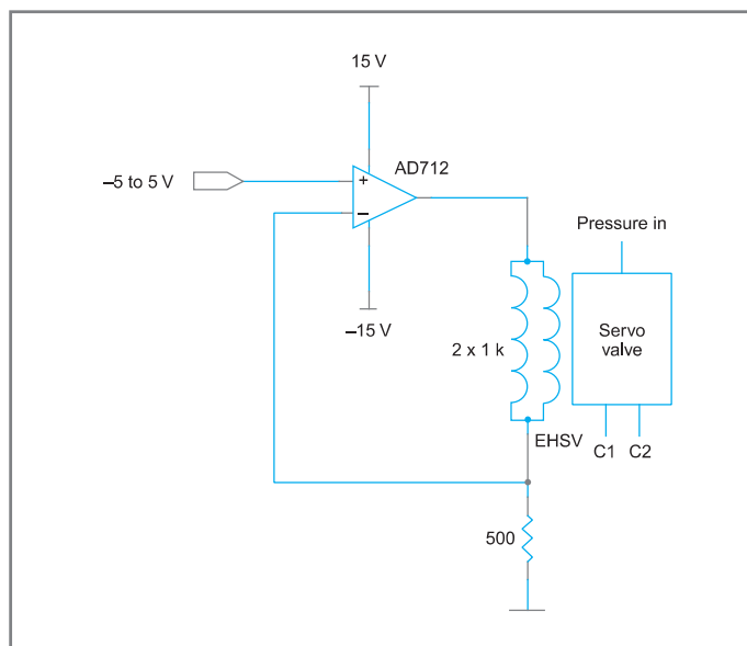
Figure 2—EHSV current driver
