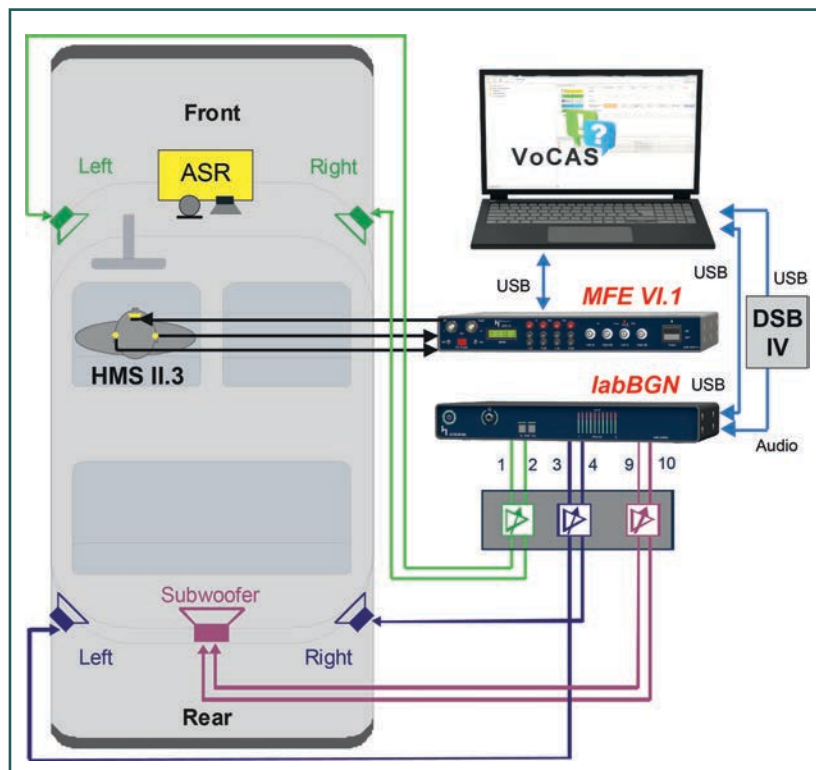
Figure 2: The test setup for ASR systems in vehicles includes necessary components for background noise simulation as well as playback and equalization.
