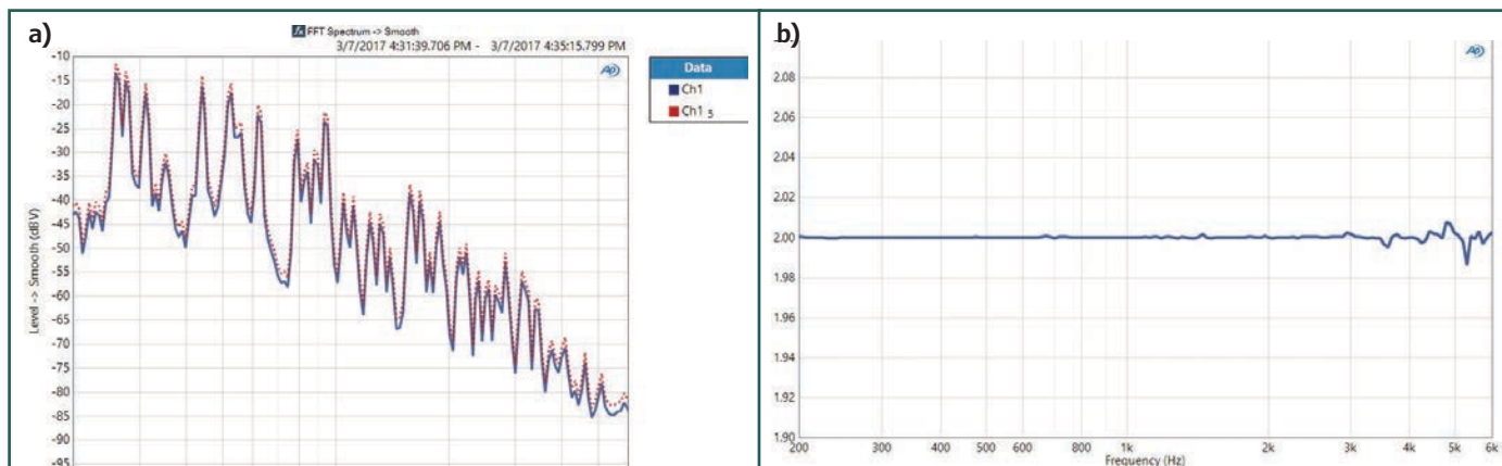
Figure 16: (a) Here we compare the frequency spectrum of transient portion of piano chord at -5 dBV (THD at -105 dB) and -3 dBV (THD at -34 dB). (b) Despite huge difference in THD, changes in frequency characteristics of transient portion of piano chord are negligible.
