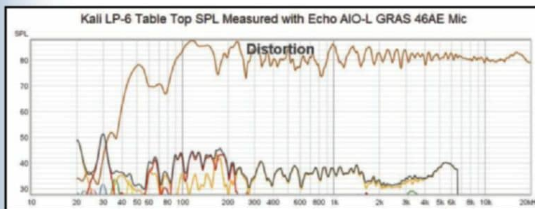
Figure 4: Using the AIO-L module and an ICP/CCP mic, I was getting good acoustic data from an active speaker within minutes.
