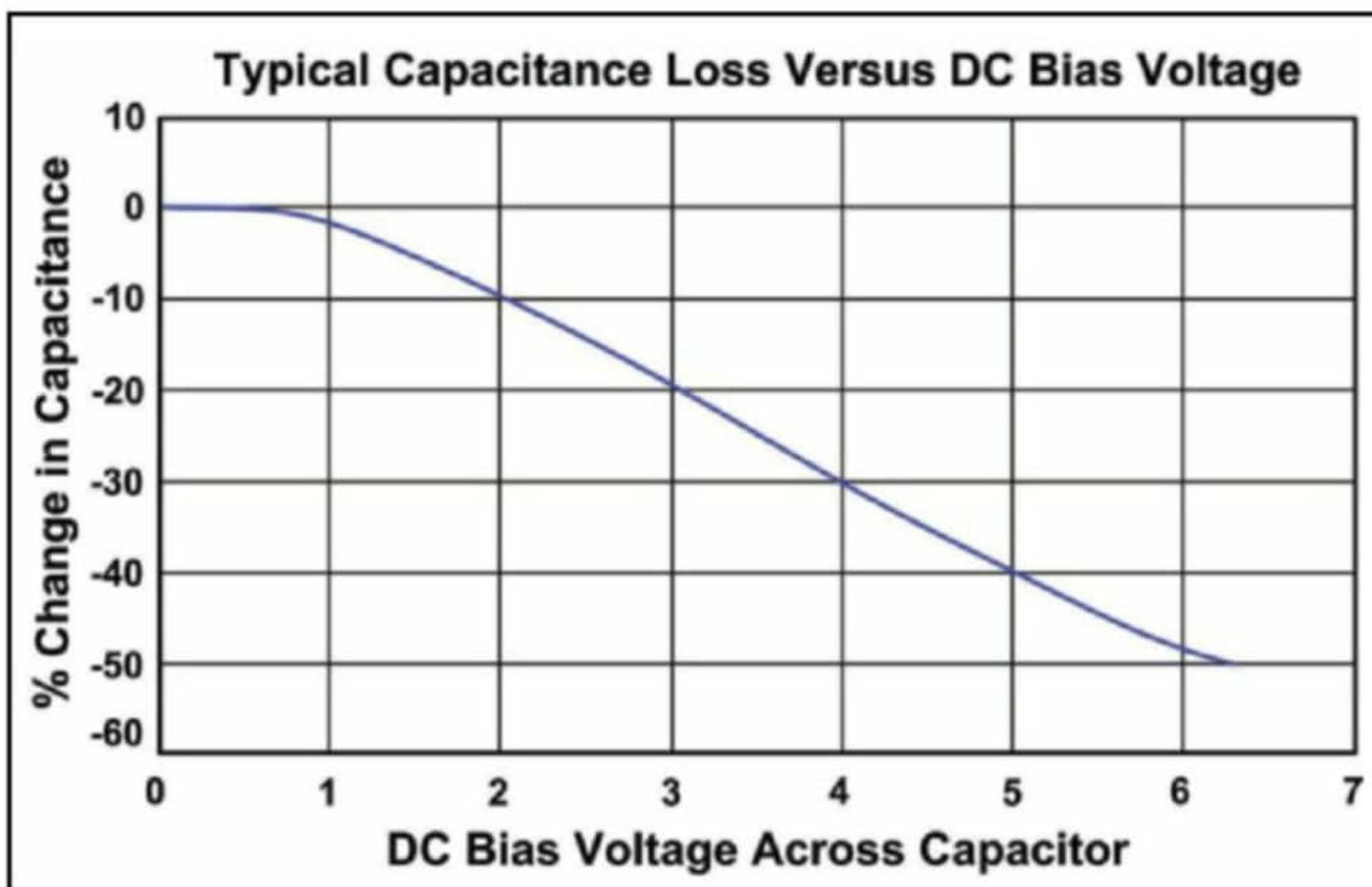
Figure 12: With Class 2 and Class 3 ceramic capacitors, their capacitance reduces as the applied DC bias voltage increases.
