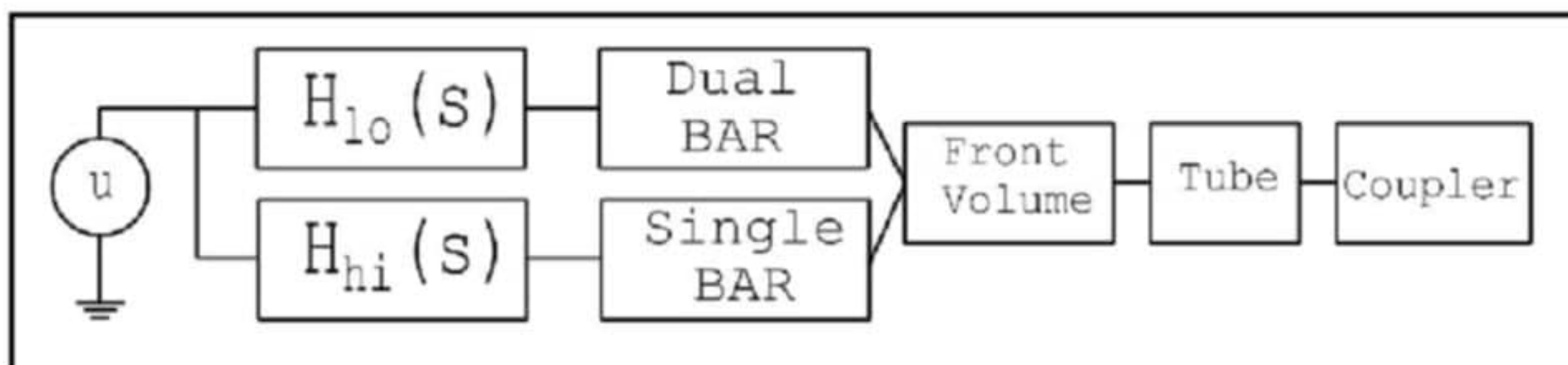
Figure 8: Block diagram for connecting the lumped element circuits
