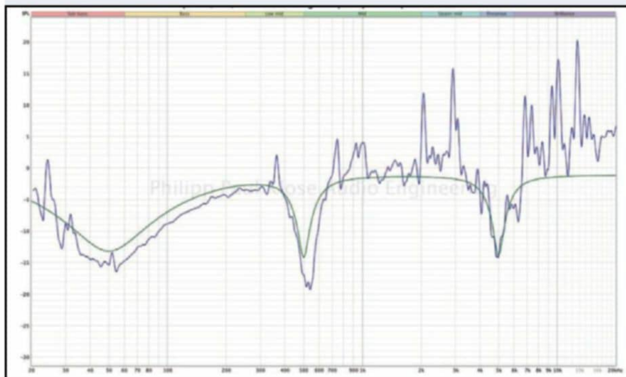
Figure 1: Filter reconstruction measurement. In the acoustical sound field, the applied filter (green) vs. the reconstructed filter from one microphone data point (blue). Errors in the high-frequency band up to 20dB.
