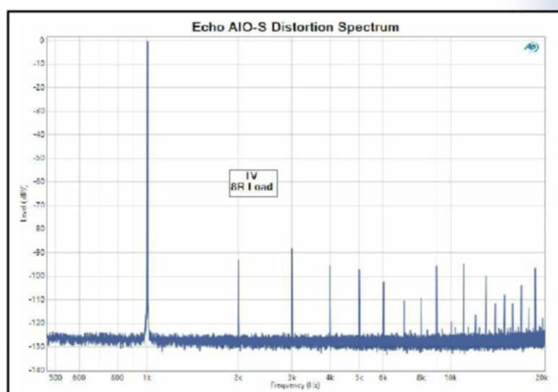
Figure 11: The output distortion spectrum of the AIO-S amplifiers at 1V and 1kHz is dominated by the third harmonic.
