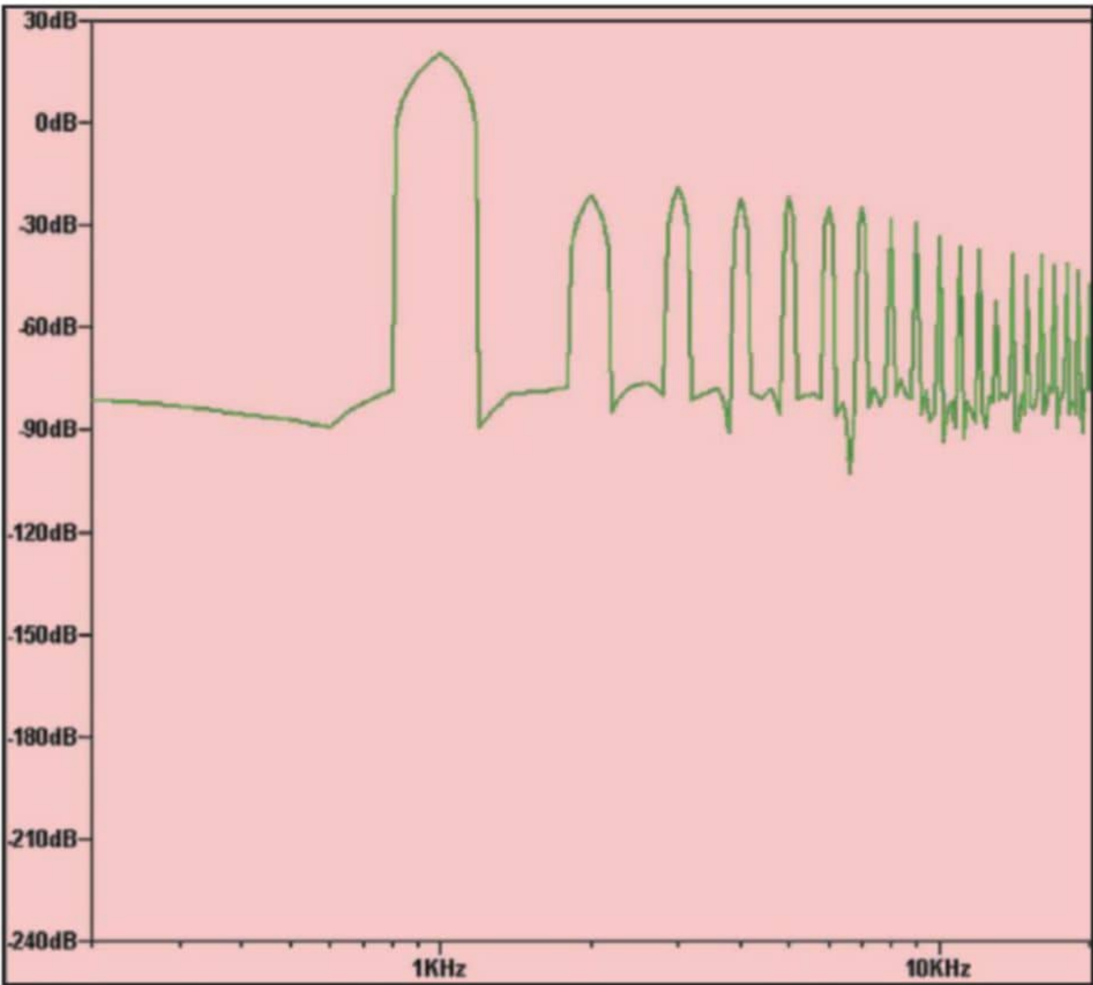
Figure 4: Third-harmonic distortion predominates.
