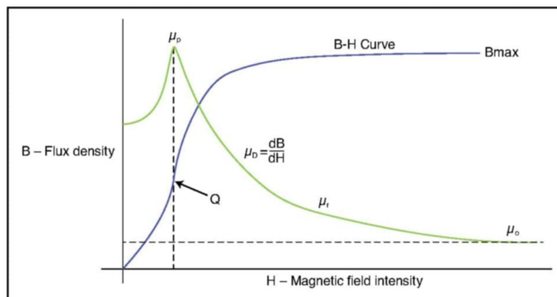
Figure 12: Differential permeability vs. magnetic field intensity (Image Source: COMSOL)
