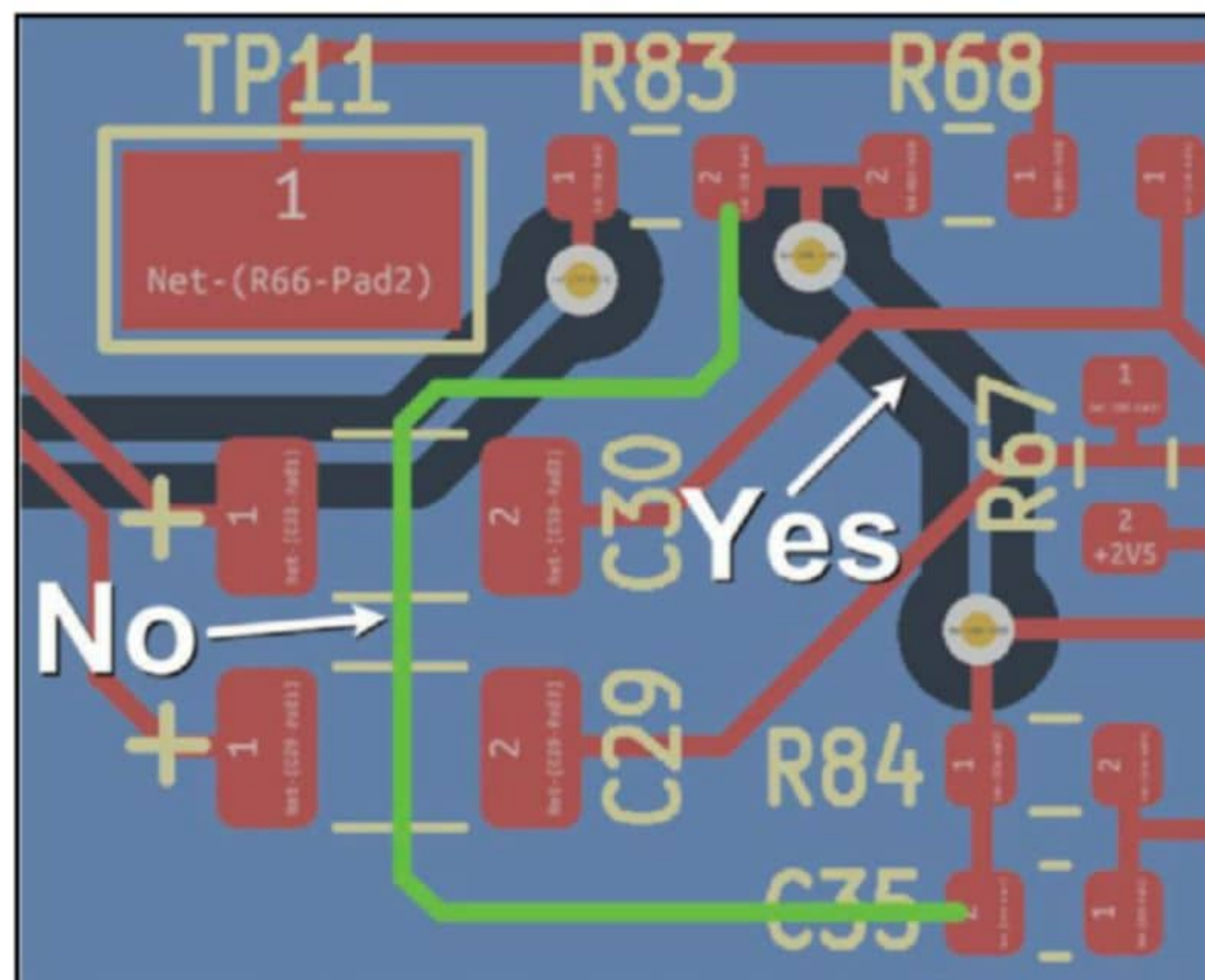
Figure 11: Short runs are always better than long runs, even when vias are needed to get to a trace on the bottom layer.
