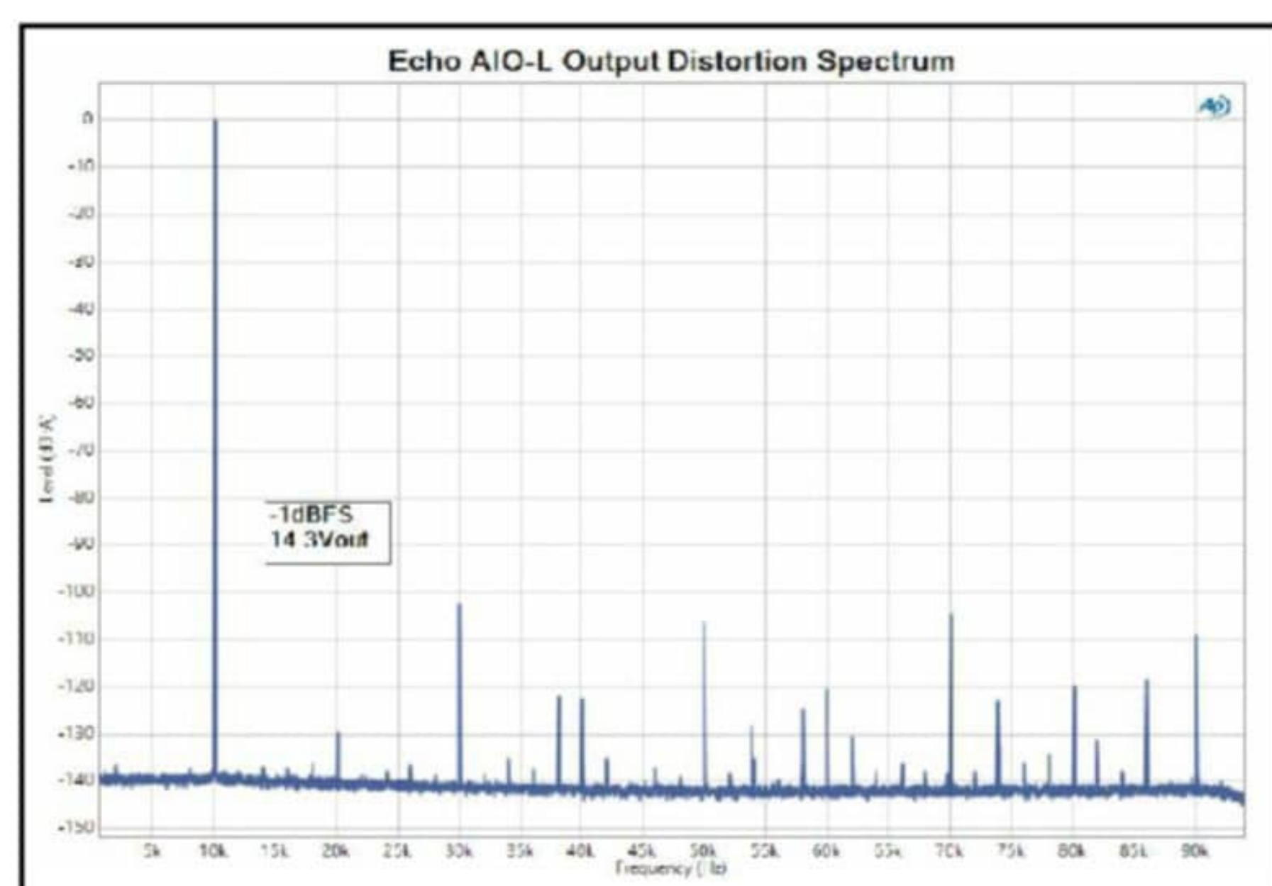
Figure 9: Raising the frequency to 10kHz shows no large distortion rise for the AIO-L module output even at near limiting voltage.
