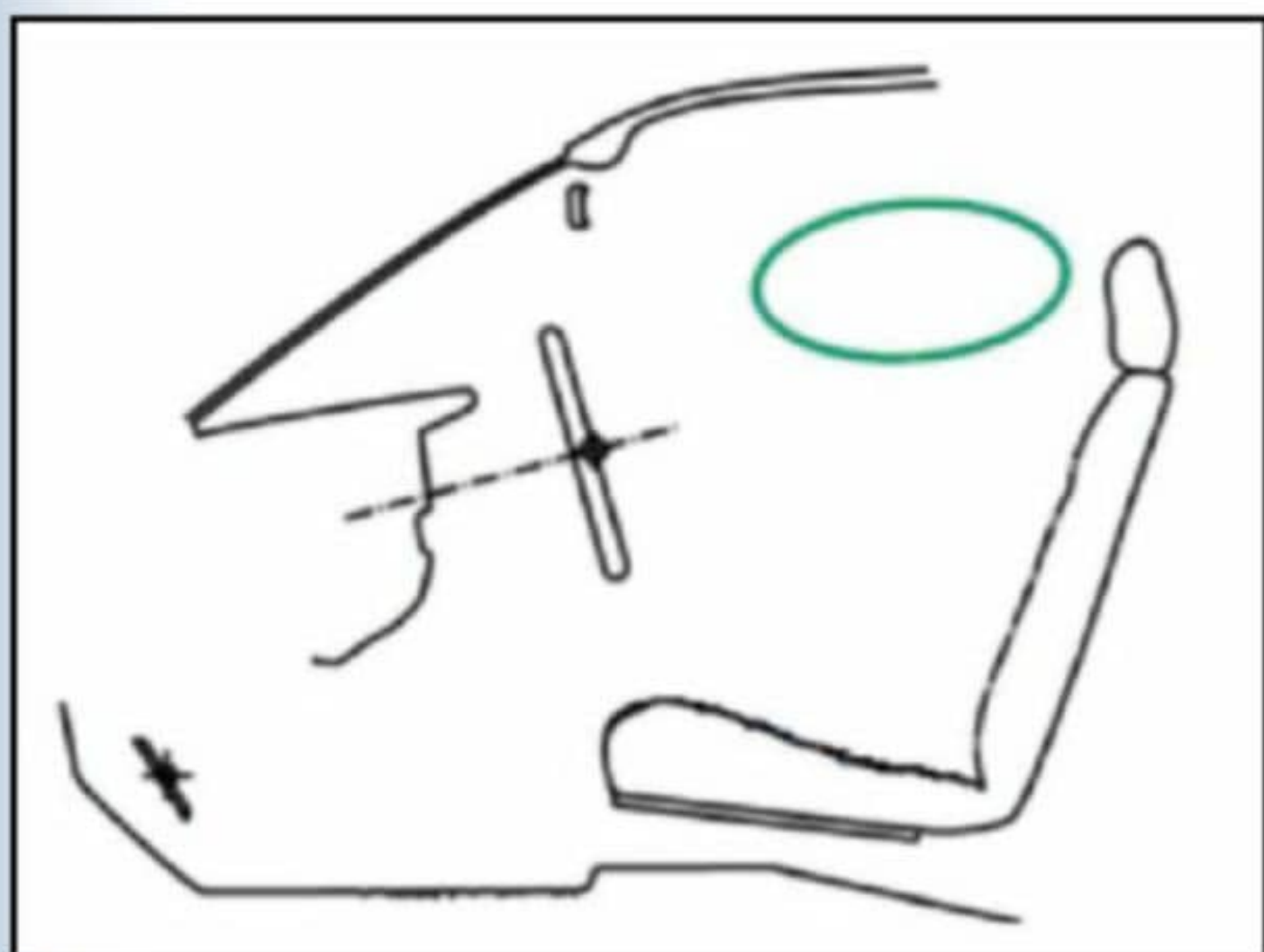
Figure 2: Geddes discovered that six equally spaced microphones placed where the ears of potential customers are (from small to very big persons, in the so-called “ear ellipsoid”) with their data points averaged, gives the best measurement result in the cars in terms of resolution, accuracy, reproducibility, and coherence with personal perception. (Image Source: Adjustment of Auditory Displays for Driver Assistance Systems by Strauß, Treichel, Kessler)
