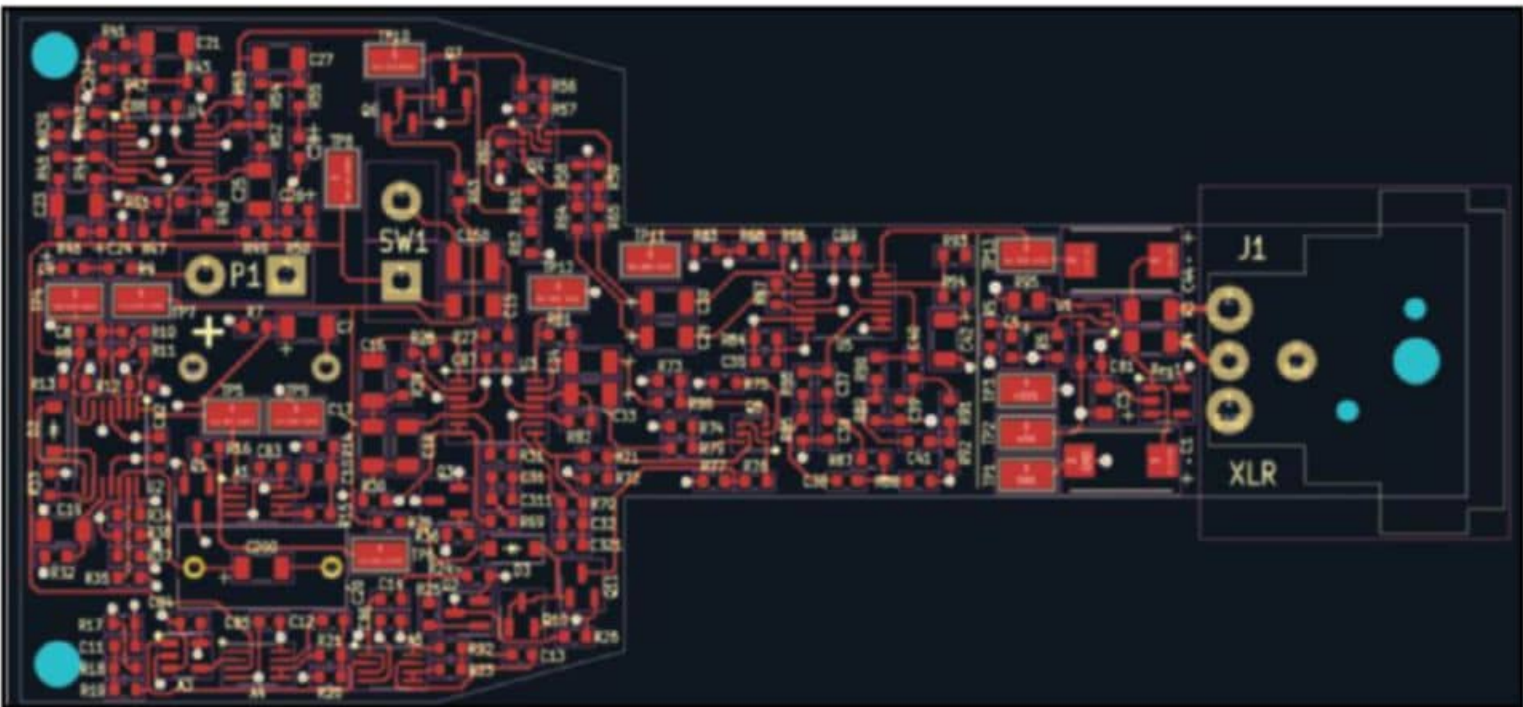
Figure 8: The top copper layer as seen in KiCad holds the solder pads needed for every SMD component, along with the traces that connect them.
