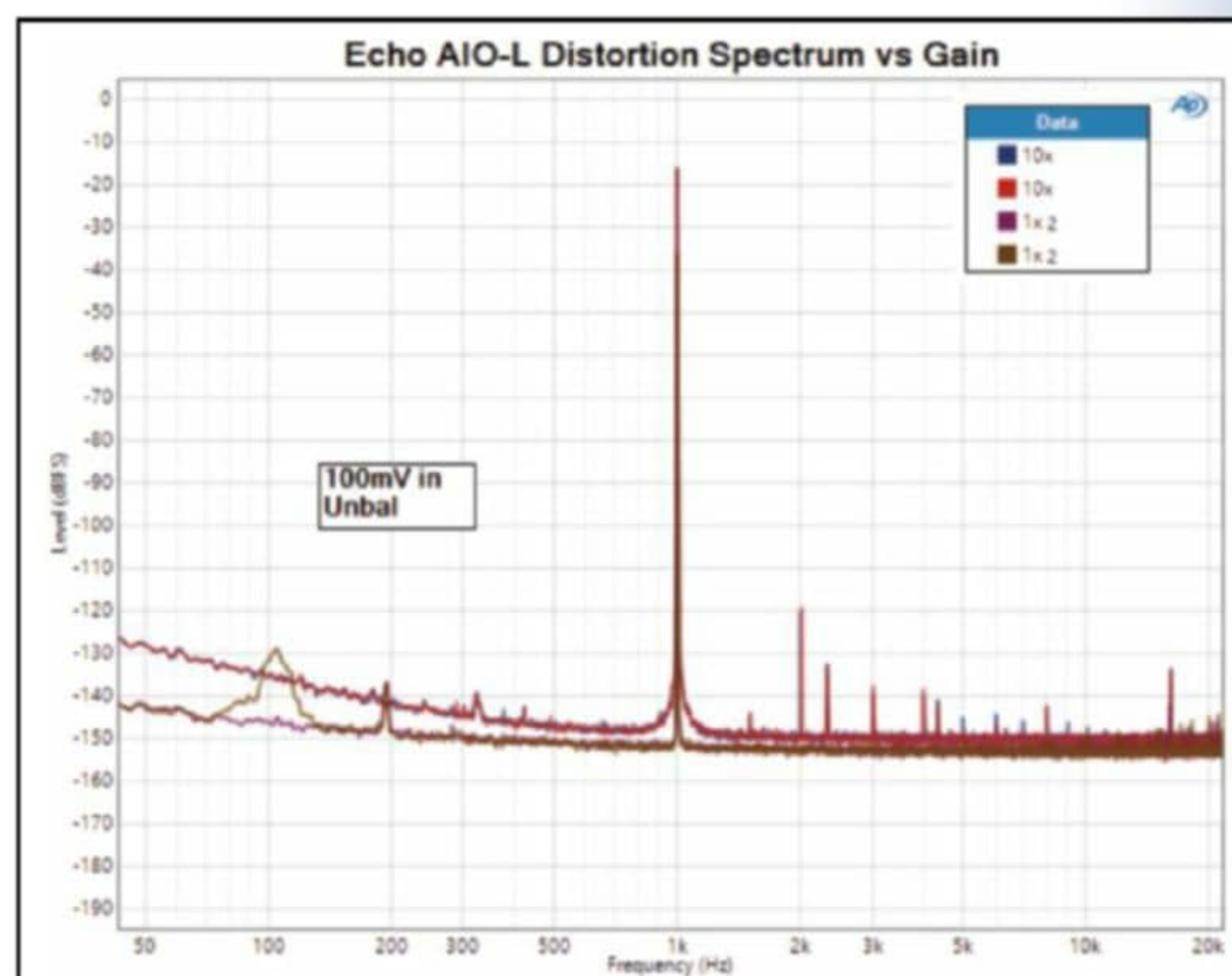
Figure 10: The input distortion of the AIO-L rises slightly with higher gain settings.
