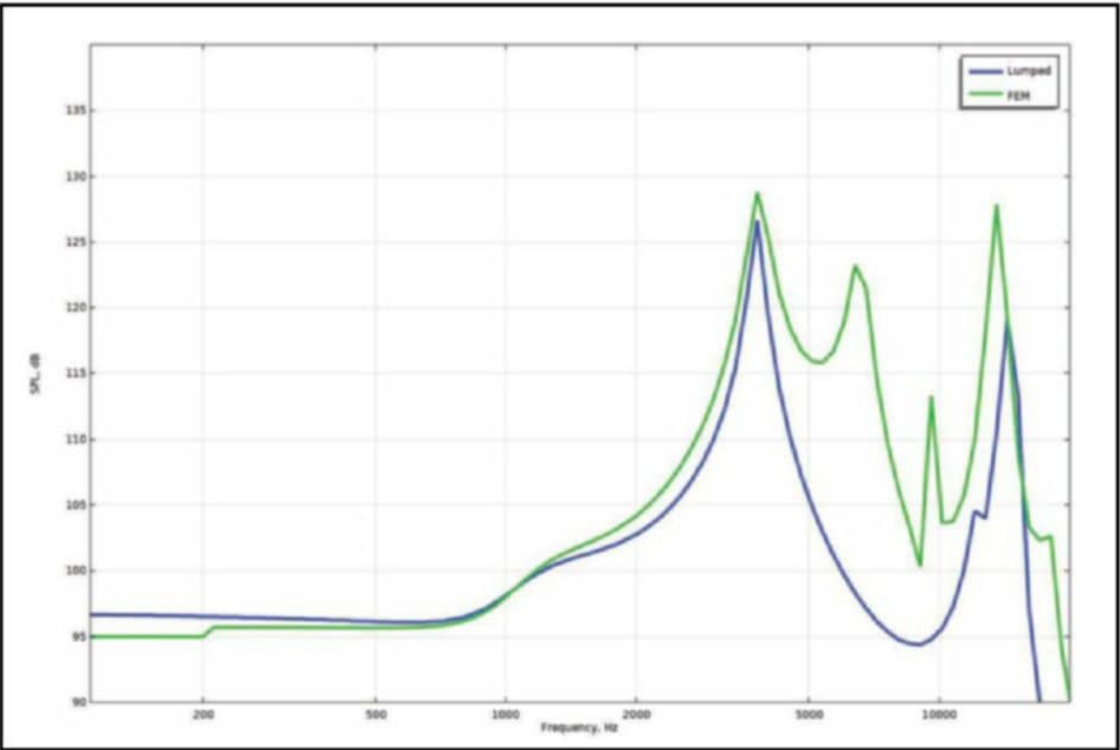
Figure 6: Sound pressure level in the coupler for the lumped model and the finite element model
