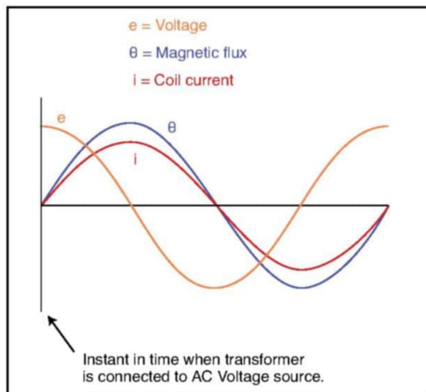
Figure 13: Transformer current when the AC voltage reaches its peak (Image Source: All About Circuits)
