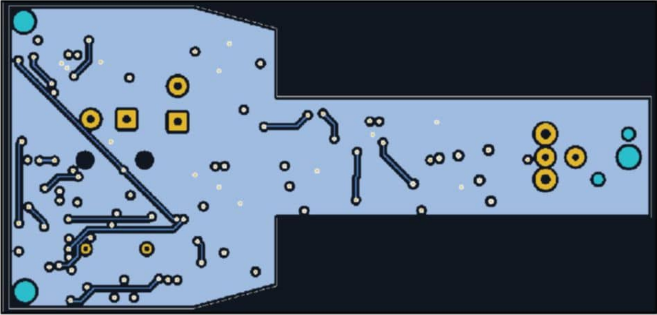
Figure 9: The bottom layer of this board is filled solid to carry the V/2 half-supply around the board, plus a few traces that couldn’t go on top.
