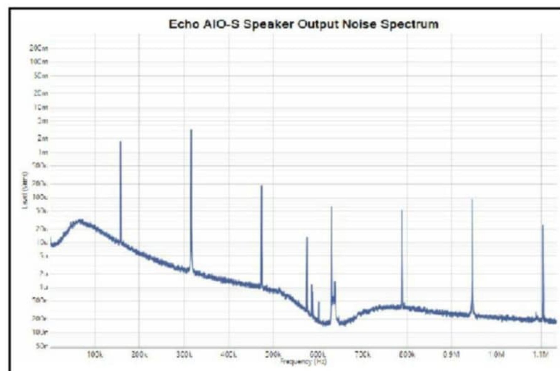
Figure 7: The output noise from the AIO-S power amplifiers is quite low in the ultrasonic range.
