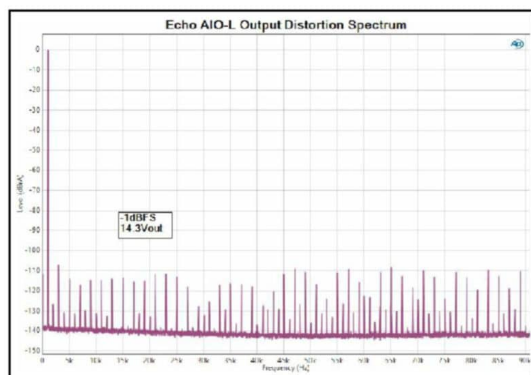
Figure 8: The output distortion of the AIO-L module at 1kHz and 14.3V shows a lot of high-order harmonics but at low level.
