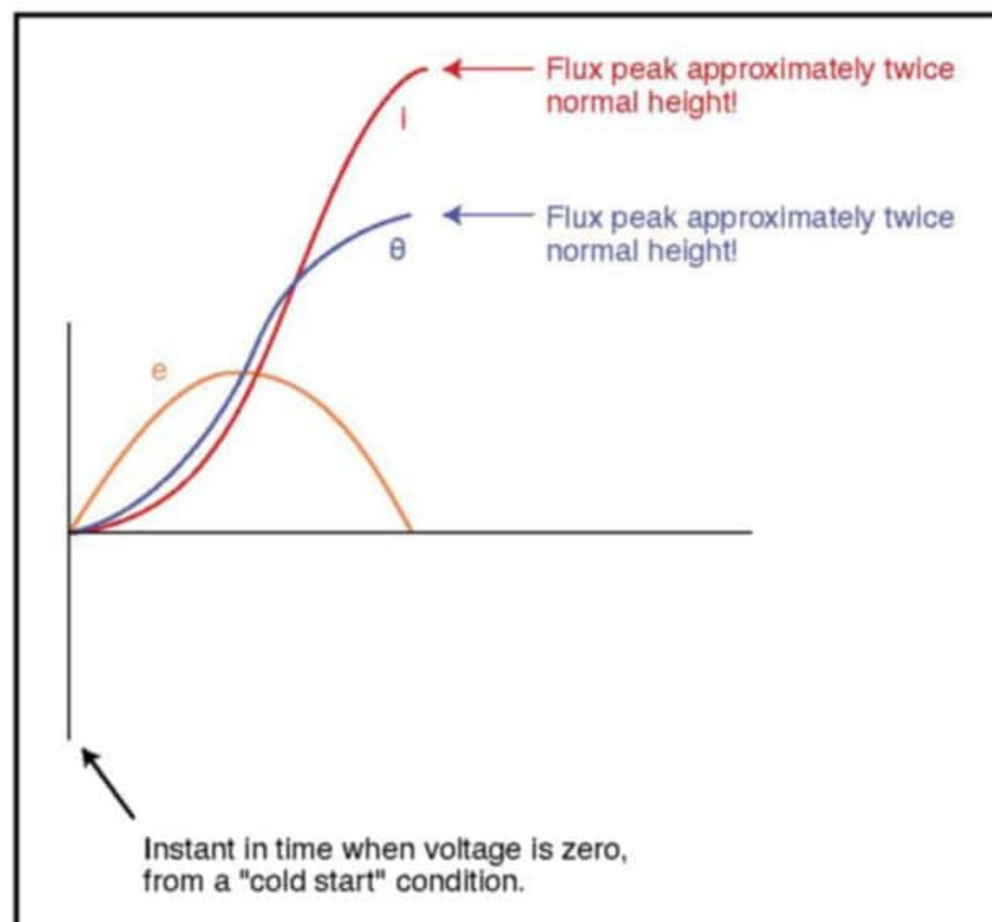
Figure 14: Transformer current when the AC voltage crosses zero (Image Source: All About Circuits)
