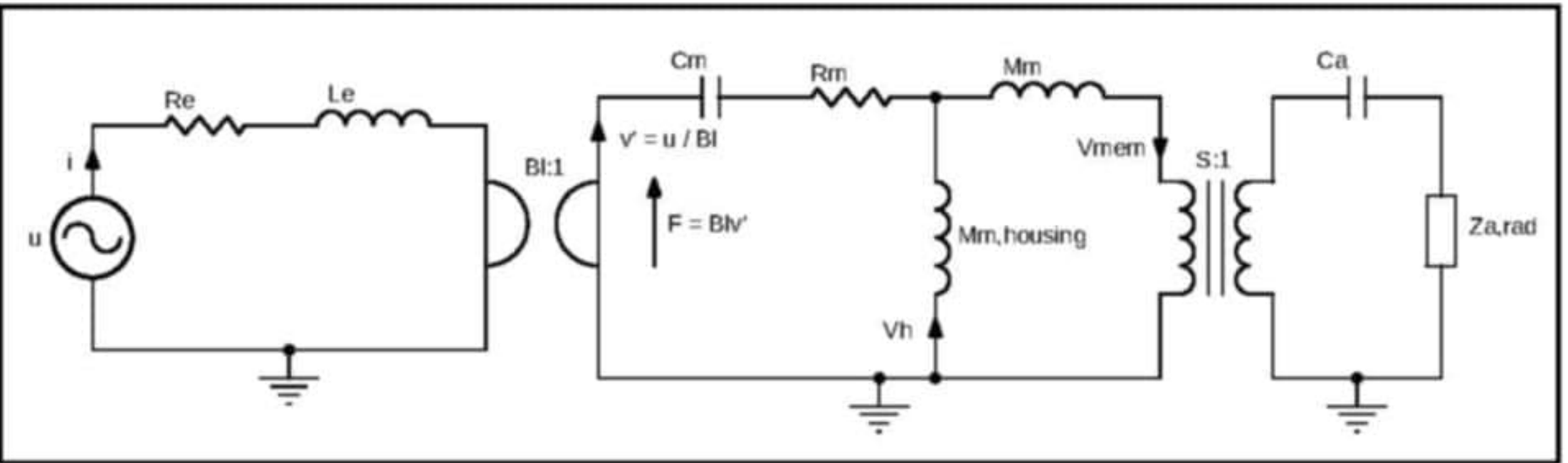
Figure 2: Analogy circuit for loudspeaker driver in a closed and mobile enclosure
