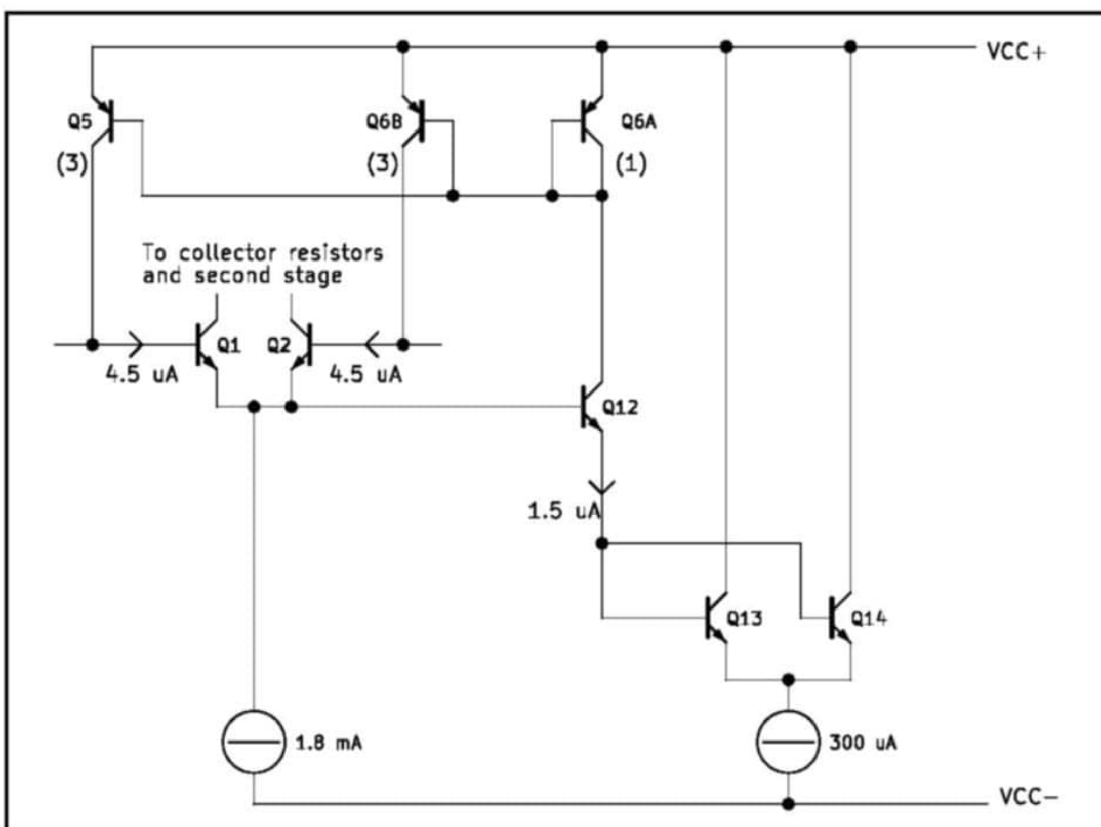
Figure 1: Simplified base current compensation of the LT1128/LT1028
