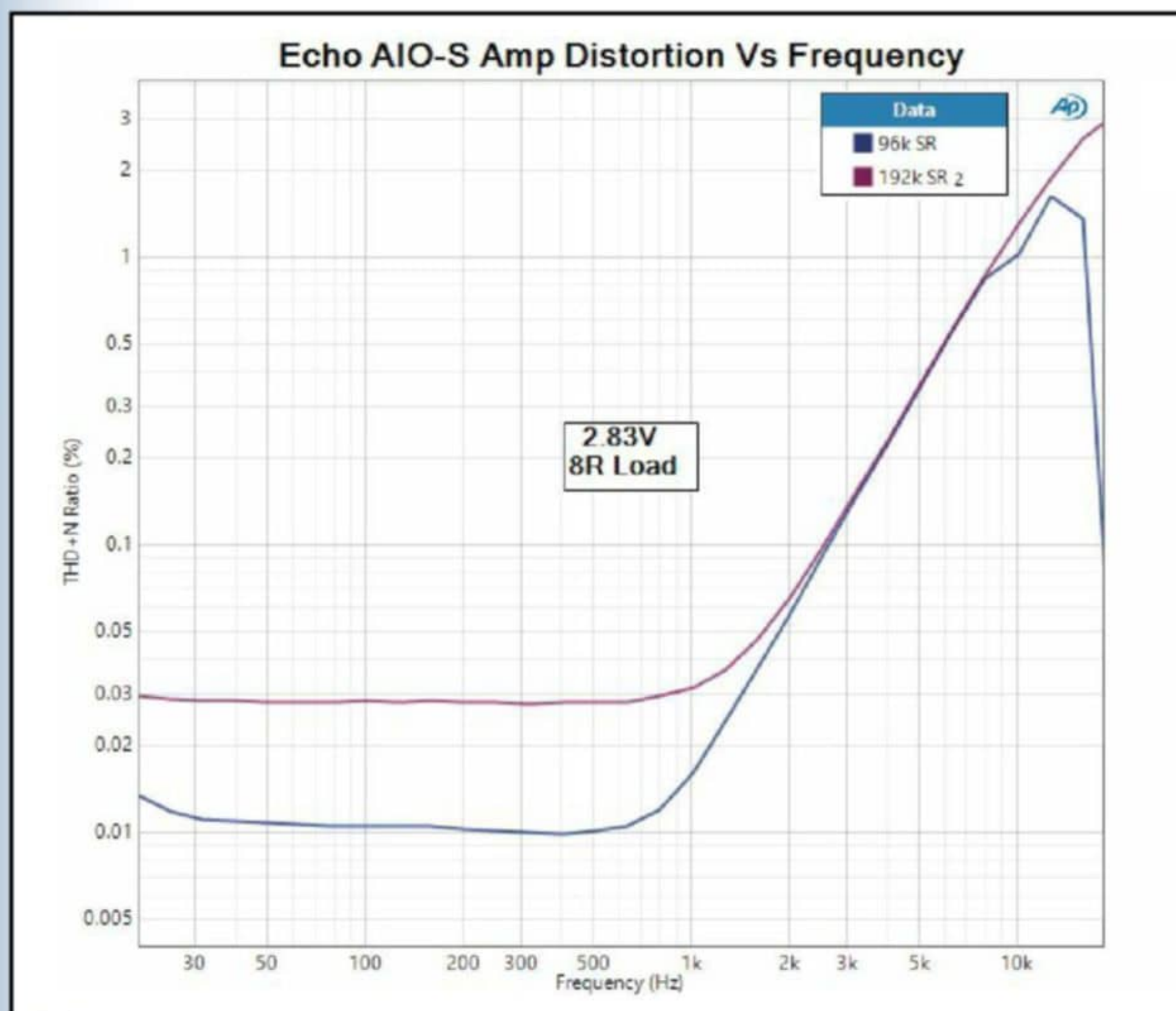
Figure 12: Distortion versus frequency for the AIO-S amplifier at 2.83V (1W) shows a very large increase at higher frequencies.
