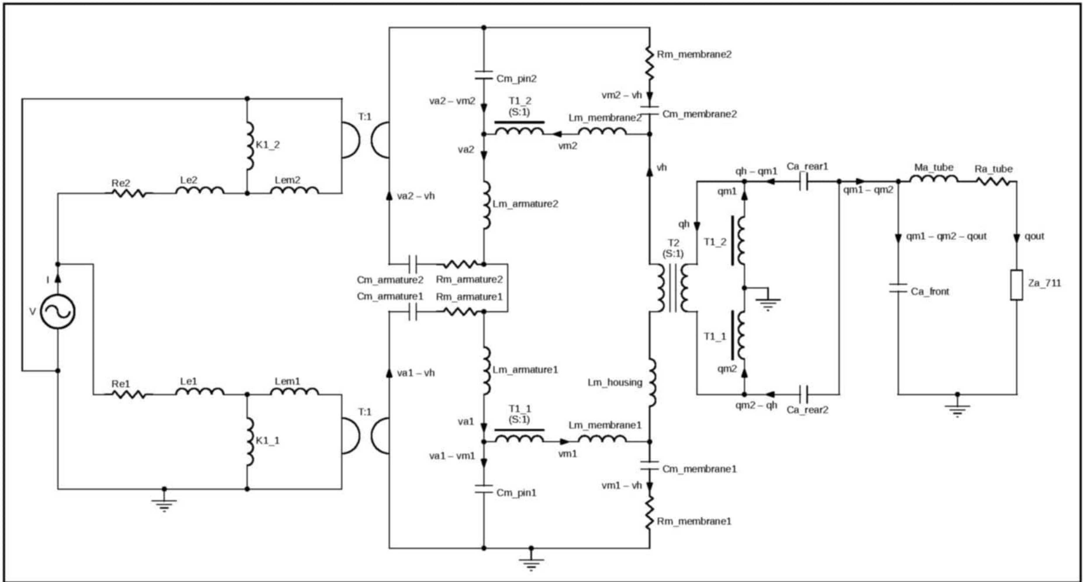
Figure 10: The principle lumped model for the Dual Balanced Armature Receiver
