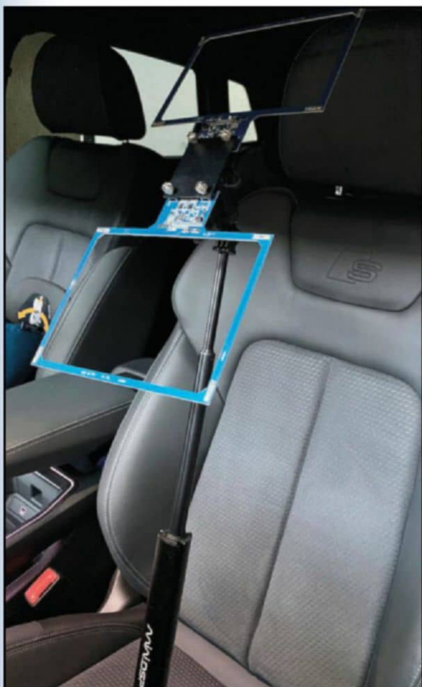
Photo 1: MiniDSP’s Umik-X is made for measurements with car cabins in mind. One group of 2x4 MEMS microphones form an array for one seat, thus increasing the resolution to the original six-point setup proposed by Geddes.
