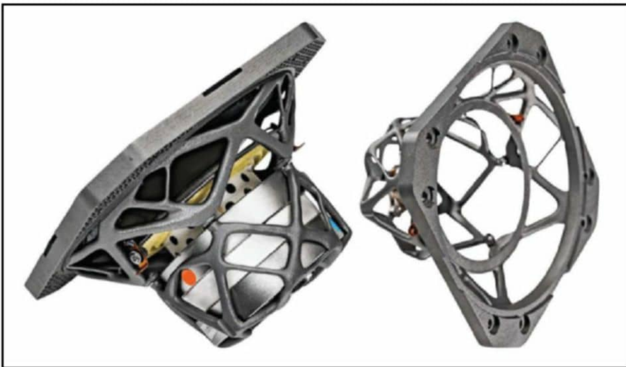
Figure 3: Børrensen's mechanical topology optimized basket for the M1 bass/midrange unit [1]
