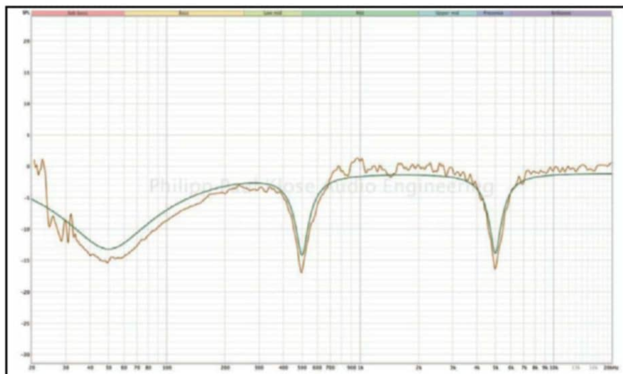
Figure 4: Filter reconstruction measurement. In the acoustical sound field, the applied filter (green) is shown vs. the reconstructed filter from the Umik-X array. The error is 2dB.
