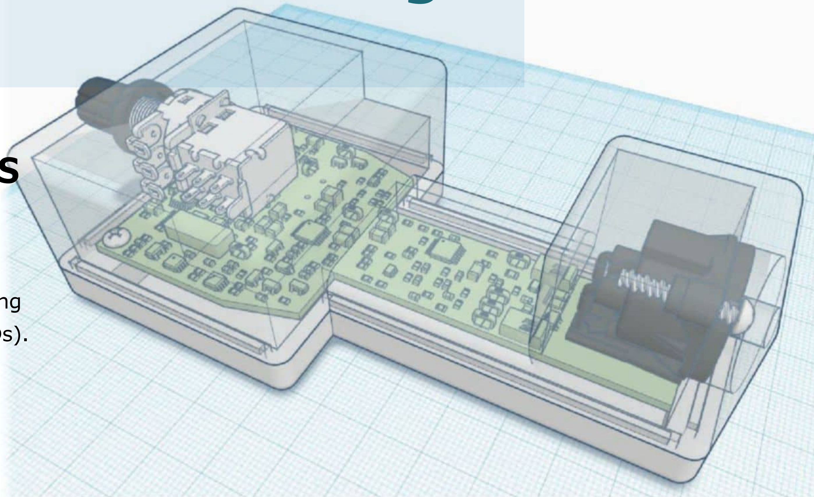
Engineer Julia Truchsess designed and 3D-printed this prototype microphone case.
