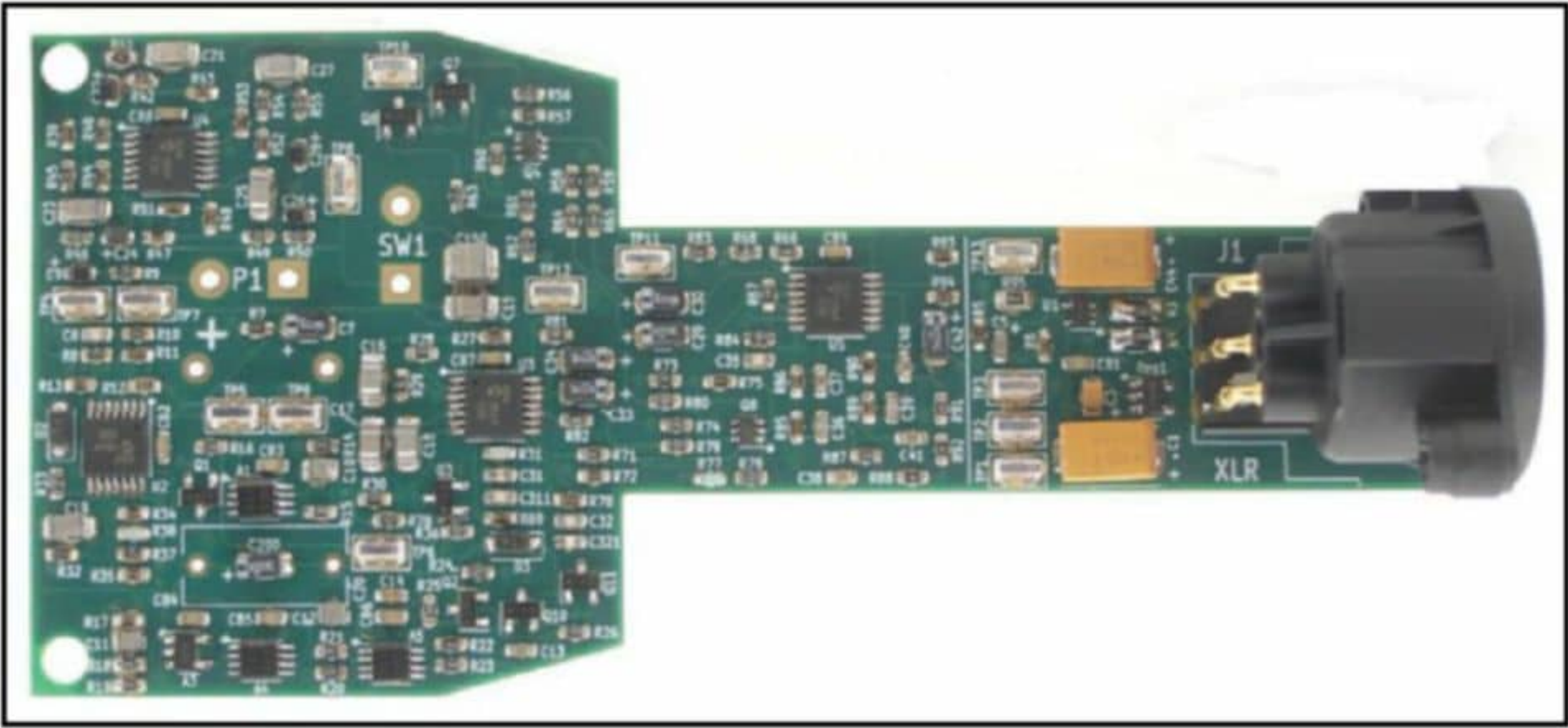
Photo 6: This is the finished board in all its glory. With nearly 200 parts packed so tightly, there’s no room for a solid copper fill between the traces as on the bottom layer in Figure 9.
