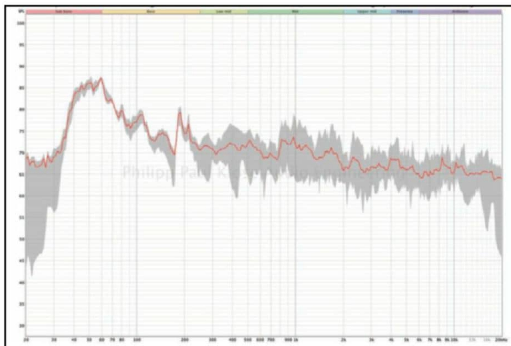
Figure 3: An array measurement. The average of all measurements (red) and minimum/maximum variations are shown as a grey tube around the average.
